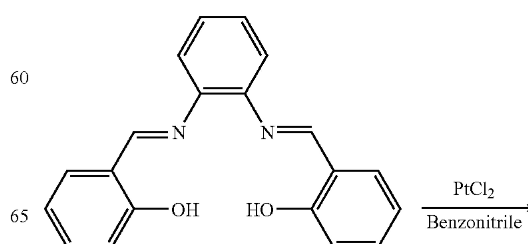
Synthesis scheme-2
