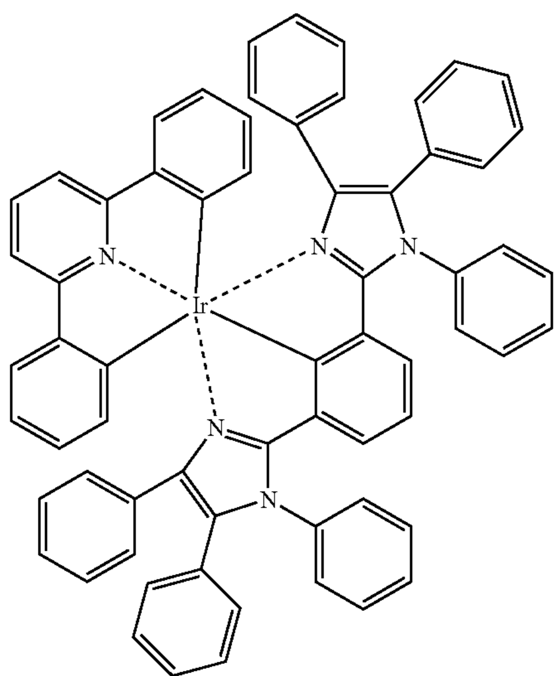
Compound (177)
