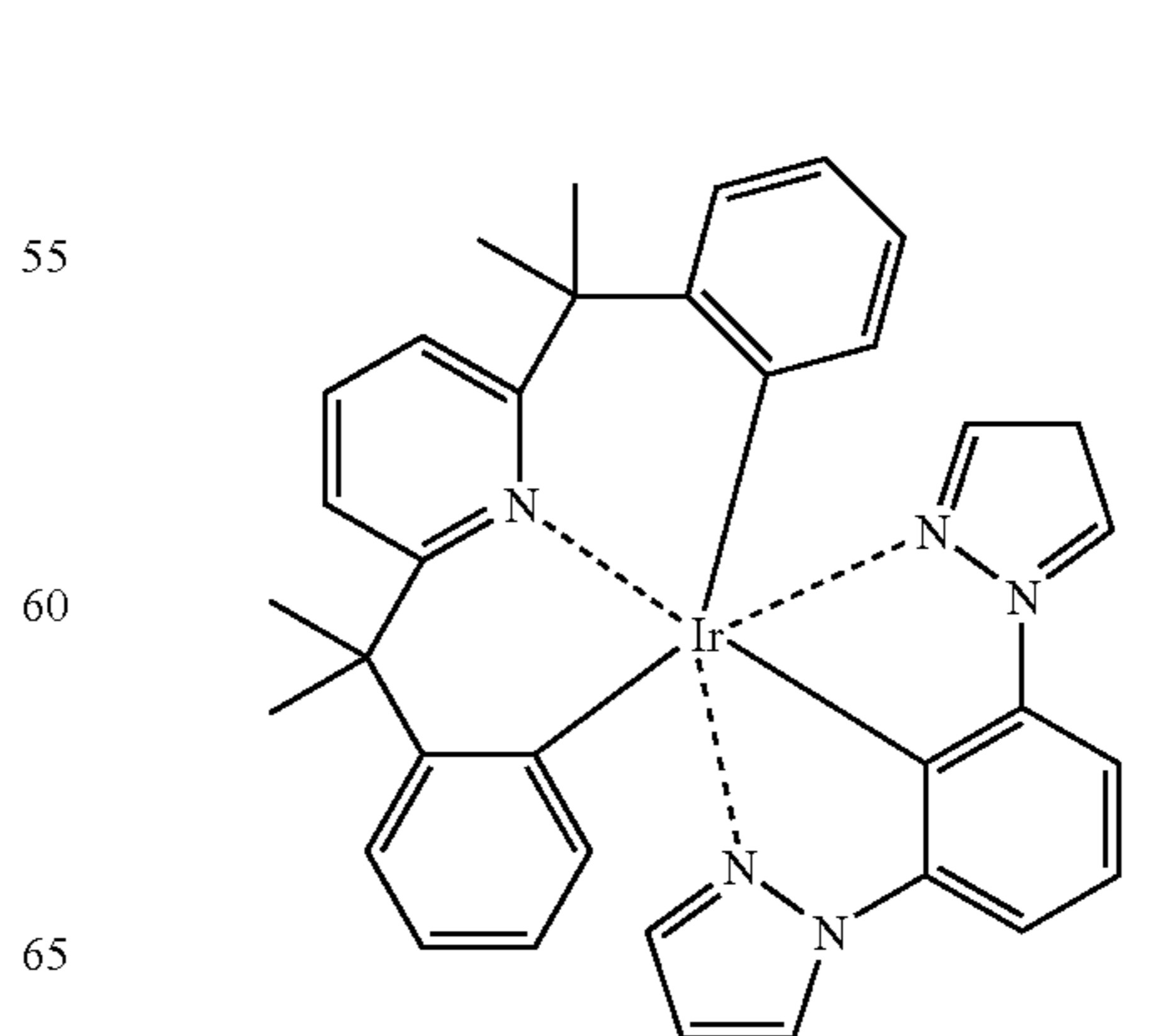
Compound (159)
