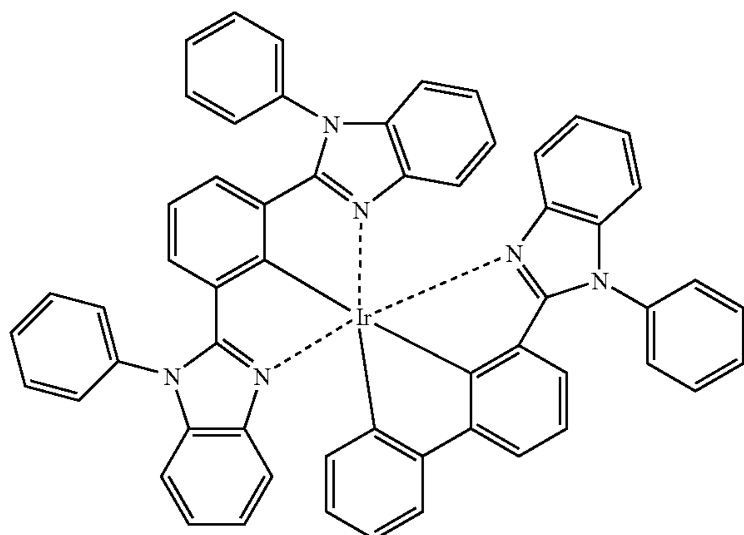
Compound (126)
