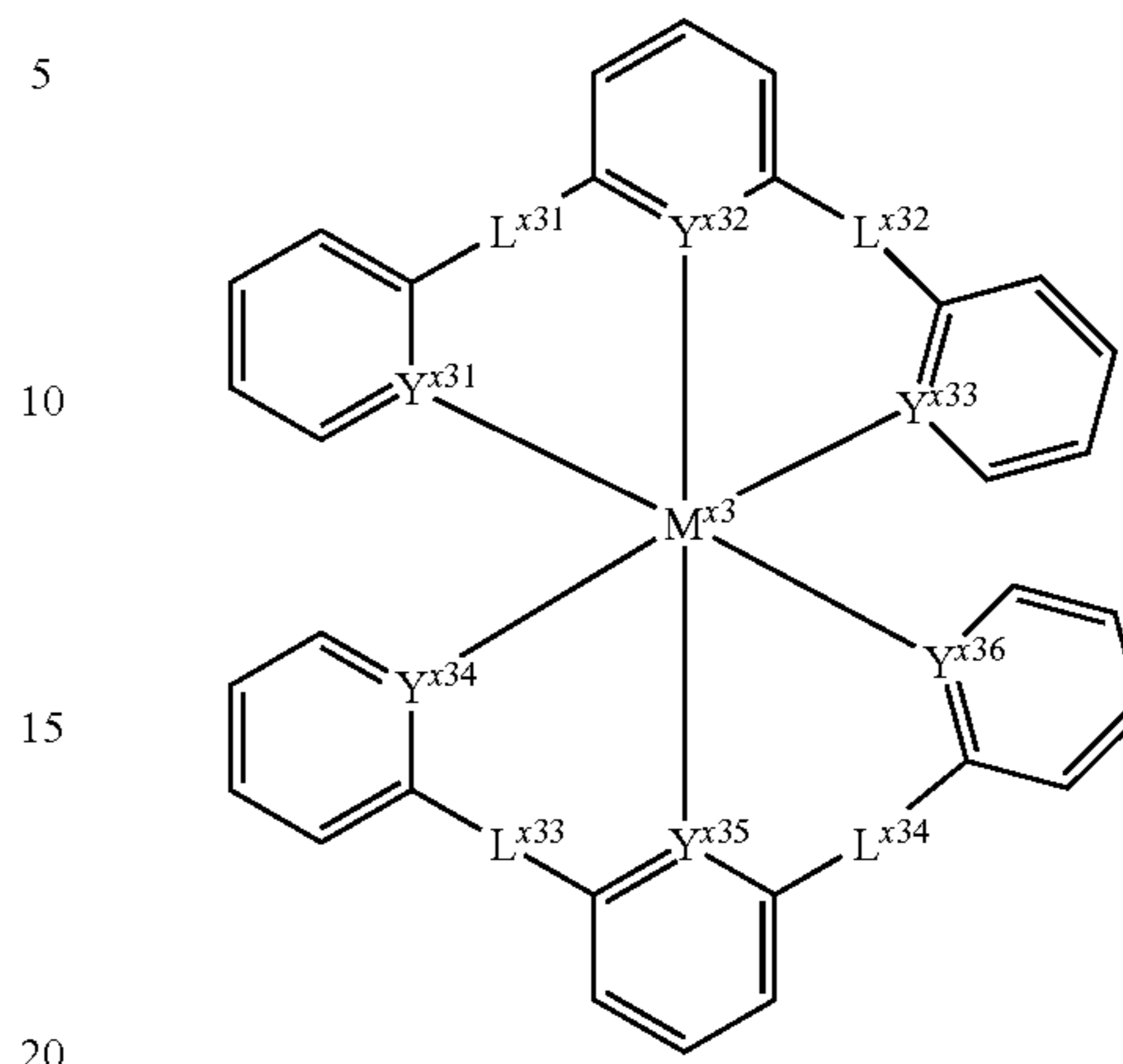
formula (X1)
