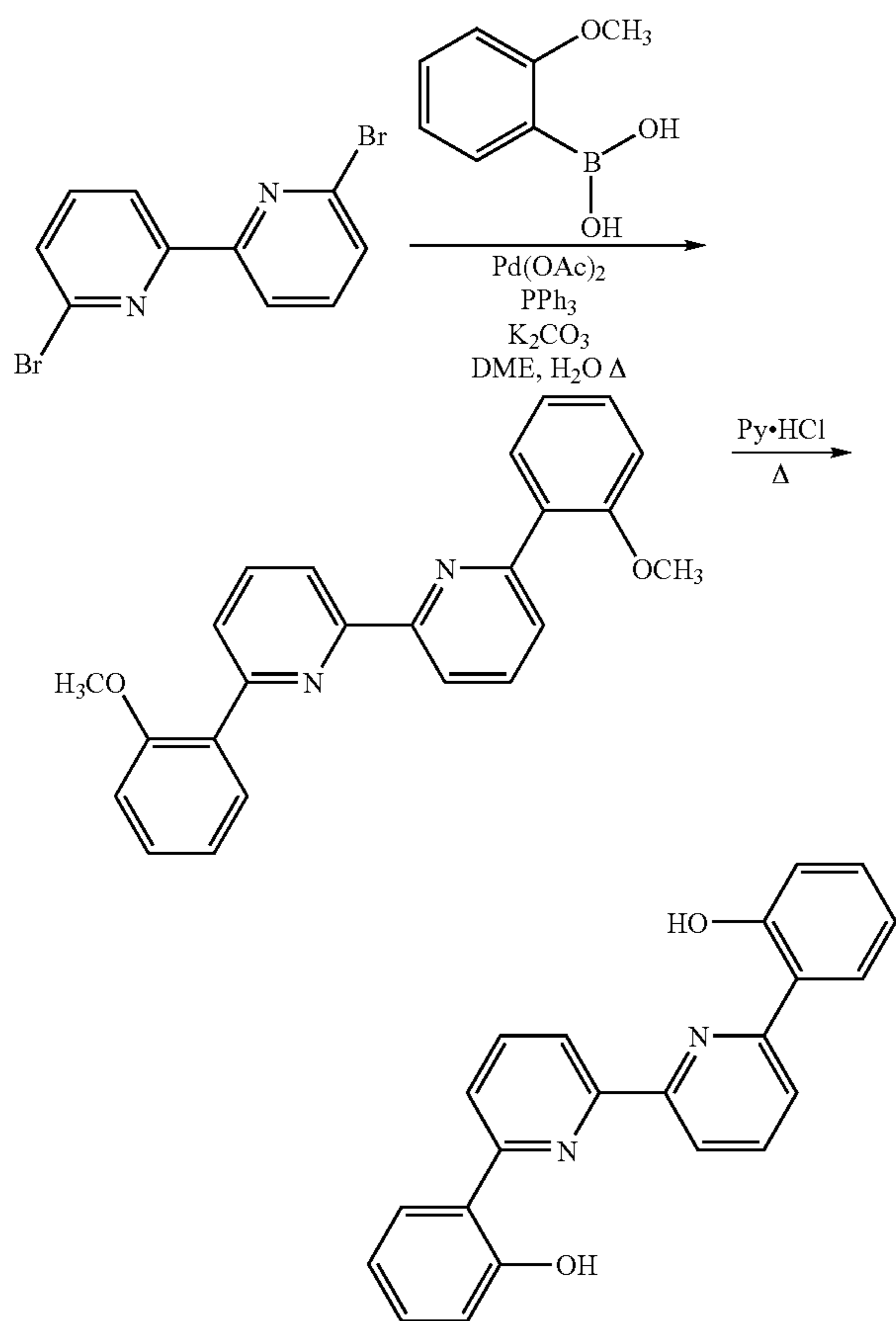
Synthesis of 6,6'-bis(2-methoxyphenyl)-2,2'-bipyridyl
