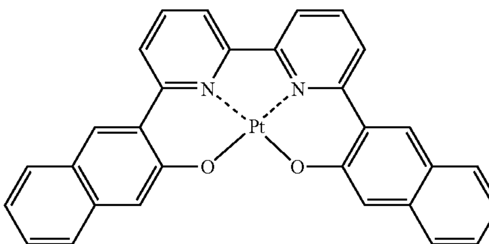
Compound (22)
