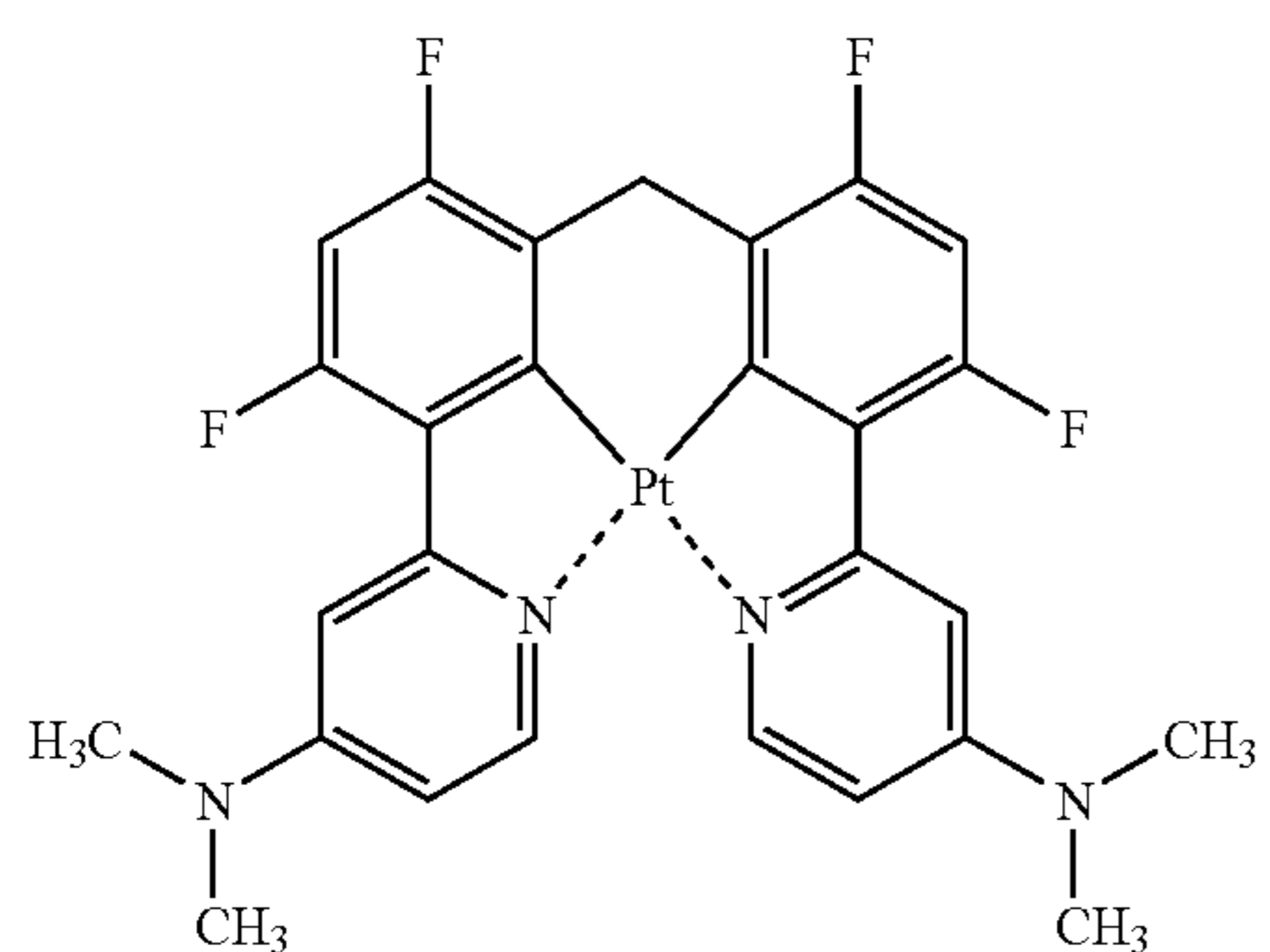
Compound (40)
