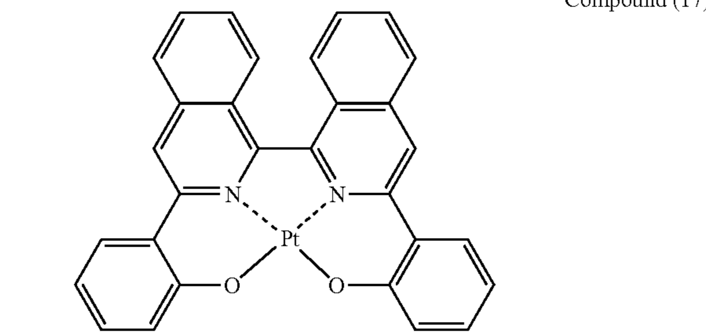
Compound (18)
