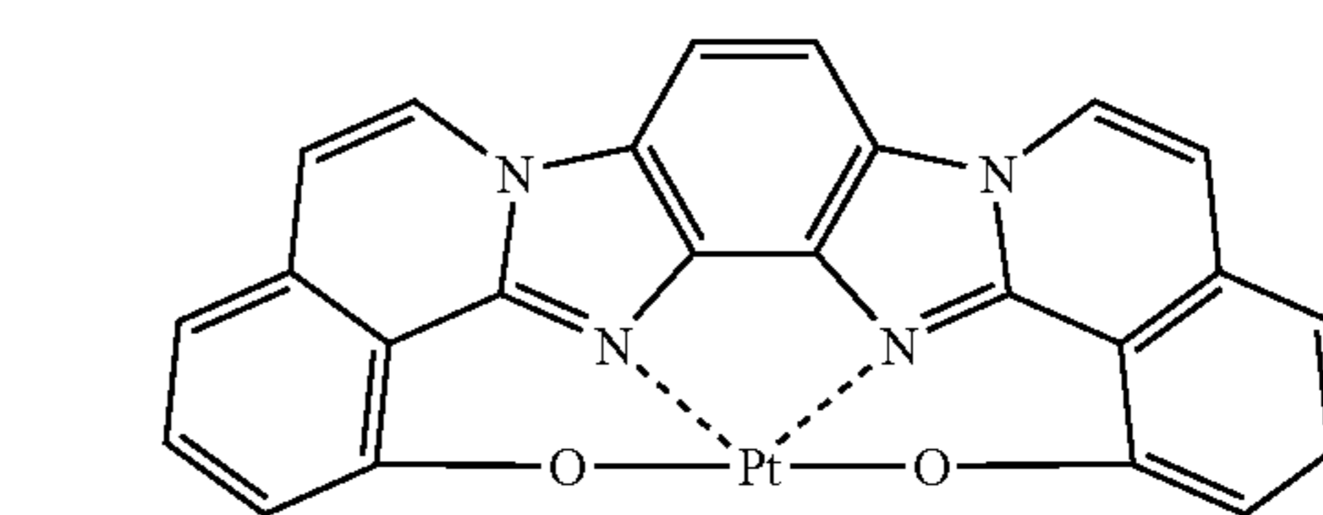
Compound (184)
