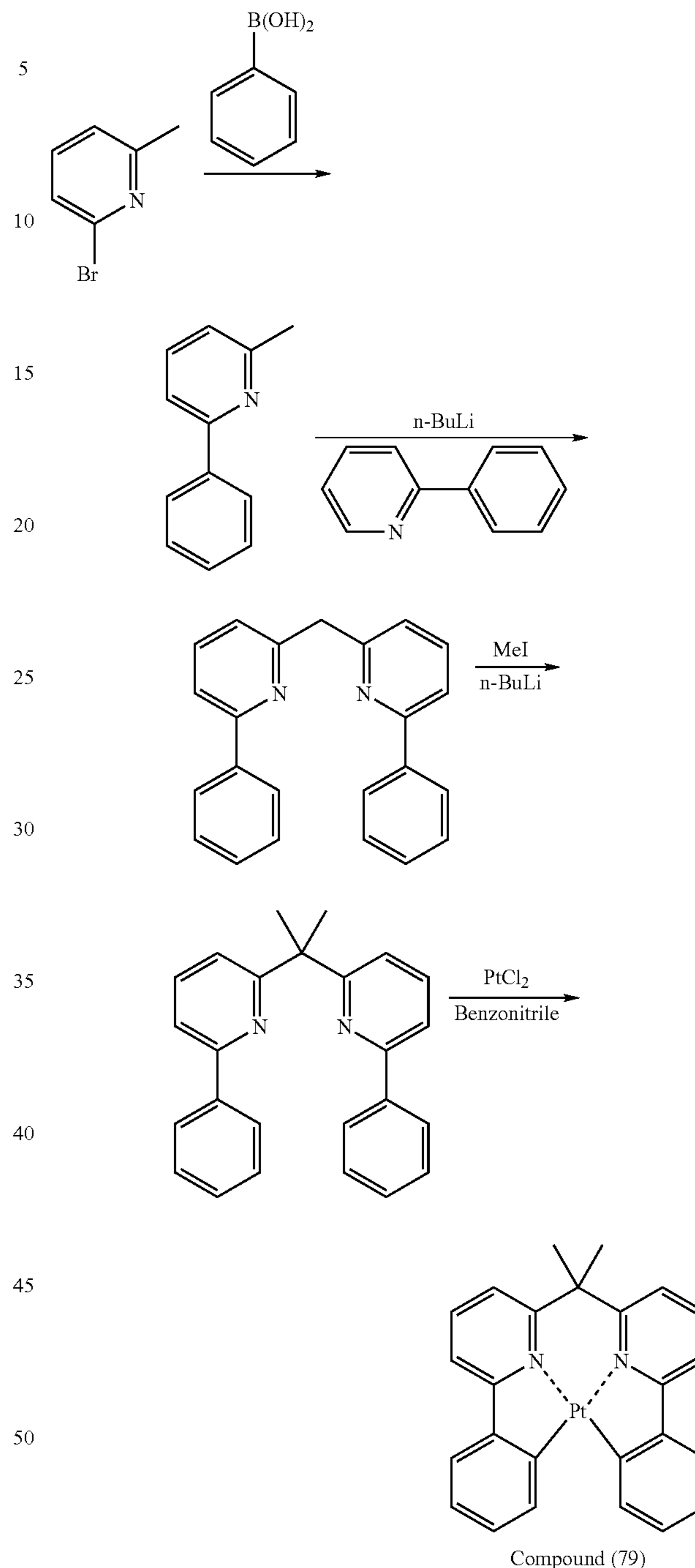
Synthesis scheme-1
