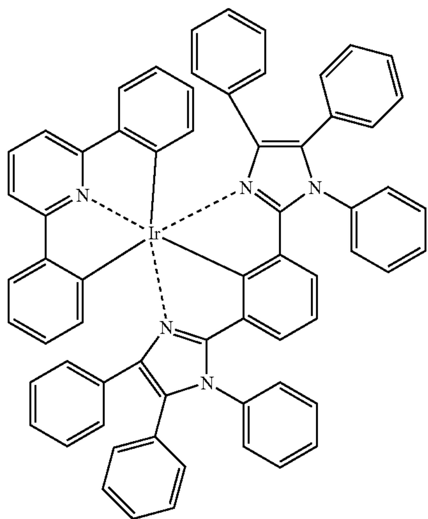
Compound (177)
