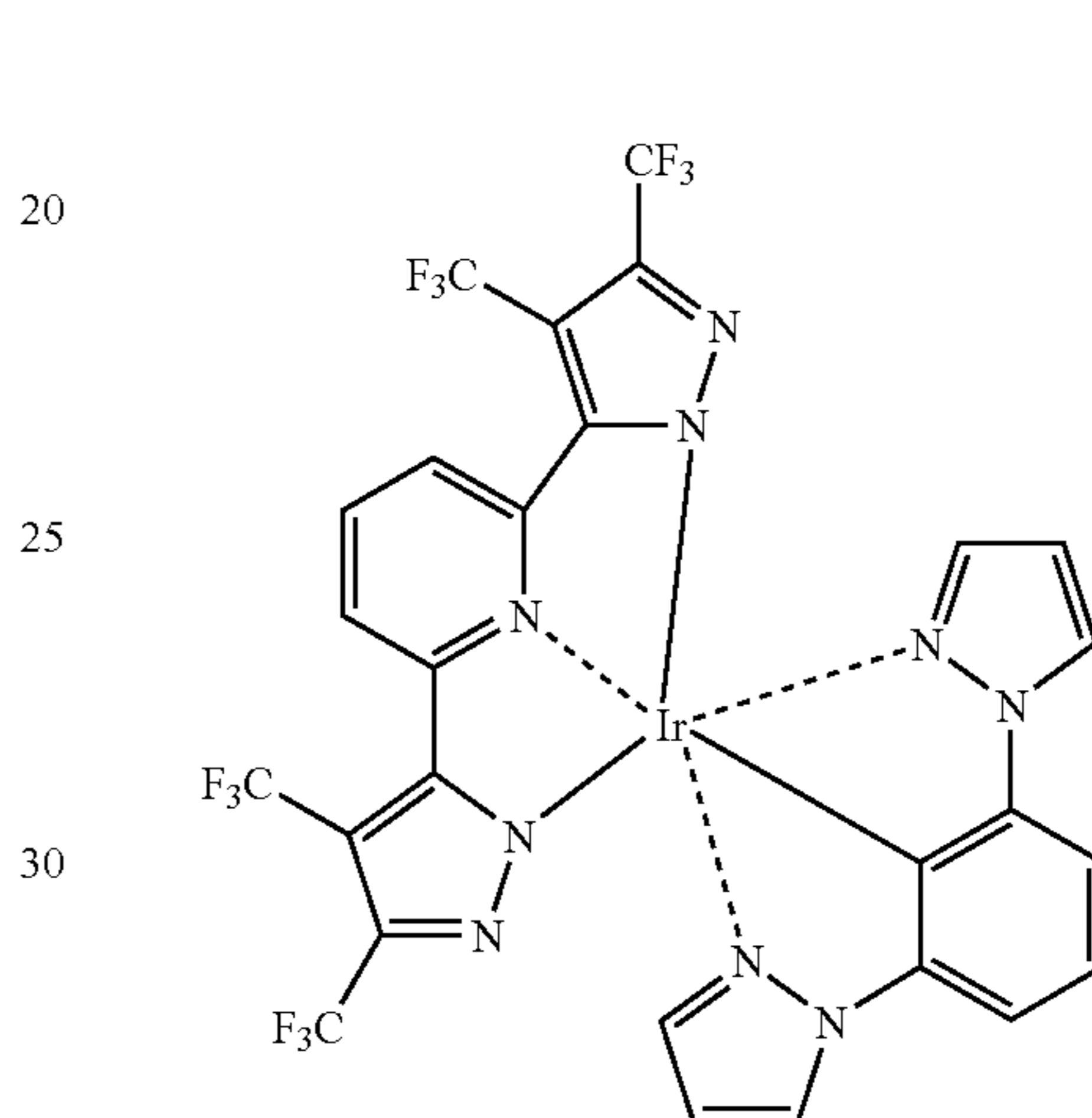
Compound (154)
