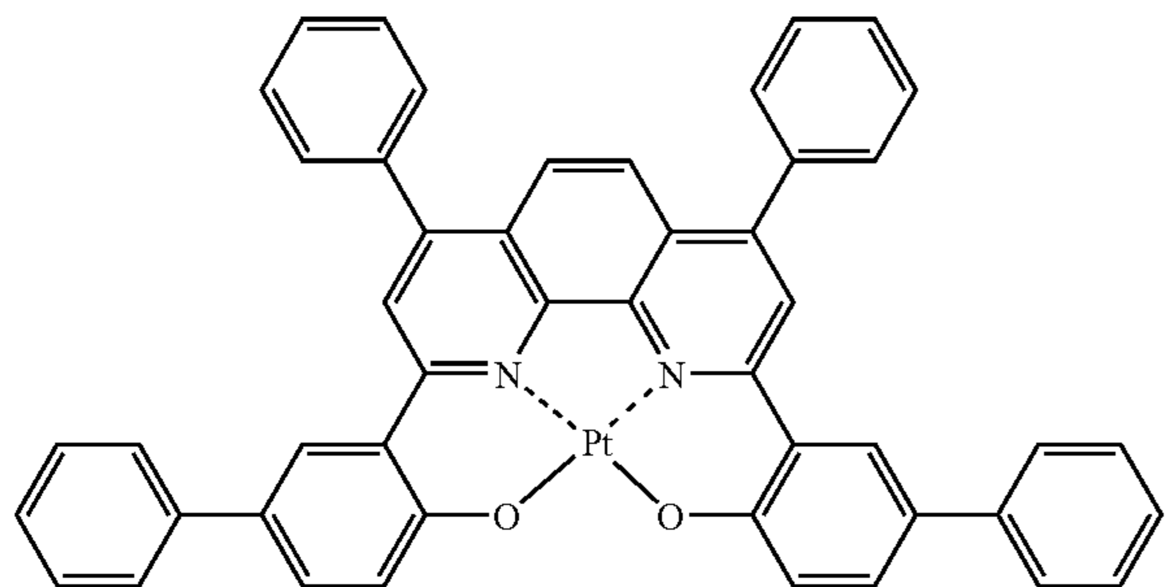
Compound (17)
