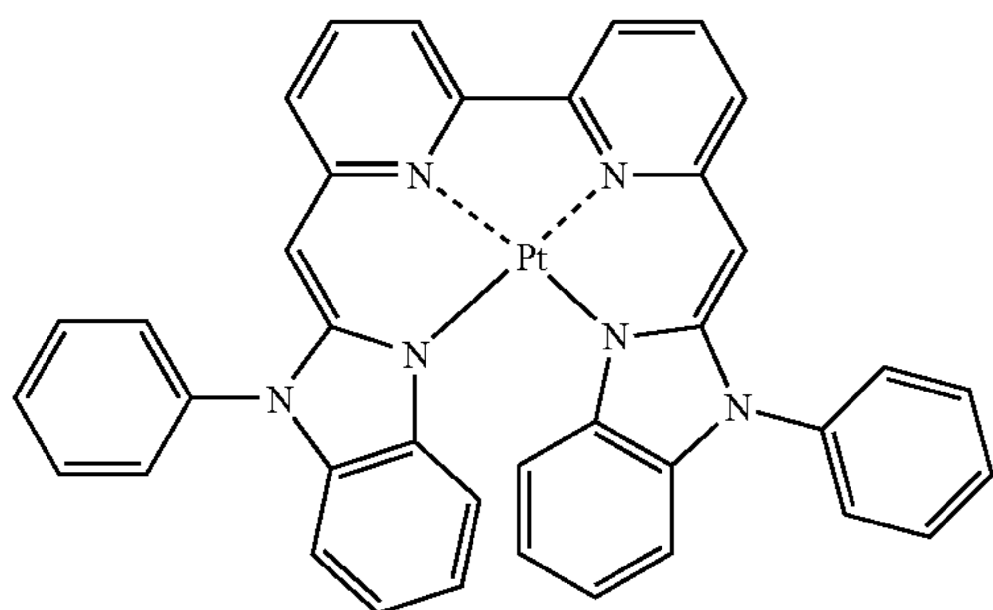
Compound (29)
