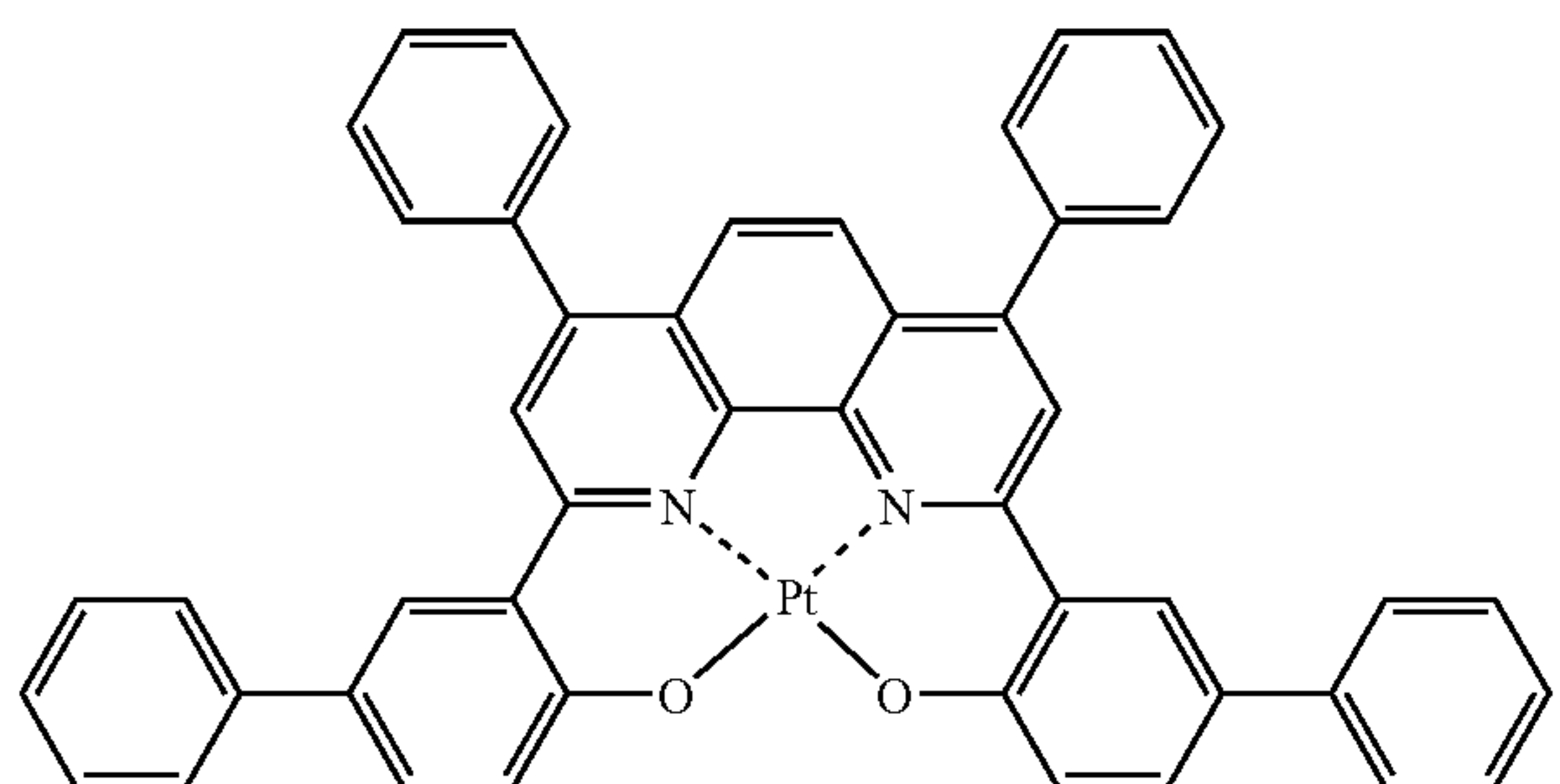
Compound (17)
