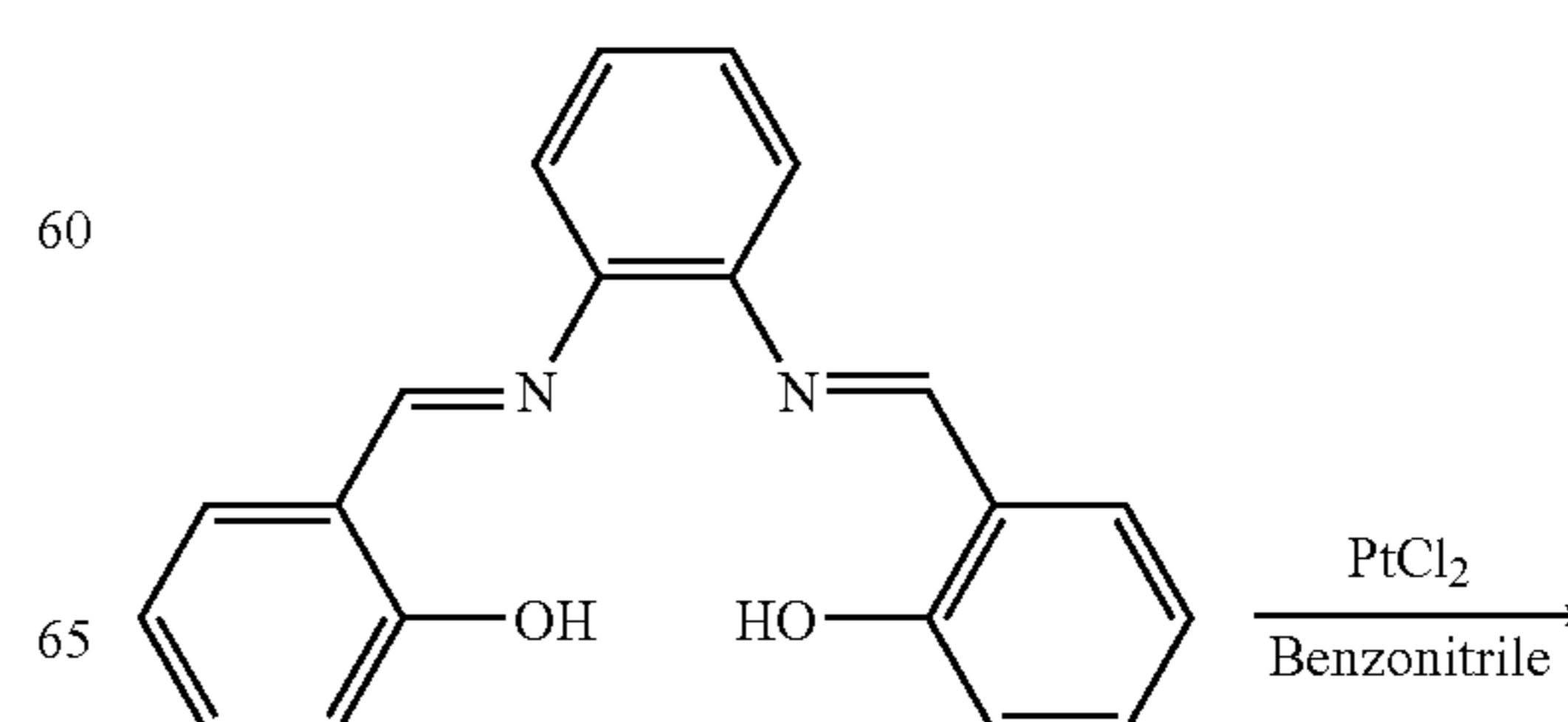
Synthesis scheme-2
