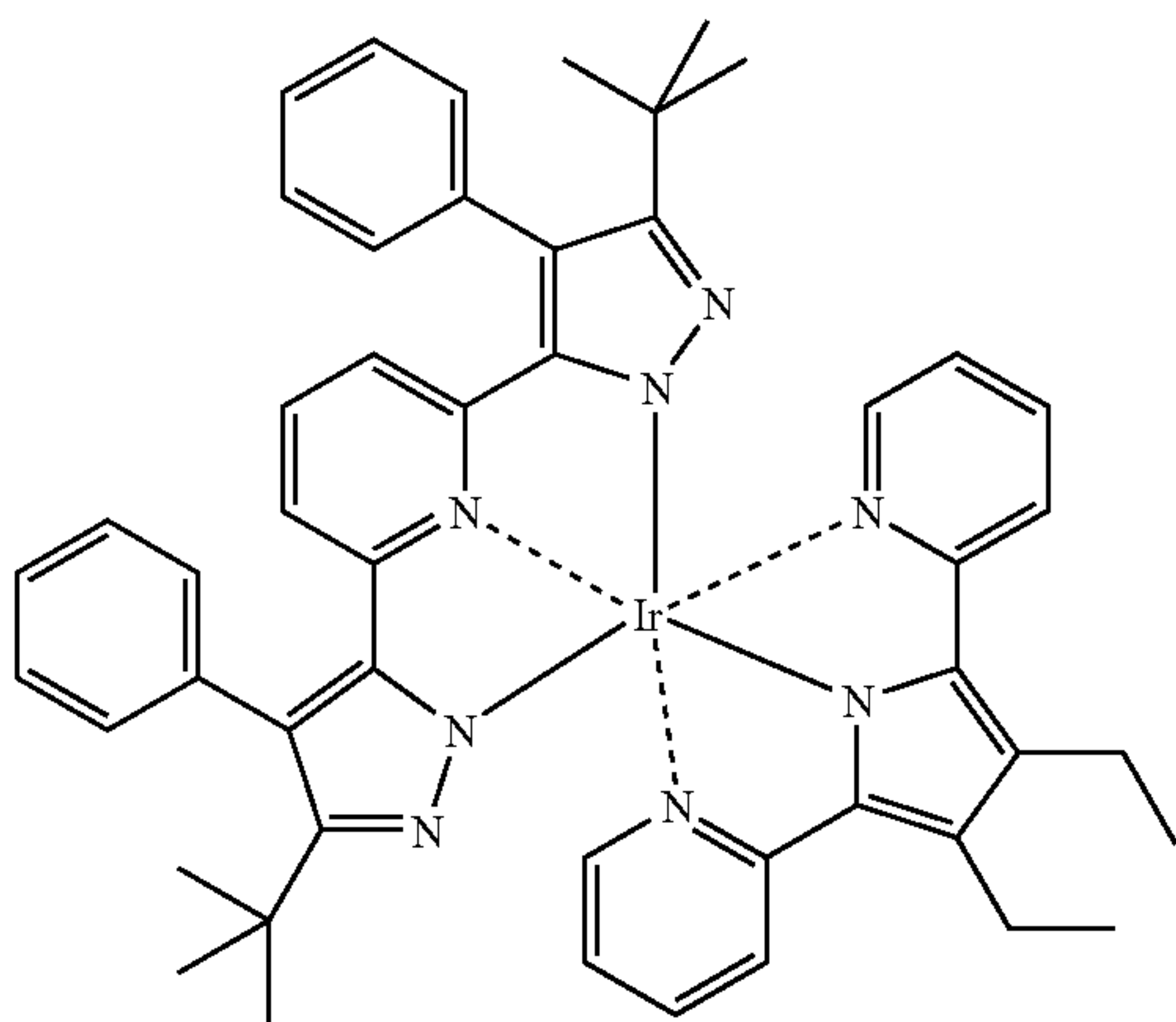
Compound (154)
