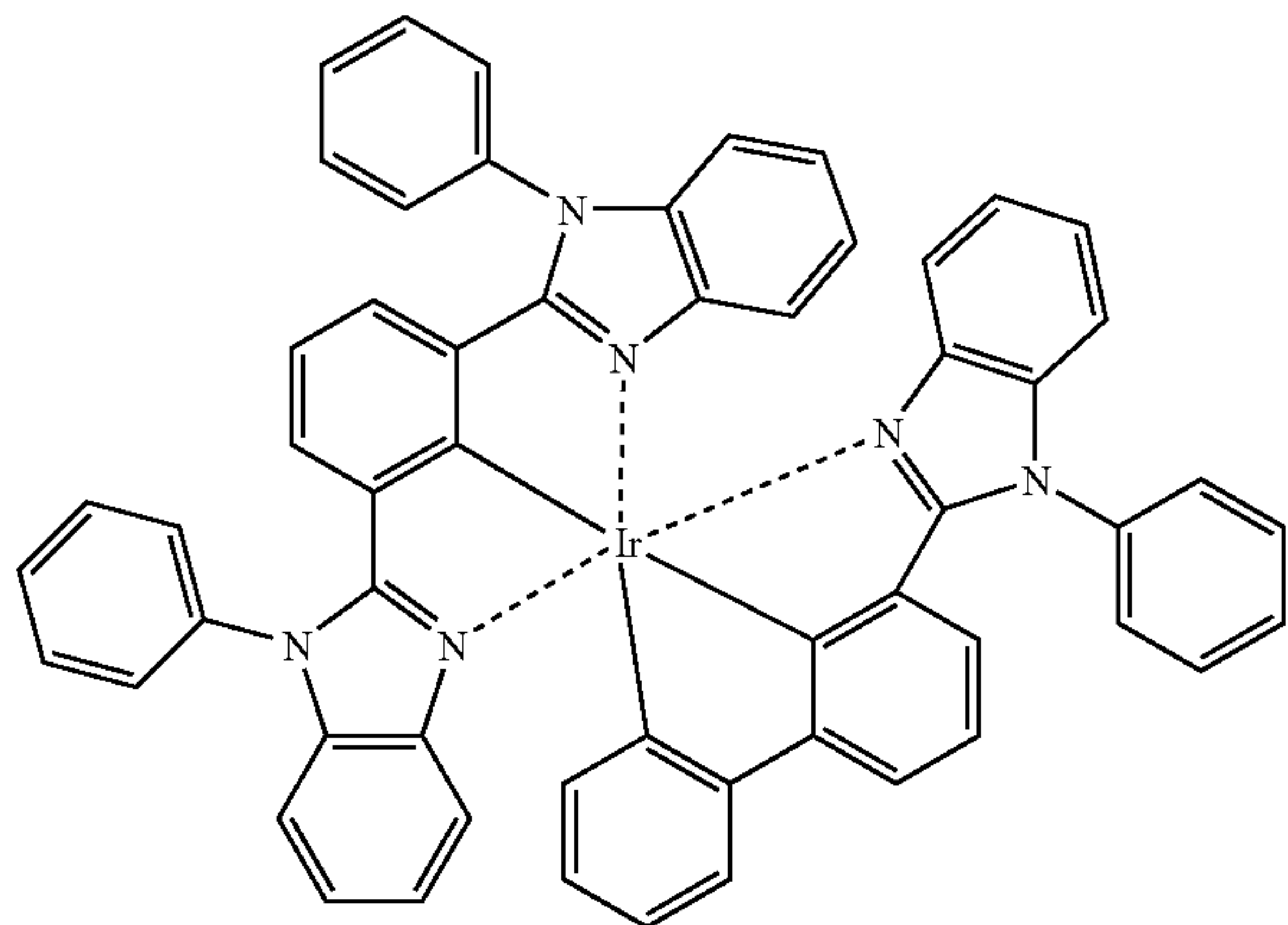
Compound (126)
