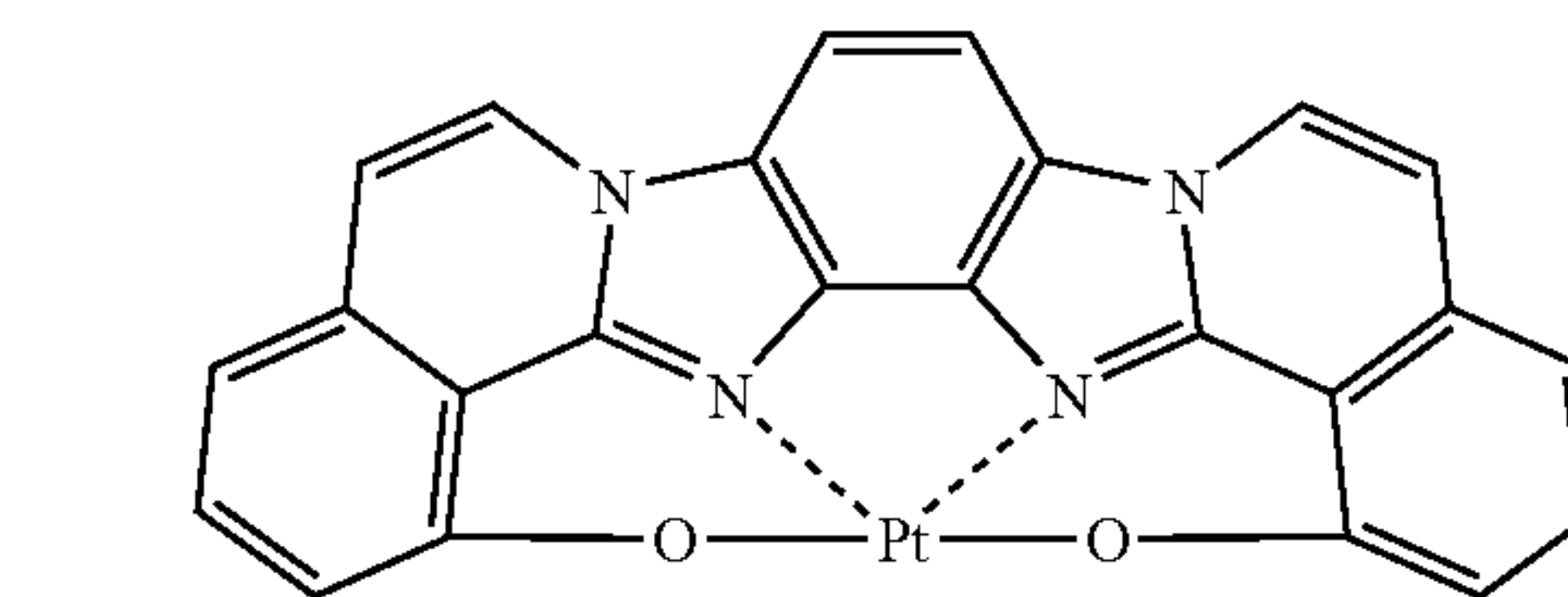
Compound (184)
