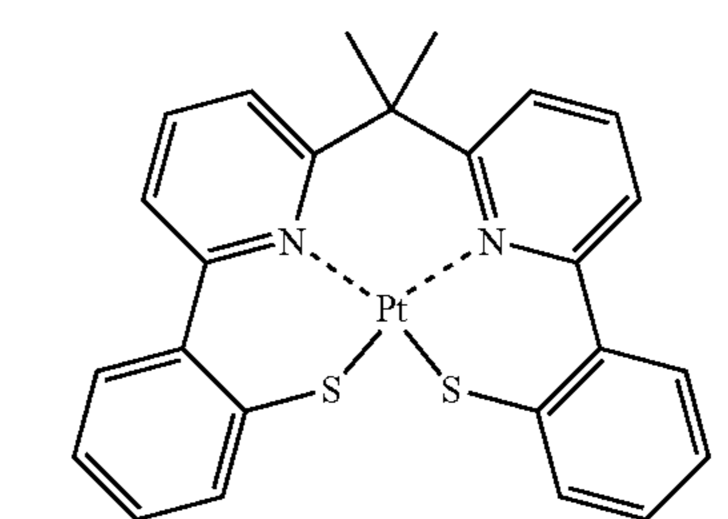
Compound (68)
