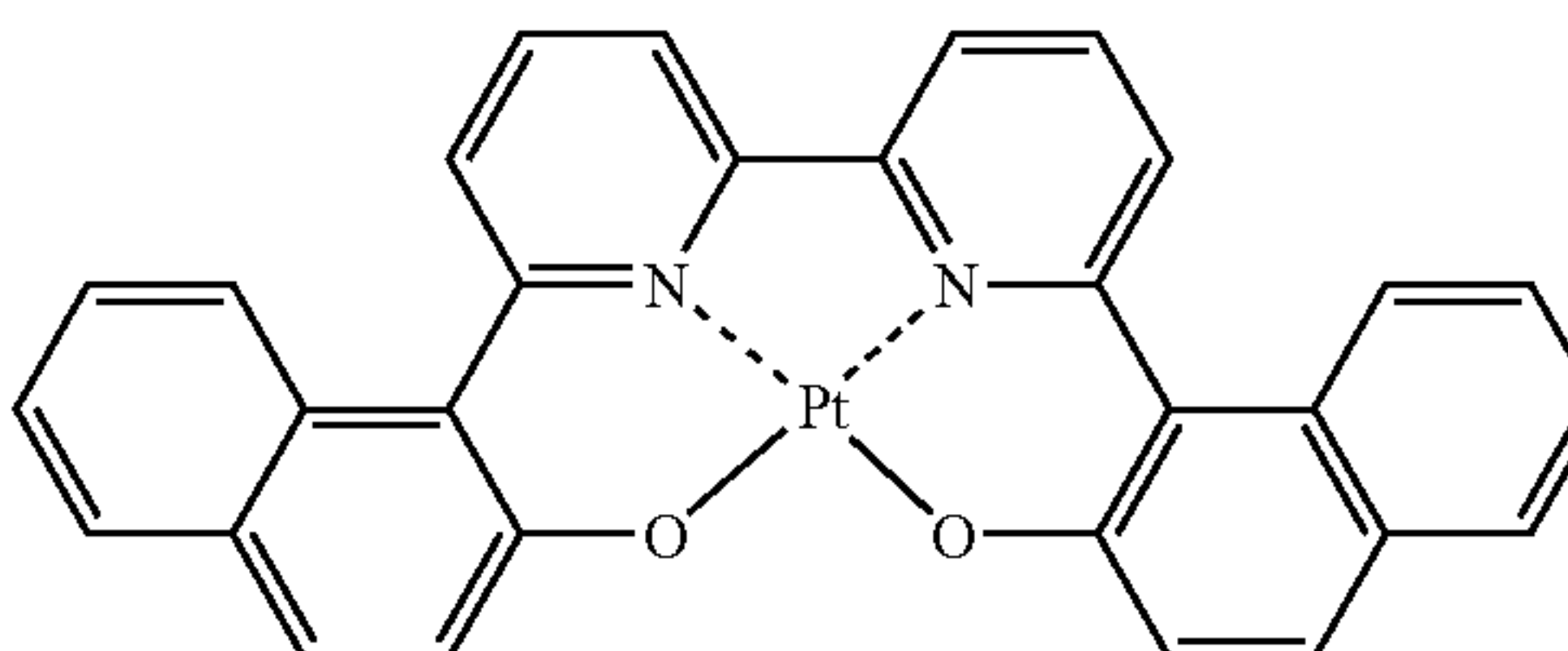
Compound (21)
