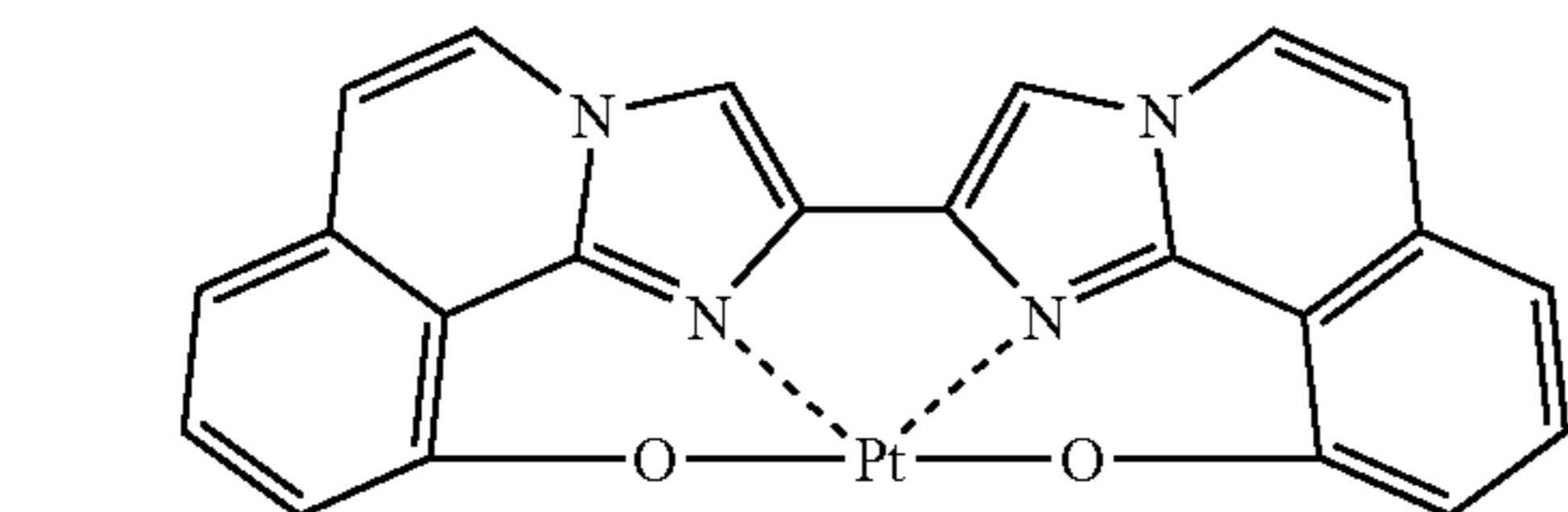
Compound (190)
