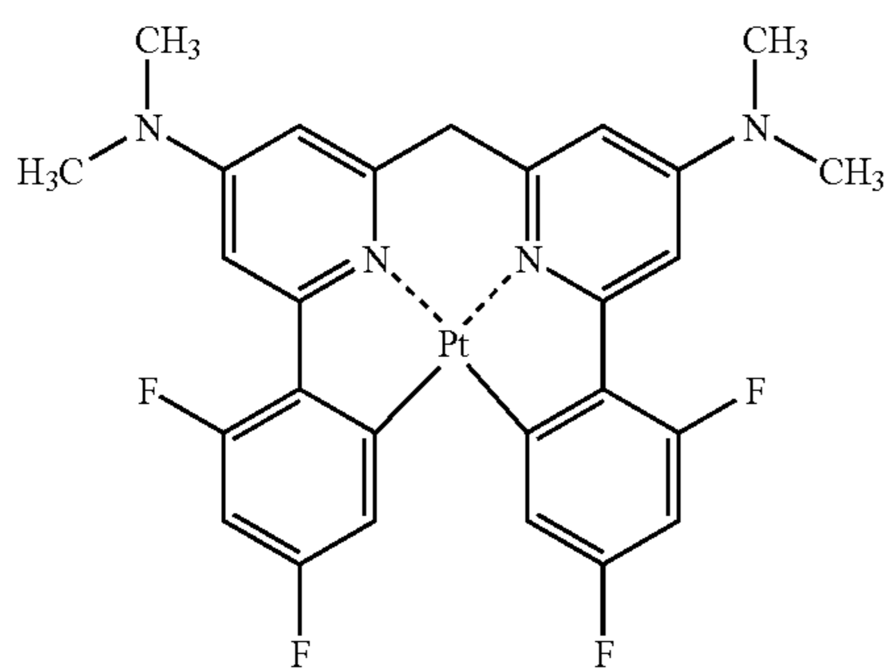
Compound (59)
