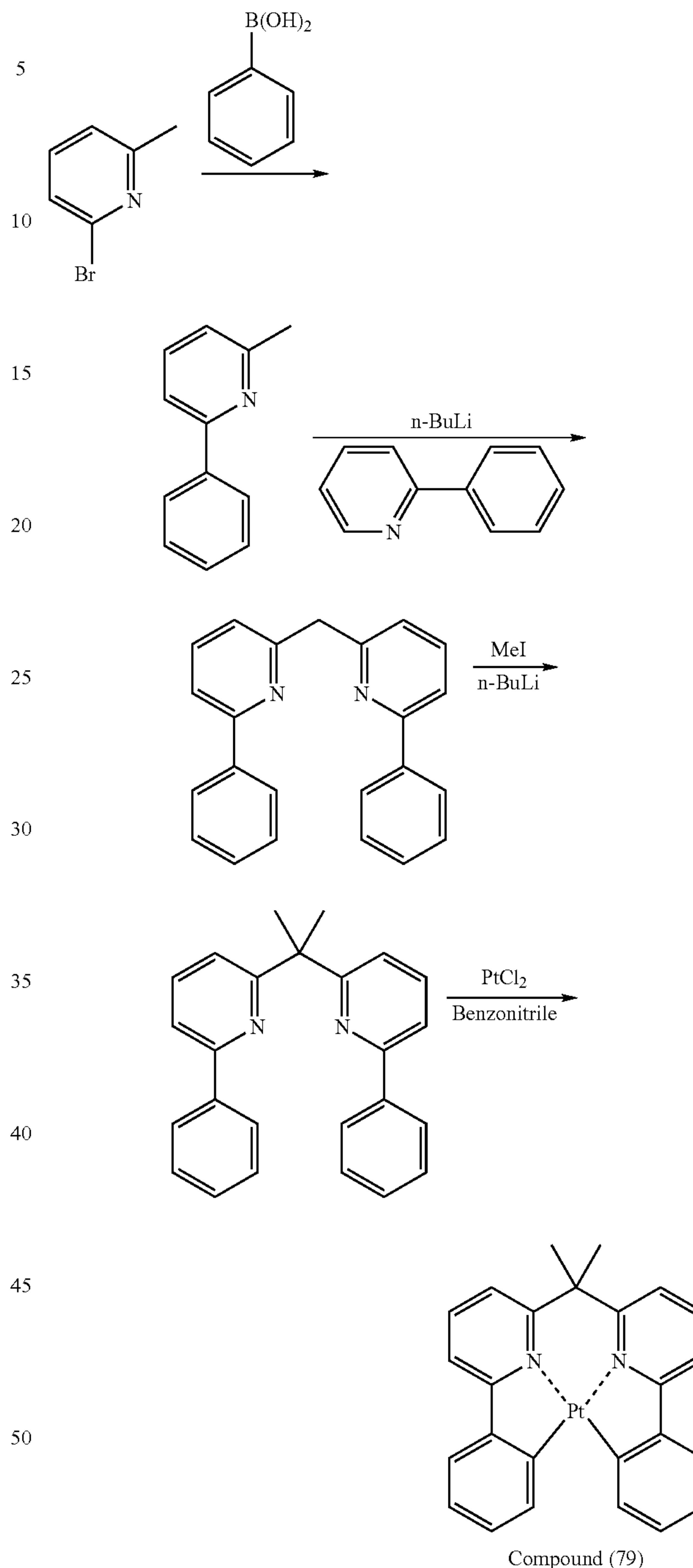
Synthesis scheme-1
