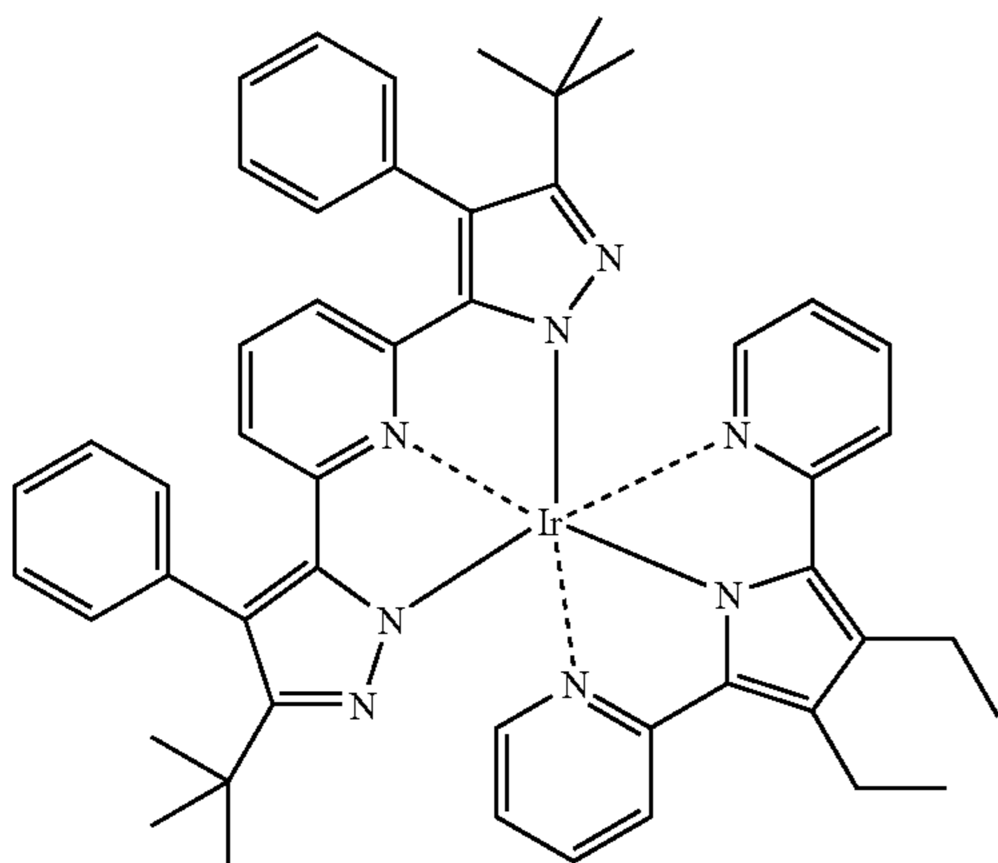
Compound (154)
