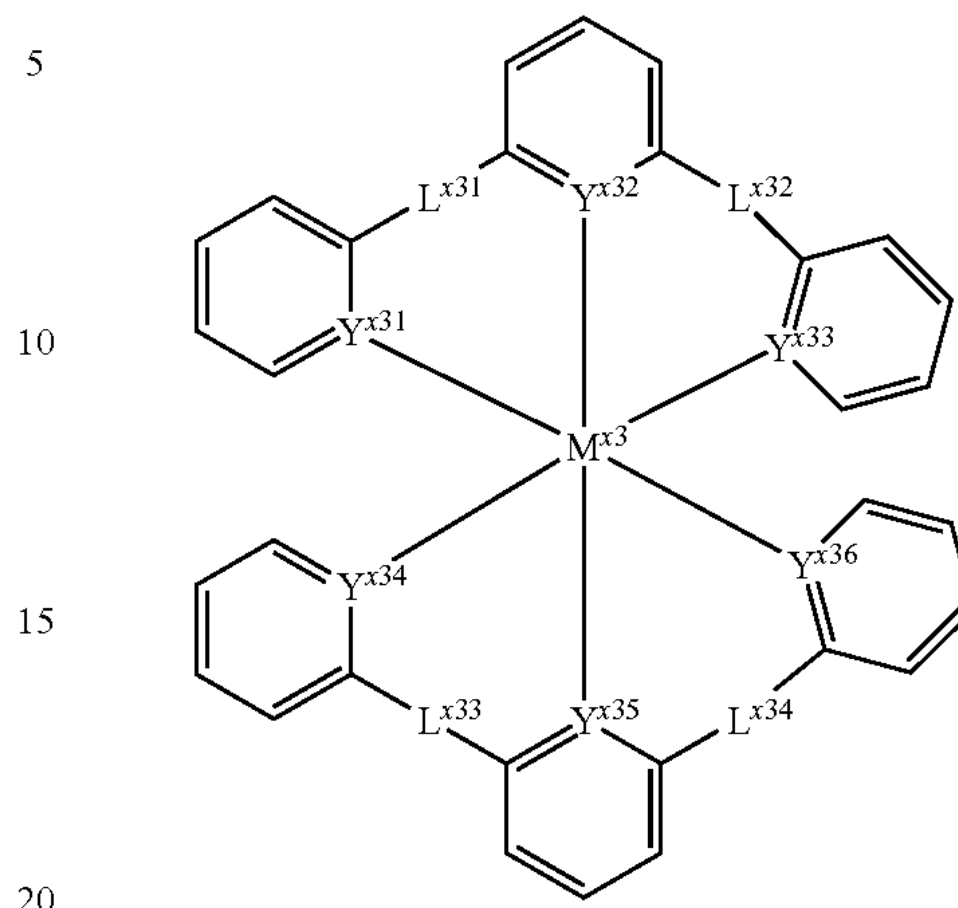
formula (X1)
