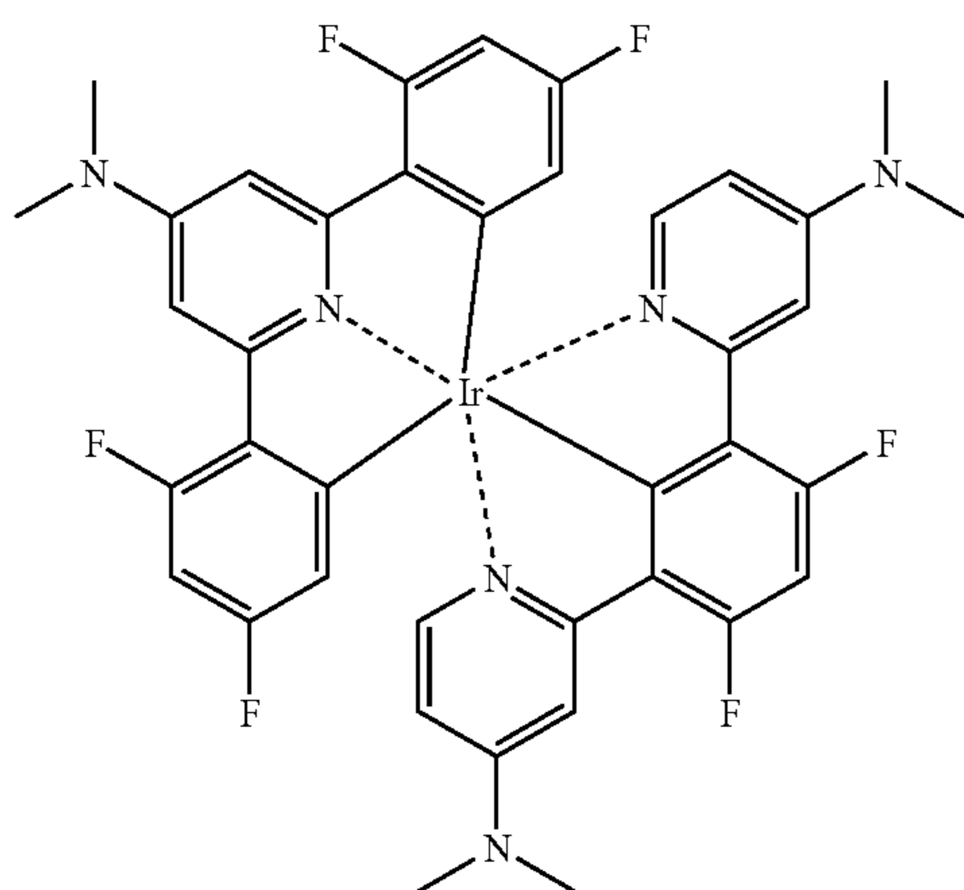
Compound (104)
