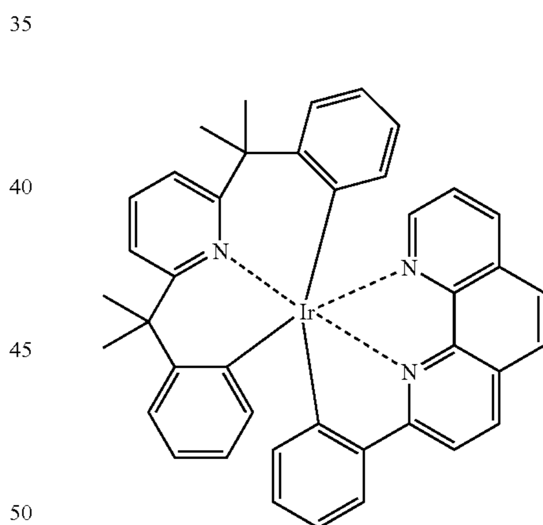
Compound (158)
