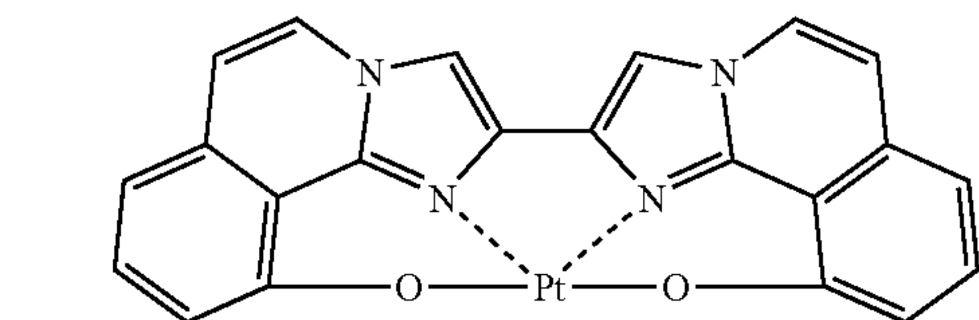
Compound (190)
