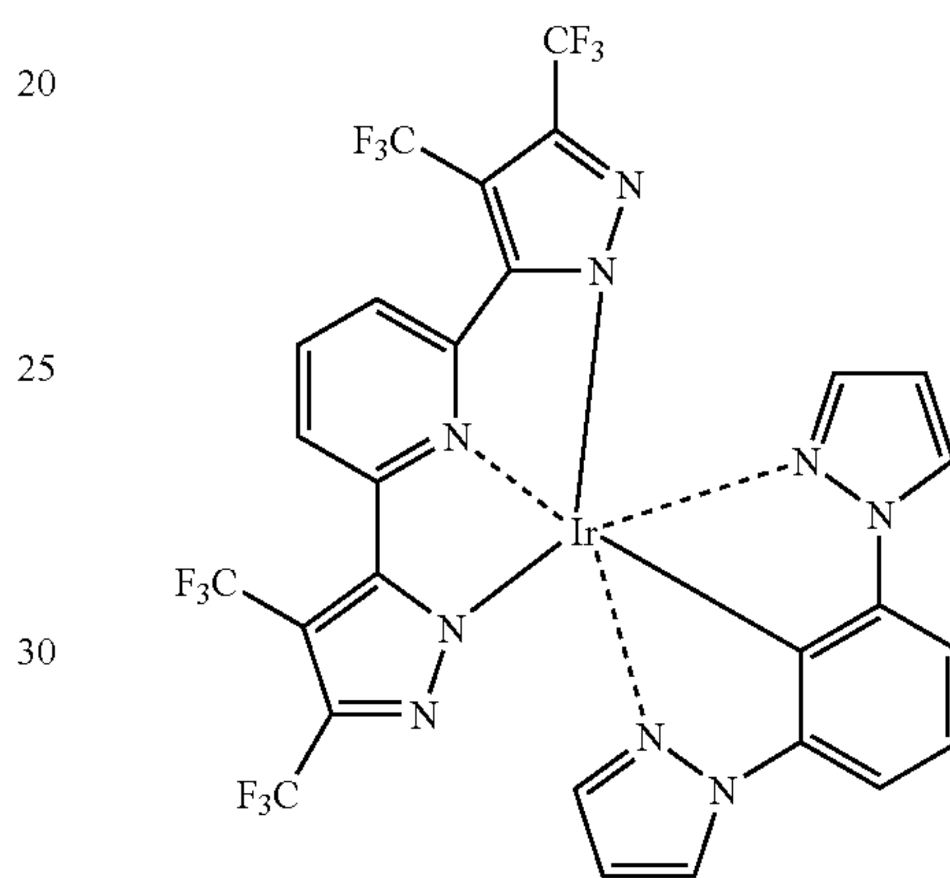
Compound (154)
