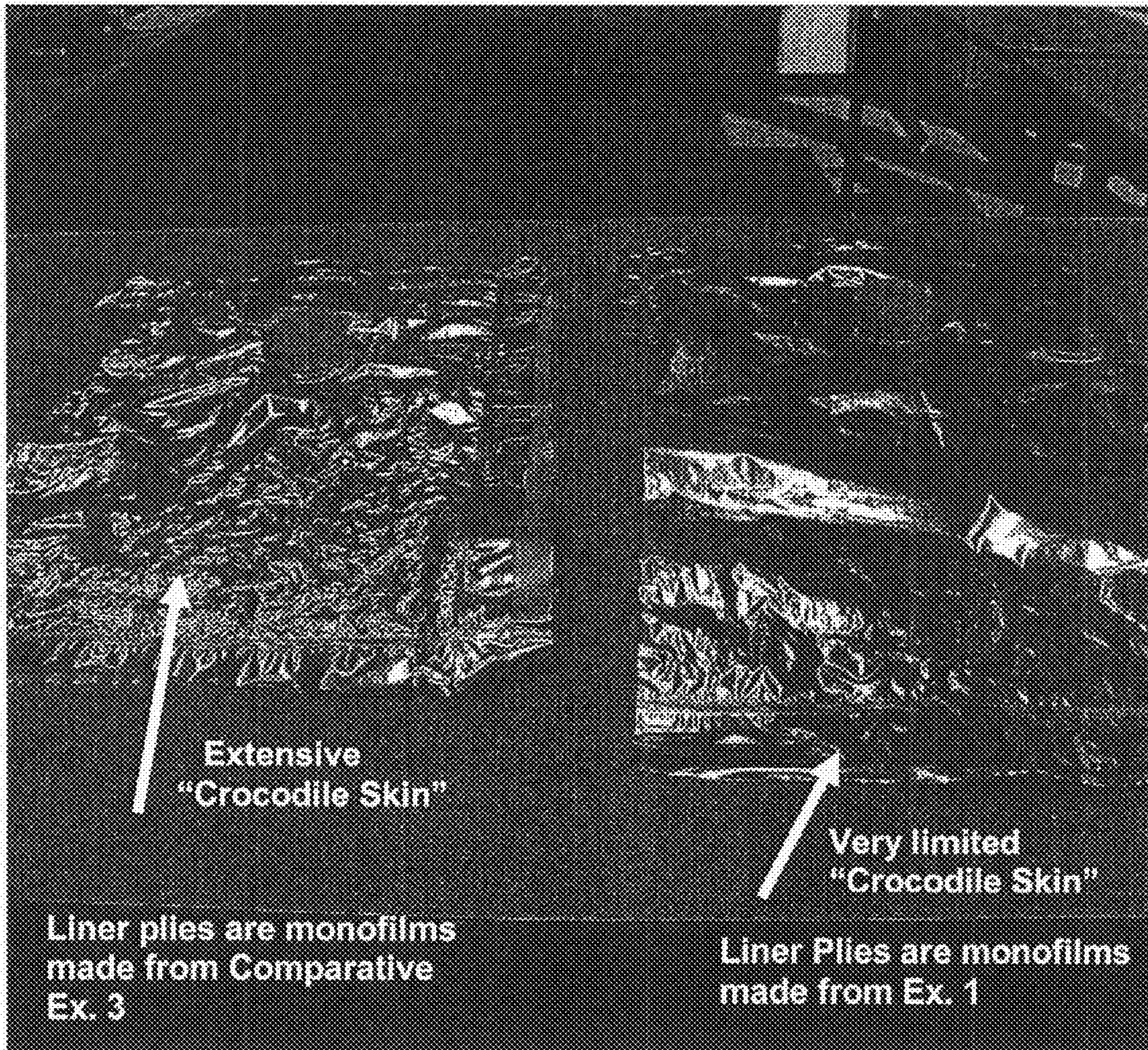
Figure 9a: Comparative Photographs of steamed 3-Ply bags with the same PE/metPET/PE outer ply and with different liner plies (middle and inner plies)
