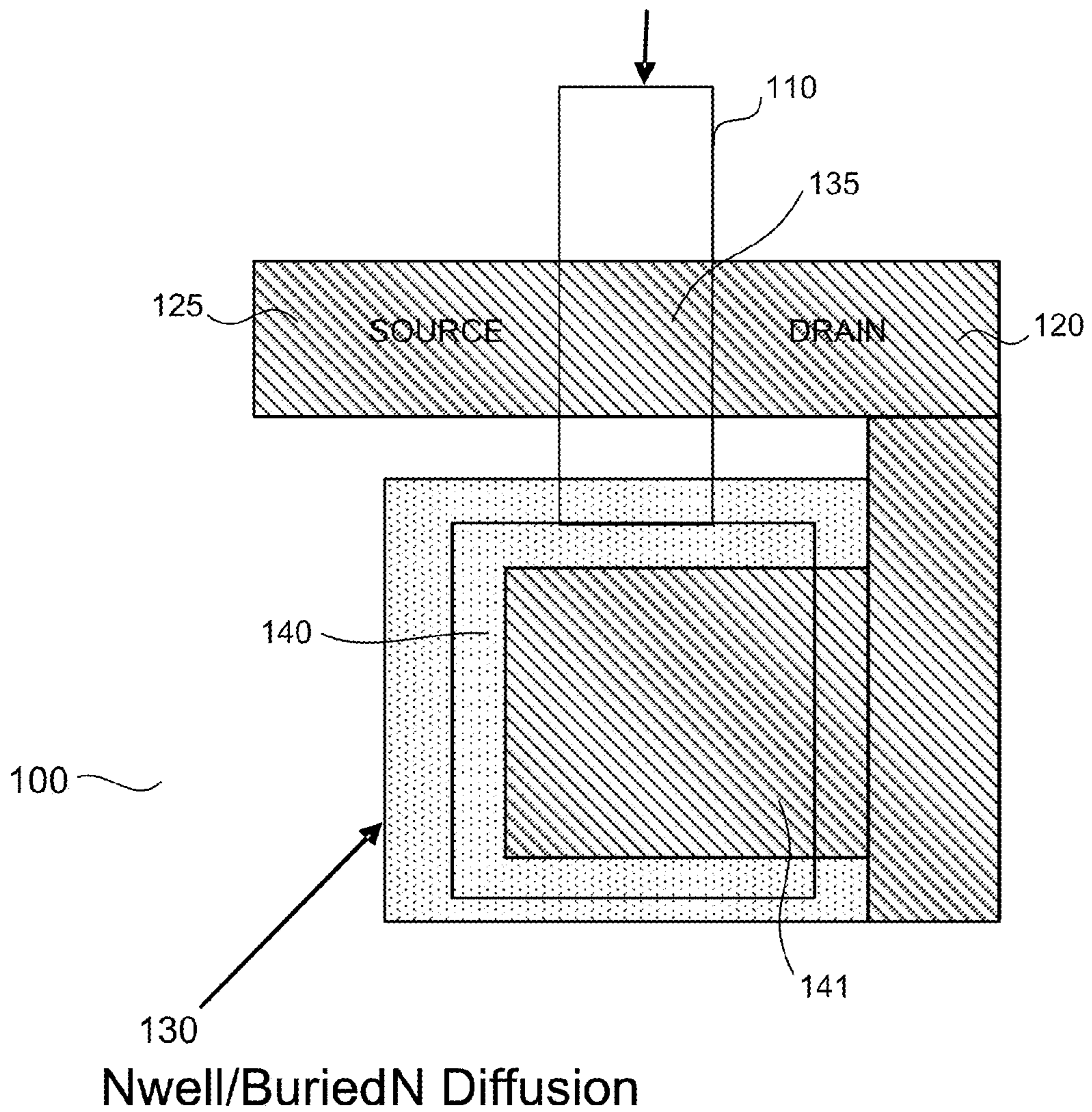
FIG. 1 Floating Gate
