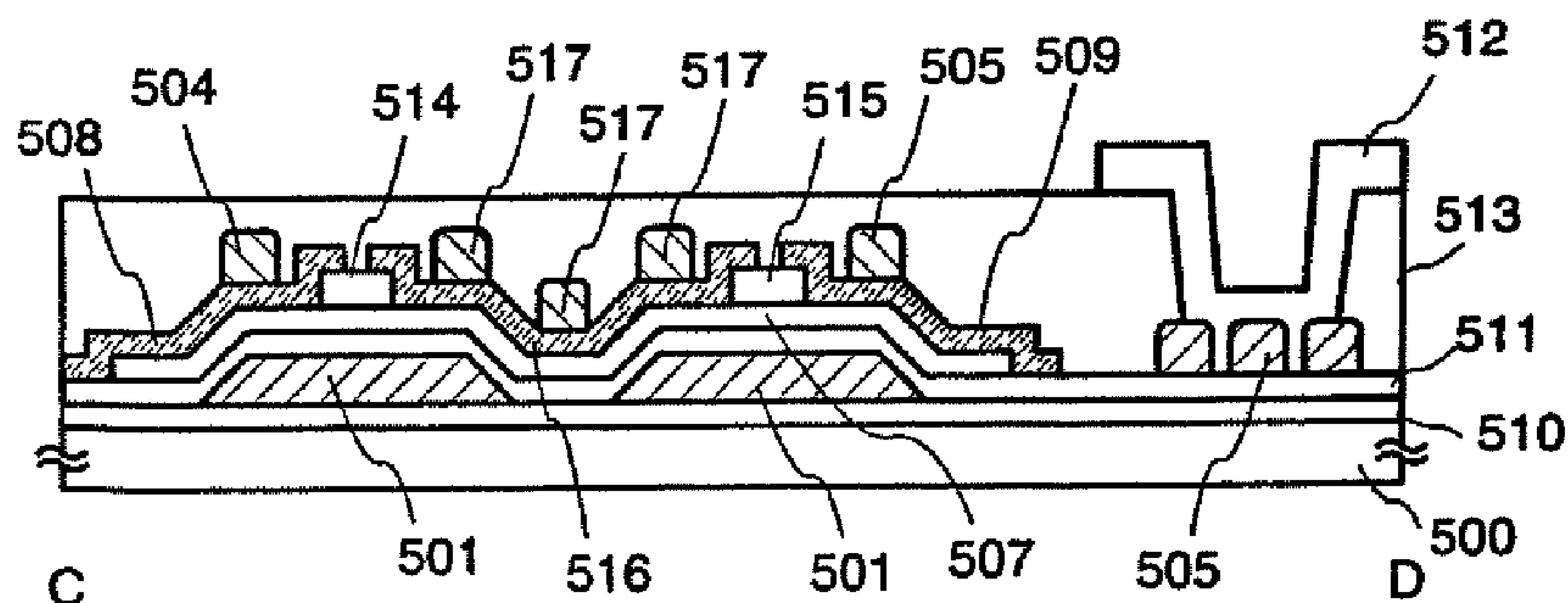
(CROSS SECTION OF C-D)
