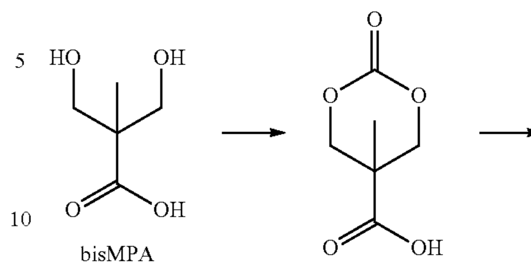
Scheme 1.
