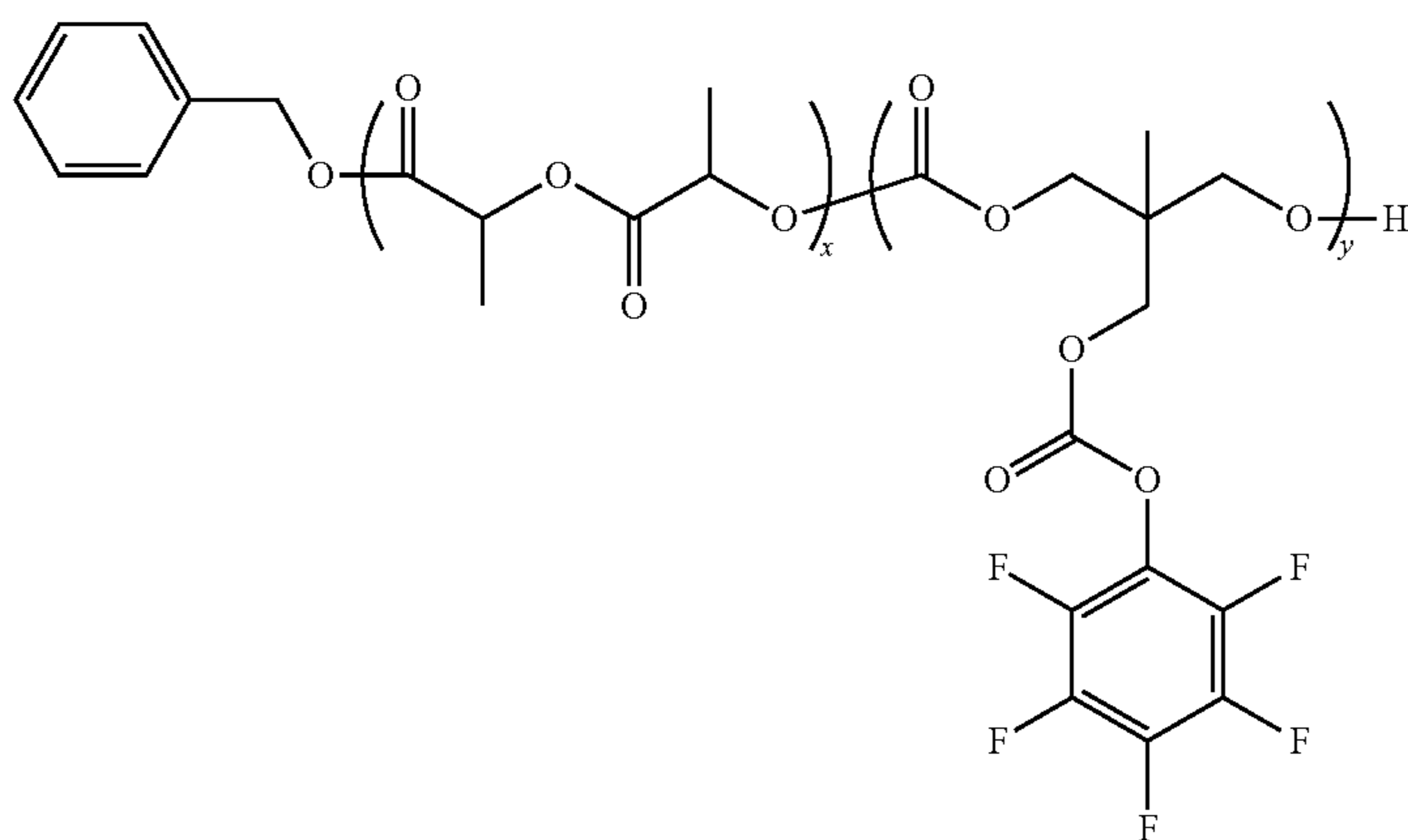
BnOH-[P(LLA-b-TMCPFP)]
