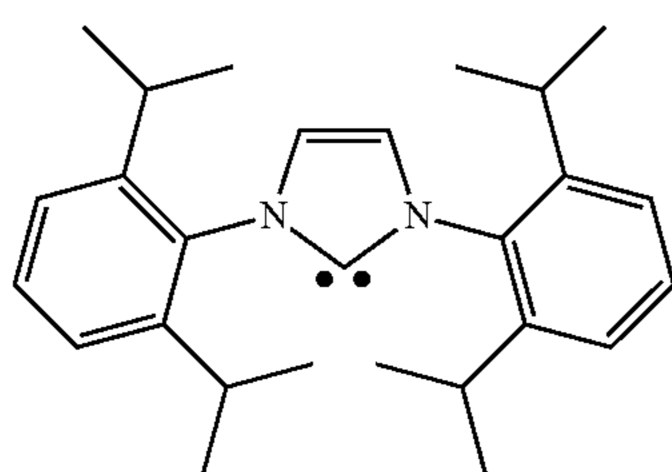
1,3-Bis(2,6-di-i-propylphenyl)imidazol-2-ylidene (Im-3)
