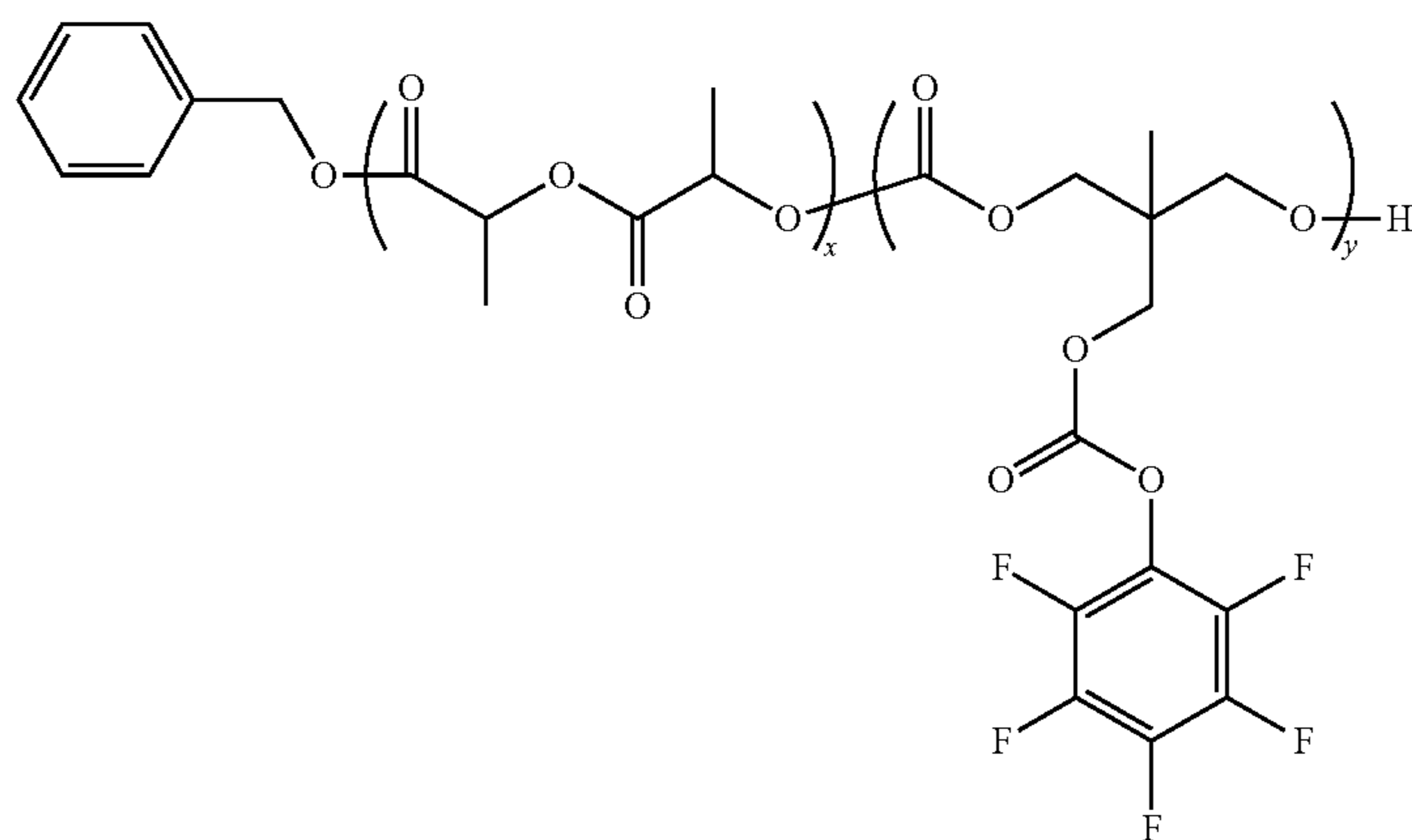
BnOH-[P(LLA-b-TMCPFP)]
