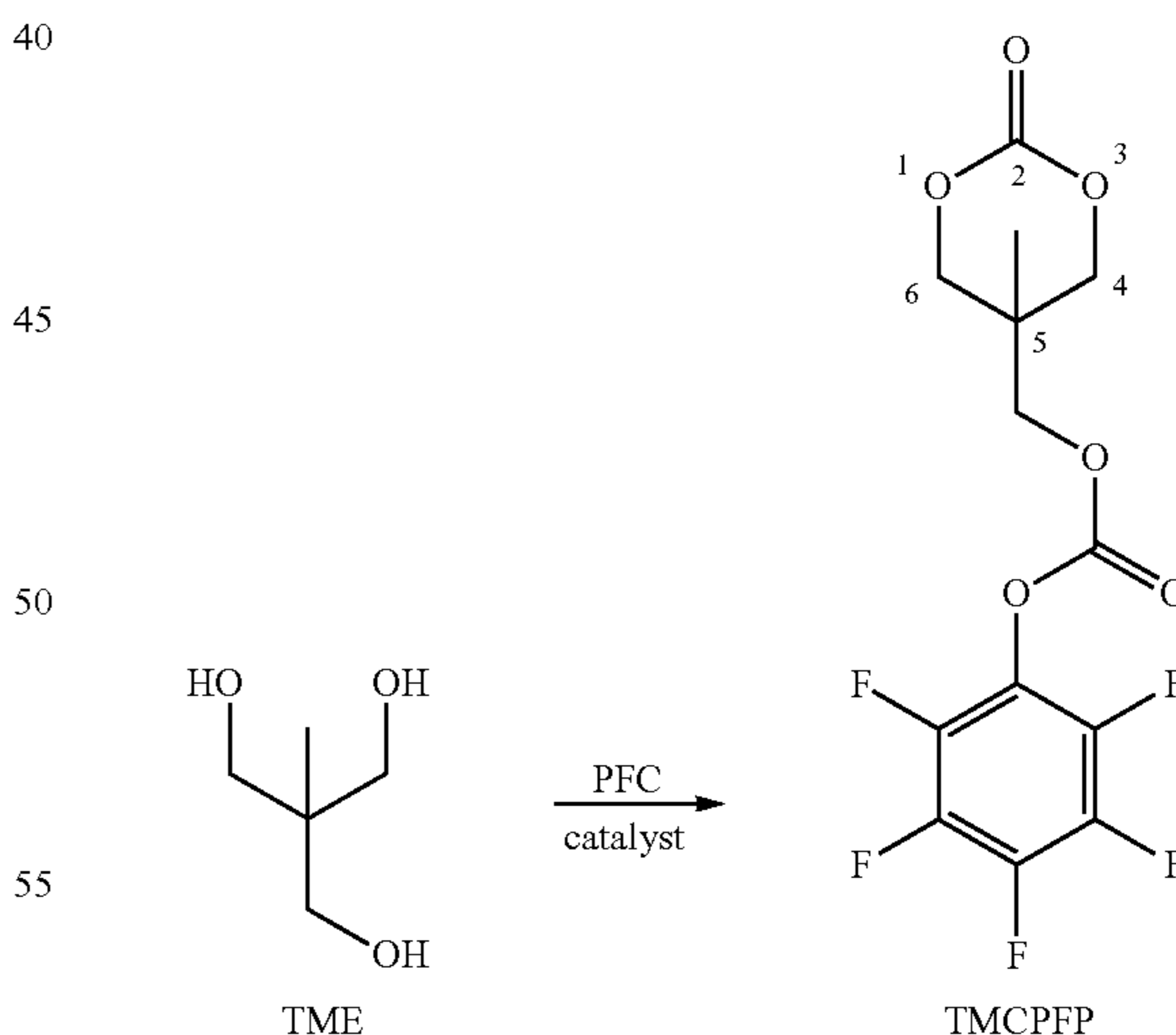
Scheme 5.
