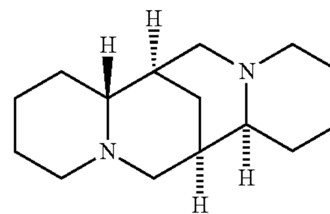
(-)-Sparteine (Sp)
