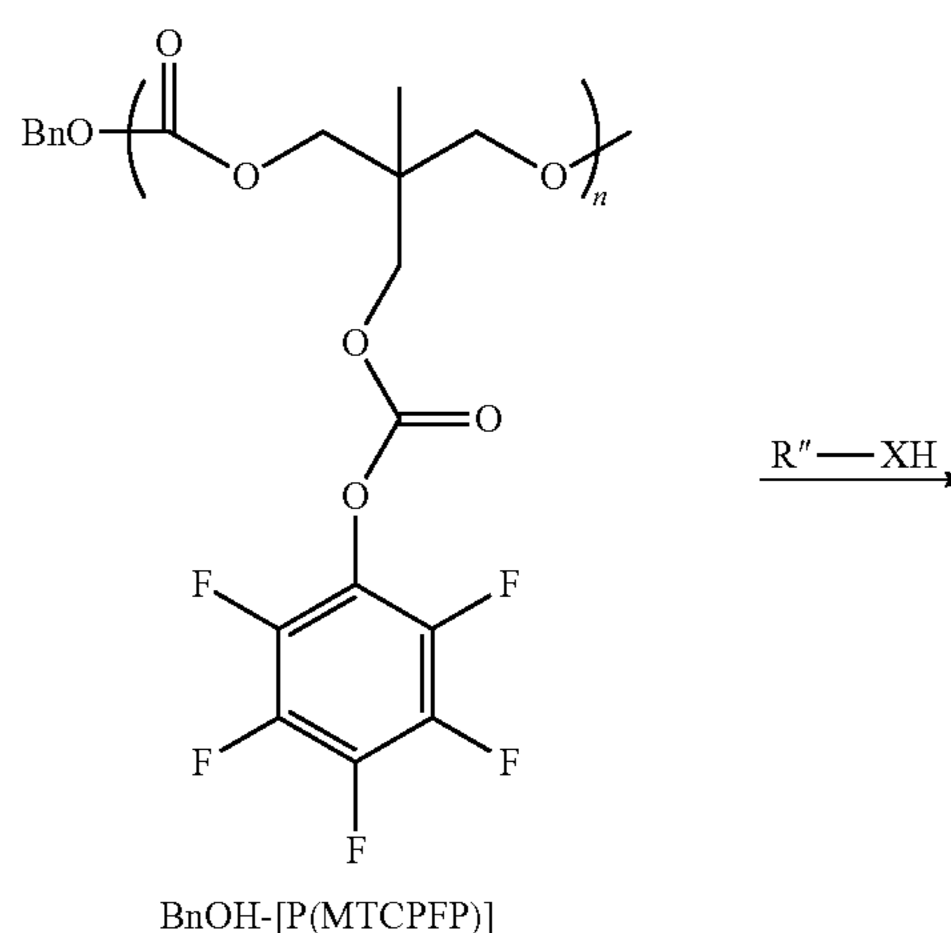
Scheme 8.
