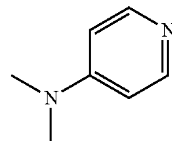
4-N,N-Dimethylaminopyridine (DMAP)
