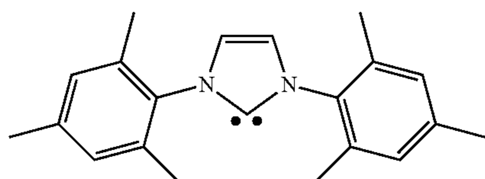
1,3-Bis(2,4,6-trimethylphenyl)imidazol-2-ylidene (Im-2)
