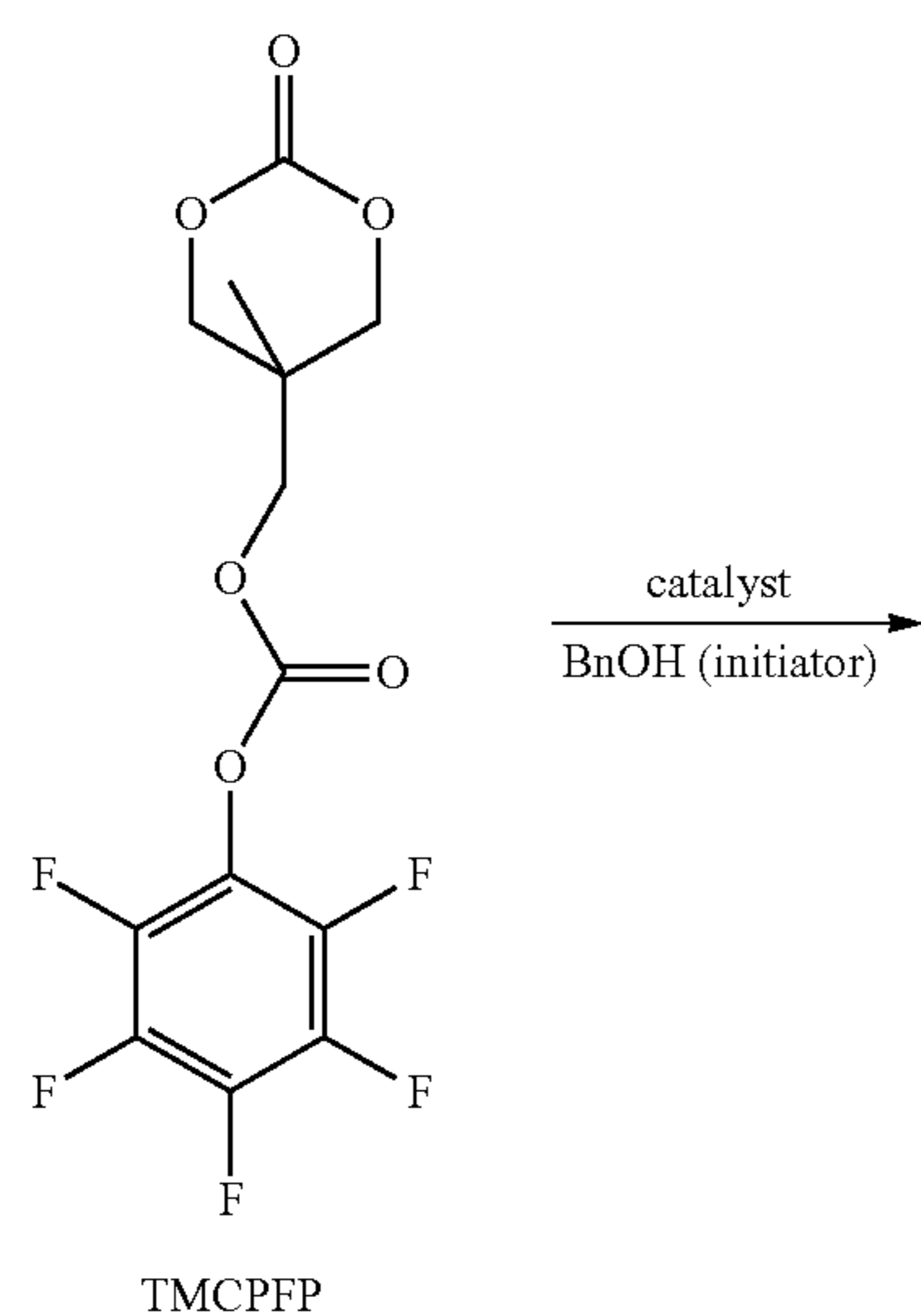
Scheme 7.
