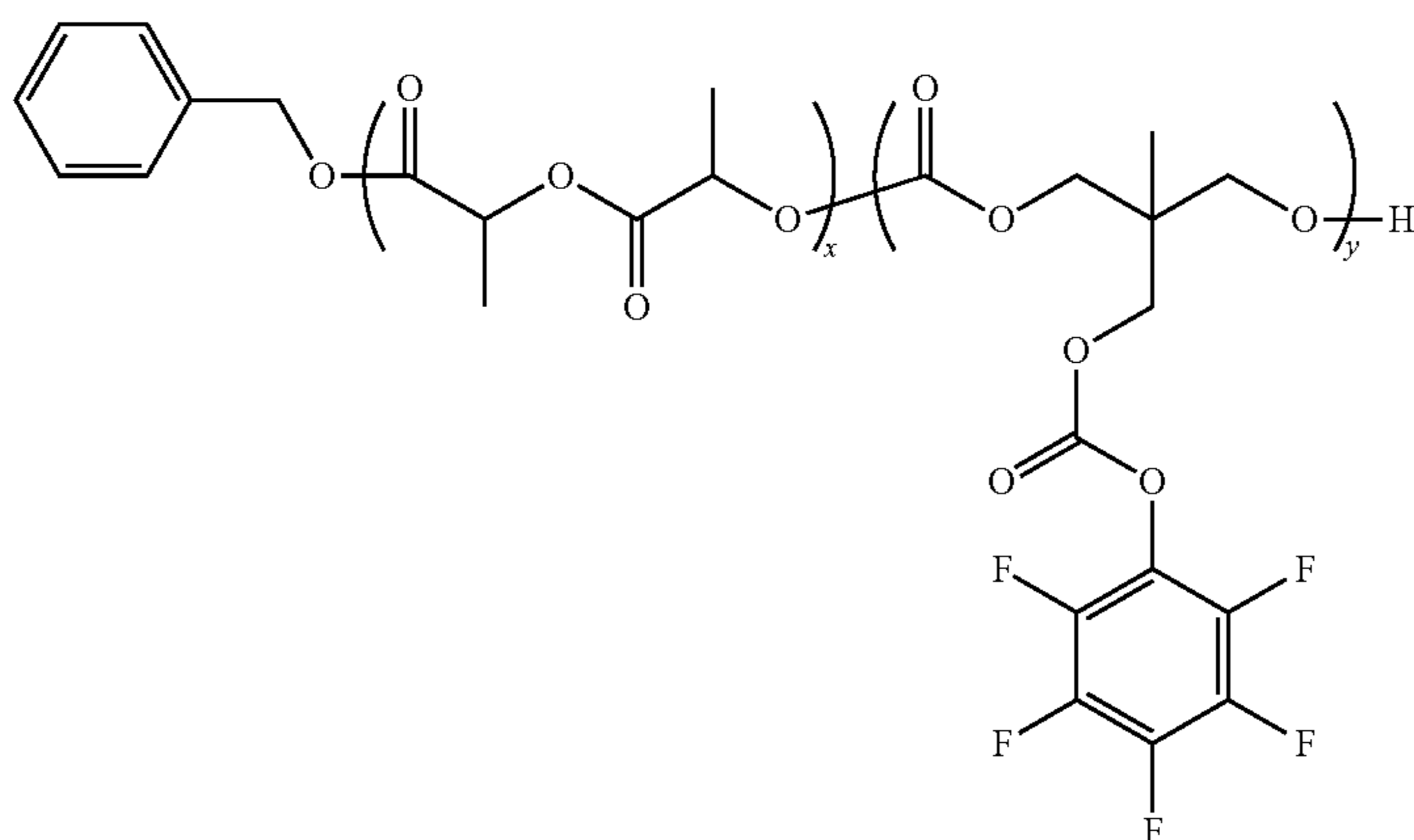
BnOH-[P(LLA-b-TMCPFP)]
