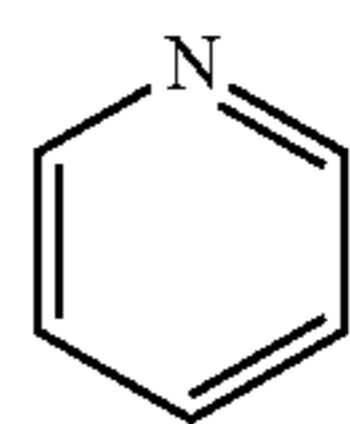
Pyridine (Py)
