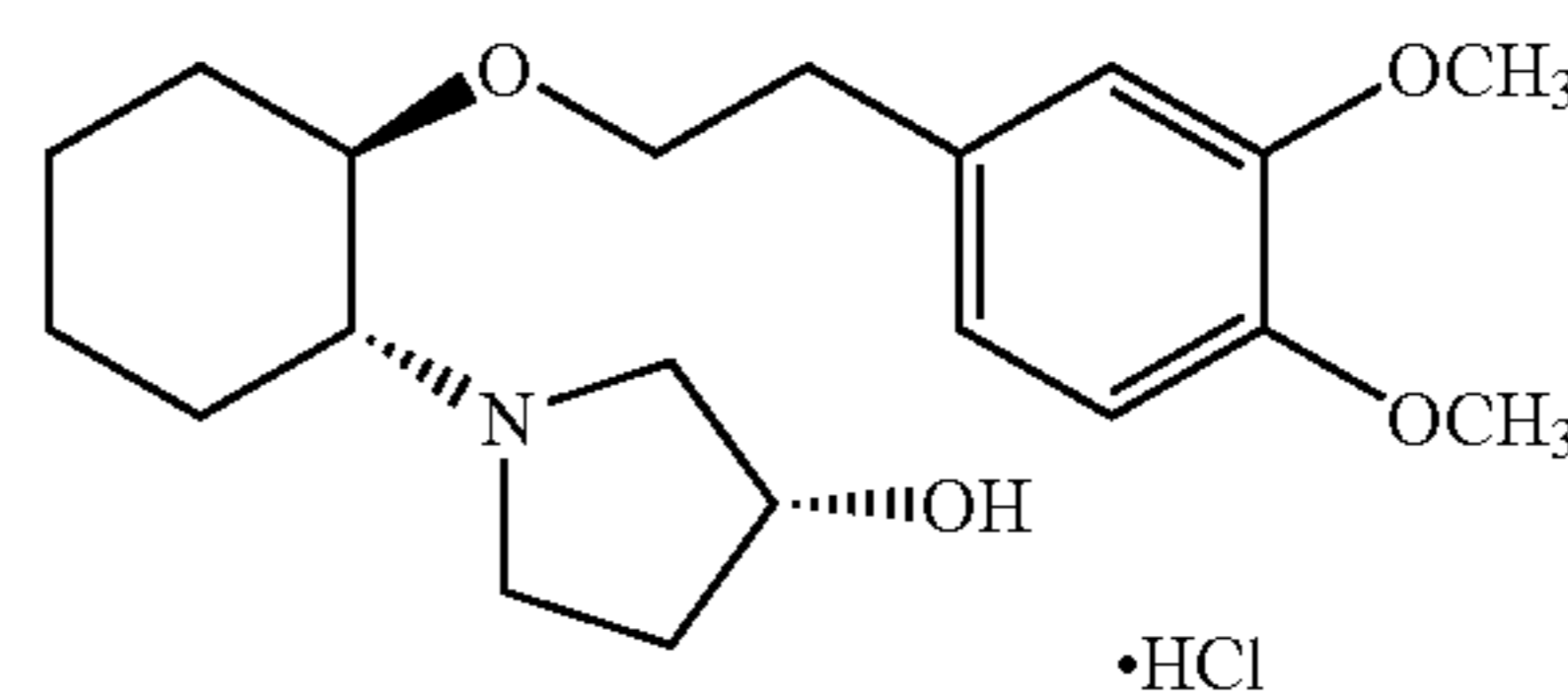
(1R,2R)-2-[(3R)-hydroxypyrrolidinyl]-1-(3,4-dimethoxyphenoxy)cyclohexane monohydrochloride
