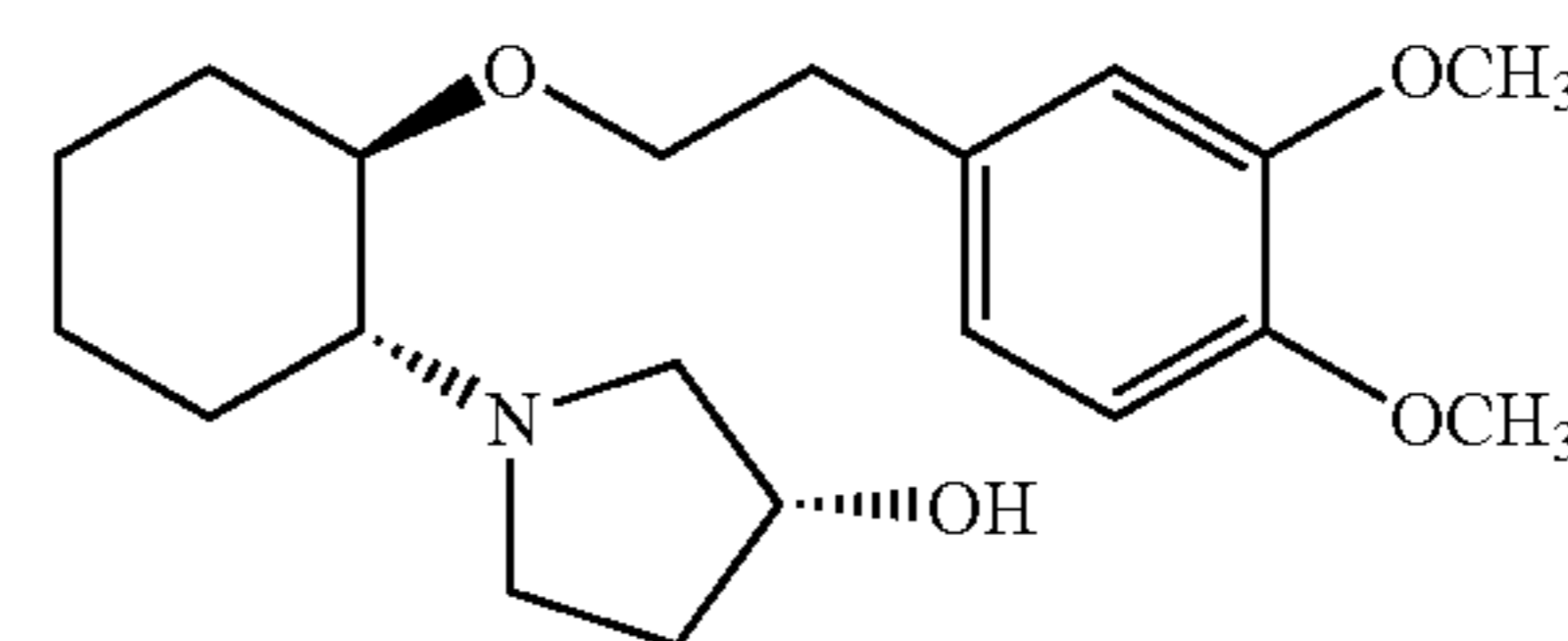
(1R,2R)-2-[(3R)-hydroxypyrrolidinyl]-1-(3,4-dimethoxyphenoxy)cyclohexane
