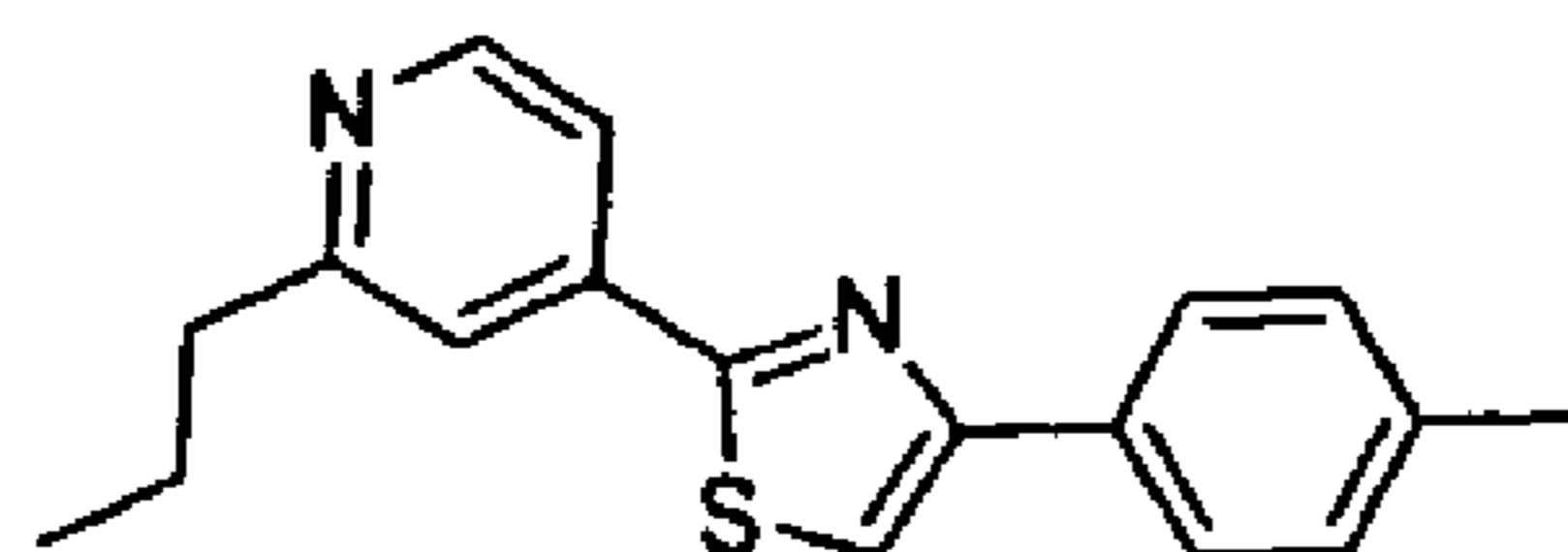
Fatostatin A
