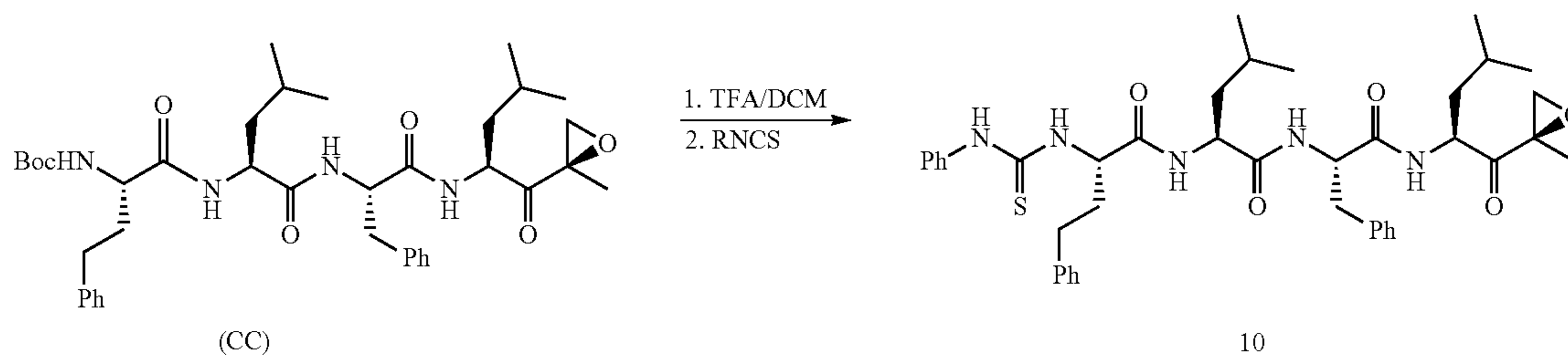
Scheme 9: Synthesis of Example 9
