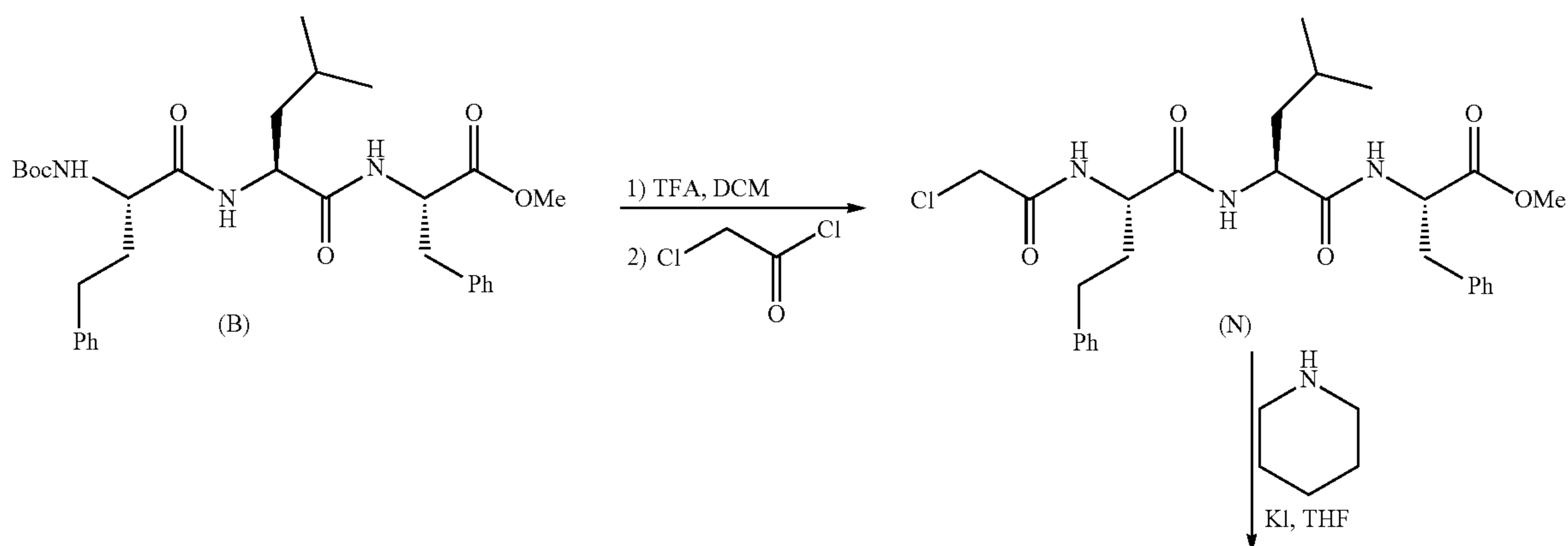
Scheme 4: Synthesis of Example 4
