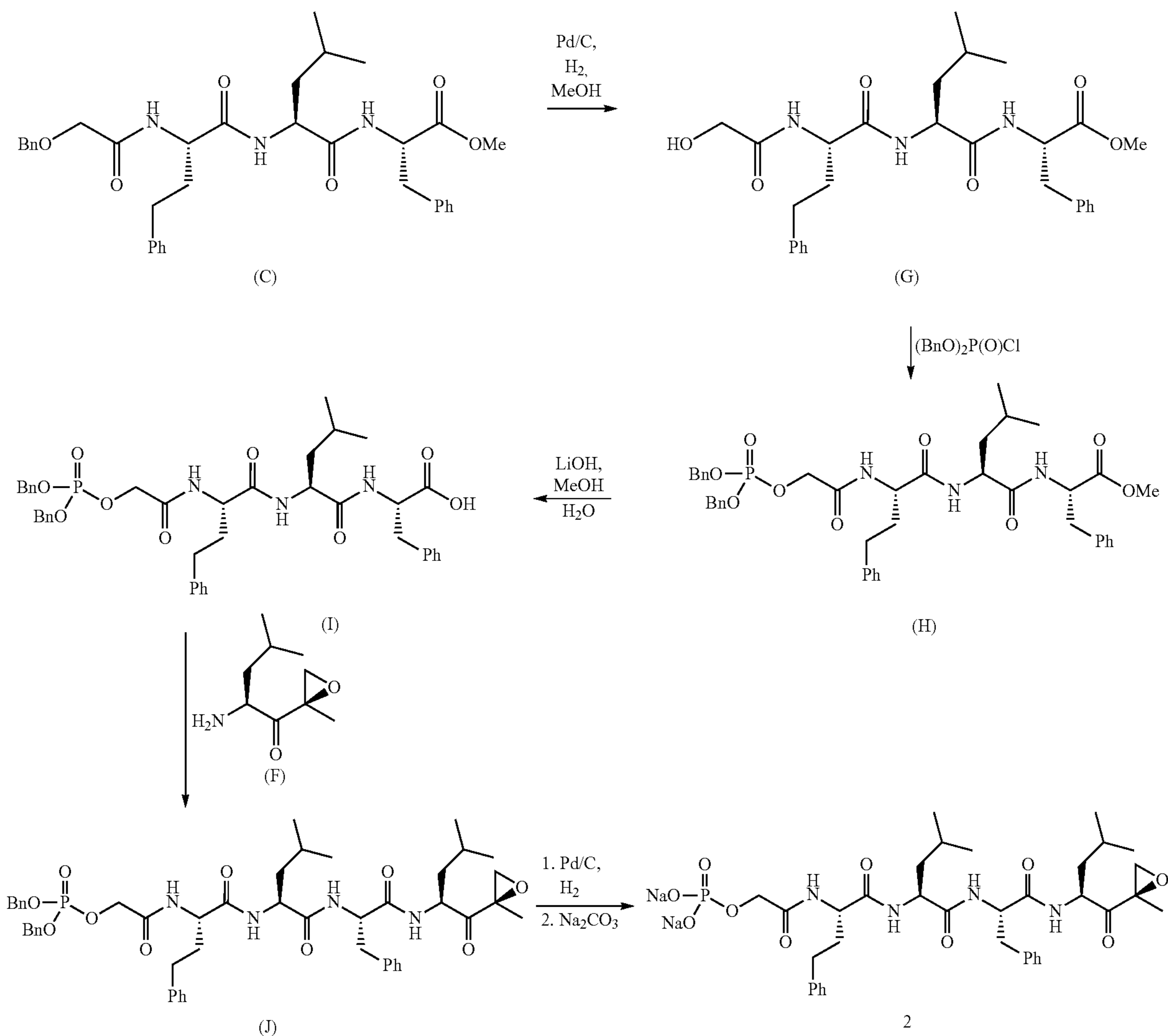
Scheme 2: Synthesis of Example 2
