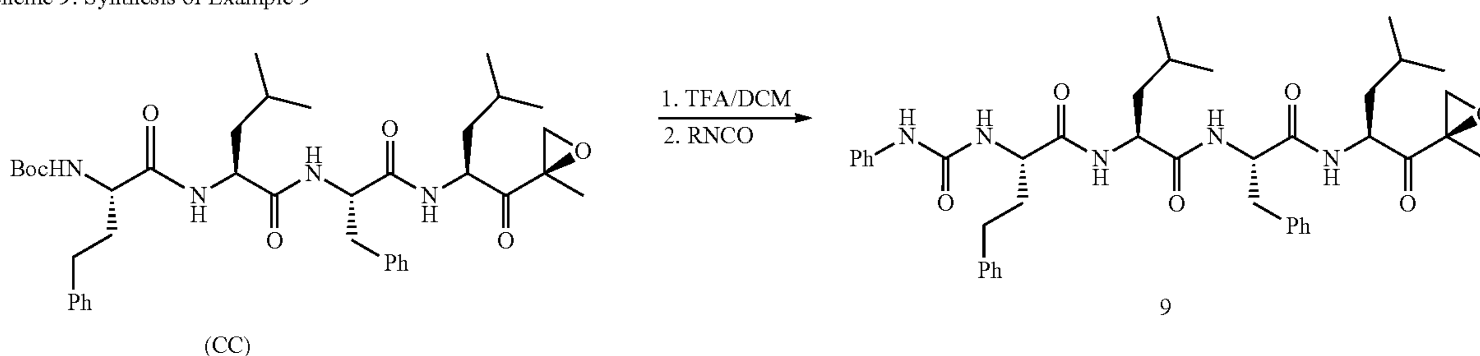
Scheme 9: Synthesis of Example 9
