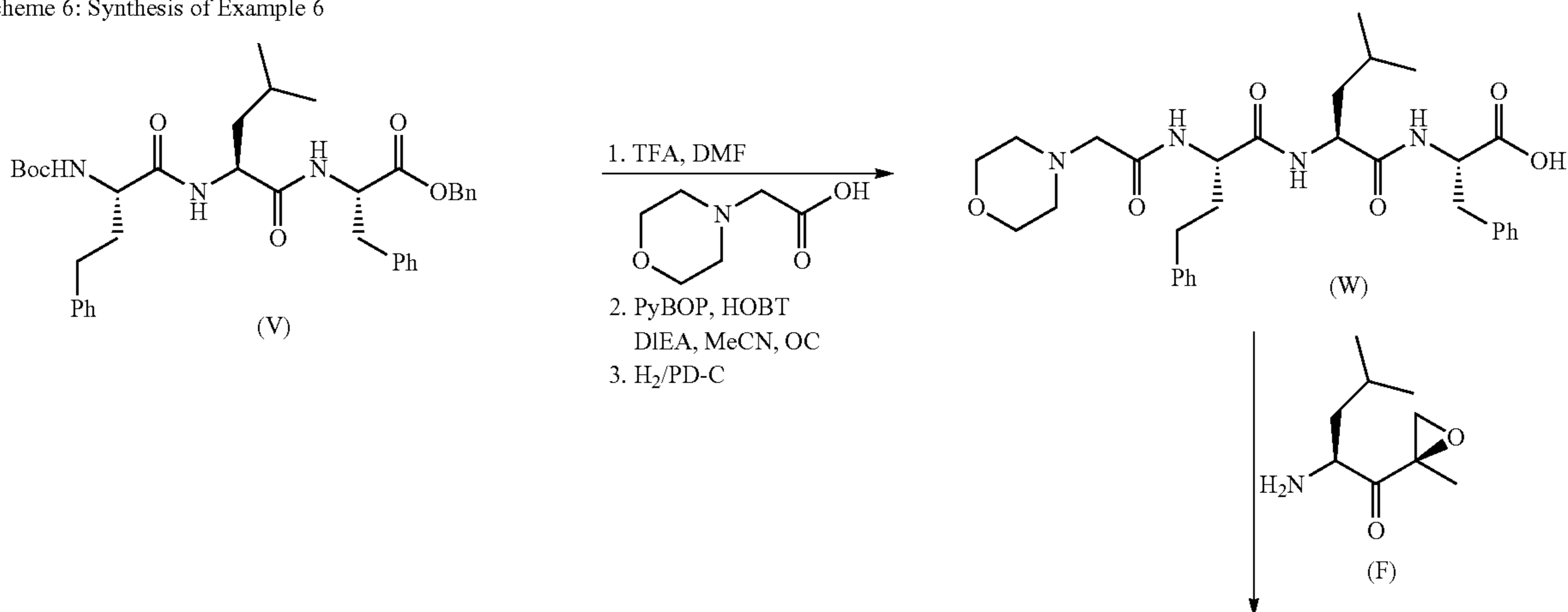
Scheme 6: Synthesis of Example 6
