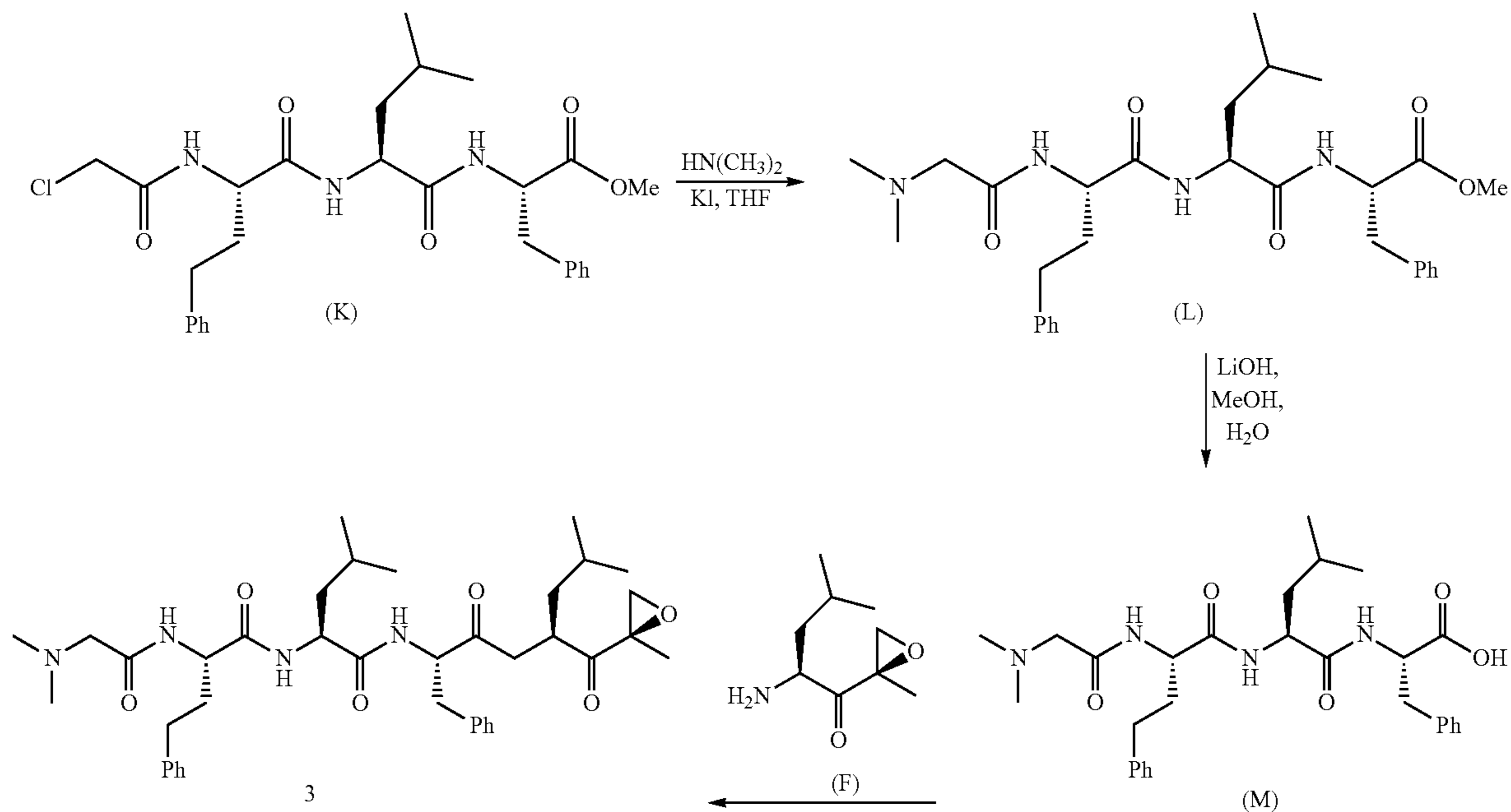
Scheme 3: Synthesis of Example 3
