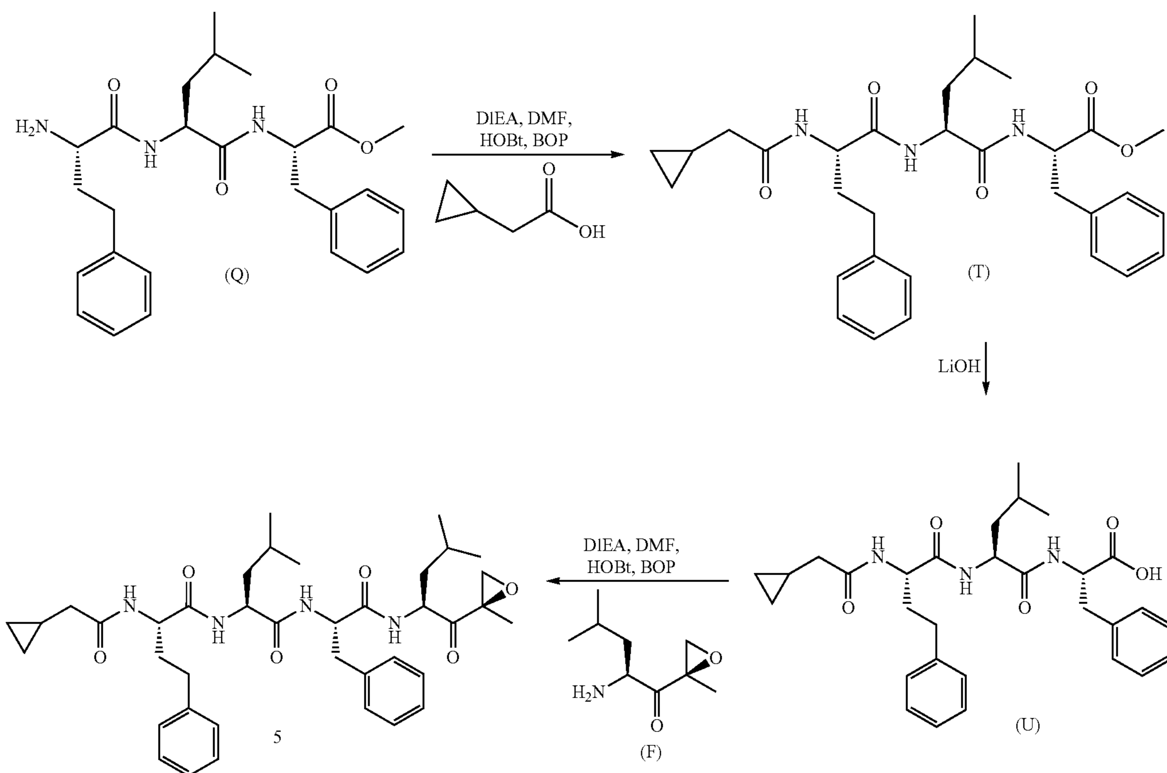
Scheme 5: Synthesis of Example 5
