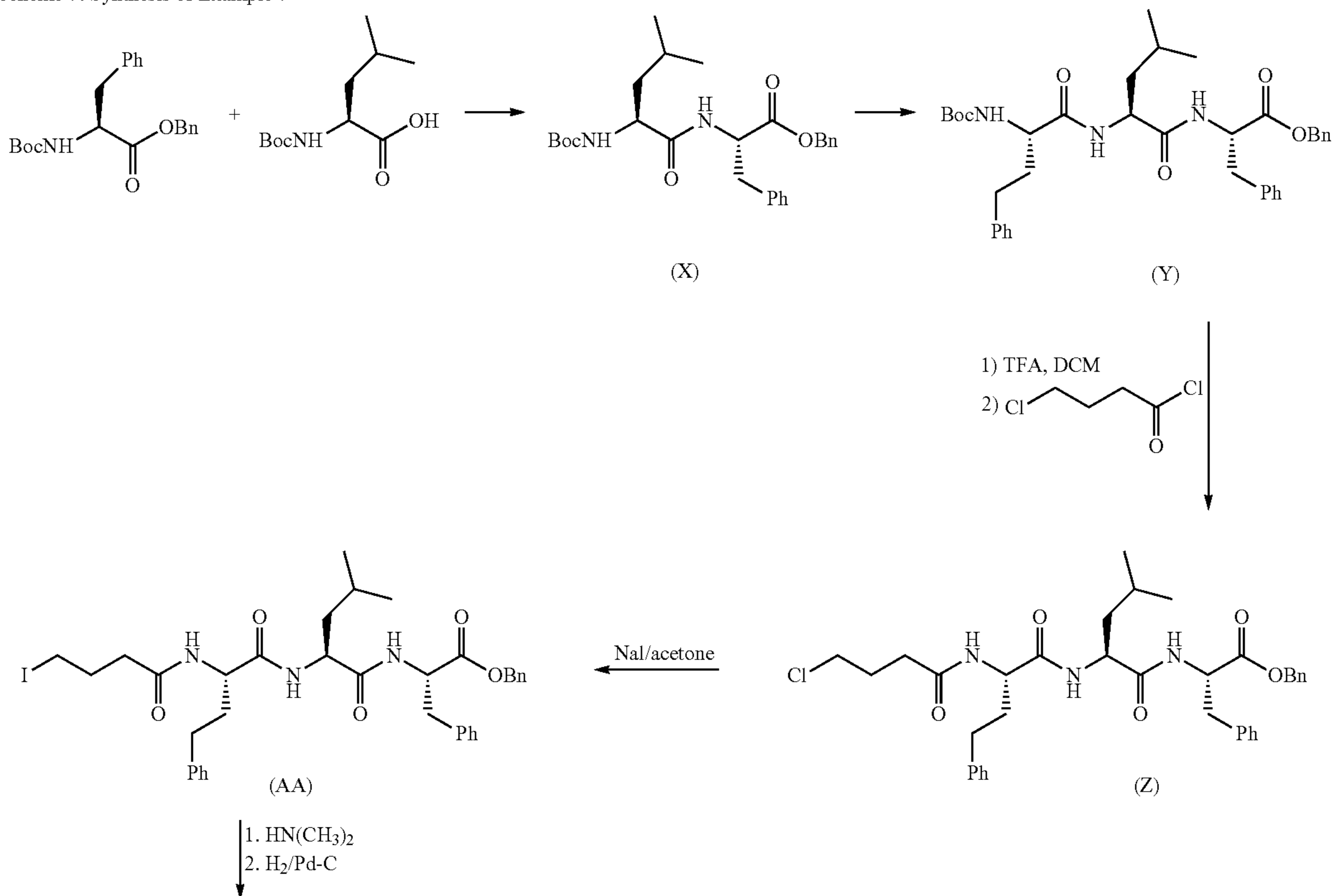
Scheme 7: Synthesis of Example 7
