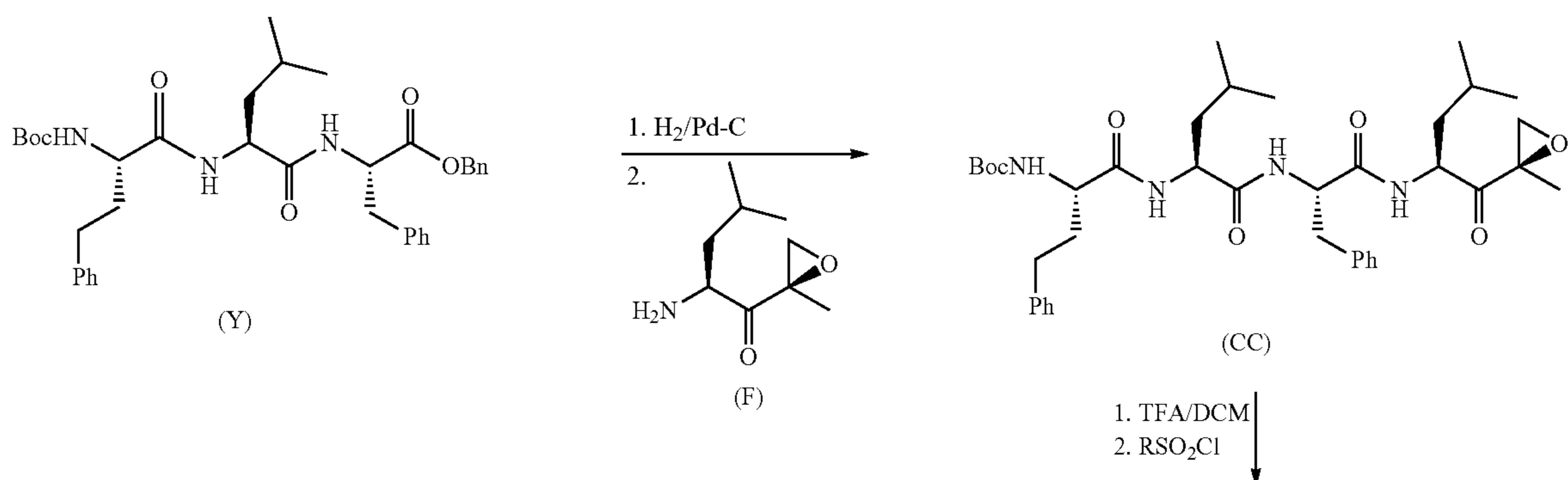
Scheme 8: Synthesis of Example 8
