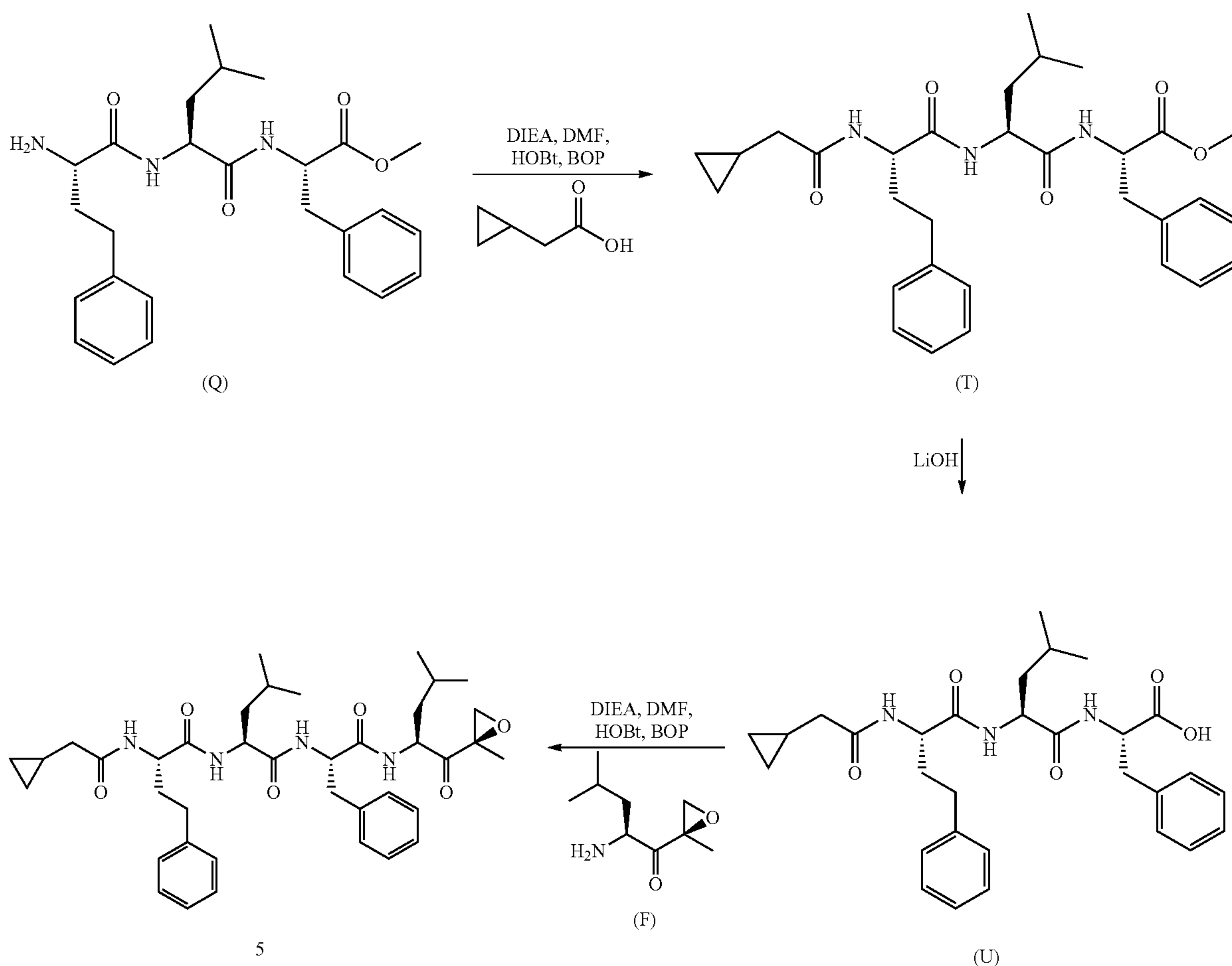
Scheme 5: Synthesis of Example 5
