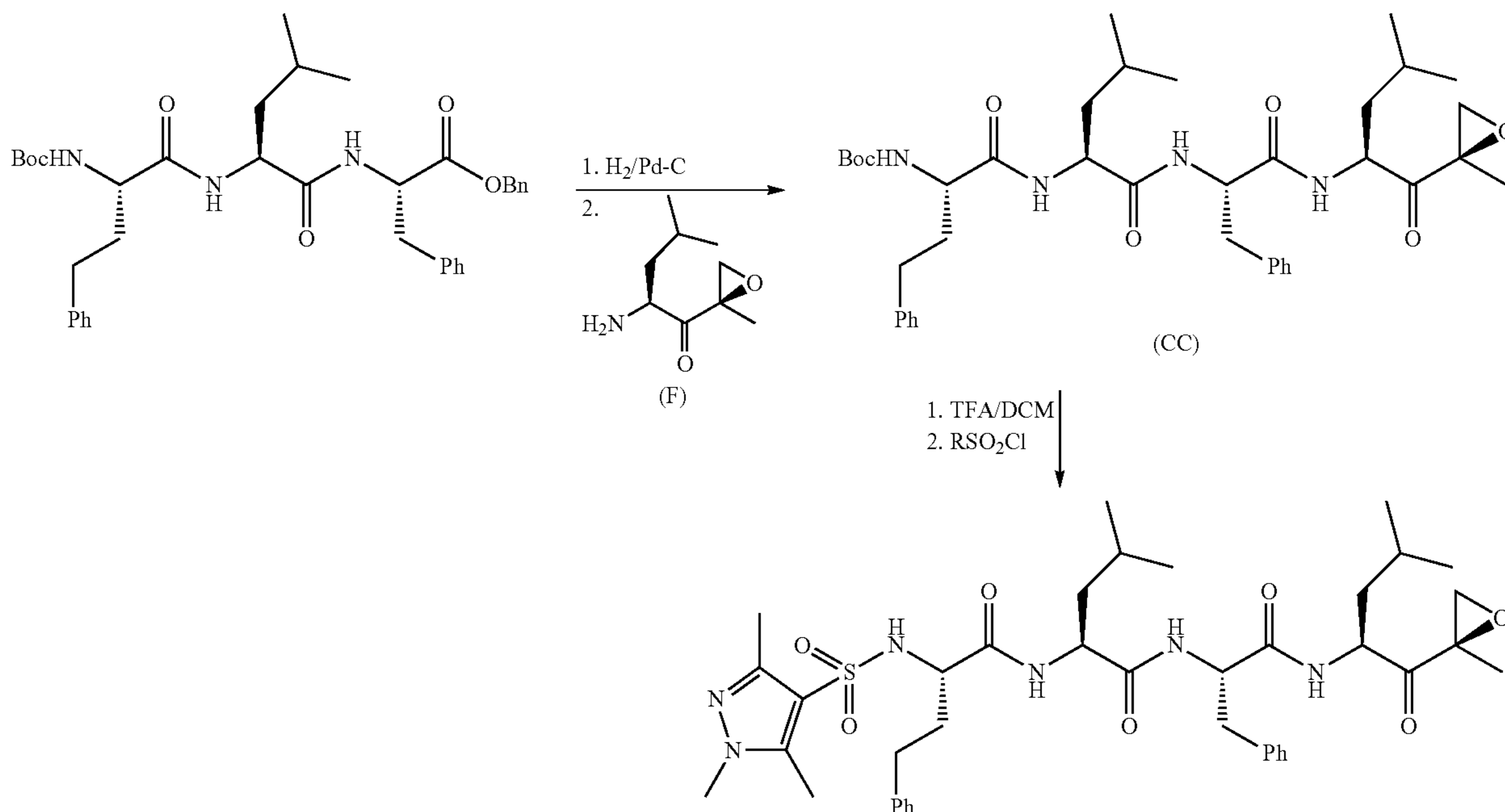
Scheme 8: Synthesis of Example 8
