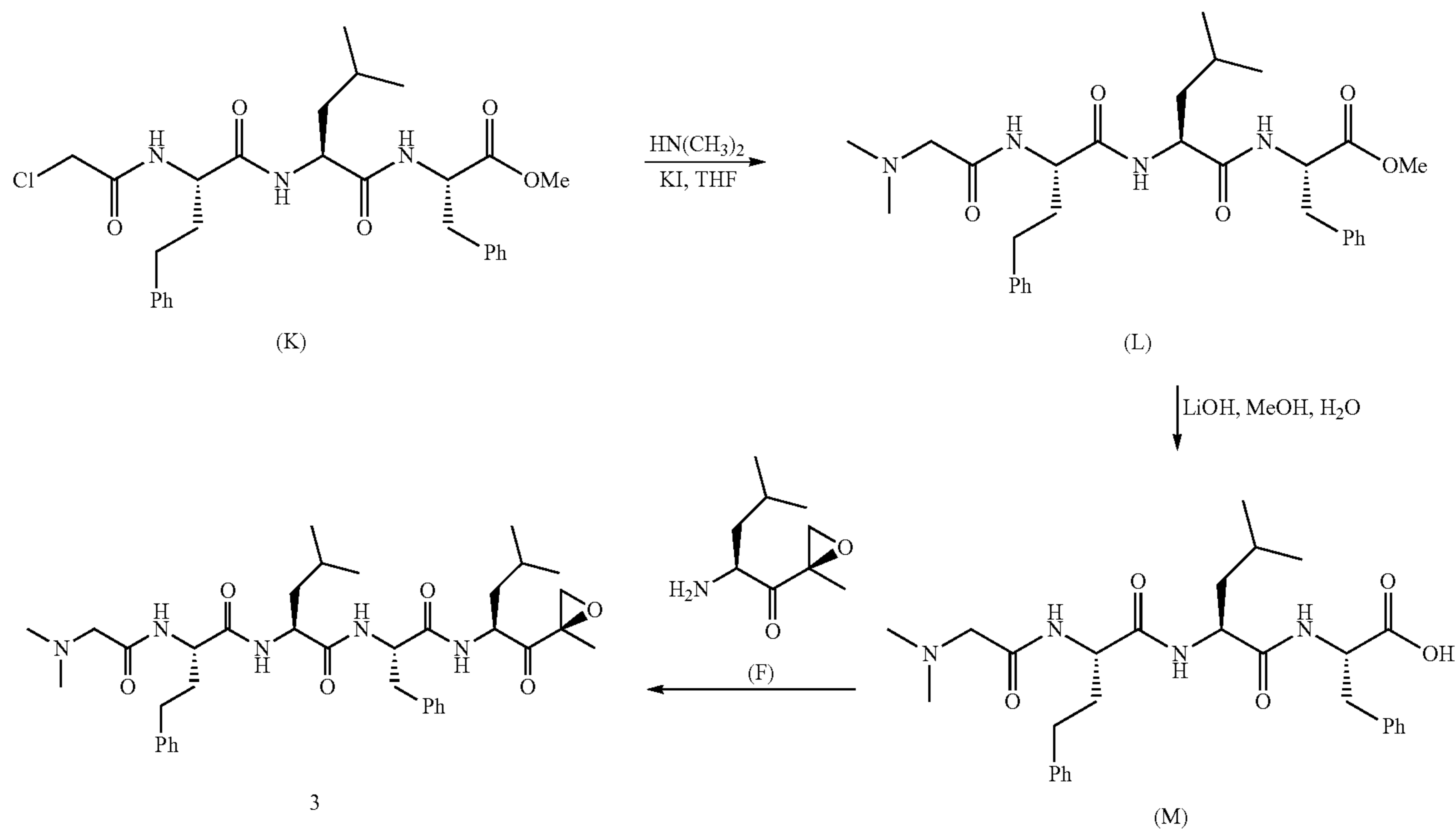
Scheme 3: Synthesis of Example 3
