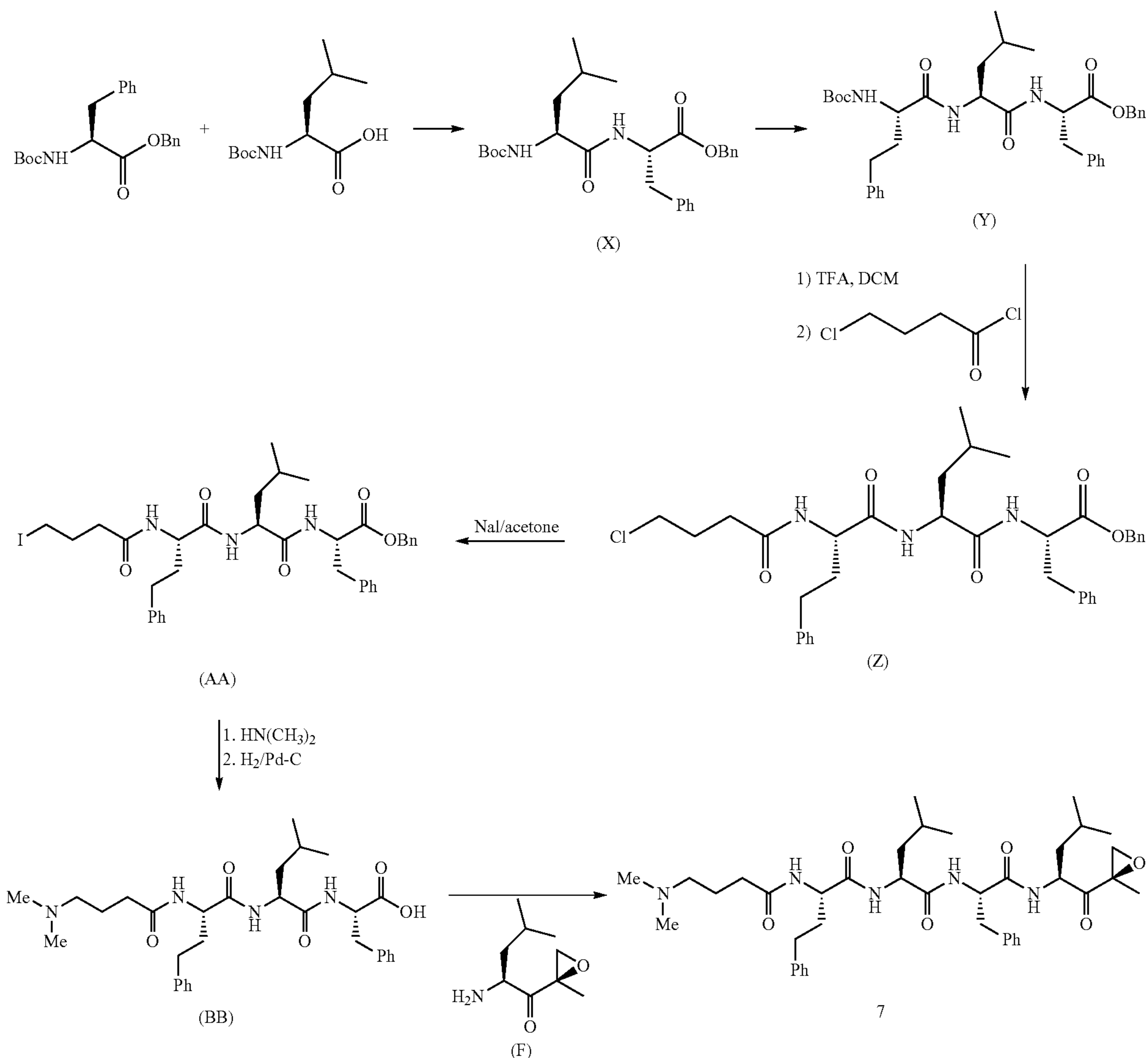
Scheme 7: Synthesis of Example 7
