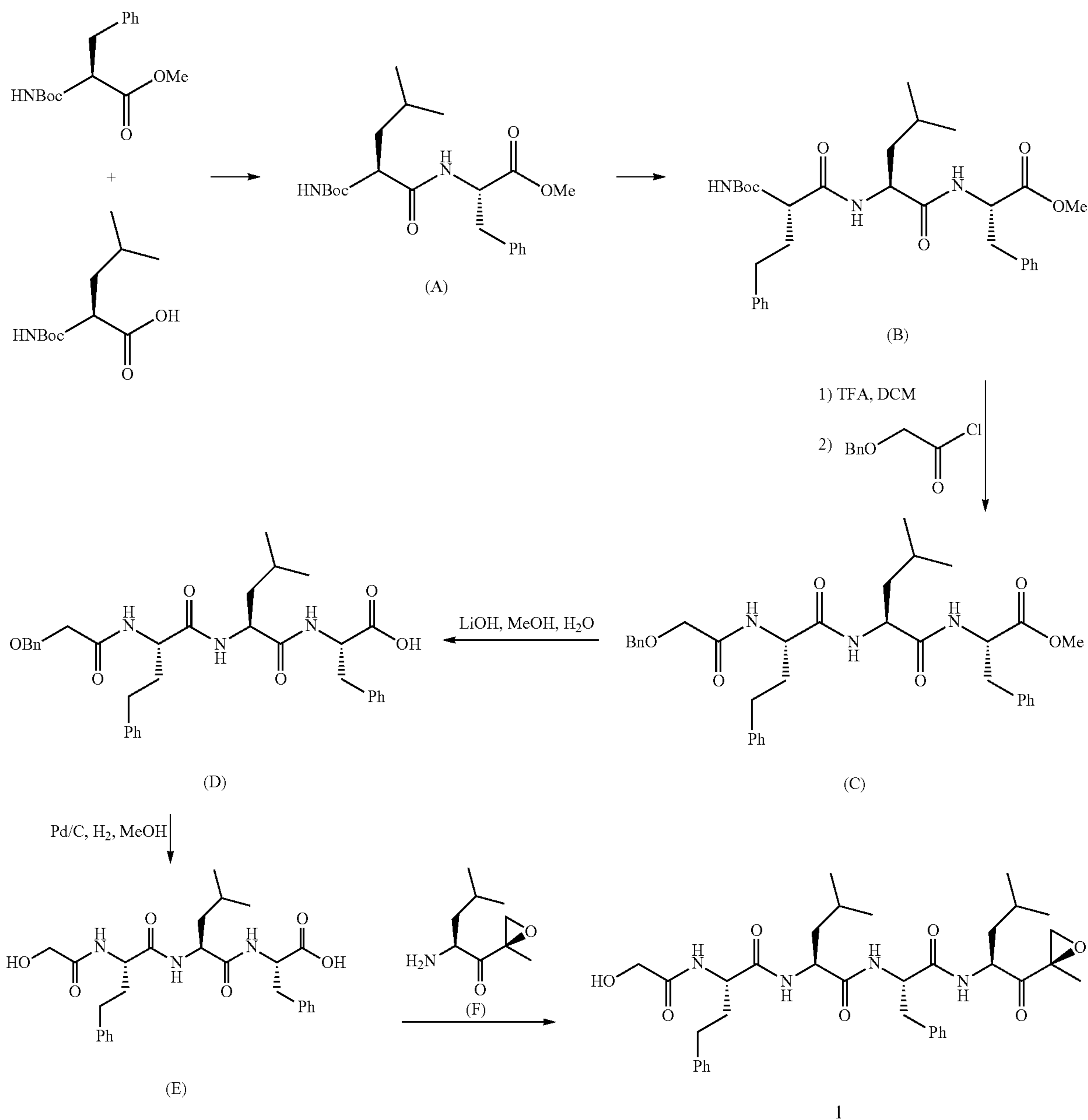
Scheme 1: Synthesis of Example 1
