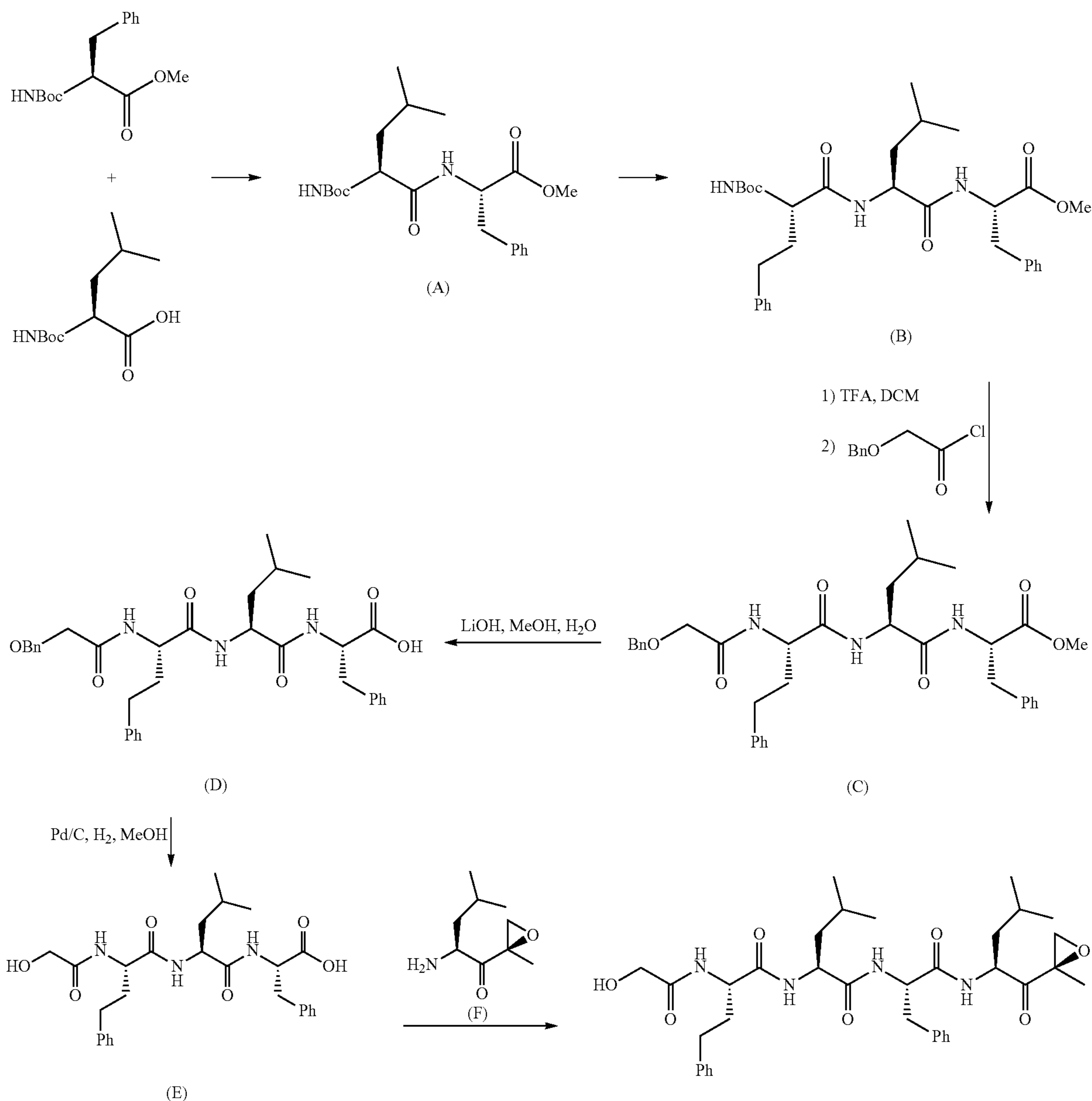
Scheme 1: Synthesis of Example 1
