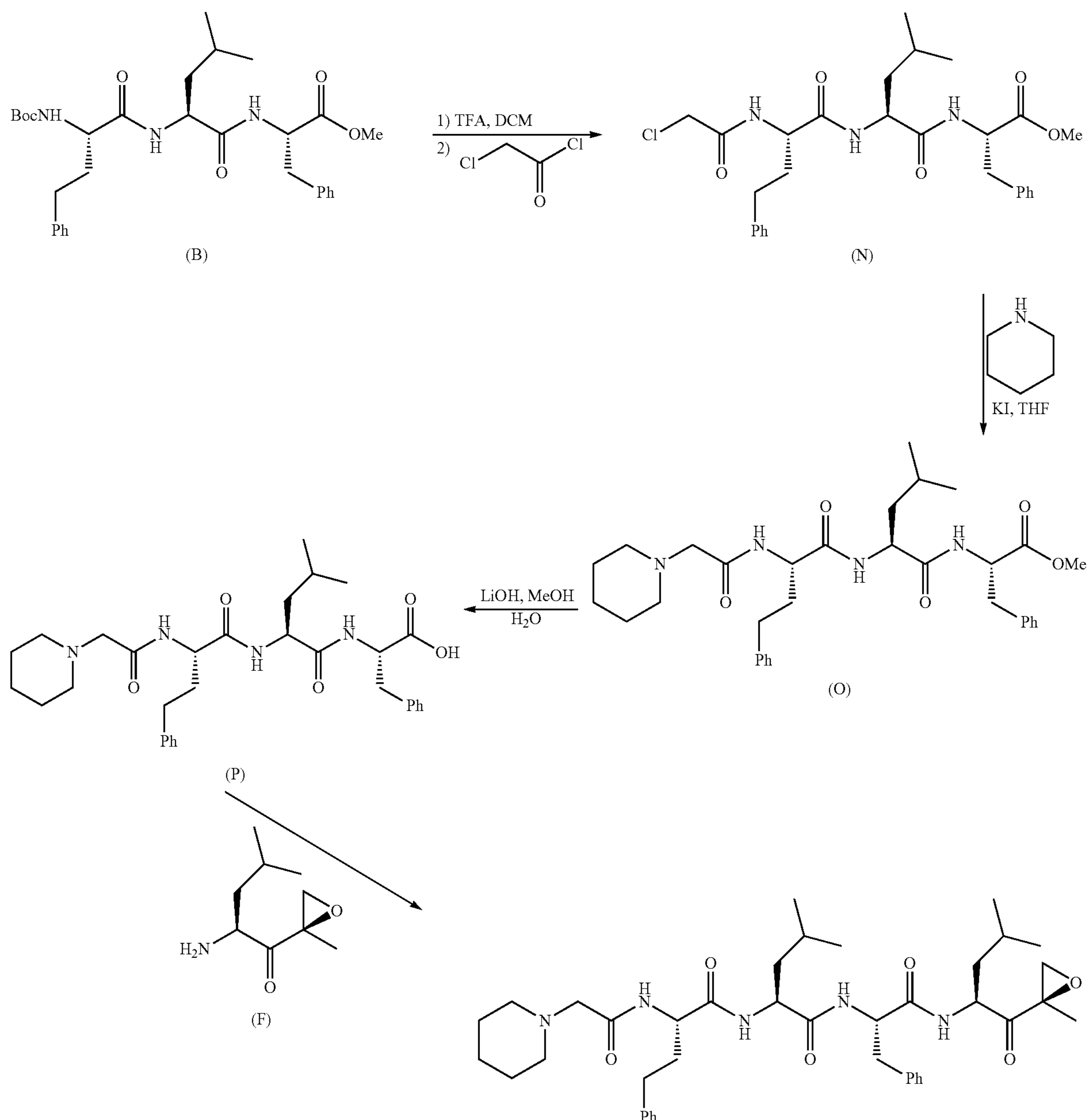
Scheme 4: Synthesis of Example 4
