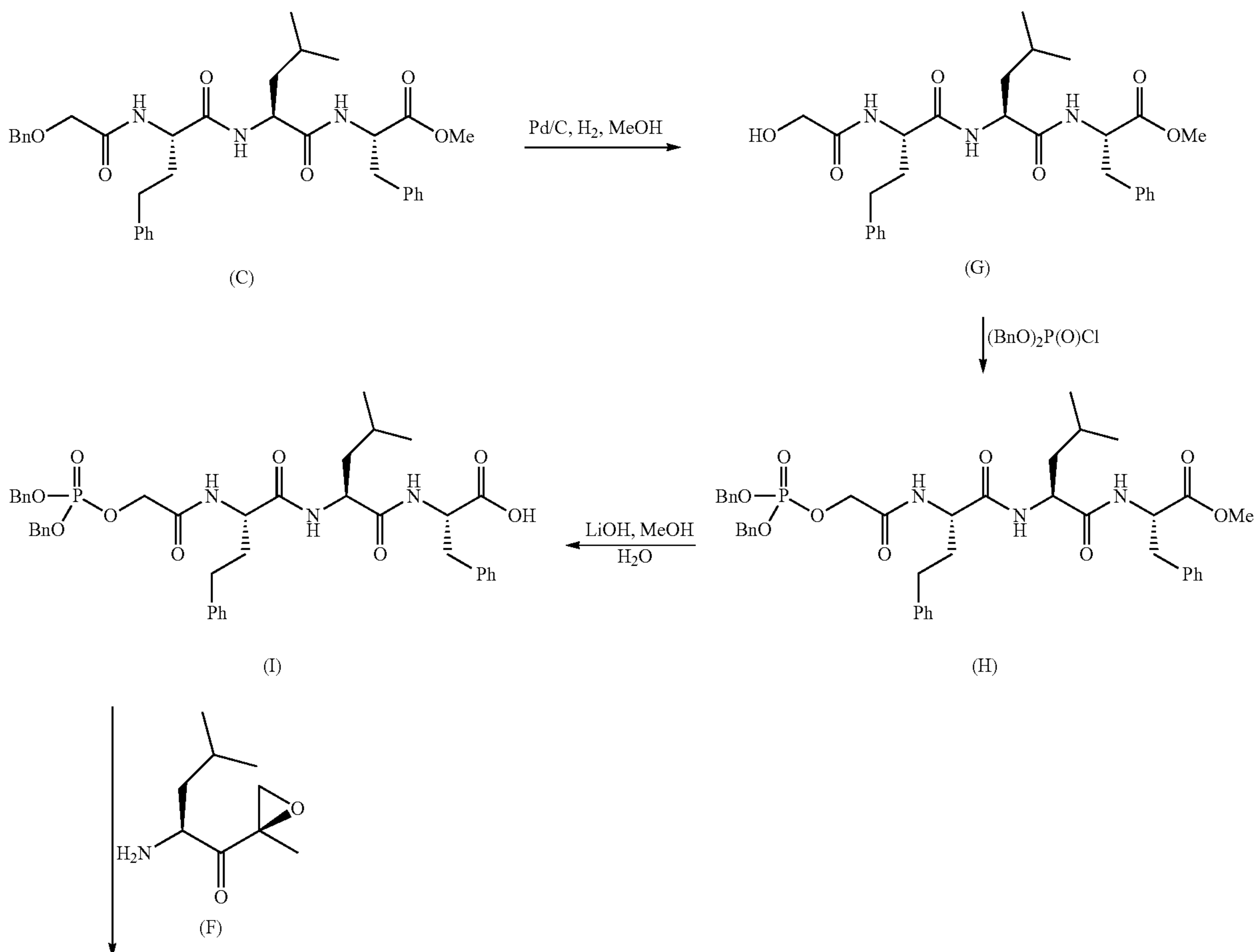
Scheme 2: Synthesis of Example 2
