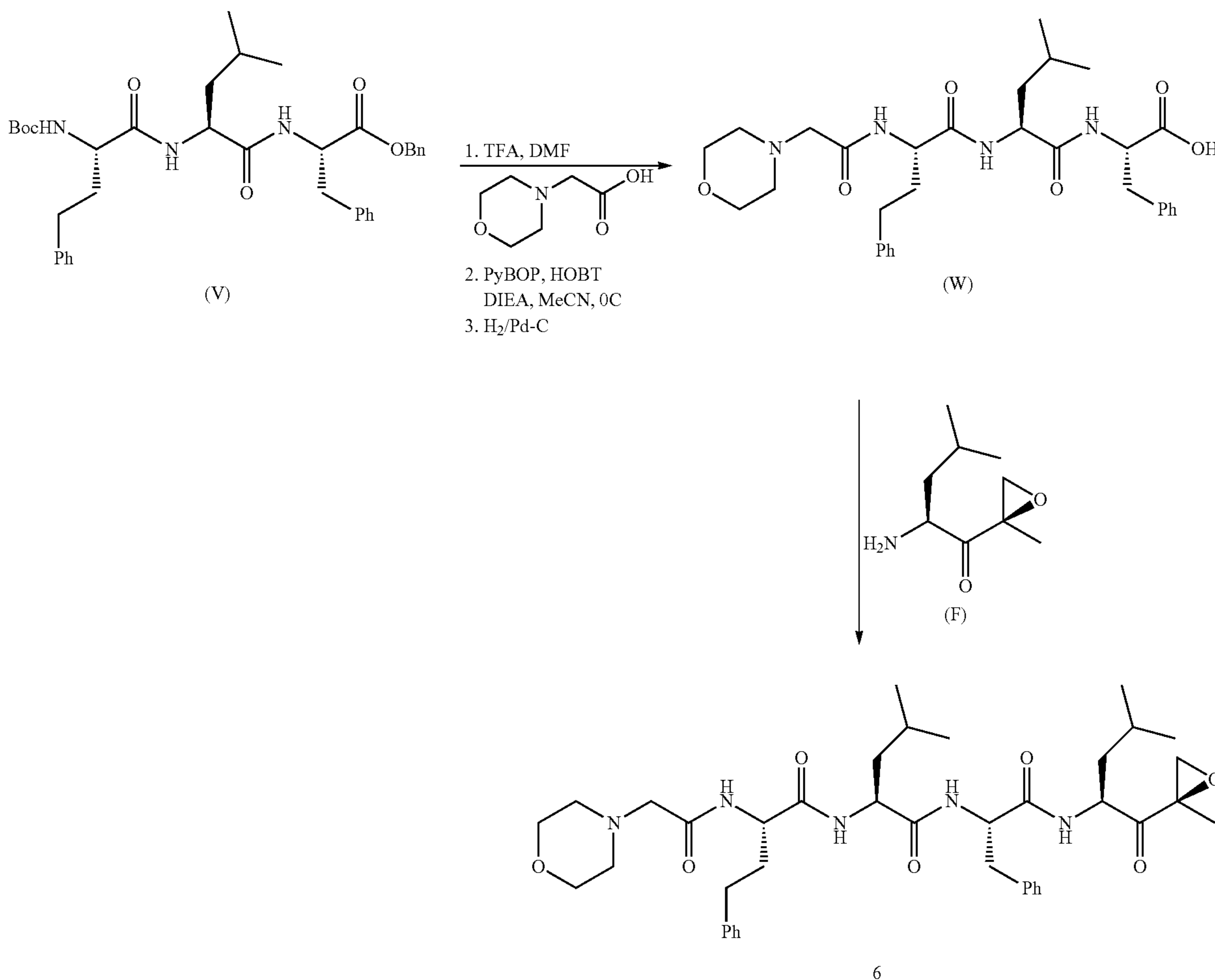
Scheme 6: Synthesis of Example 6
