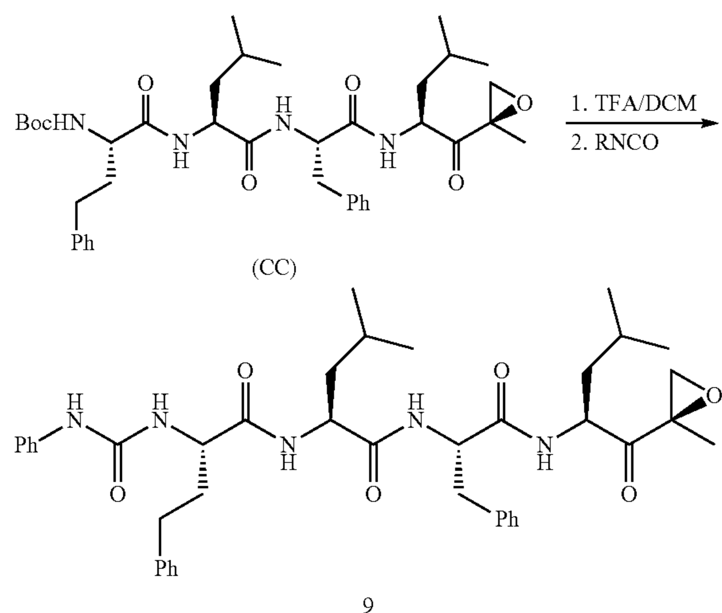
Scheme 9: Synthesis of Example 9
