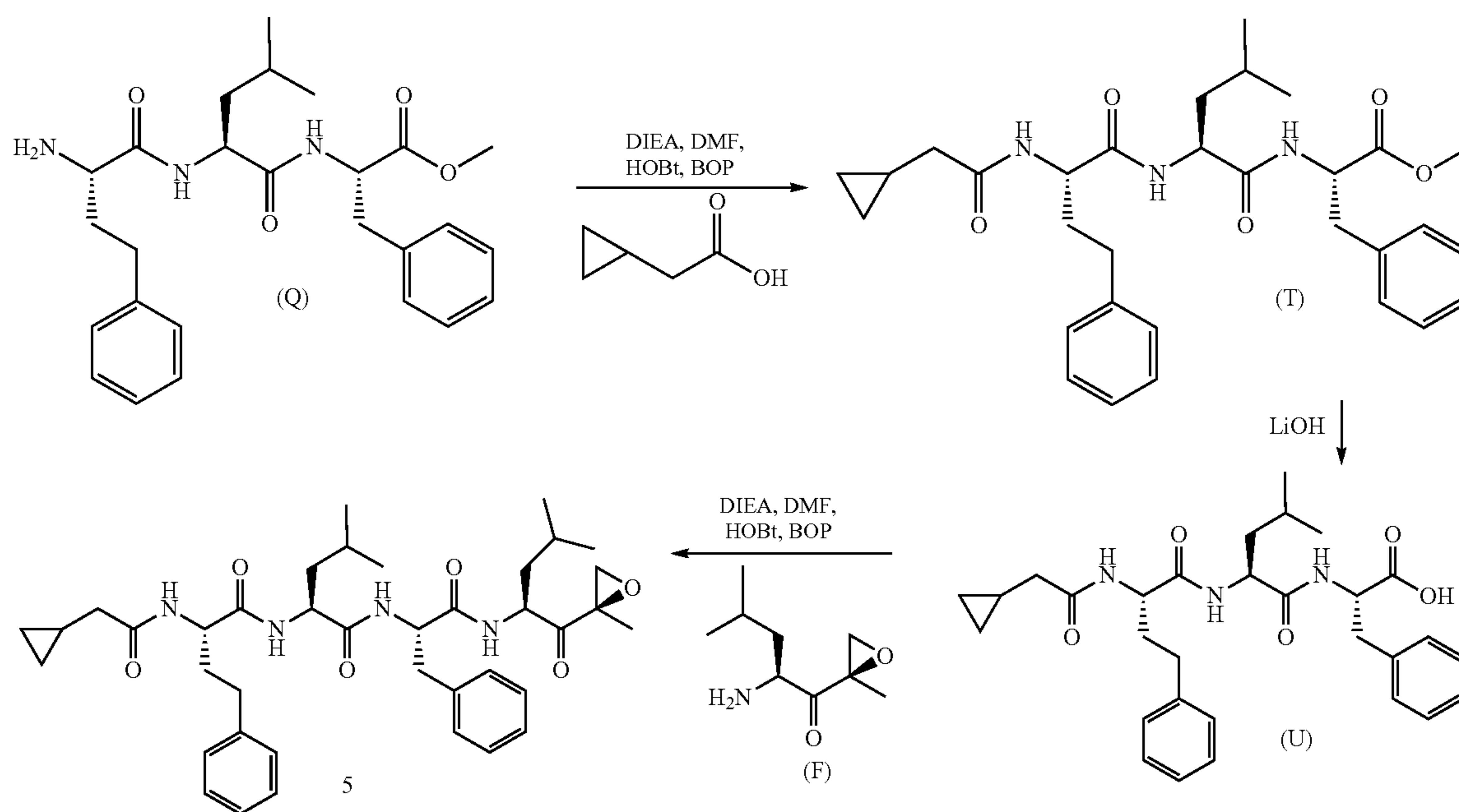
Scheme 5: Synthesis of Example 5
