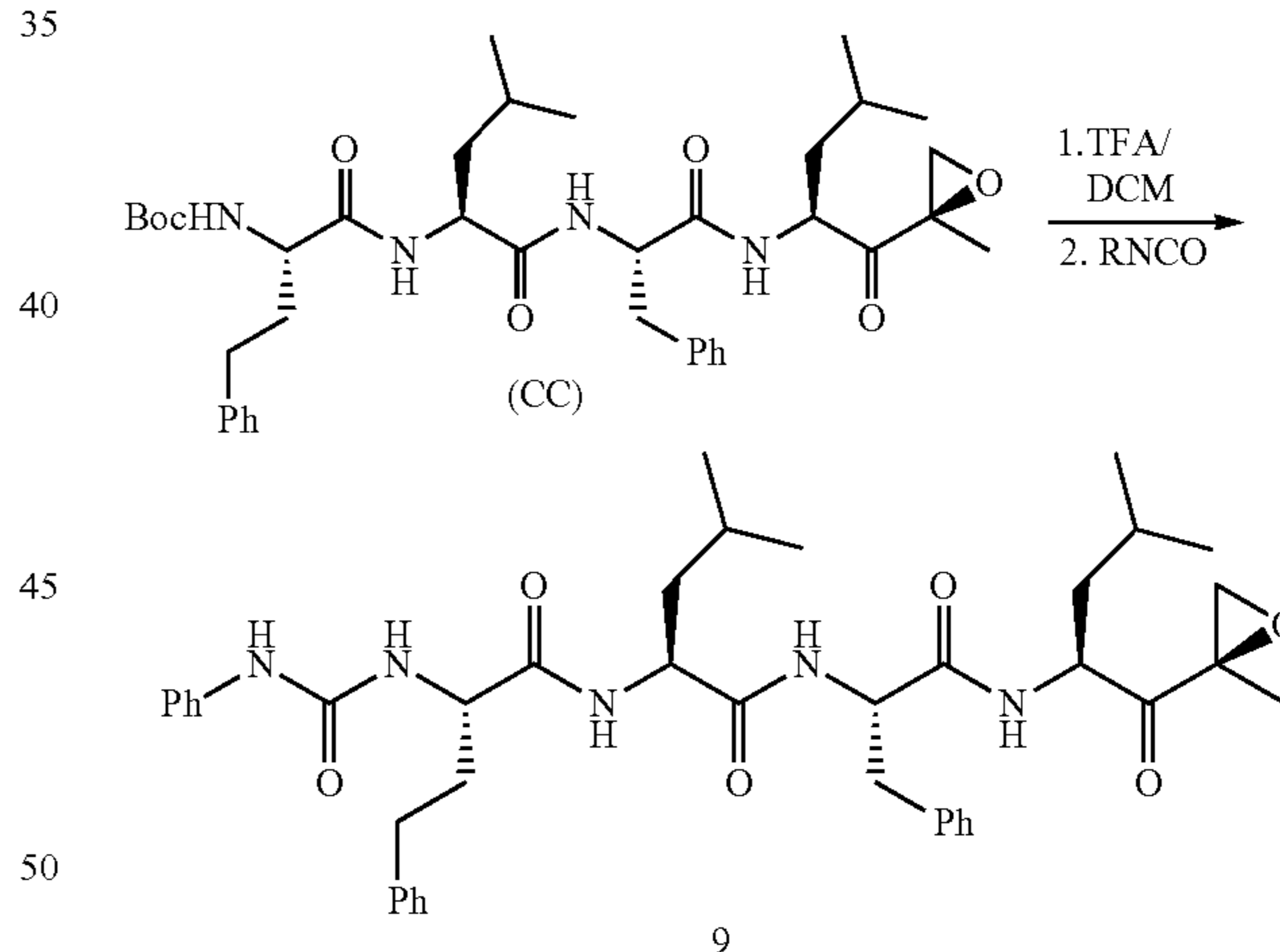
Scheme 9: Synthesis of Example 9
