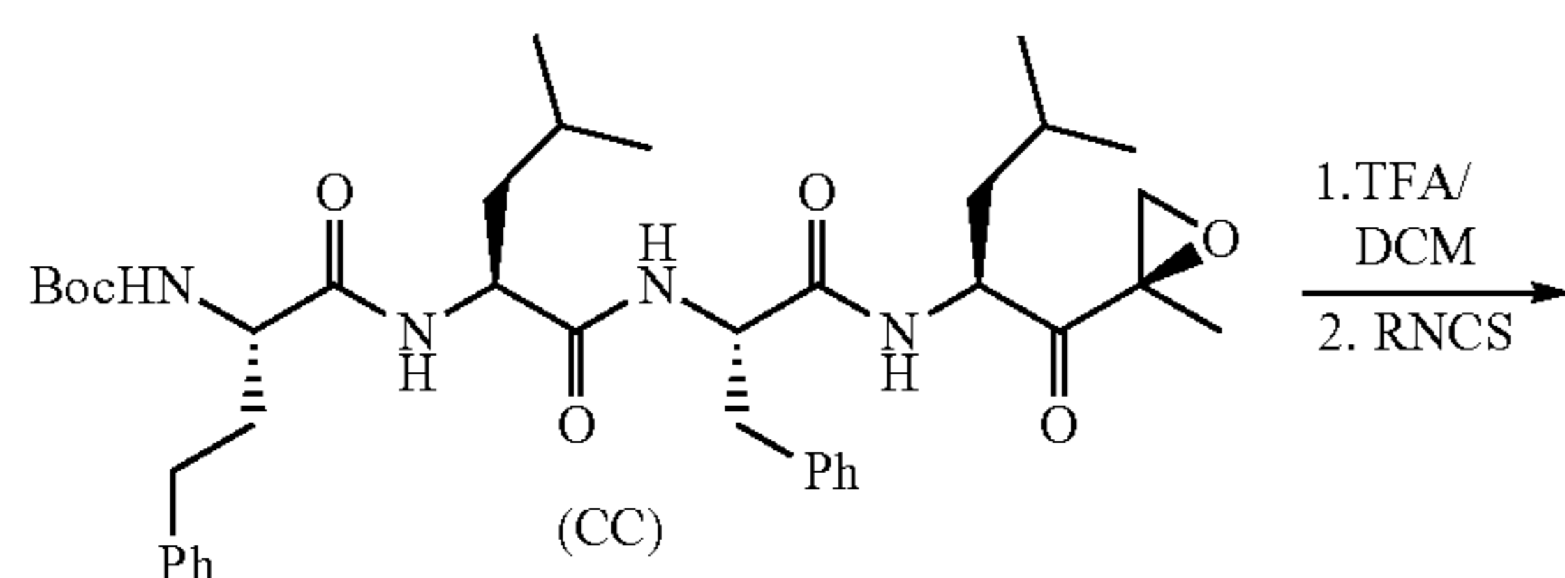
Scheme 10: Synthesis of Example 10
