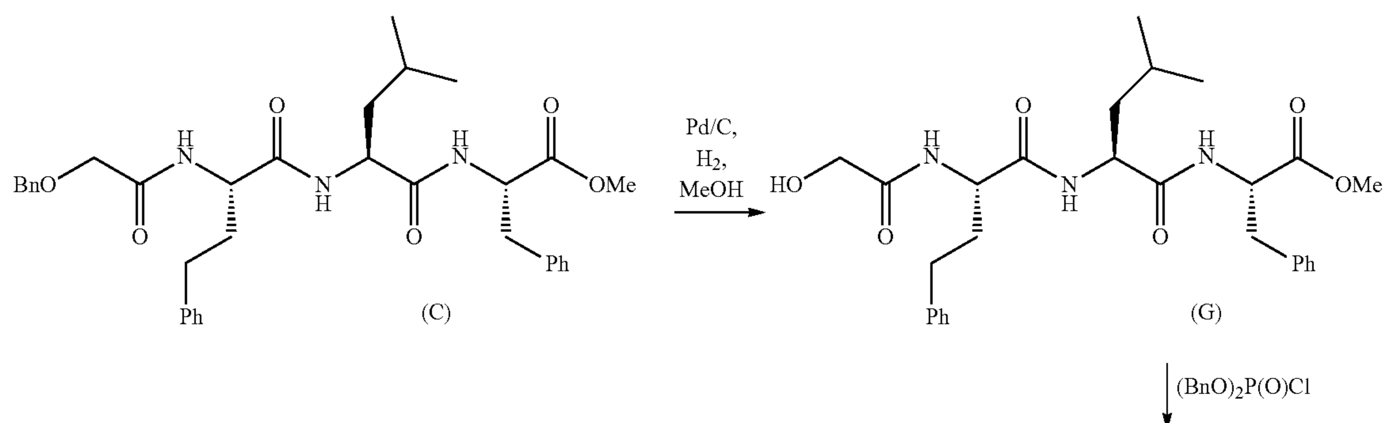
Scheme 2: Synthesis of Example 2
