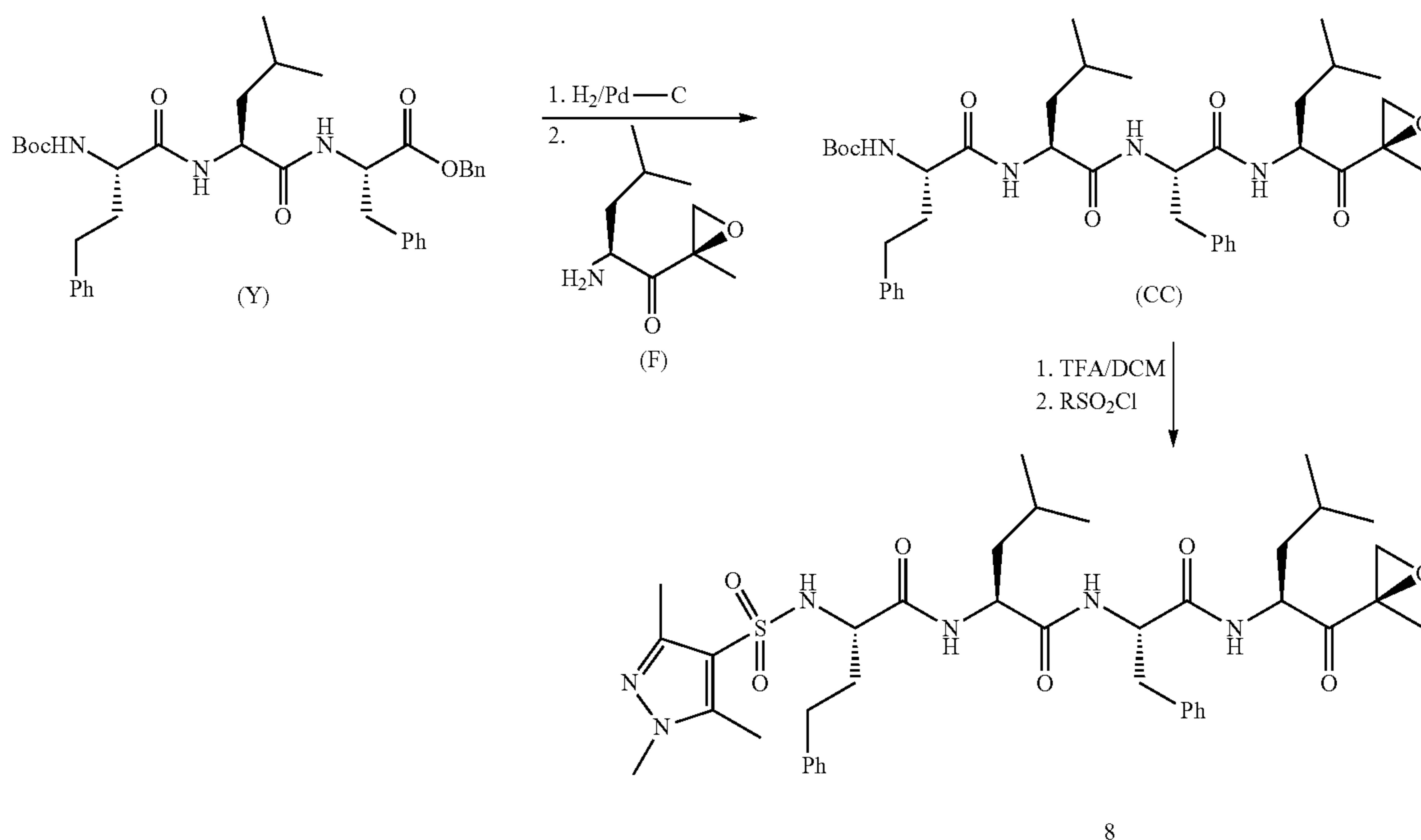
Scheme 8: Synthesis of Example 8
