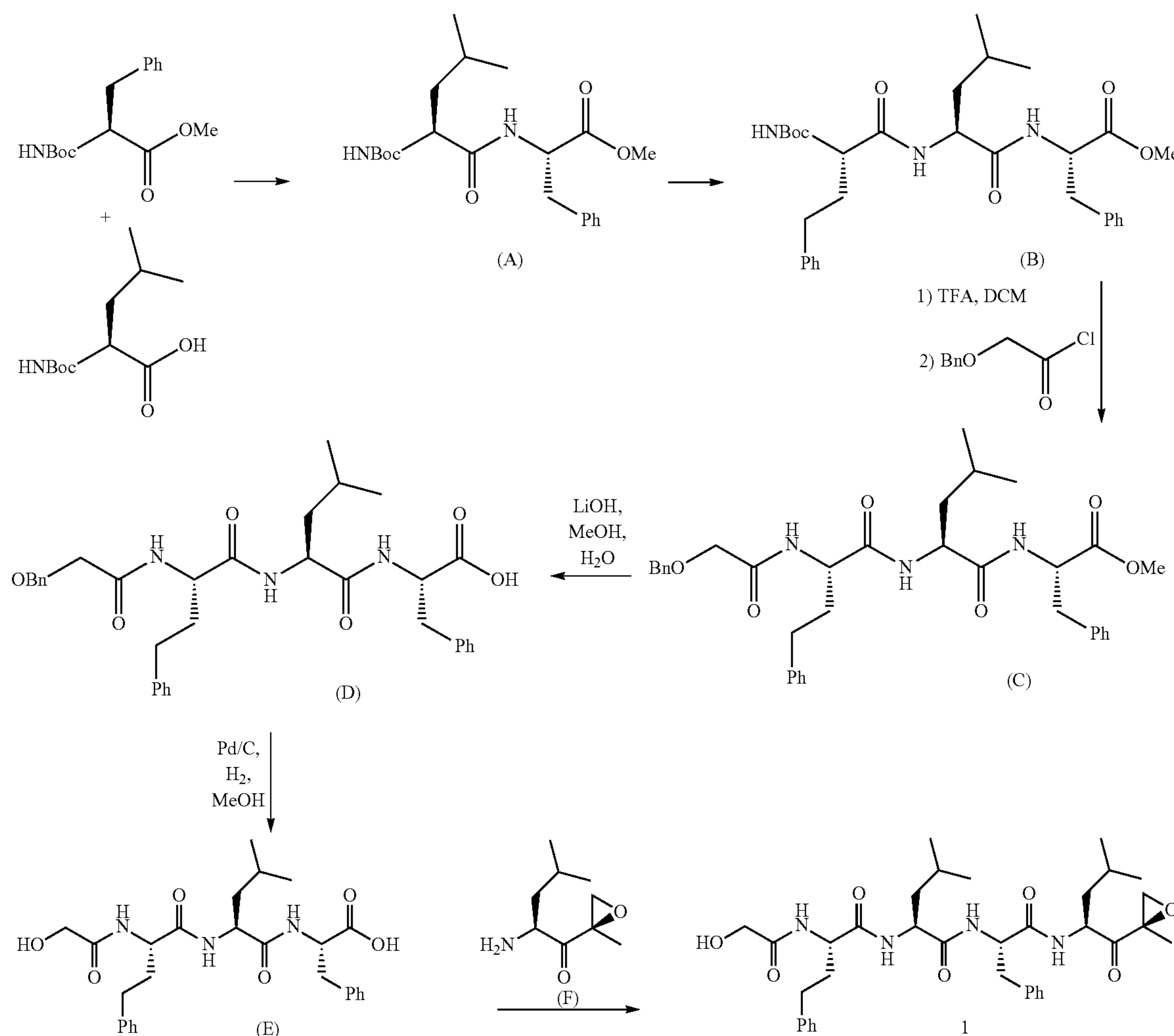
Scheme 1: Synthesis of Example 1
