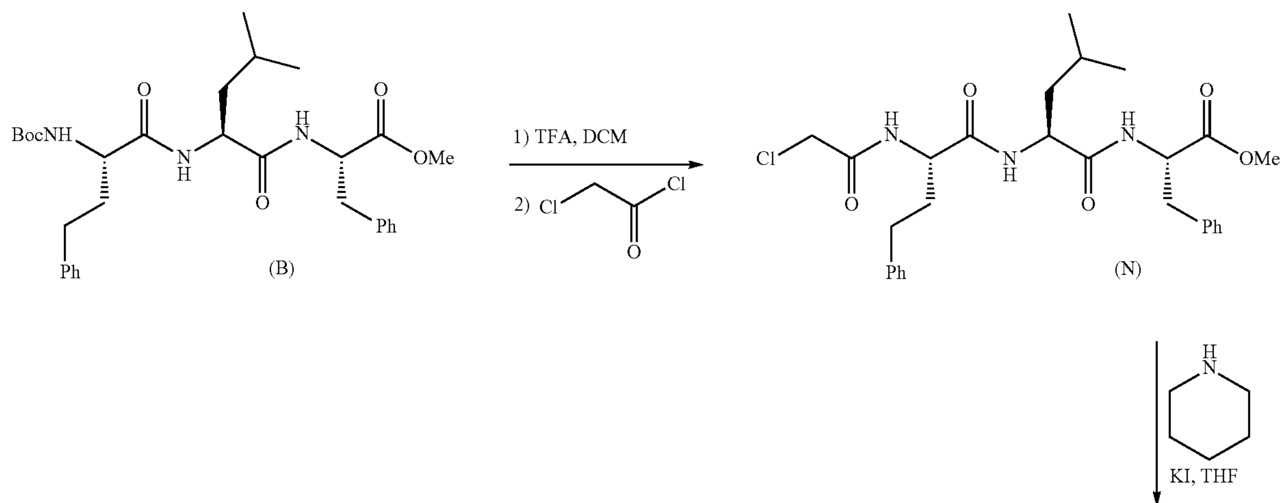
Scheme 4: Synthesis of Example 4
