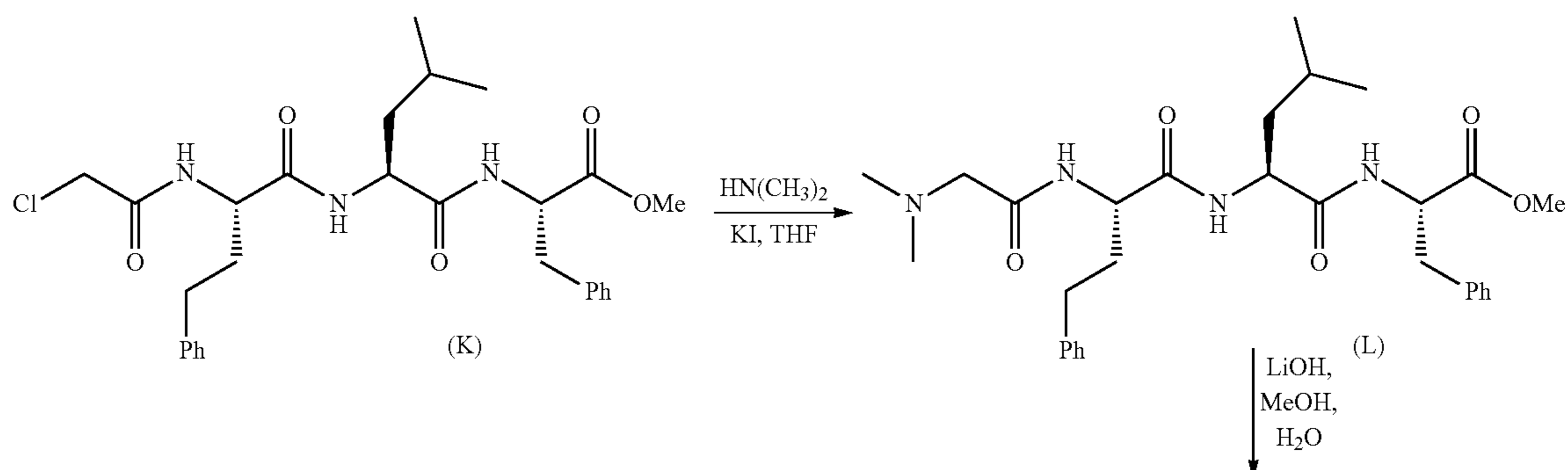
Scheme 3: Synthesis of Example 3
