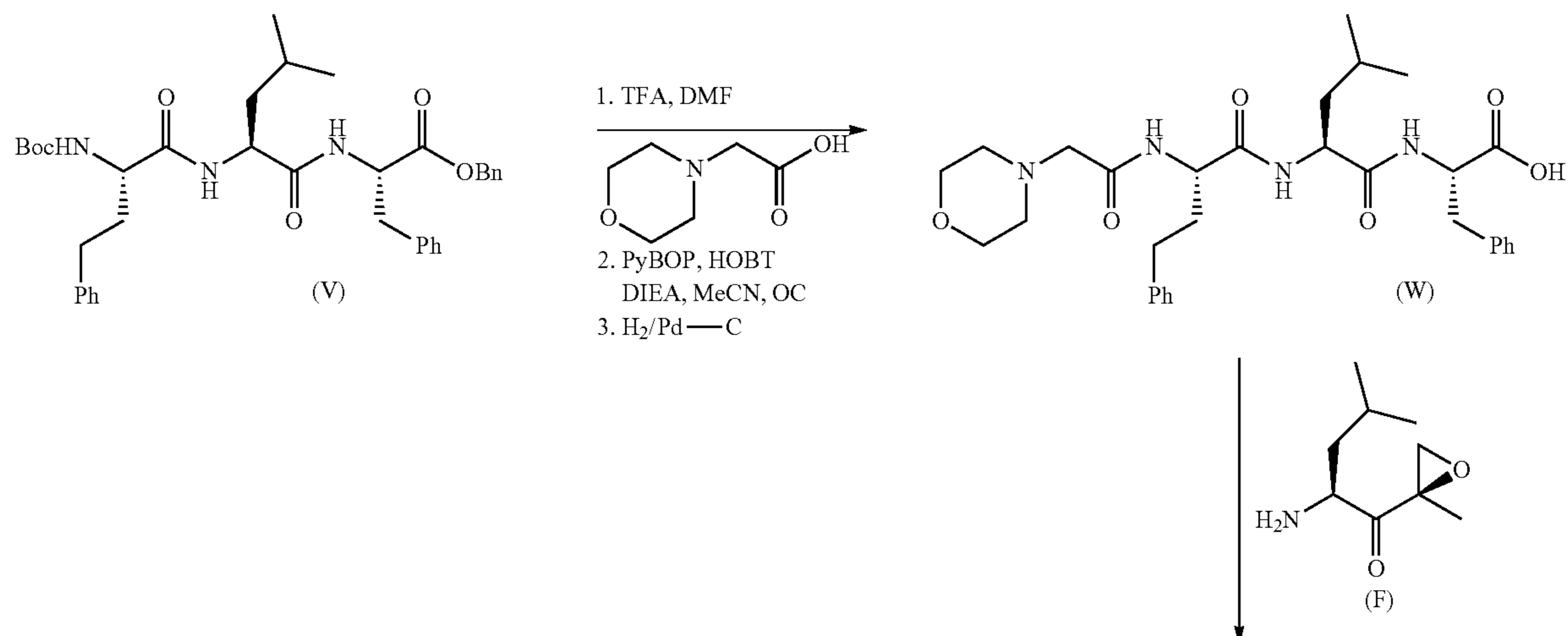
Scheme 6: Synthesis of Example 6
