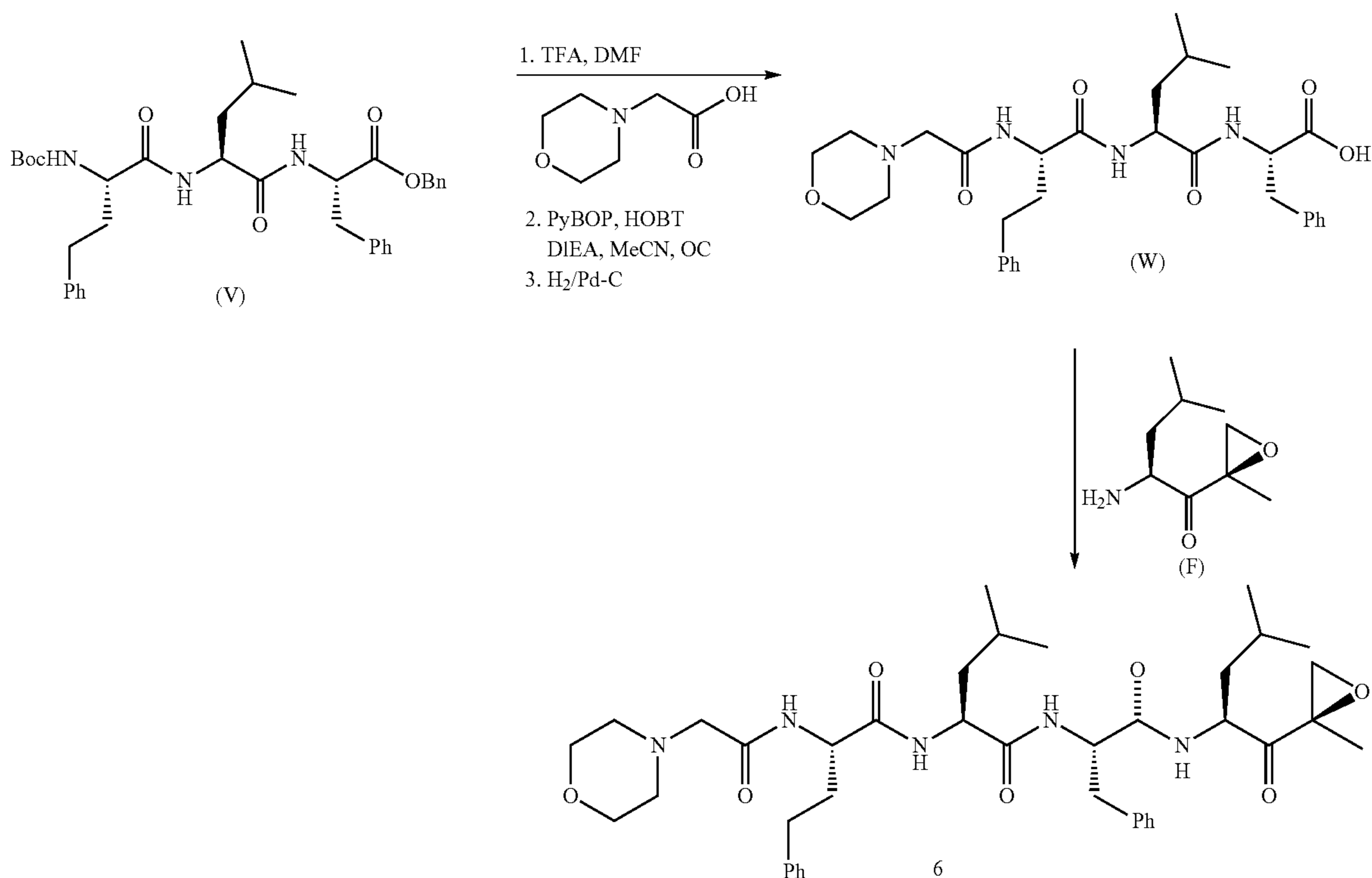
Scheme 6: Synthesis of Example 6
