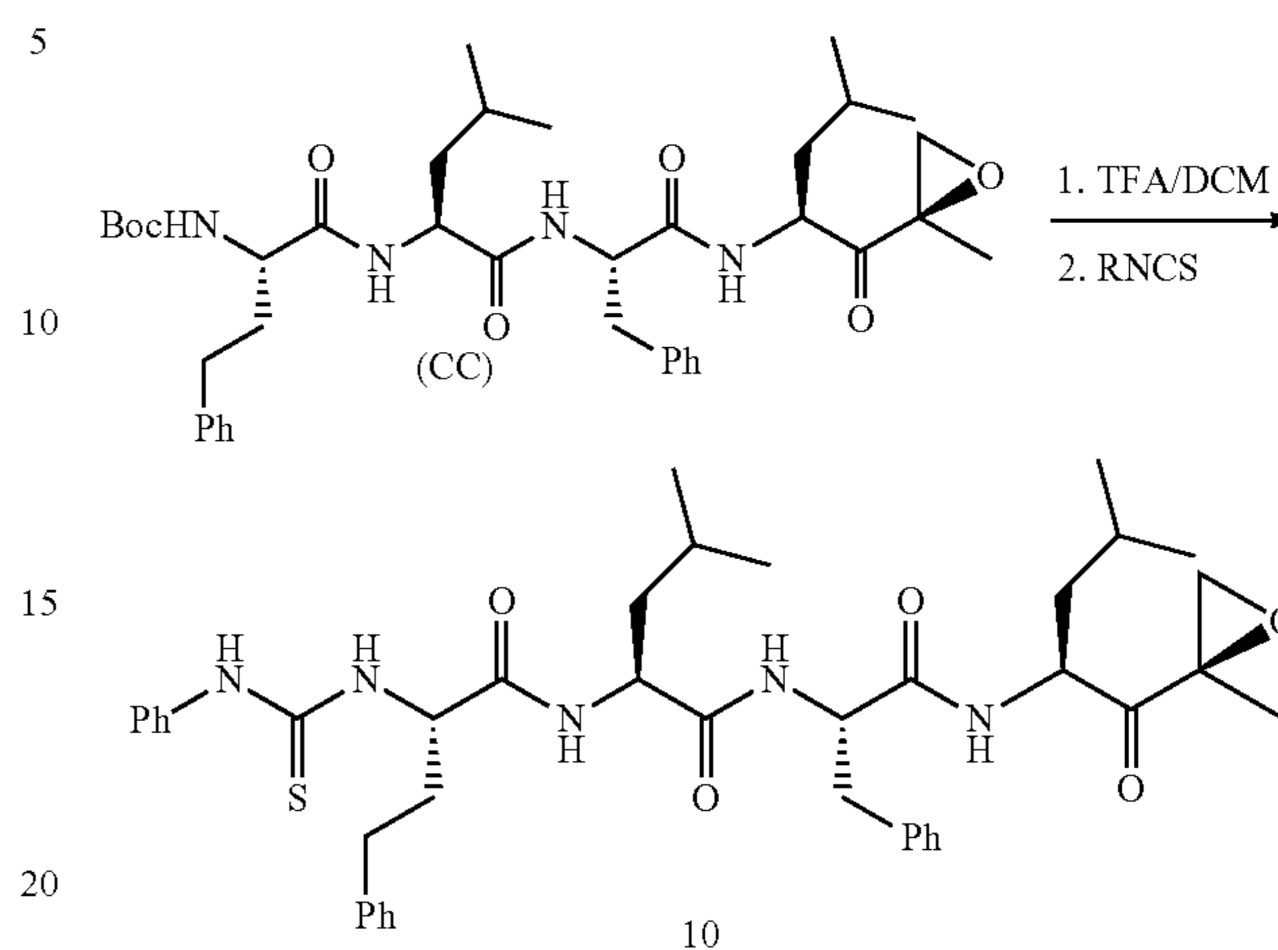
Scheme 10: Synthesis of Example 10
