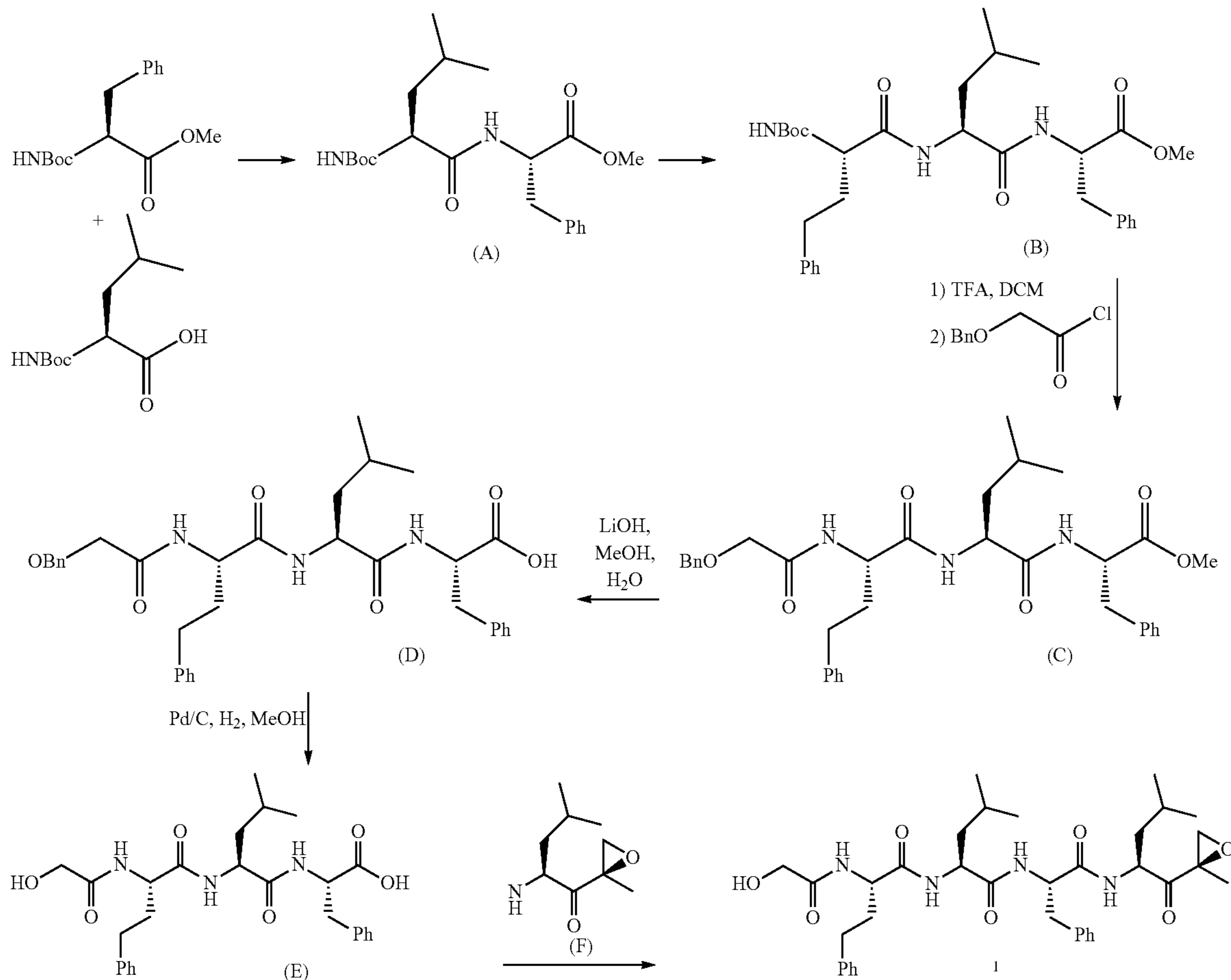
Scheme 1: Synthesis of Example 1
