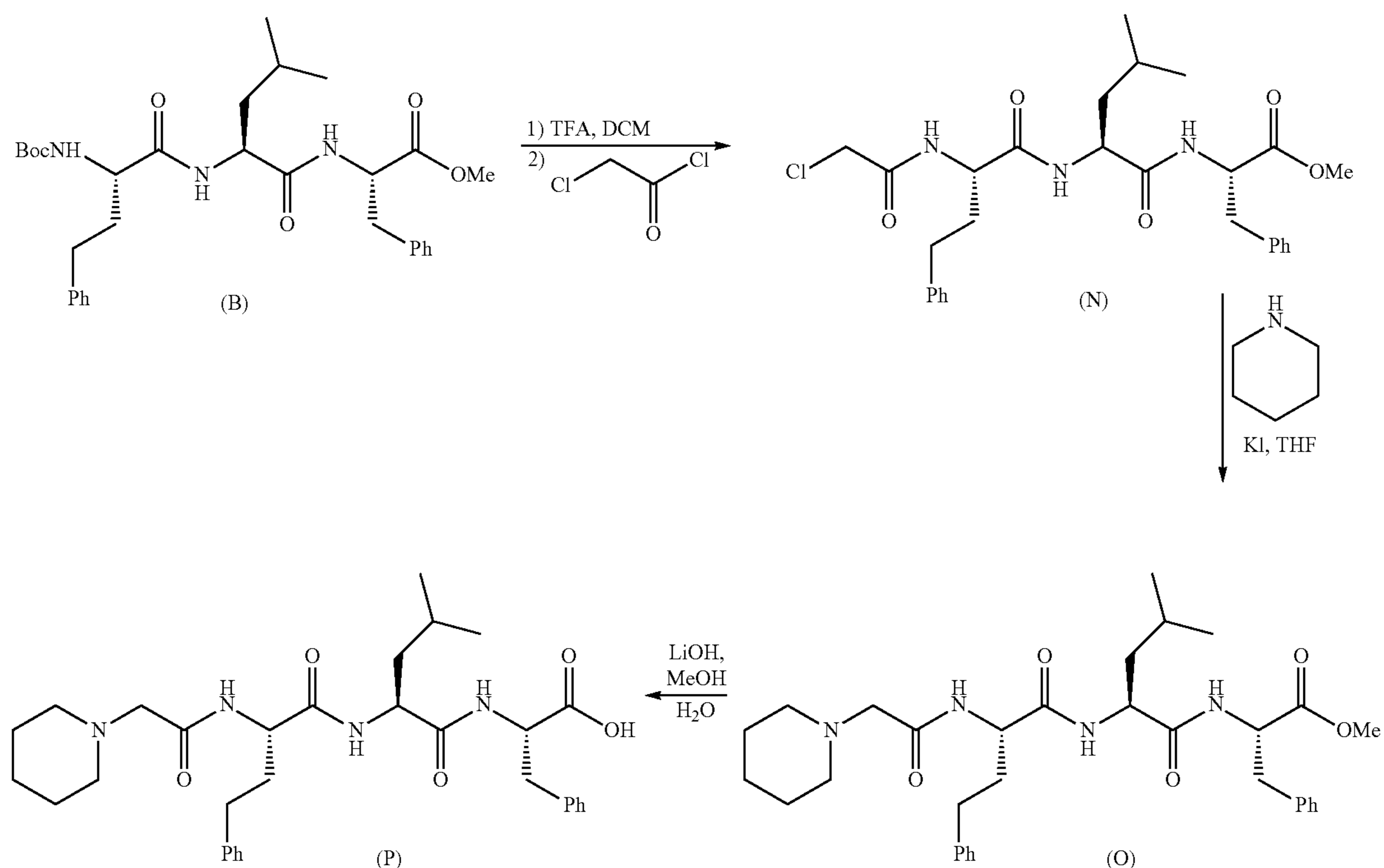
Scheme 4: Synthesis of Example 4
