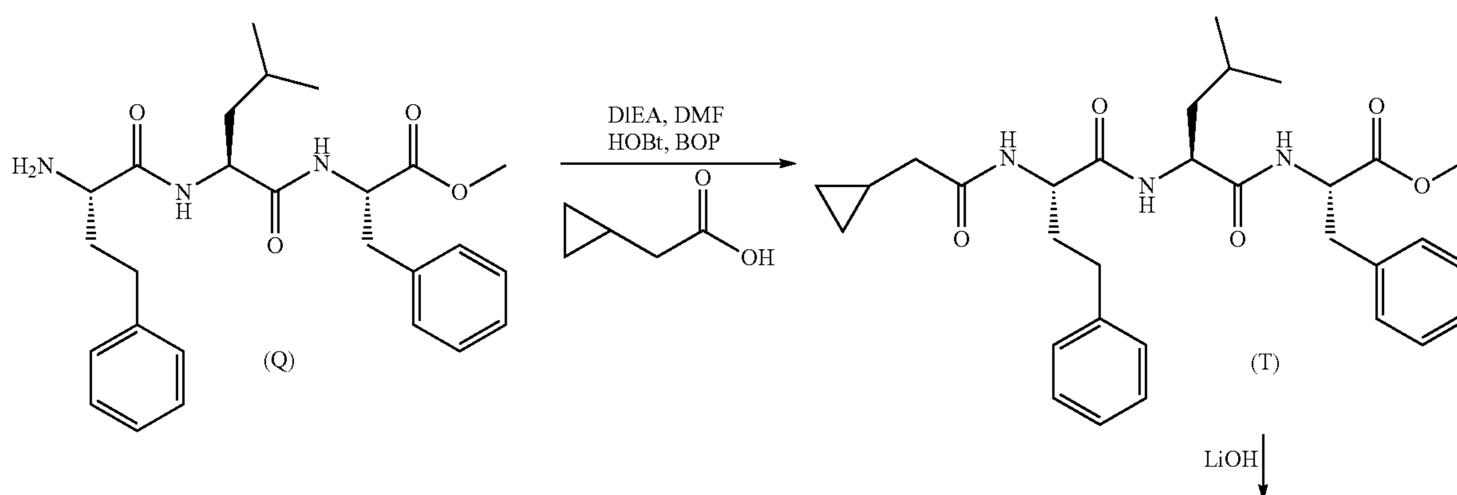
Scheme 5: Synthesis of Example 5
