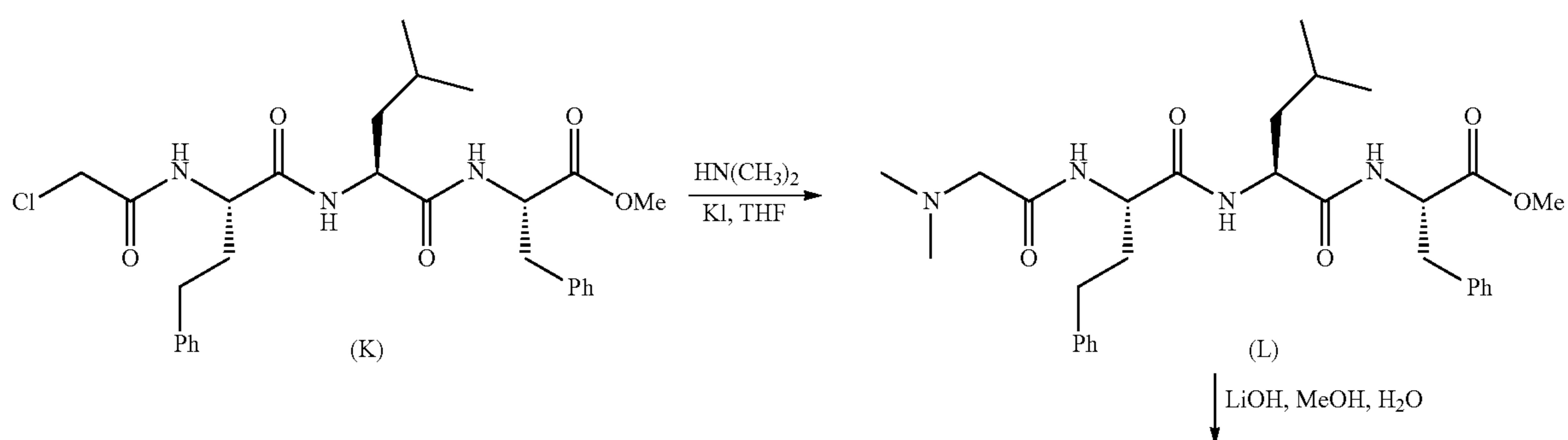
Scheme 3: Synthesis of Example 3
