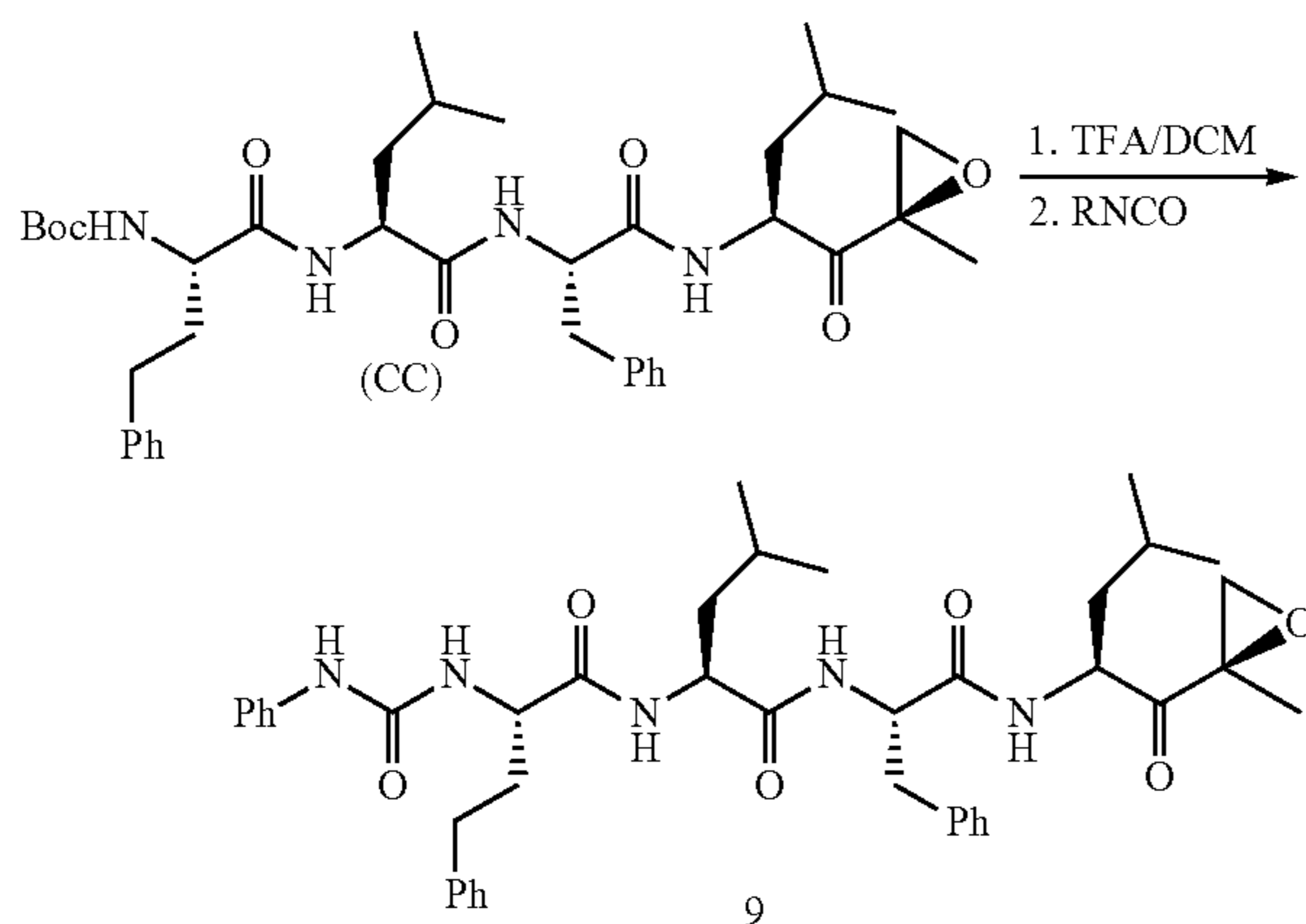
Scheme 9: Synthesis of Example 9
