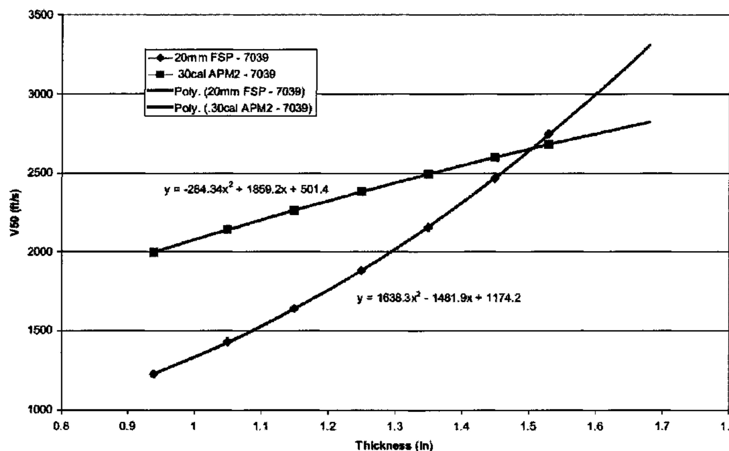
V50 vs. Thickness for 7039
