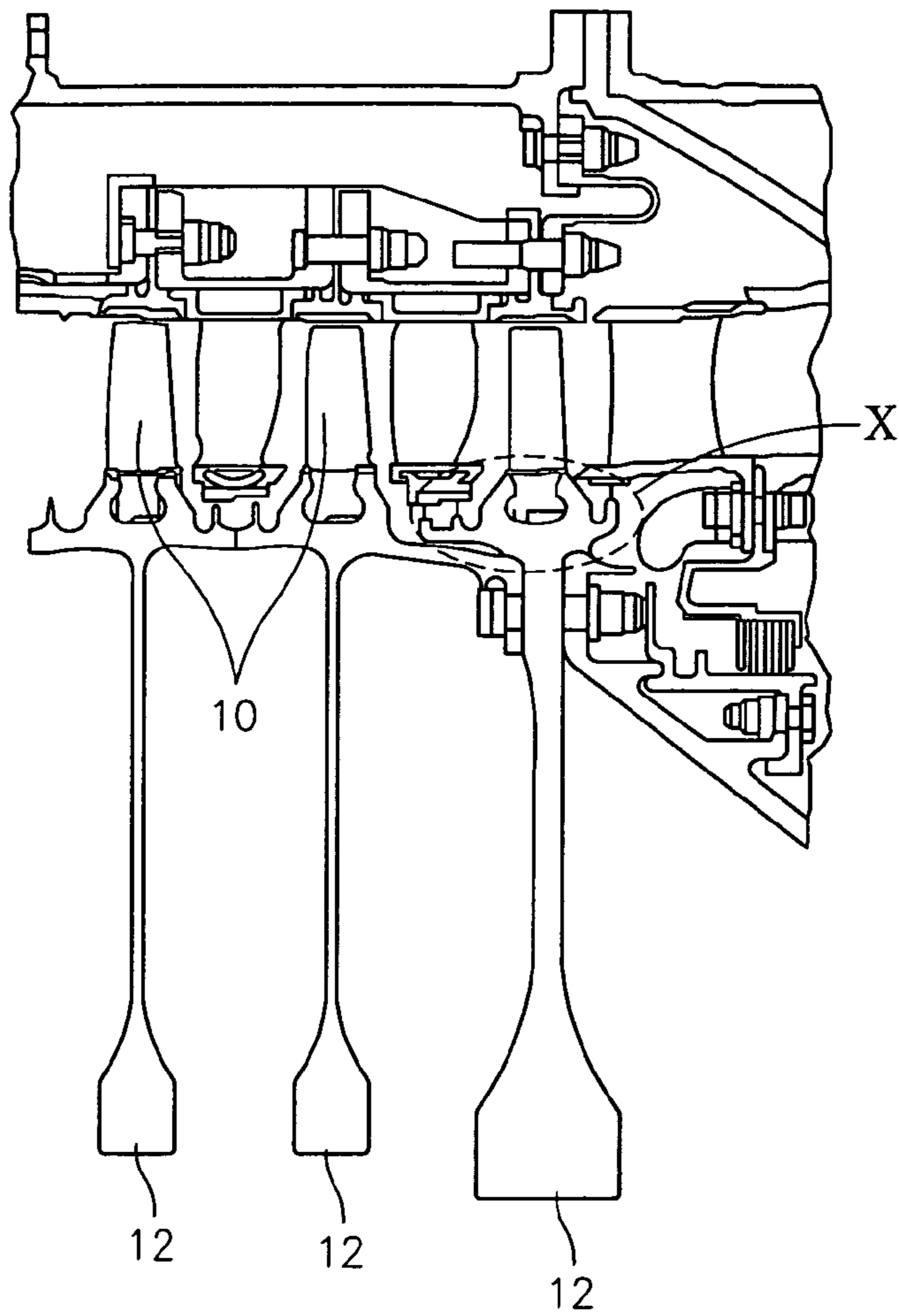
FIG. 1 (PRIOR ART)
