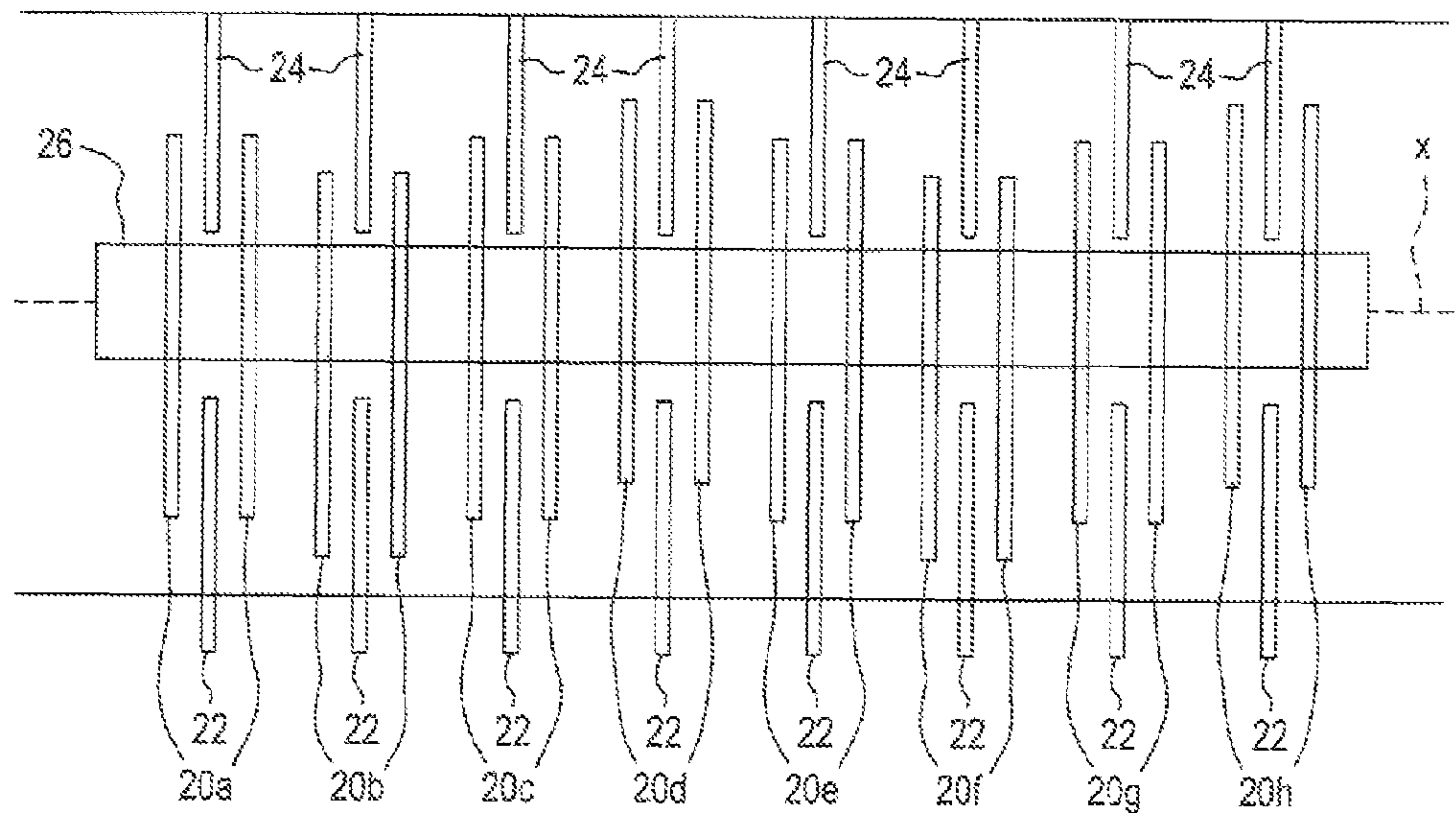
FIG. 3 (PRIOR ART)
