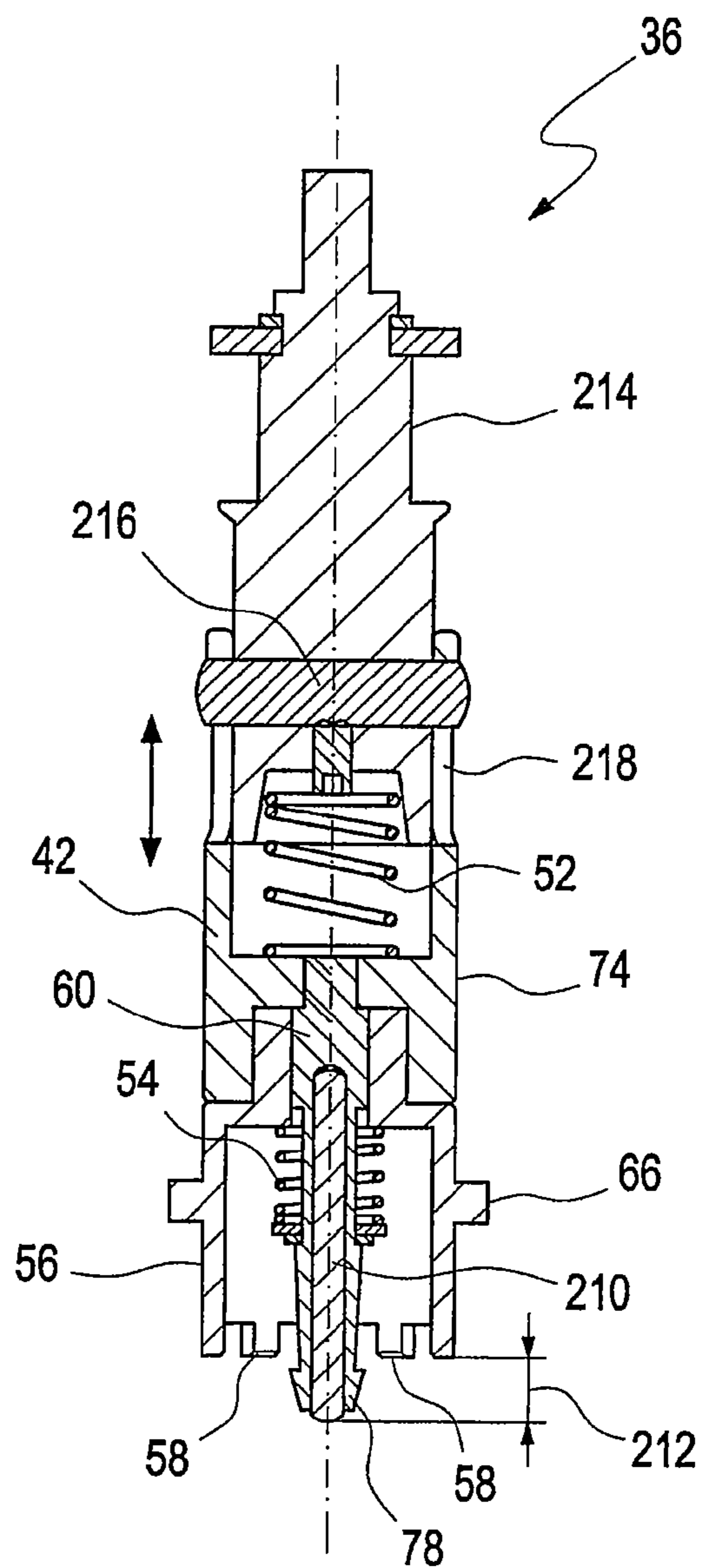
Fig. 12D
