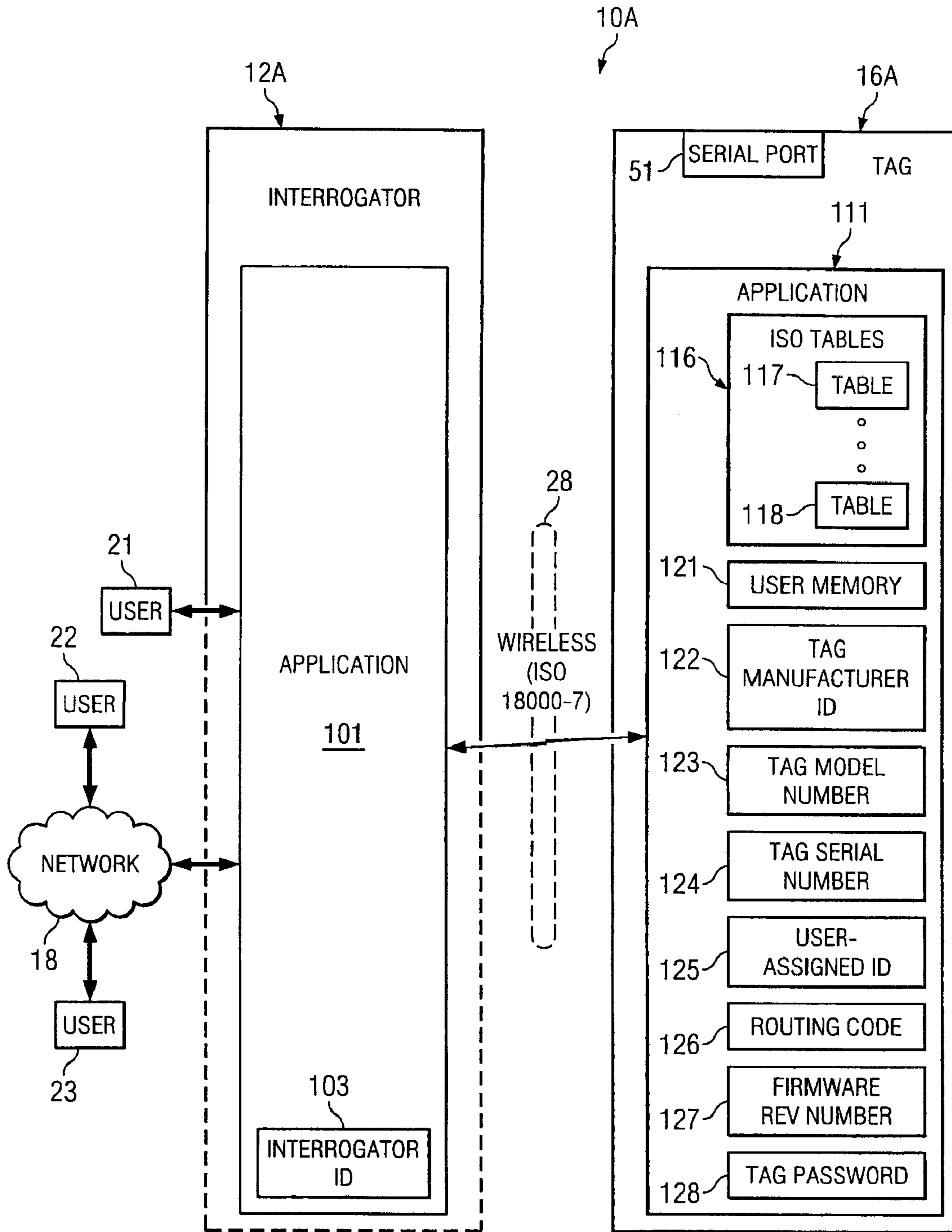
Fig. 2 (PRIOR ART)
