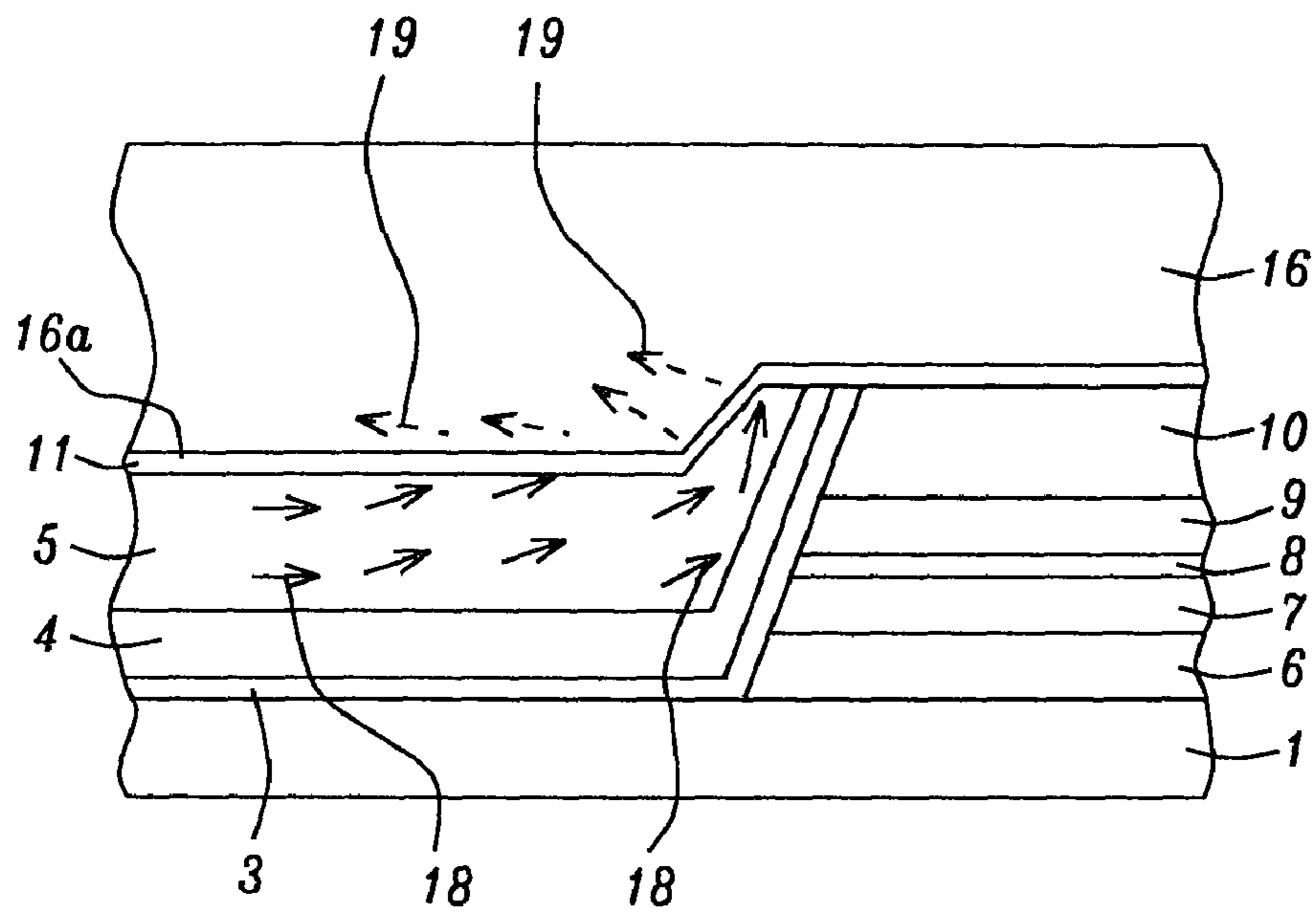
FIG. 4 - Prior Art
