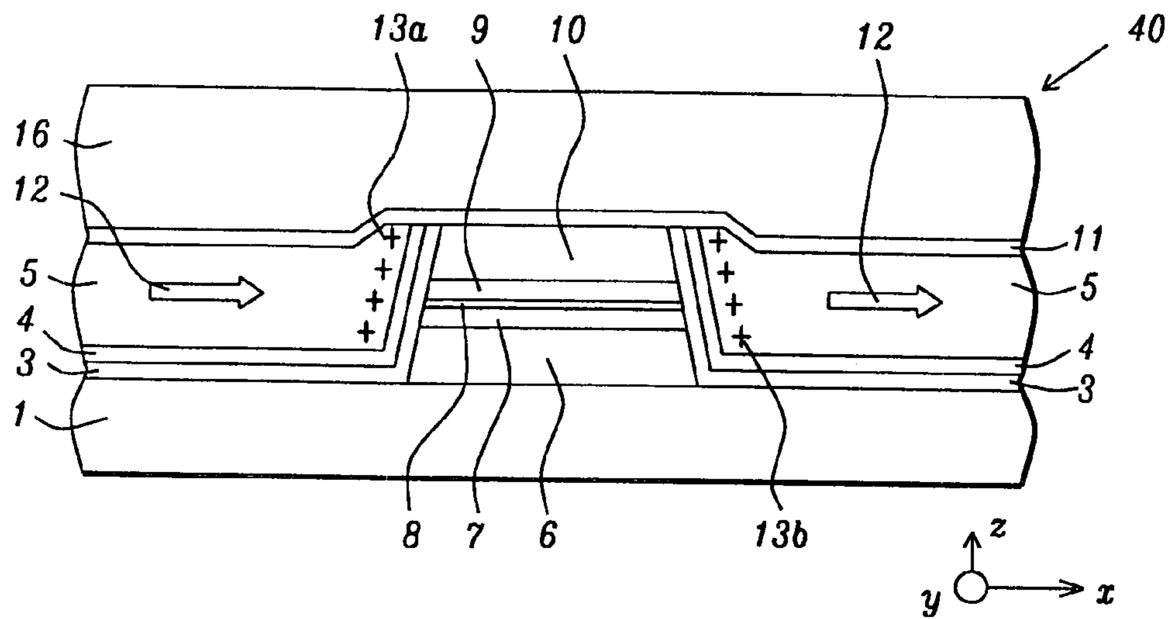
FIG. 1 - Prior Art
