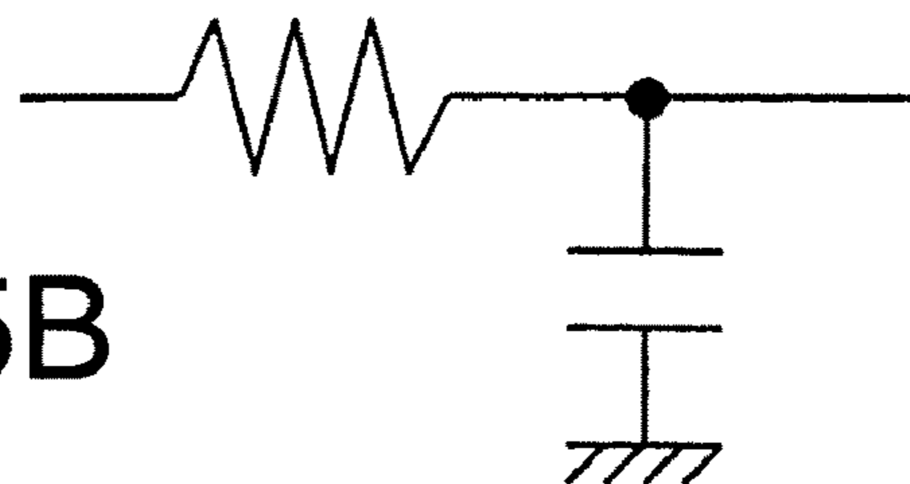
FIRST APPROXIMATION CIRCUIT OF CS BUSLINE LOAD IMPEDANCE: CR LOW PASS FILTER
