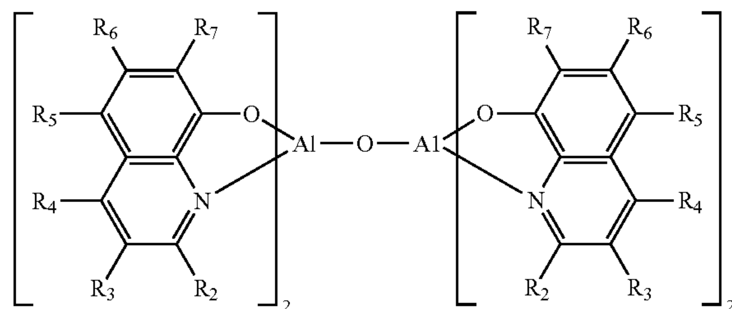
[Chem 4]
