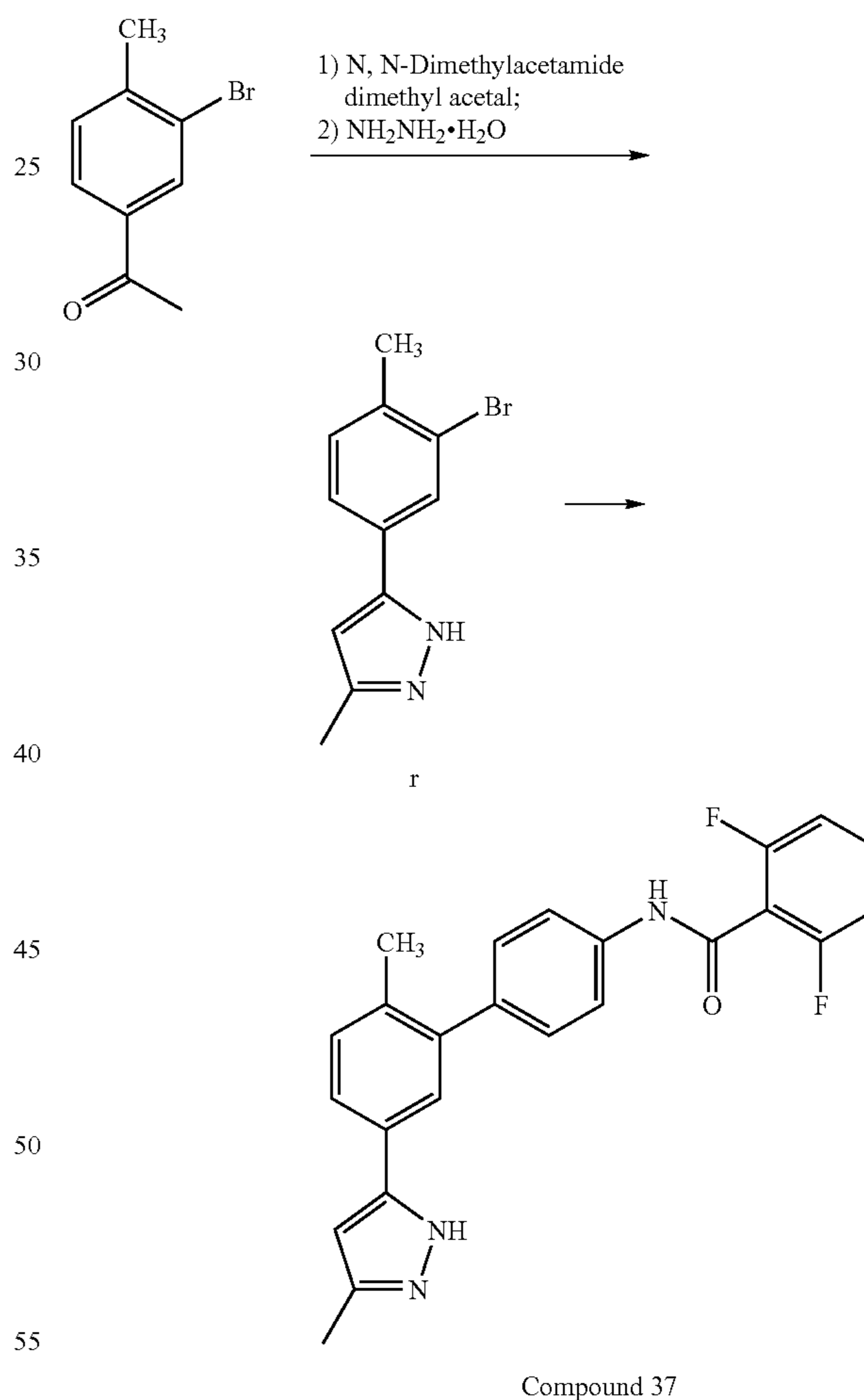
Scheme XIII
