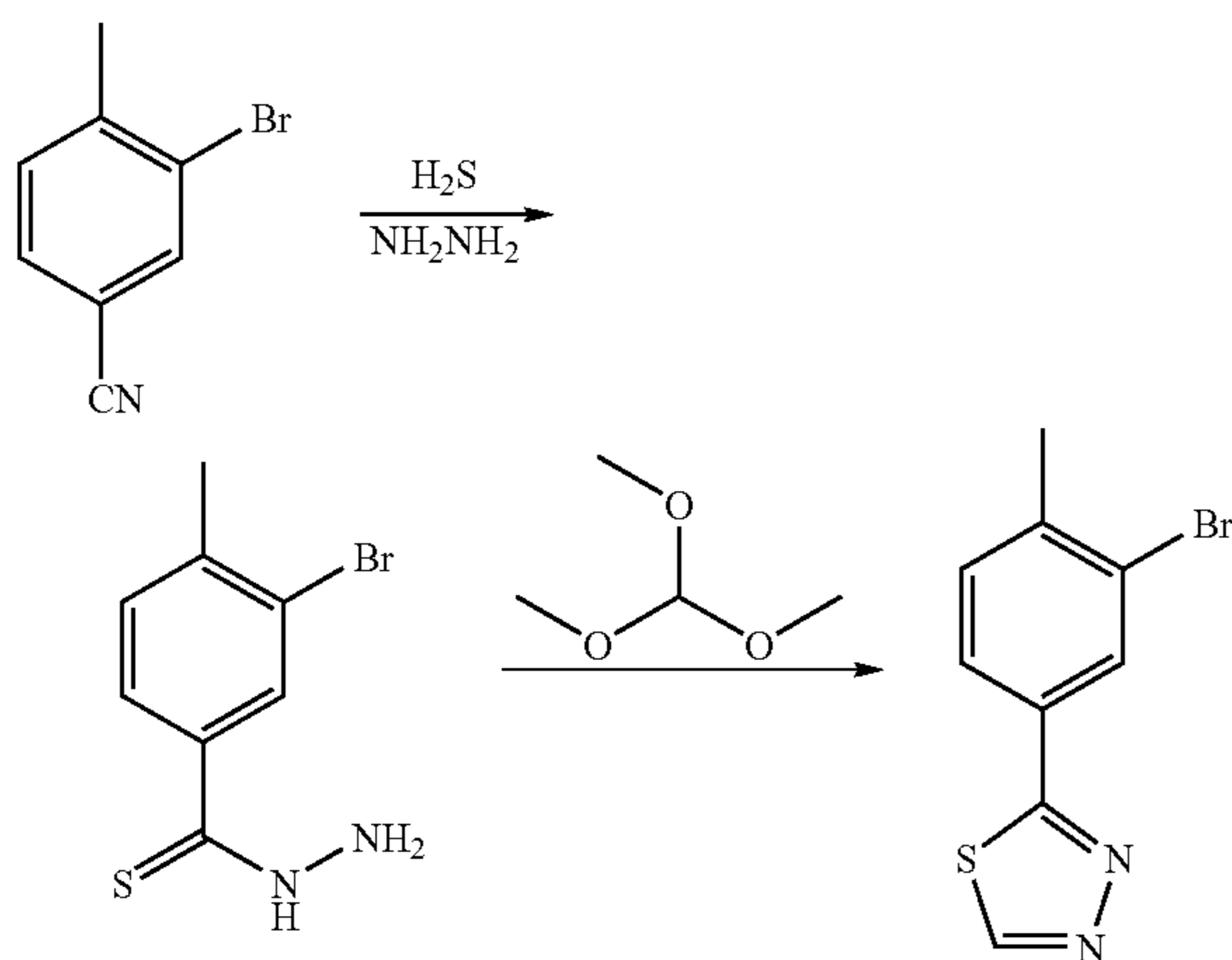
Scheme XXI
