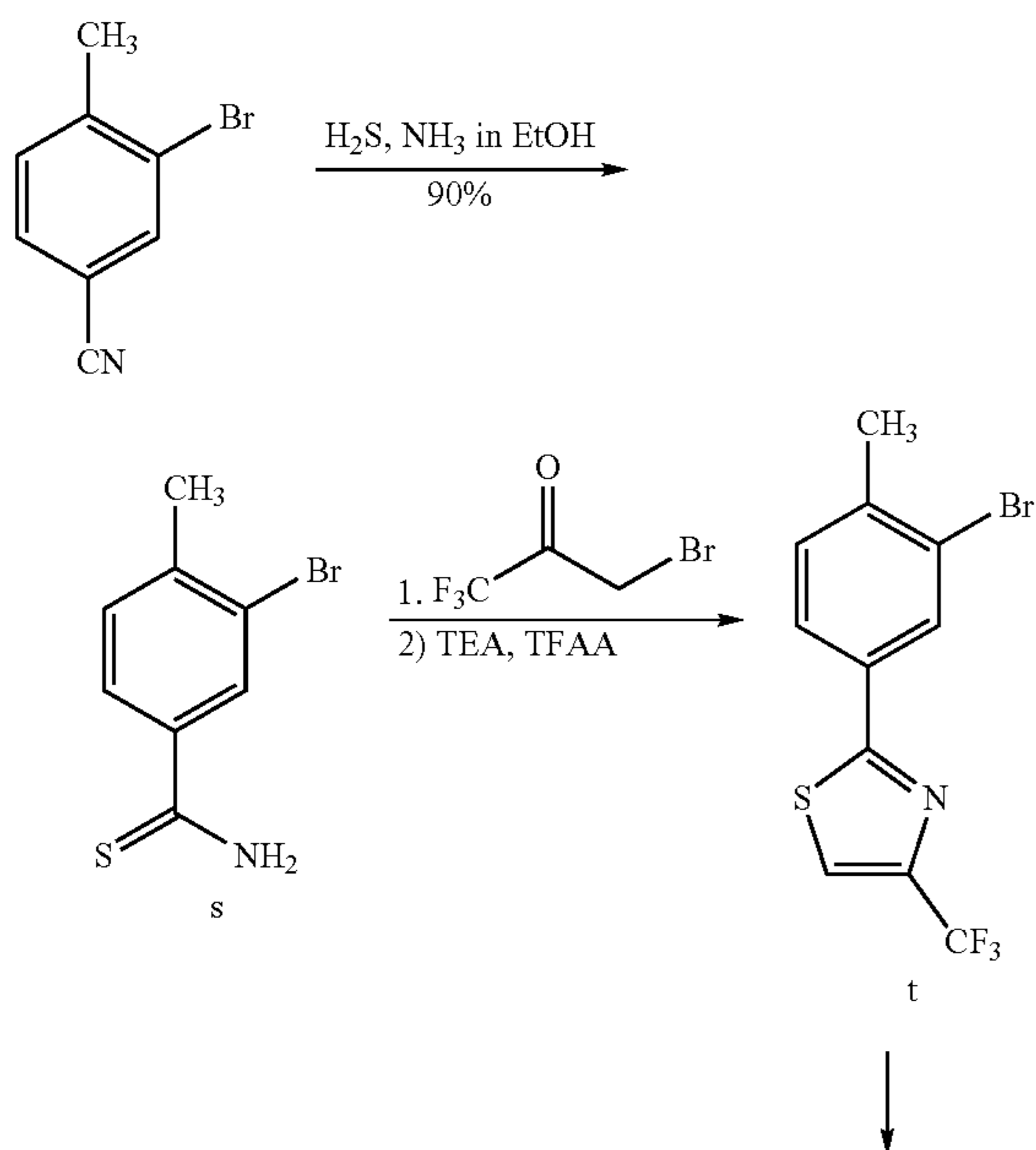
Scheme XV
