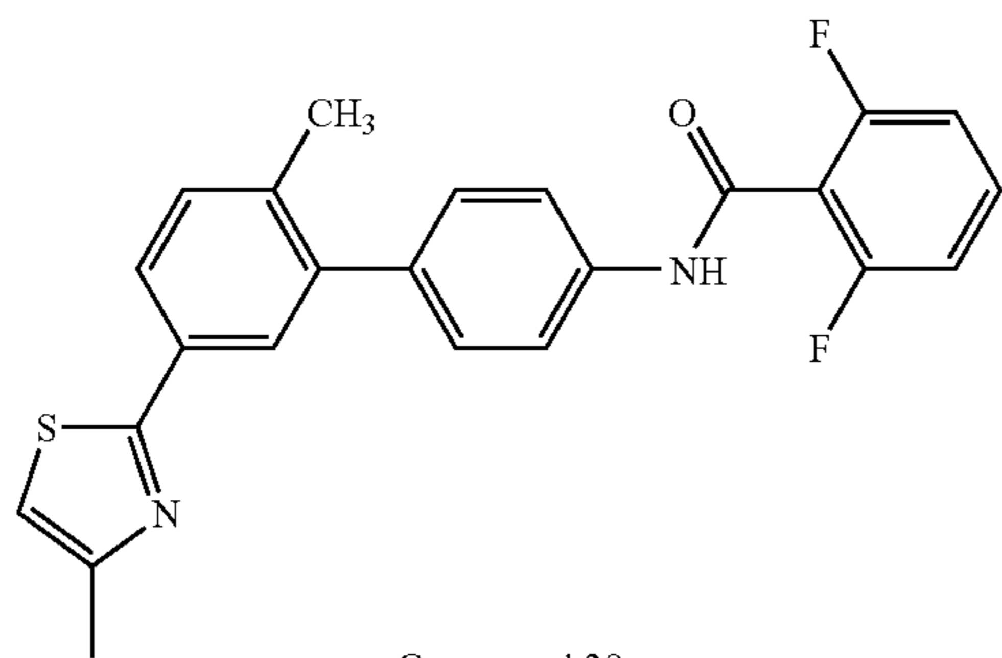
Compound 38
