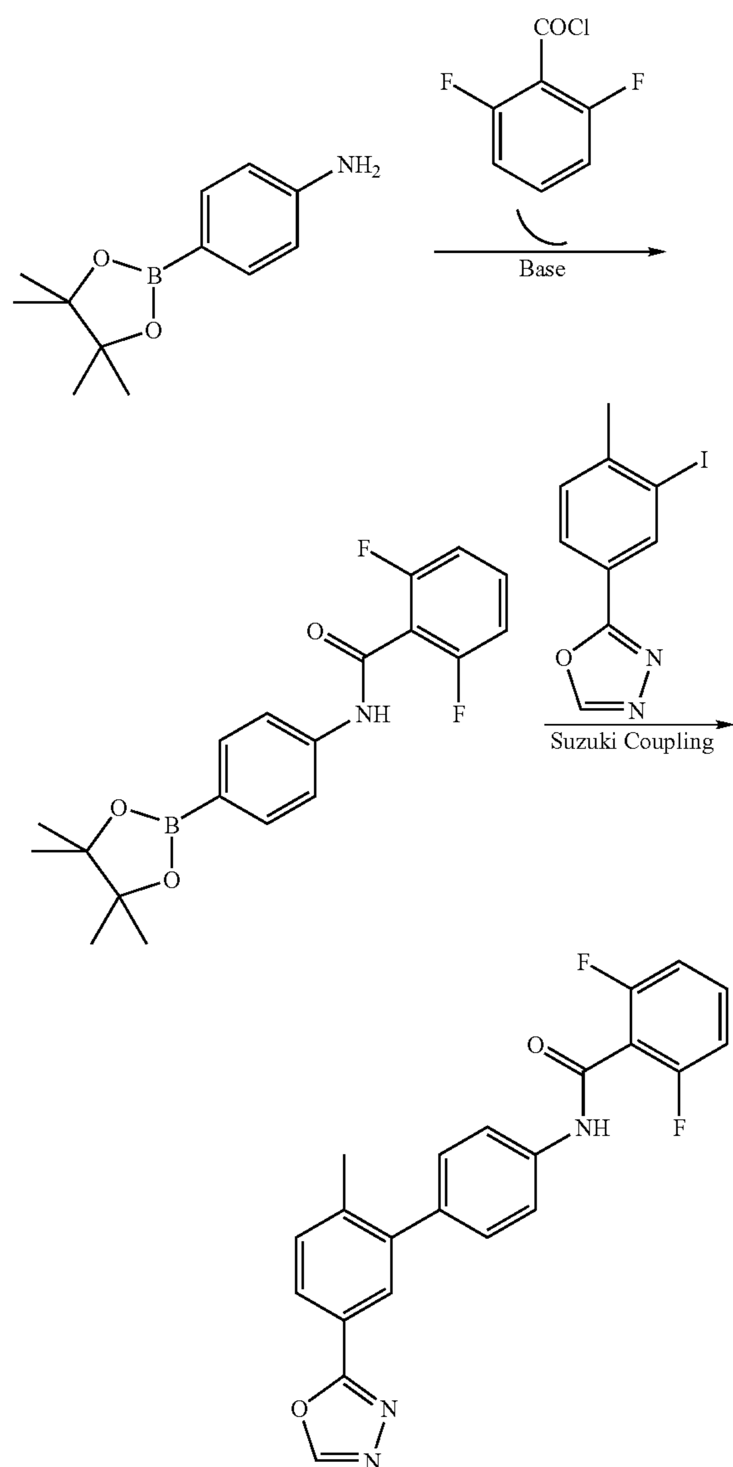
Compound 69
