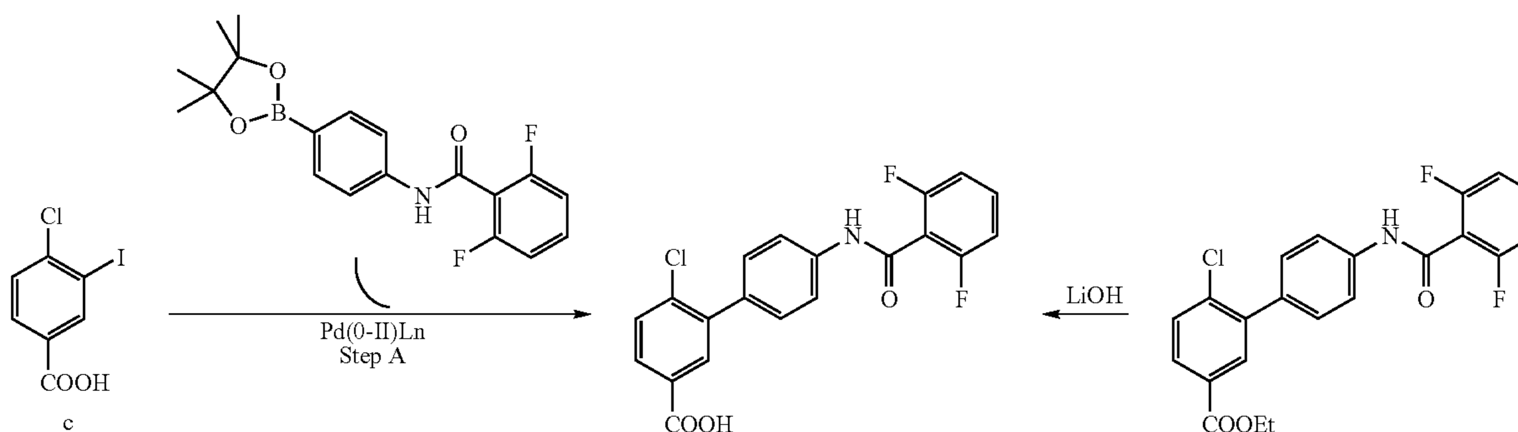
Scheme II
