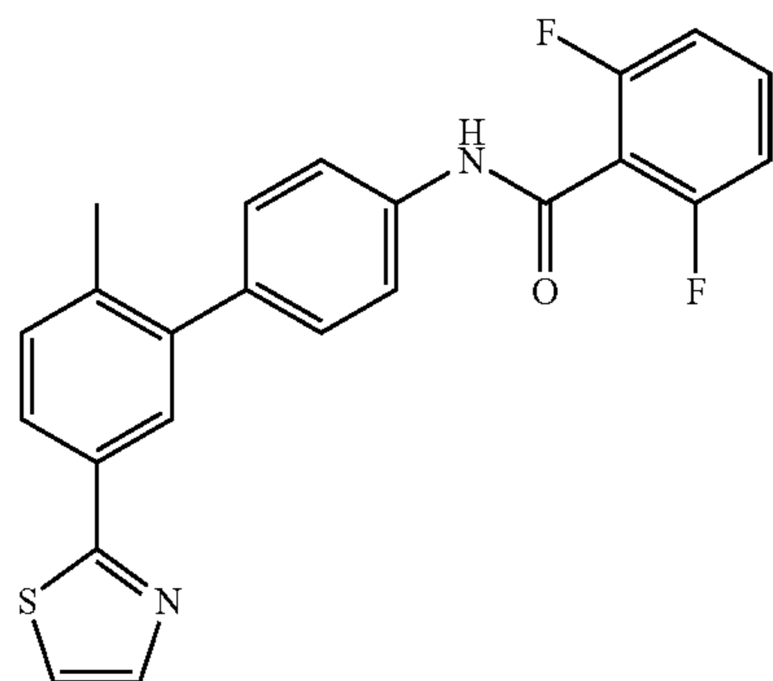
Compound 15
