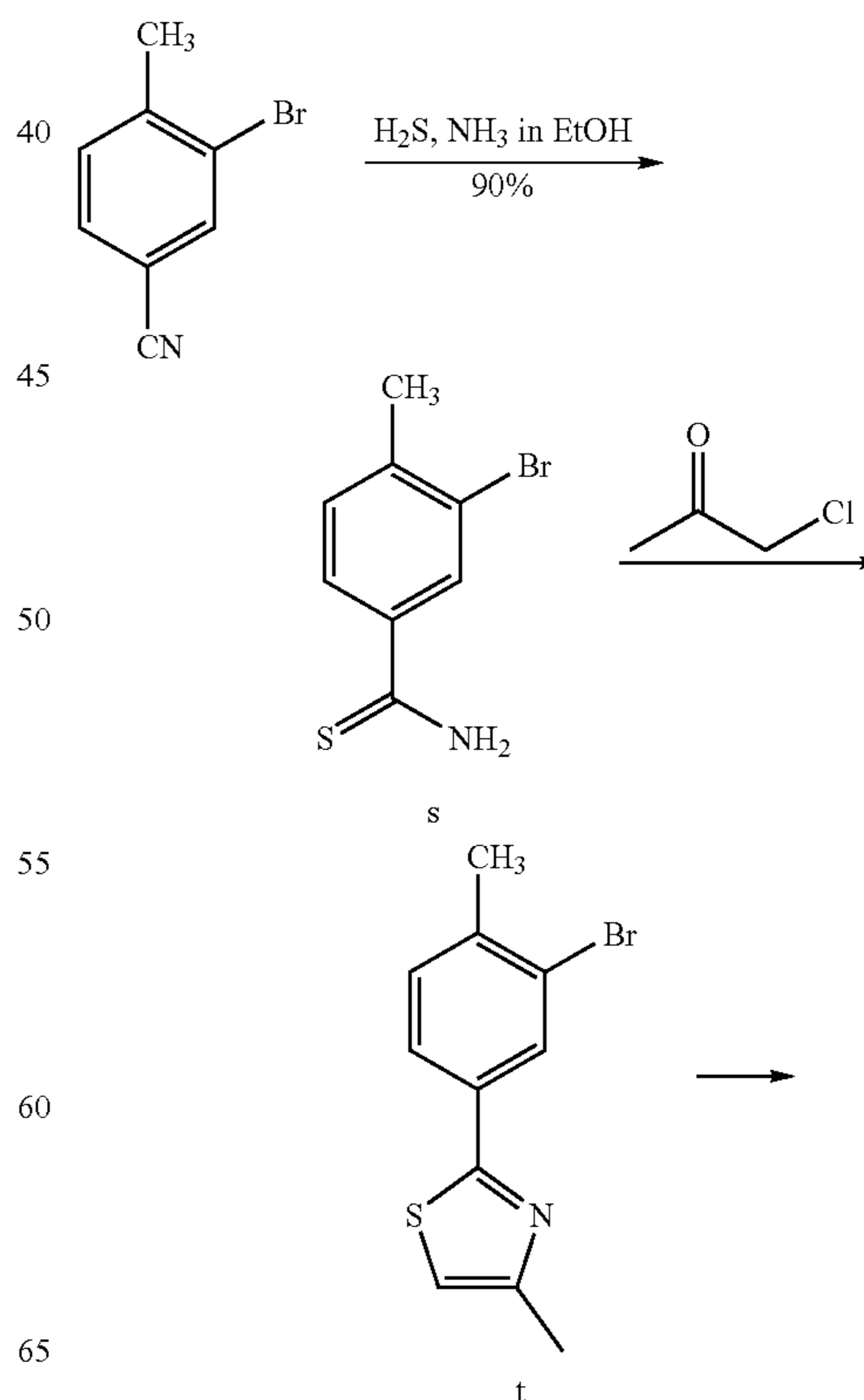
Scheme XIV
