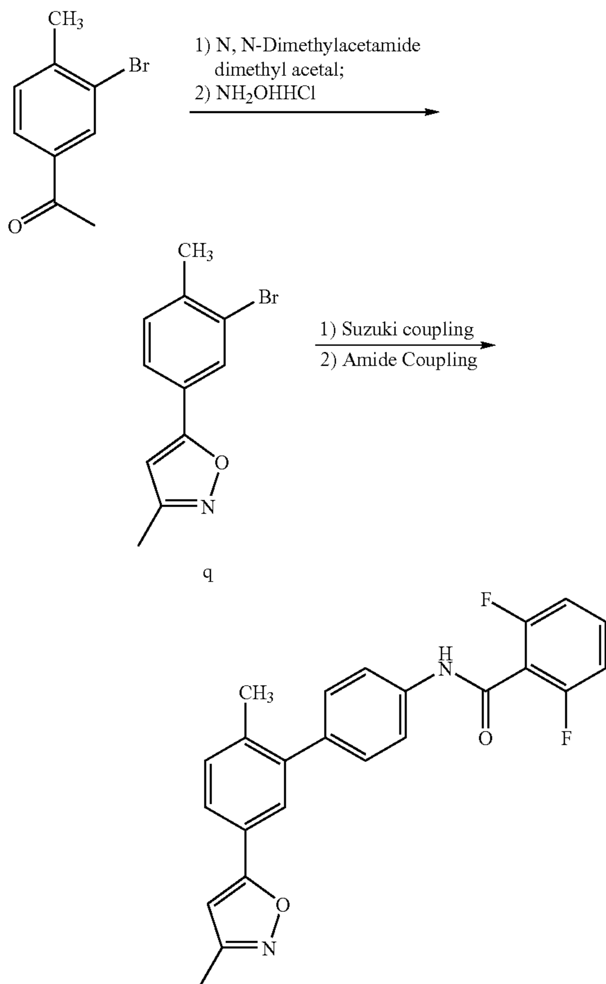
Compound 35
