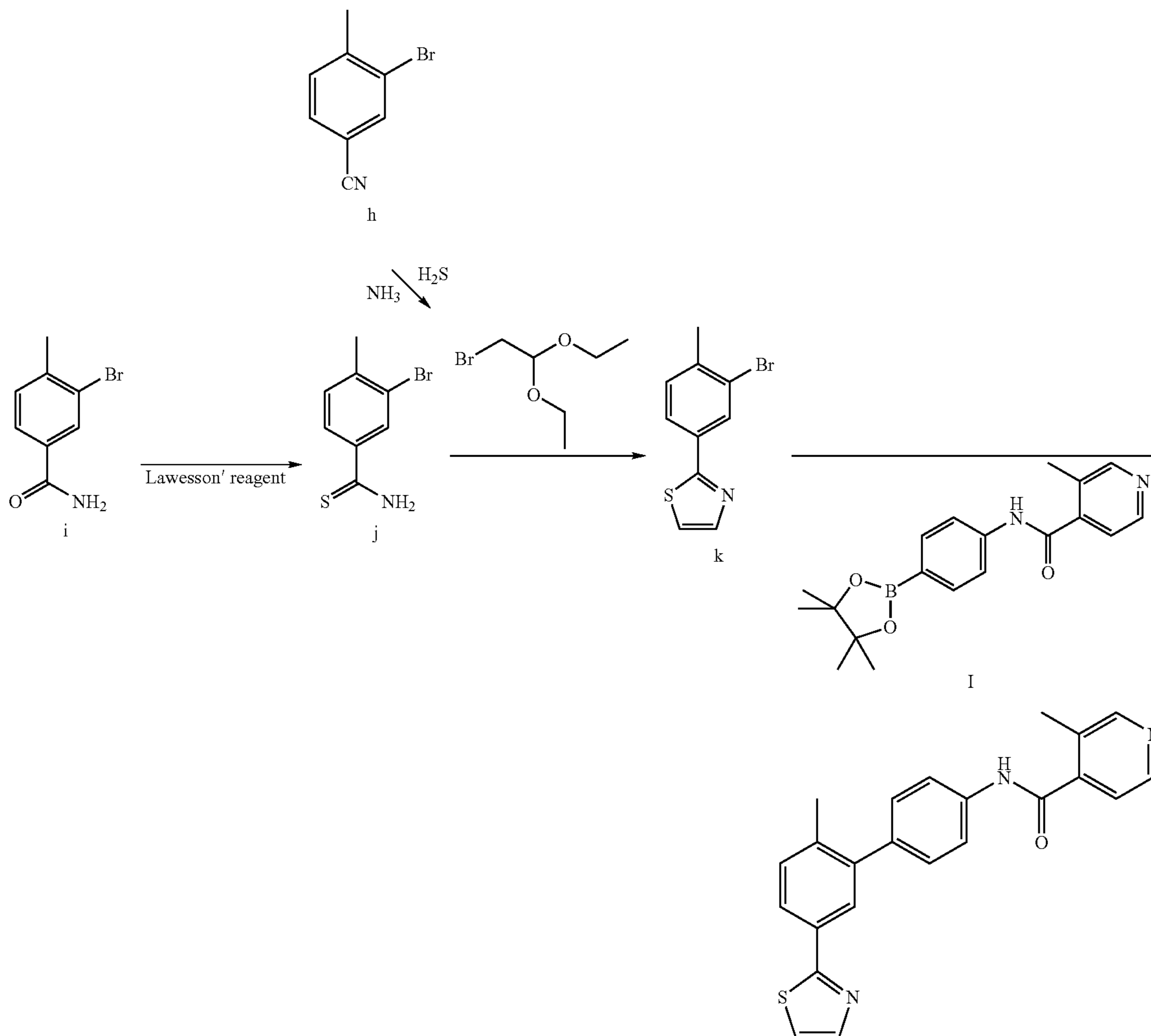
Compound 14
