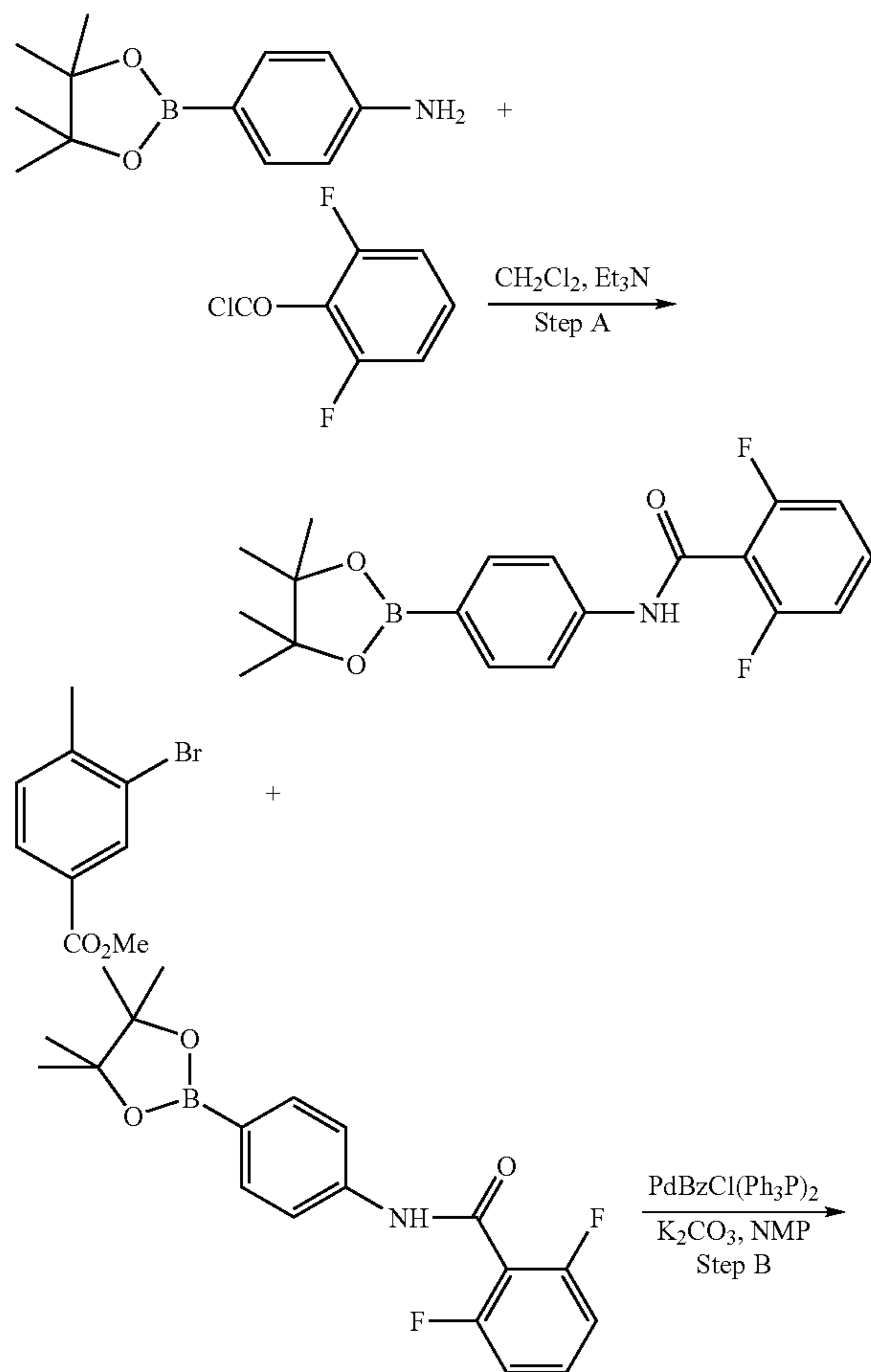
Scheme I
