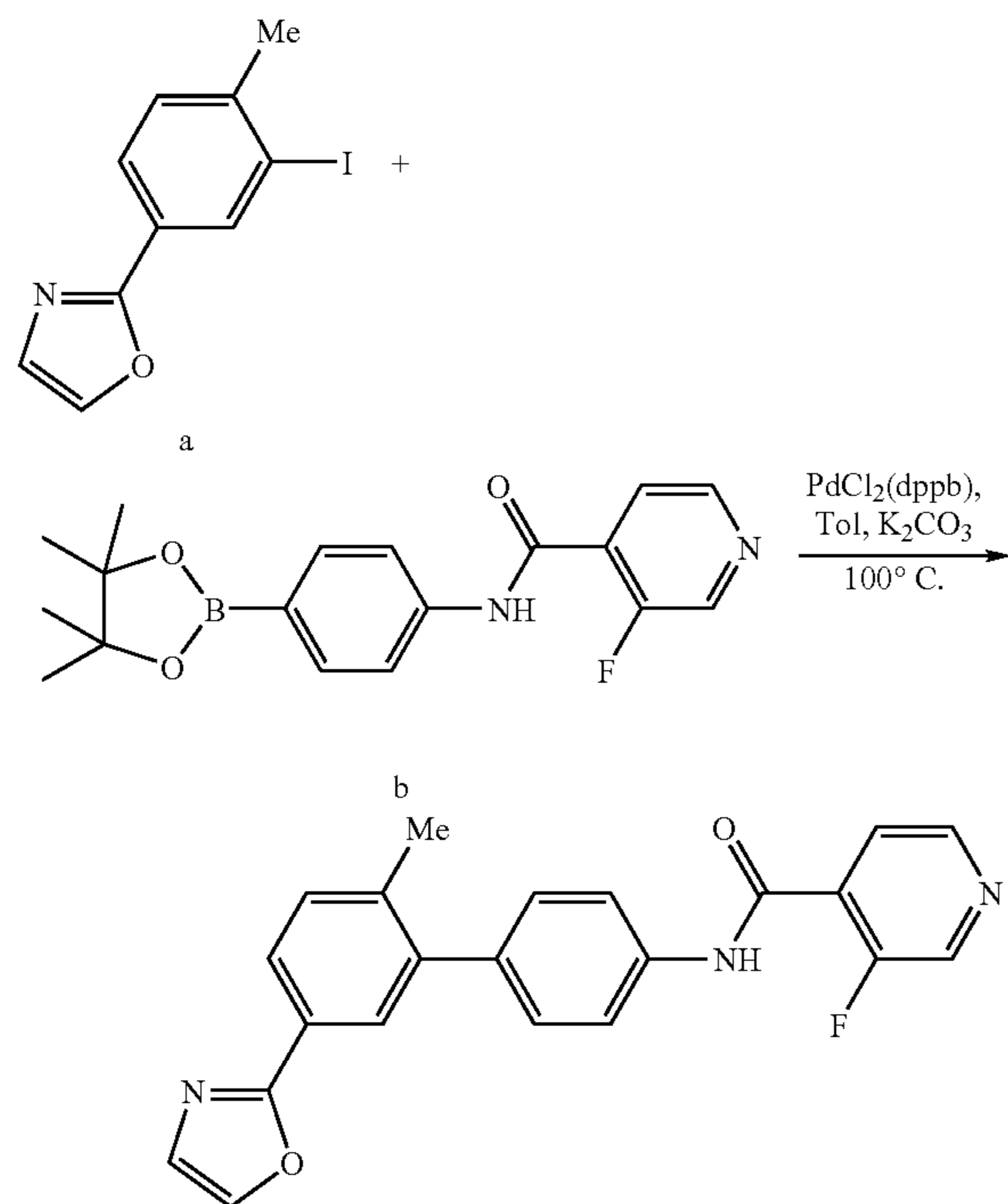
Compound 10
