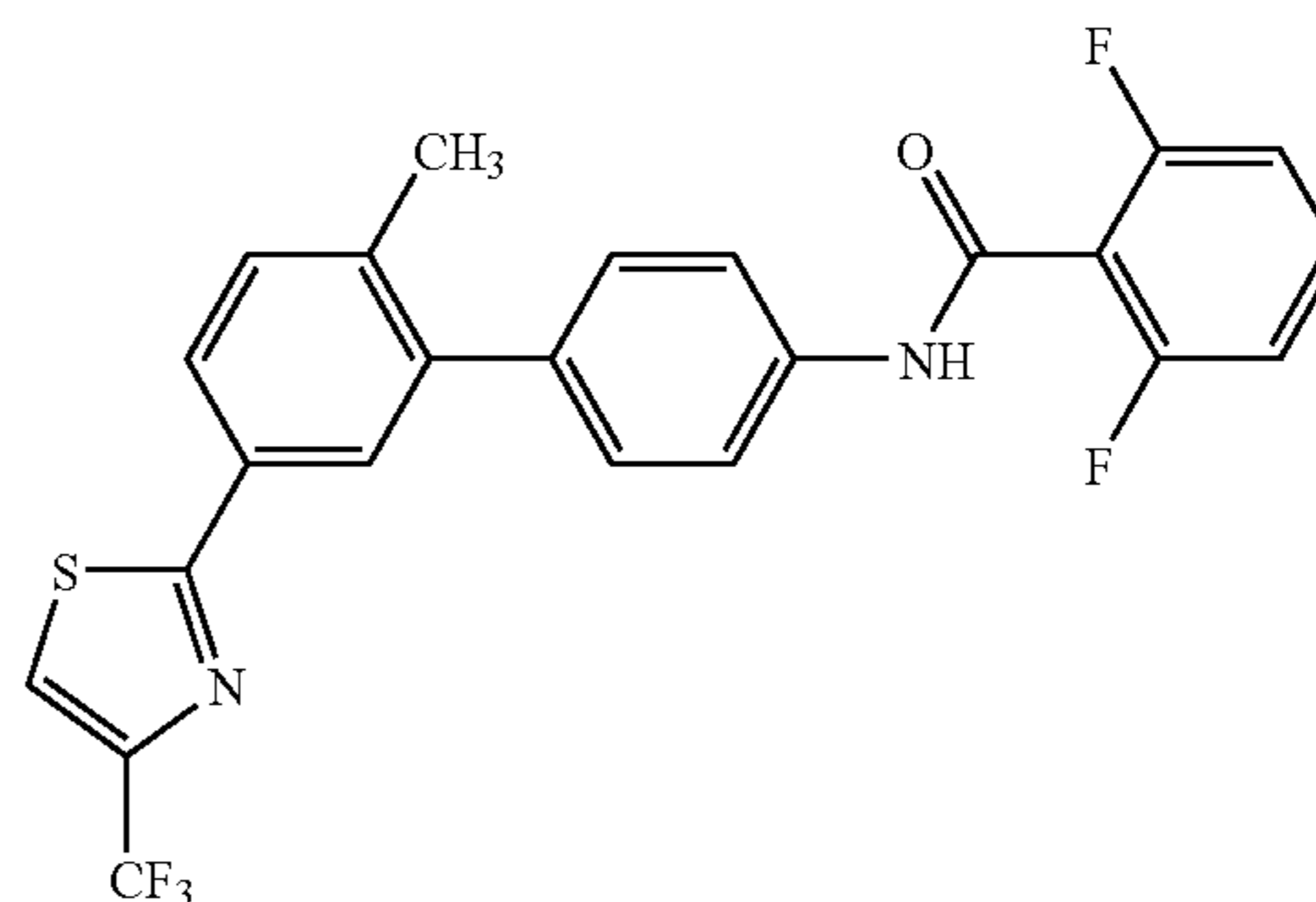
Compound 39
