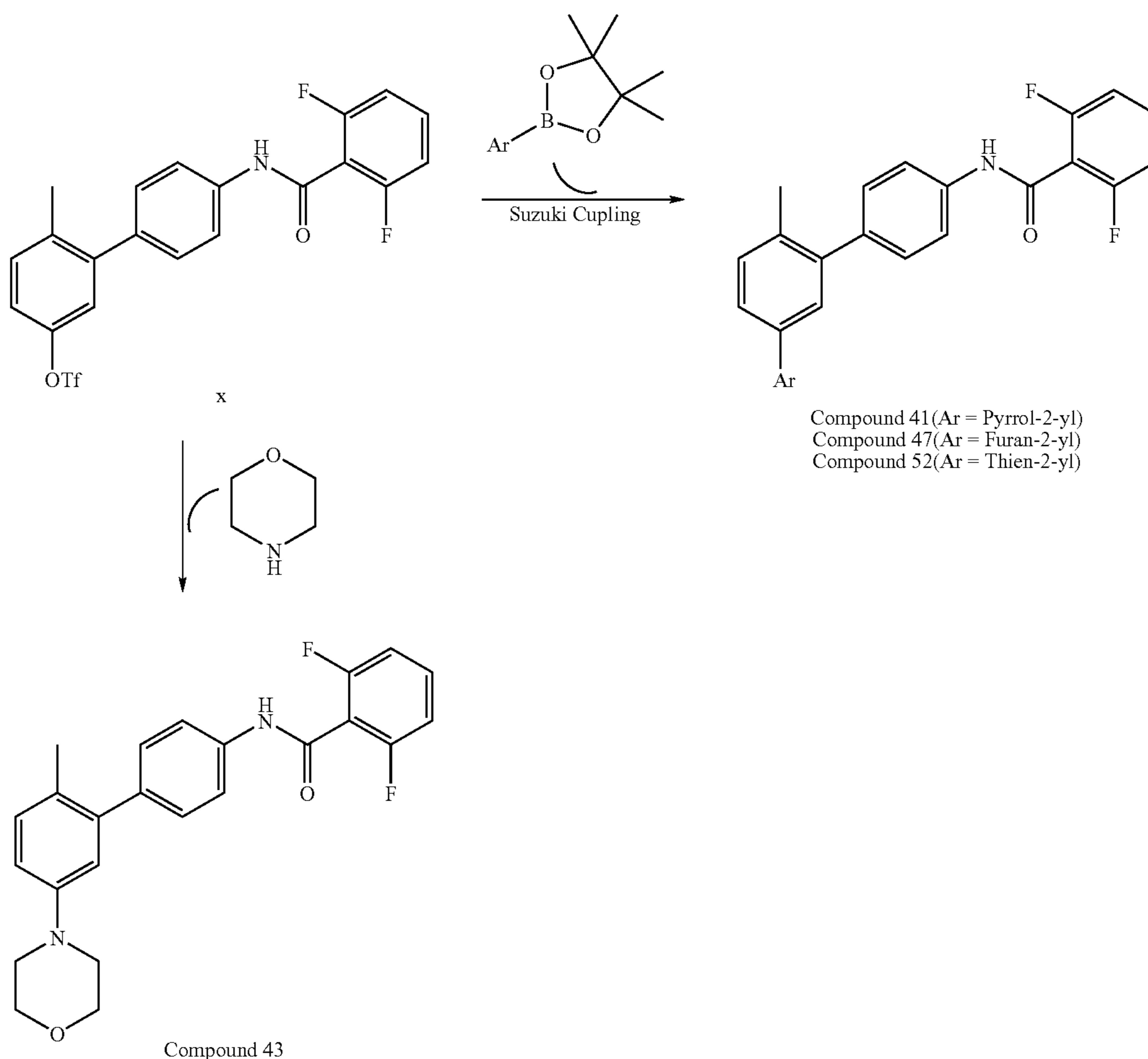
Scheme XVIII
