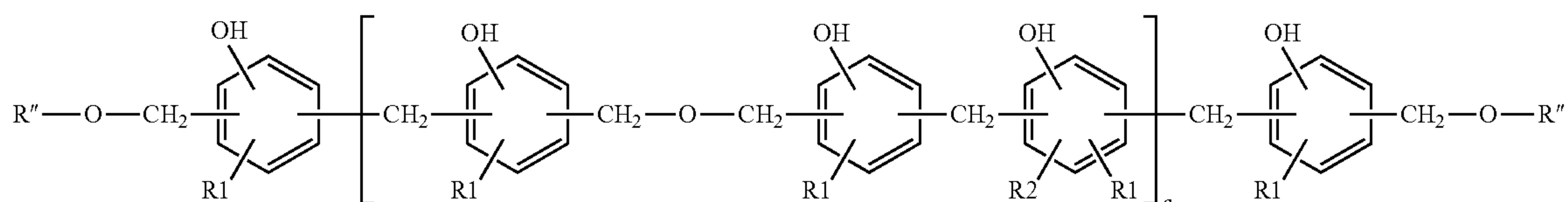
Formula (VIII)
