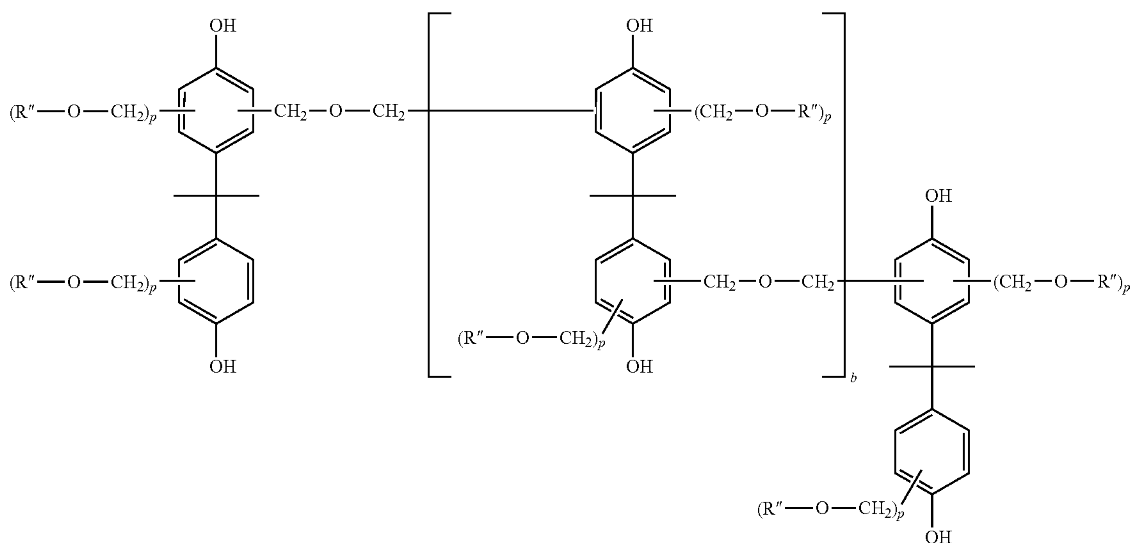
Formula (IXa)
