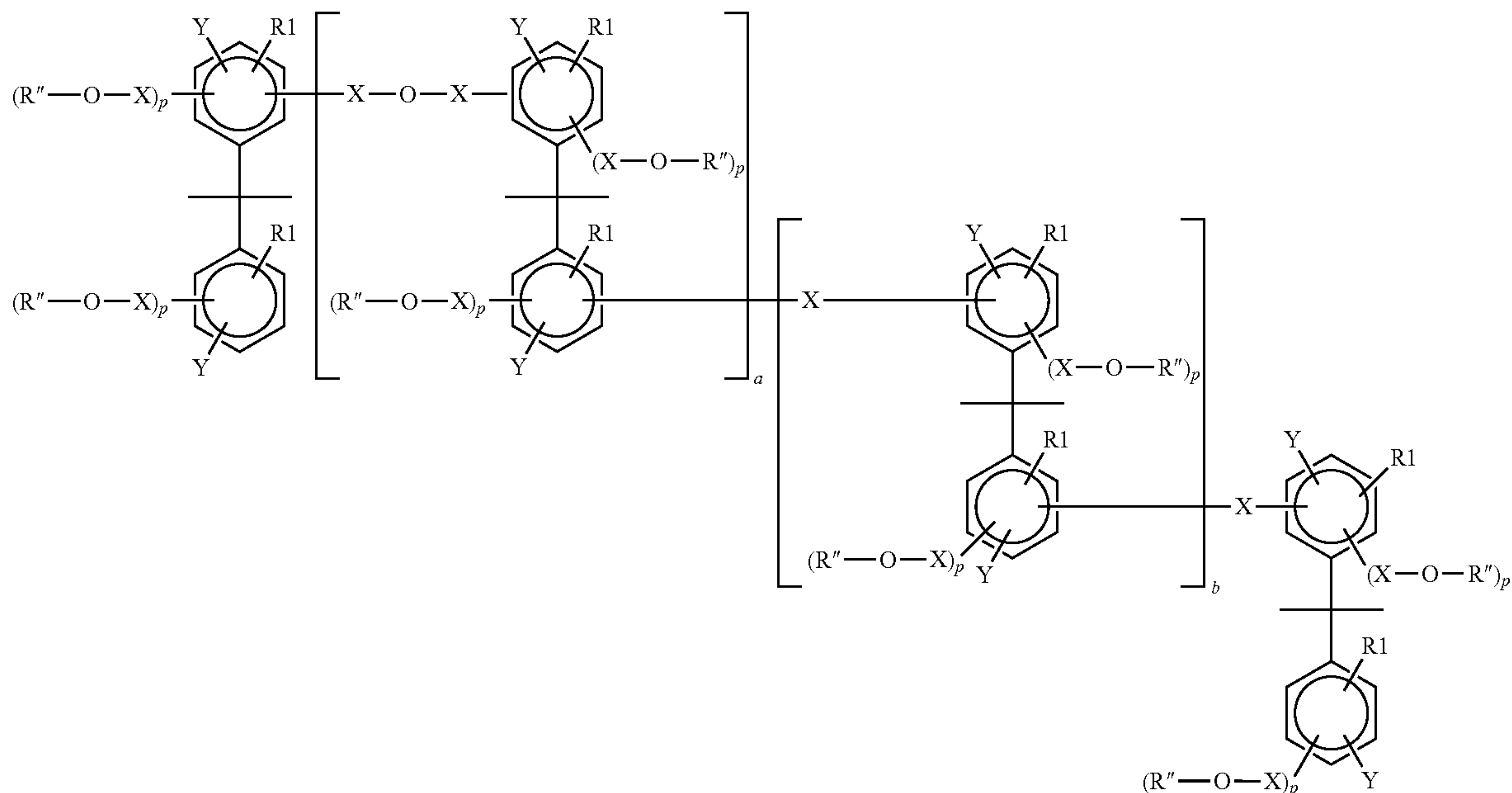
Formula (VI)
