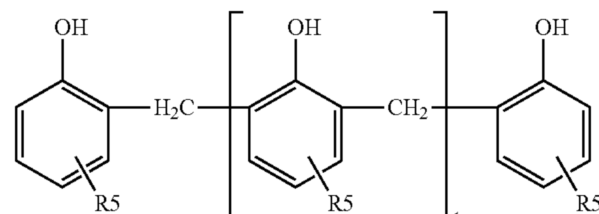
Formula (XXXII)
