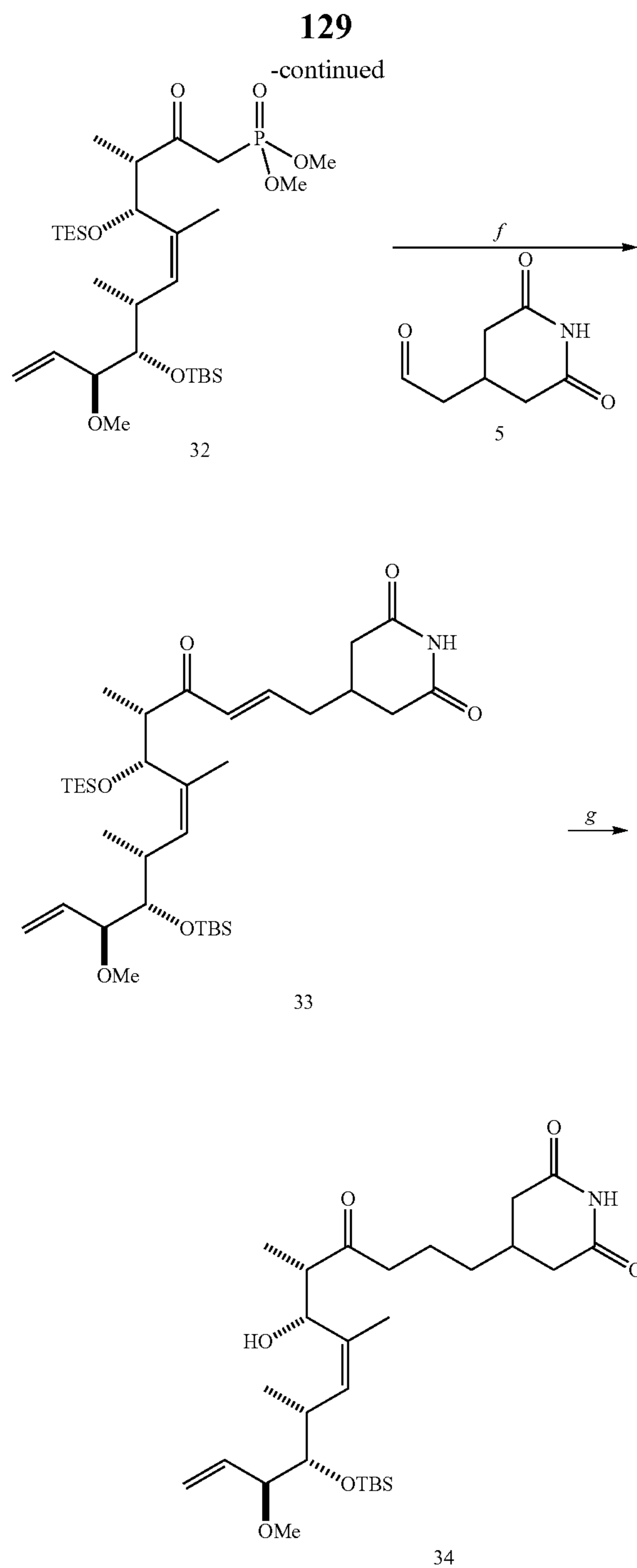
Scheme 22. Acylation of Alcohol 34 by a Modified Yamaguchi Procedure a
