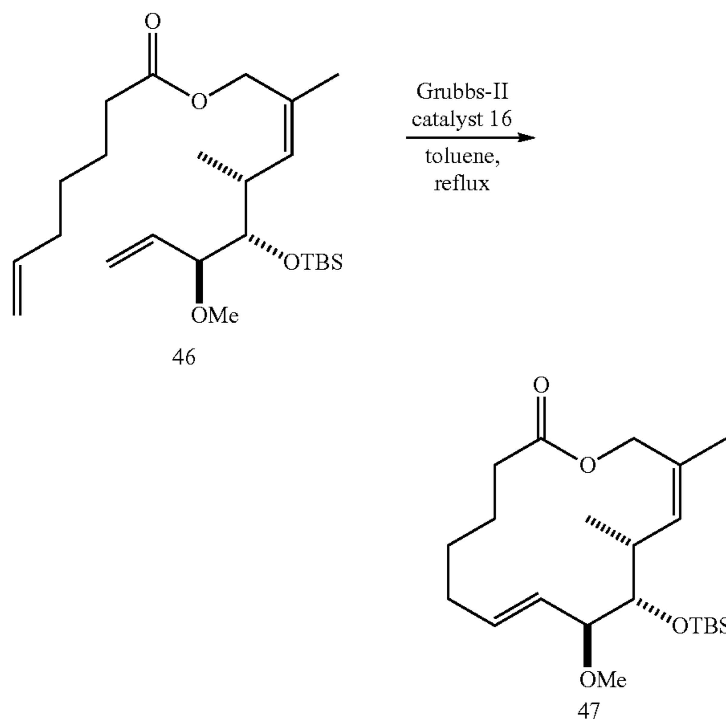
Scheme 26. Optimization of the RCM Conditions for Scale-Up Purposes
