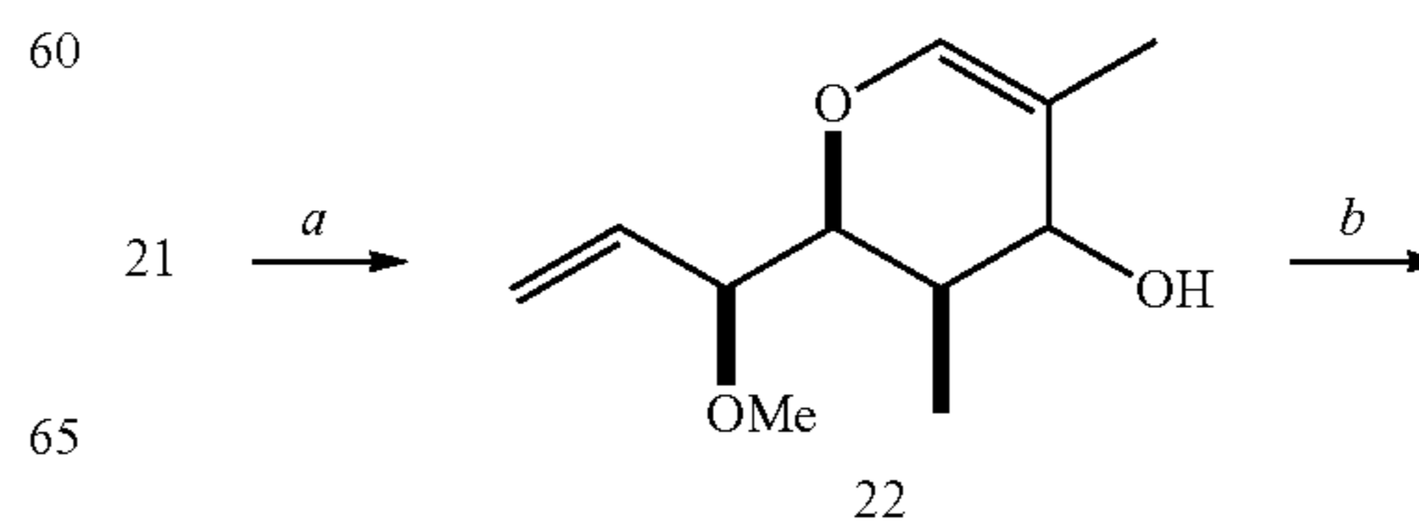
Scheme 20. Synthesis of Intermediate 26 a
