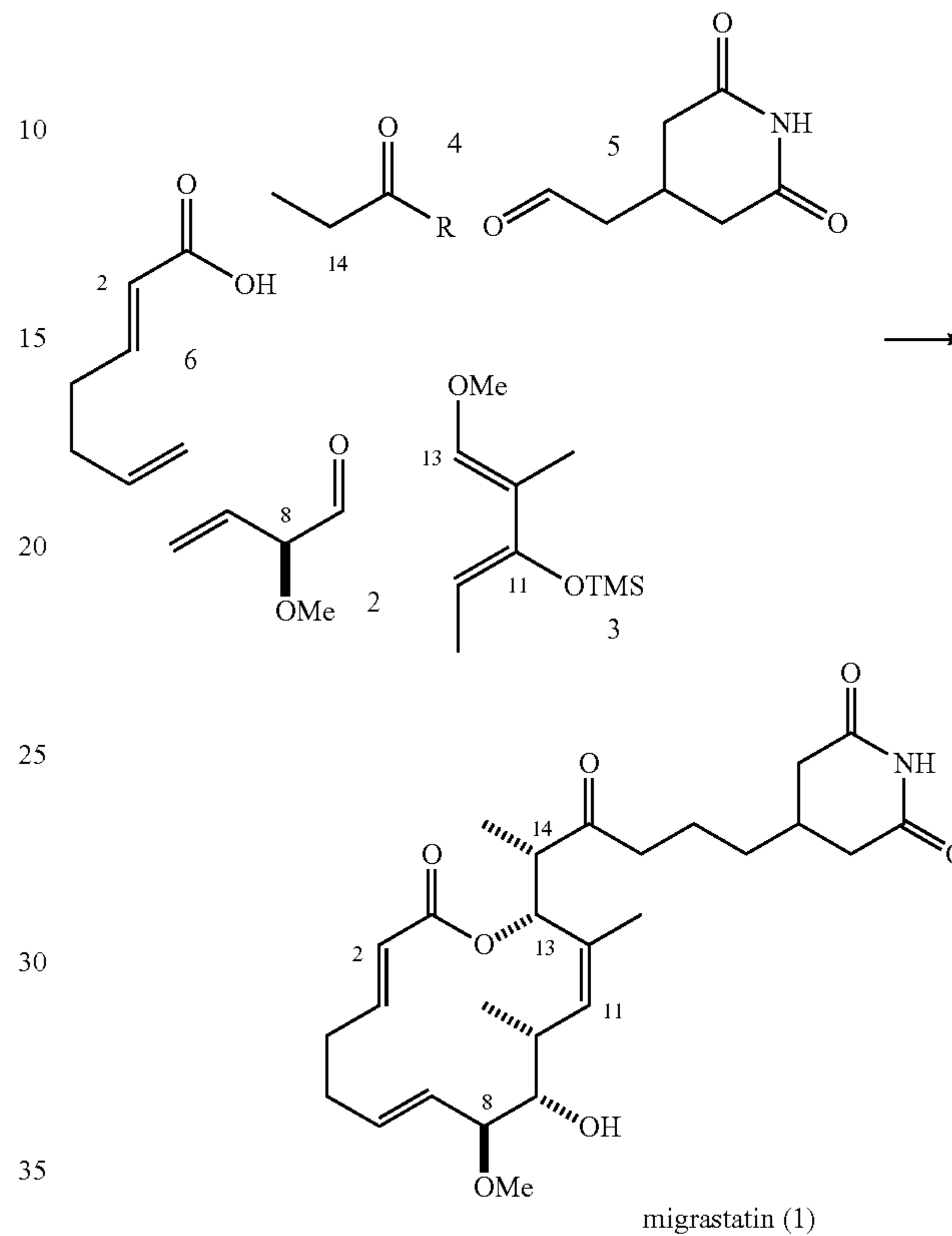
Scheme 17. Exemplary Strategy for the Assembly of Migrastatin
