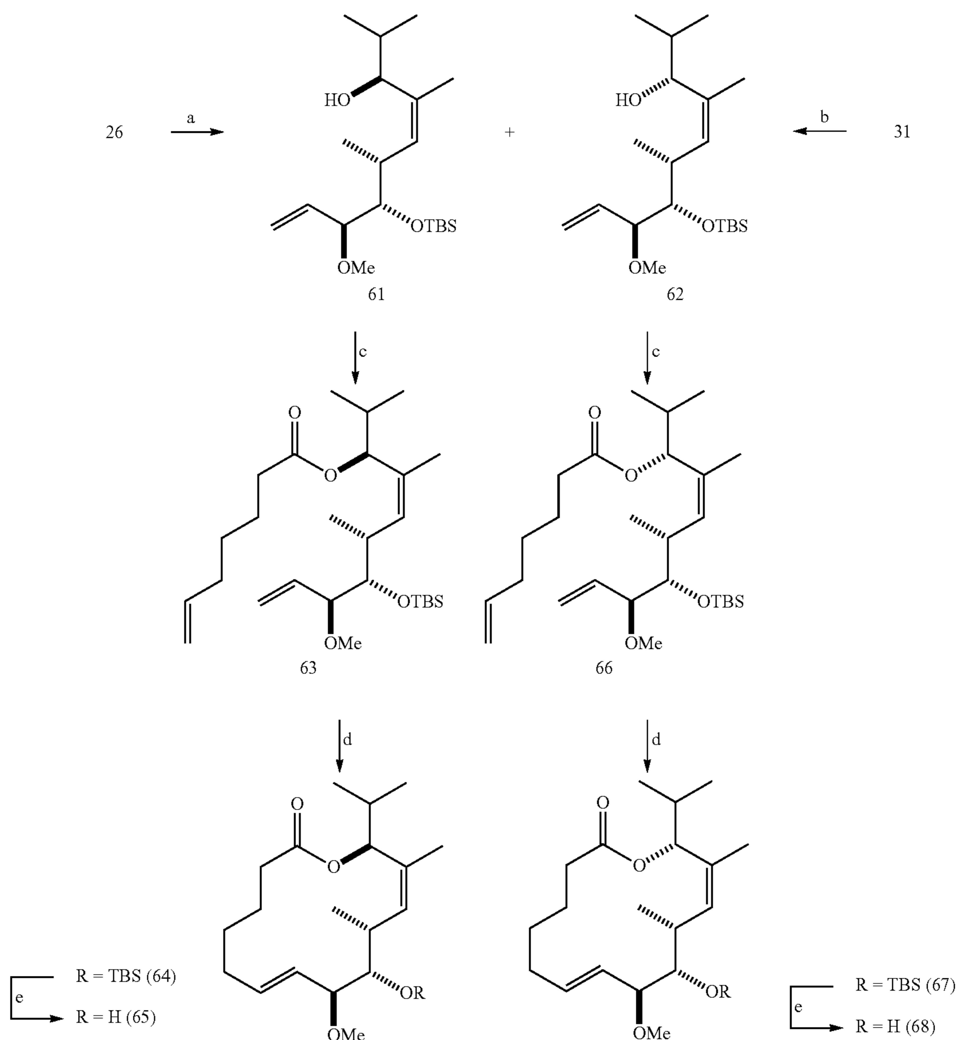
Scheme 29. Synthesis of the Diastereomeric Isopropyl Macrolactones 65 and 68 a
