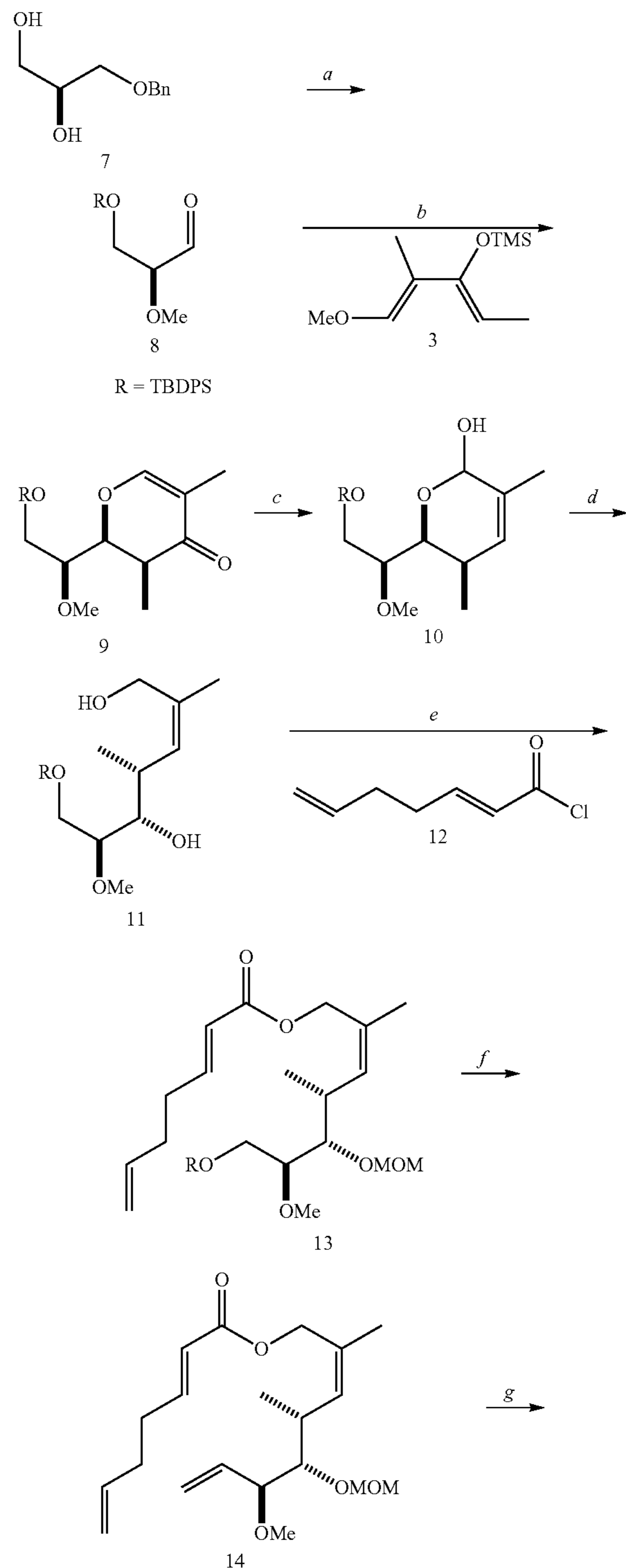
Scheme 18. A Model Study: Synthesis of the Migrastatin Core 15 a
