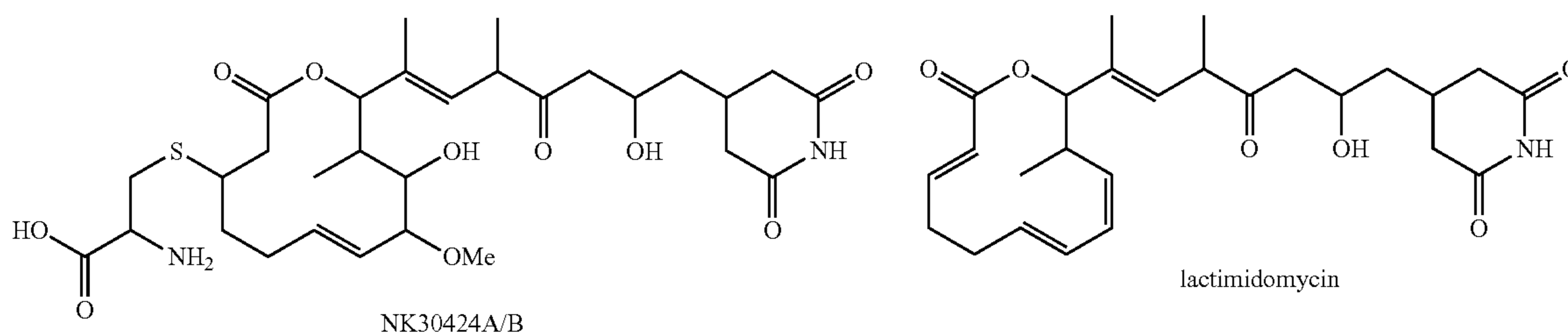
Scheme 16. Structure of Migrastatin and Related Natural Products
