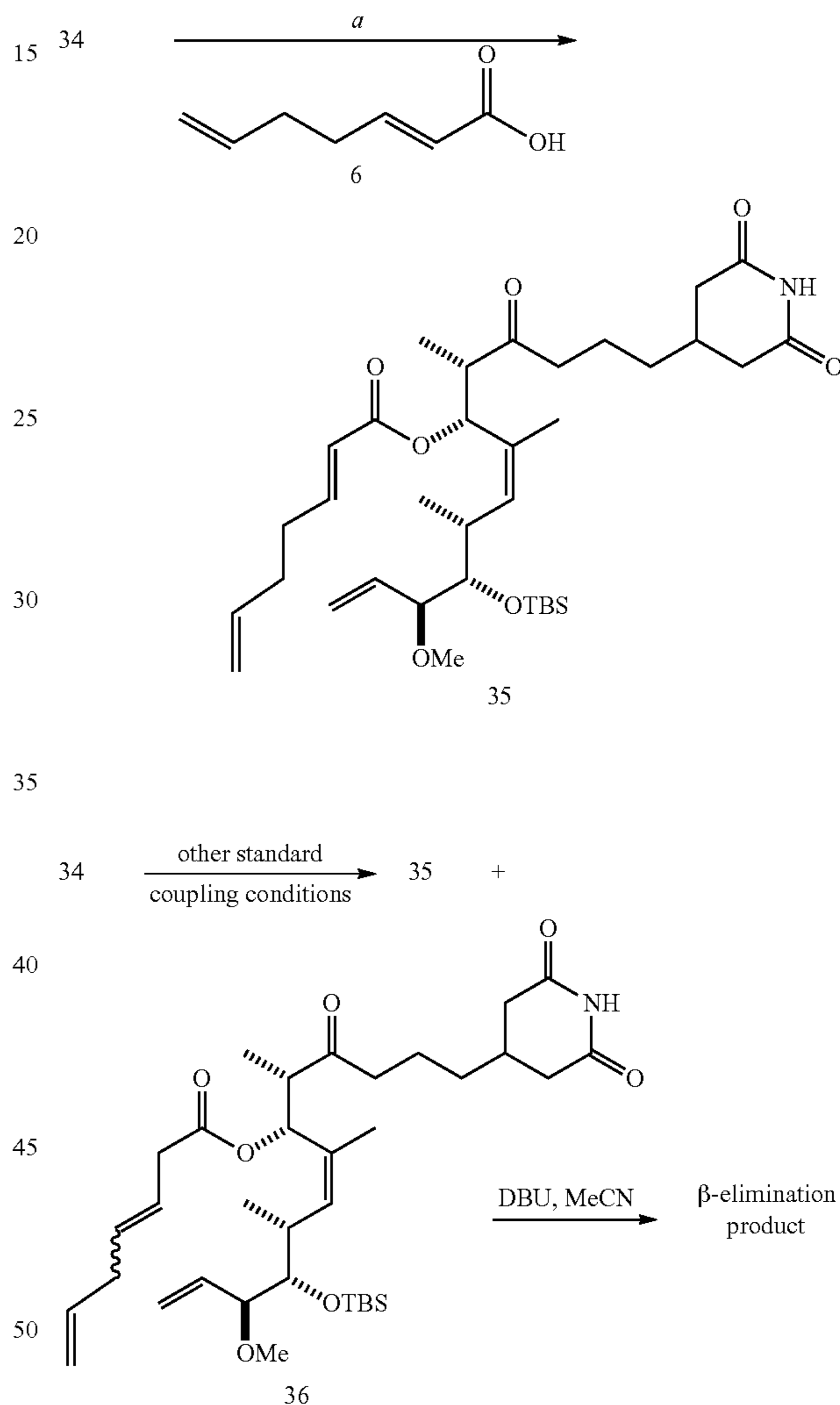
Scheme 22. Acylation of Alcohol 34 by a Modified Yamaguchi Procedure a
