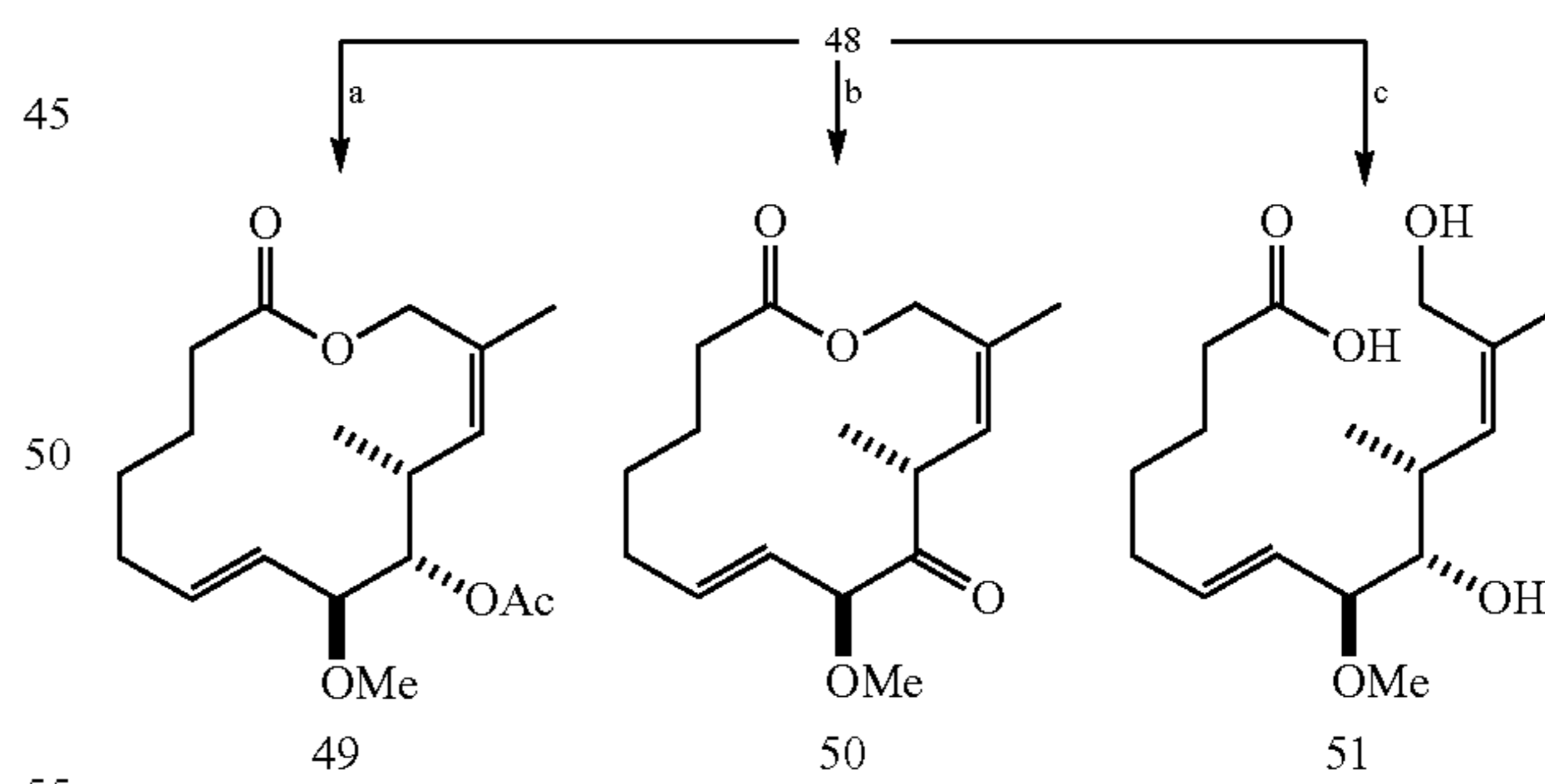
Scheme 27. Modification of Macrolactone 48 at the C9 position and Hydrolysis of 48 a
