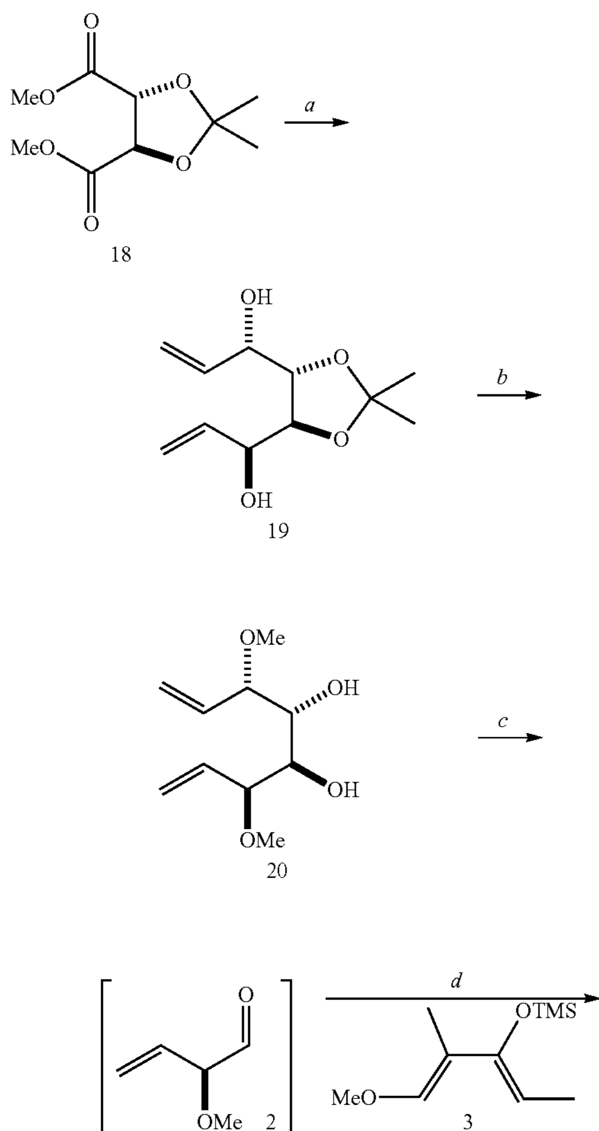
Scheme 19. Synthesis of Dihydropyrone 21 by a Cyclocondensation (LACDAC) a
