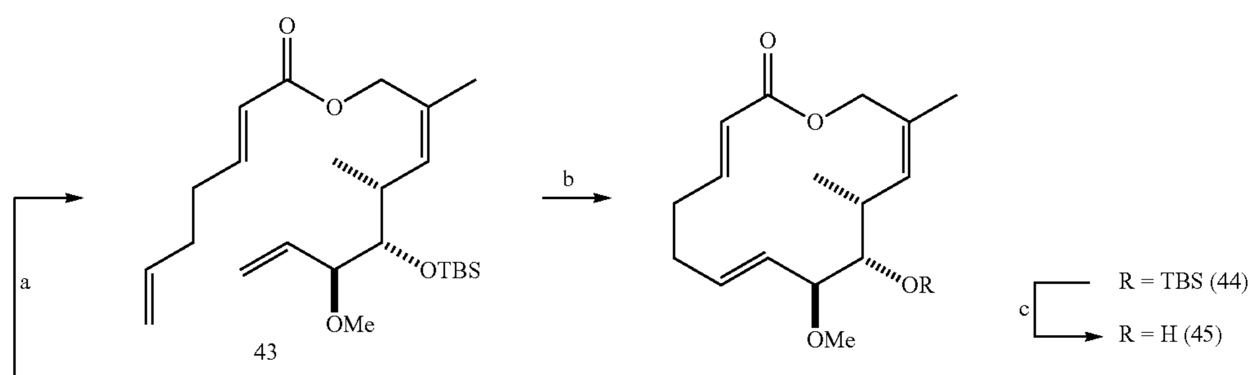
Scheme 25. Synthesis of Migrastatin Core 45 and Macrolactone 48 a
