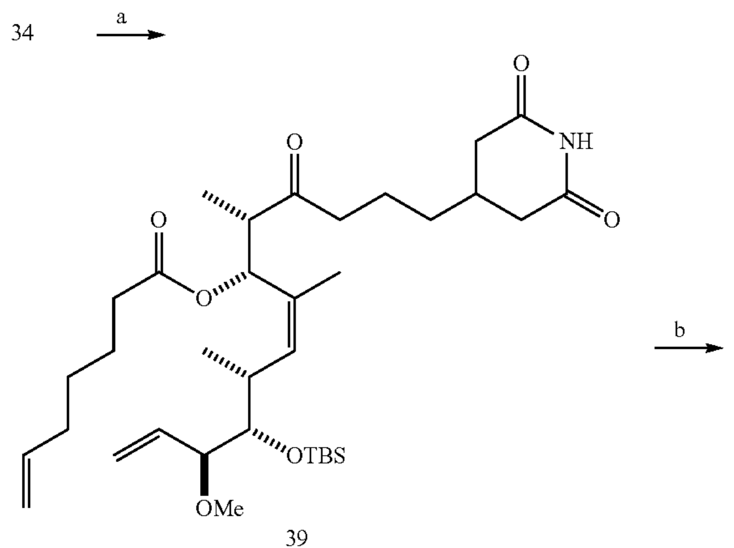
Scheme 24. Preparation of Migrastatin Analogs 41 and 42a
