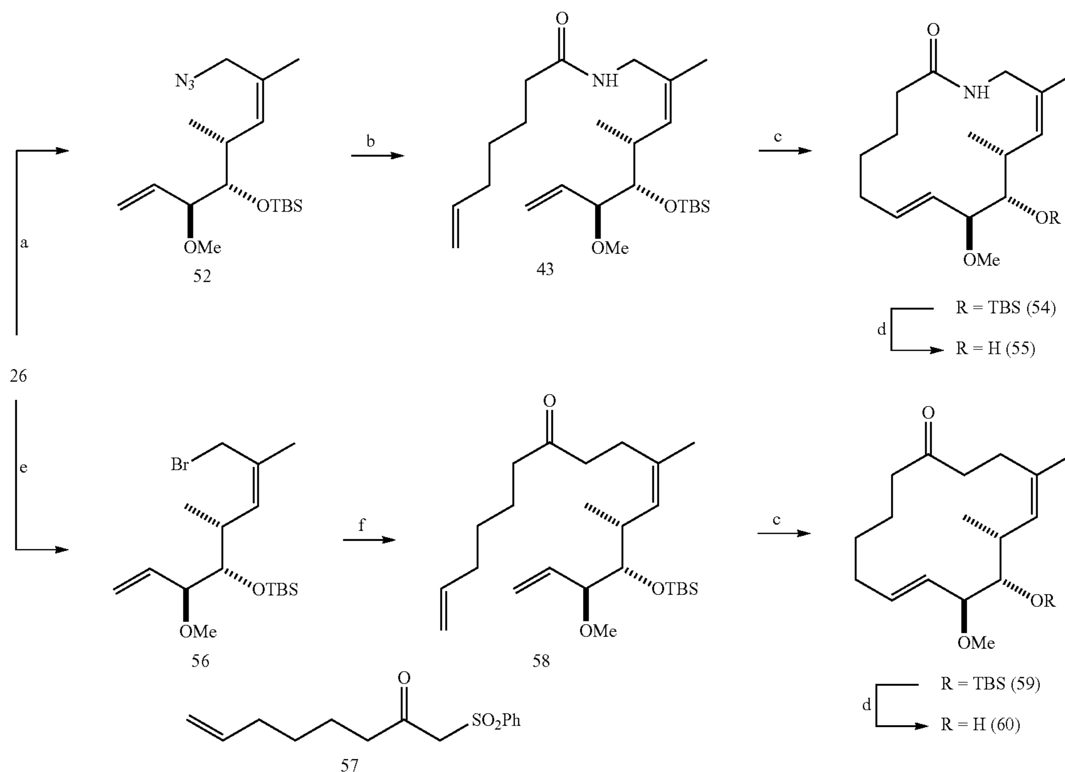
Scheme 28. Synthesis of Macrolactam 55 and Macroketone 60 a
