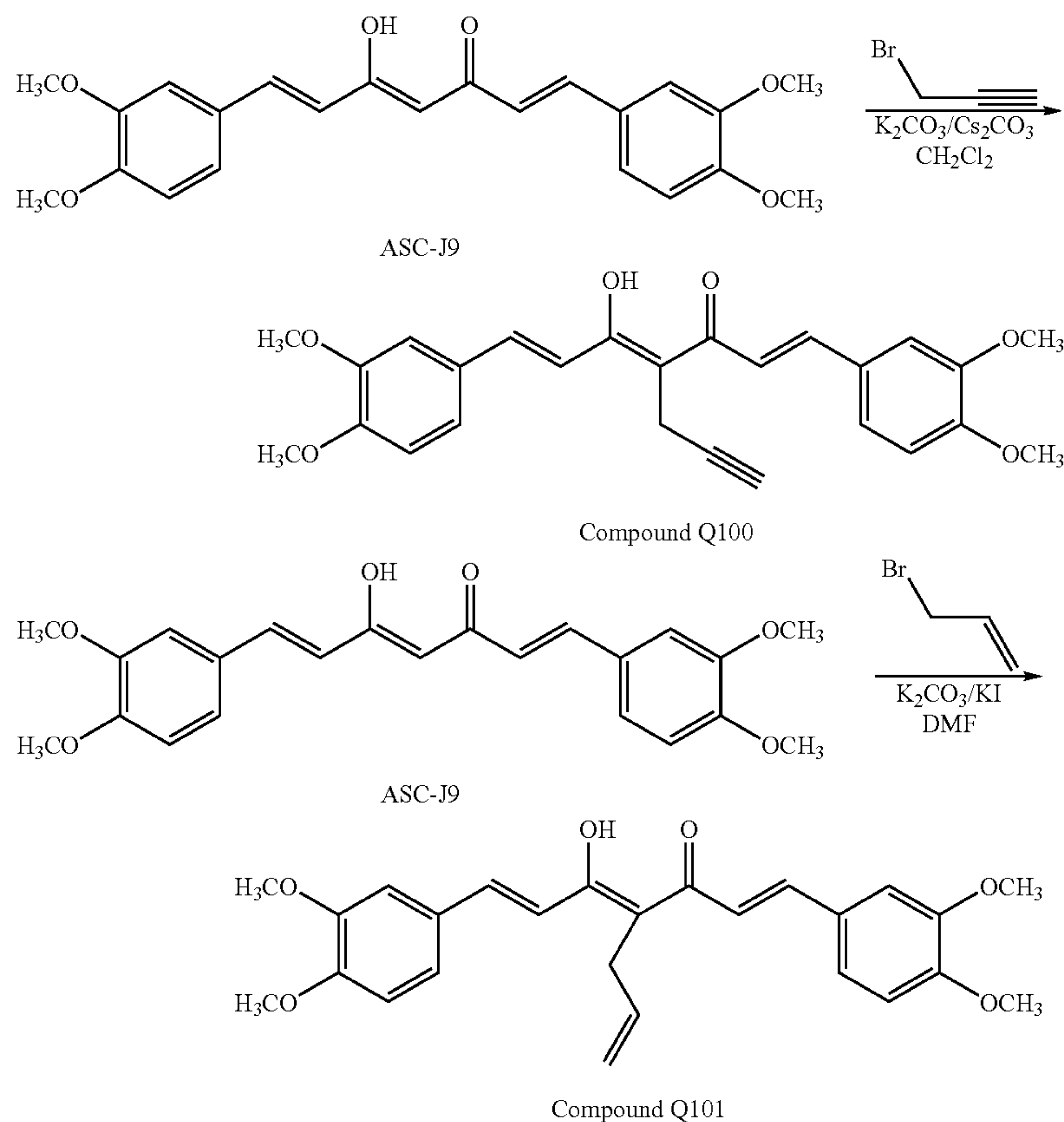
Scheme 8
