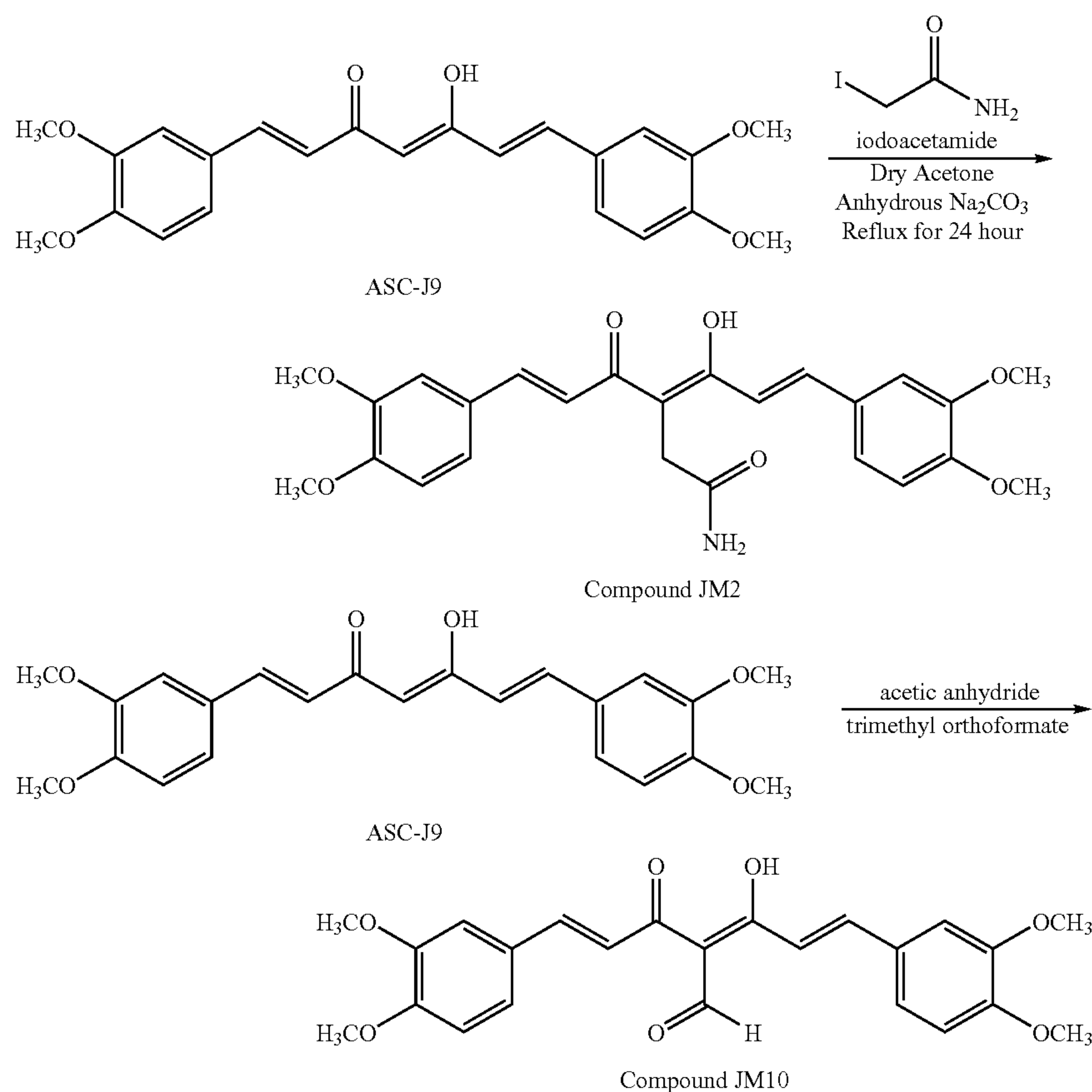
Scheme 7
