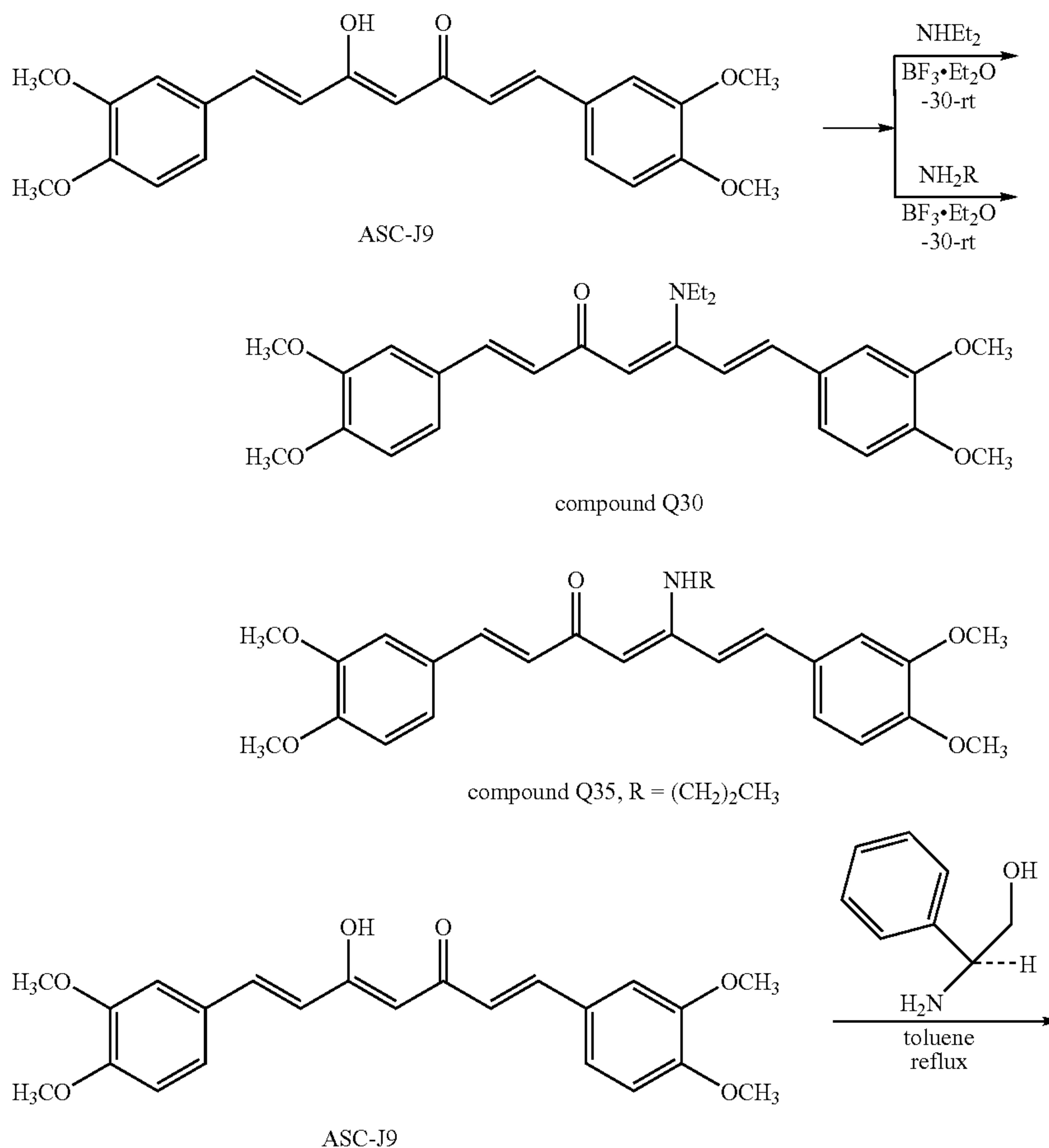
Scheme 5
