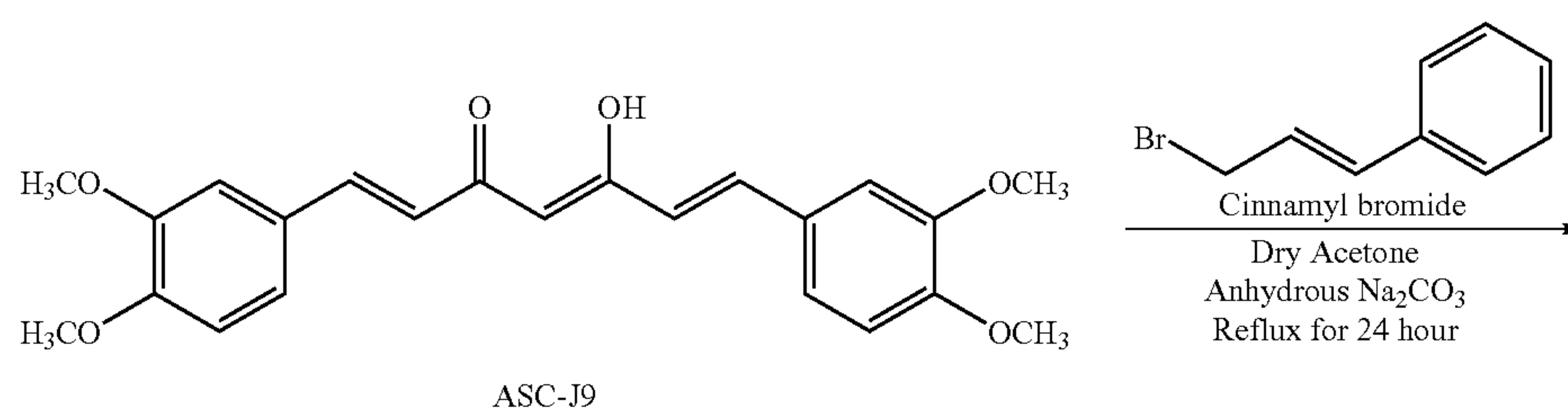
Scheme 9
