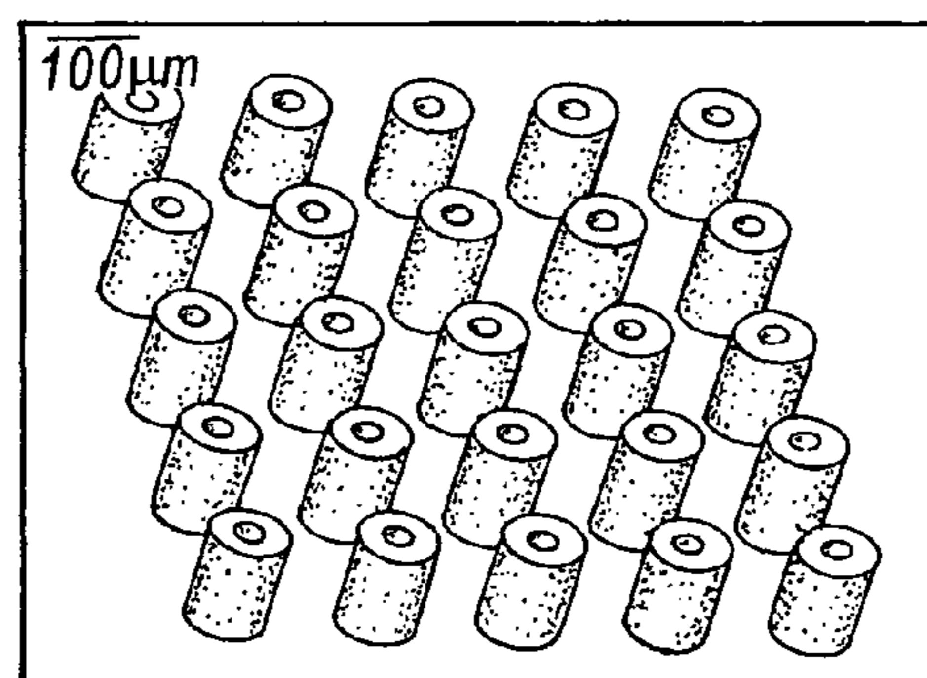
An array of silicon microneedles
