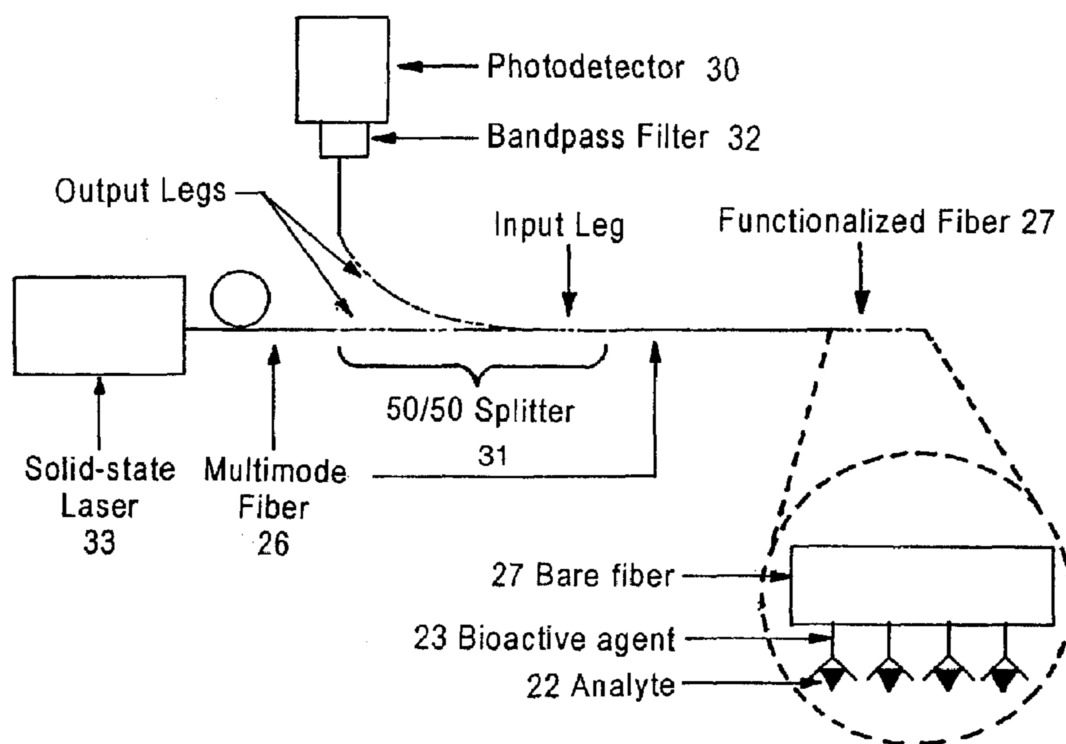
Schematic diagram of fiber optic TIRF sensor. Incoming laser light is directed through the output leg of a 50:50 fiber optic splitter onto the functionalized fiber. Emitted fluorescence couples back into the fiber and propagates towards the detector with little interference from the laser light.
