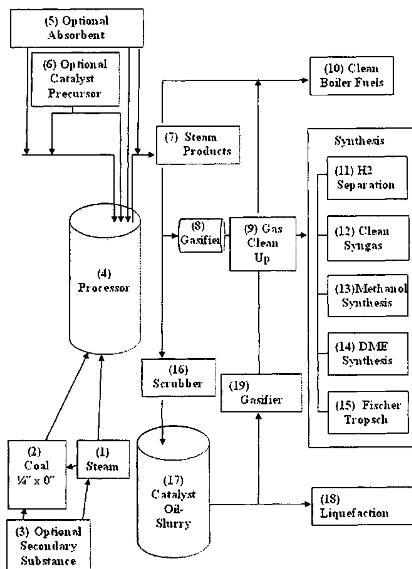
Overview of Products and Processes in Illustrative In-Line Configuration
