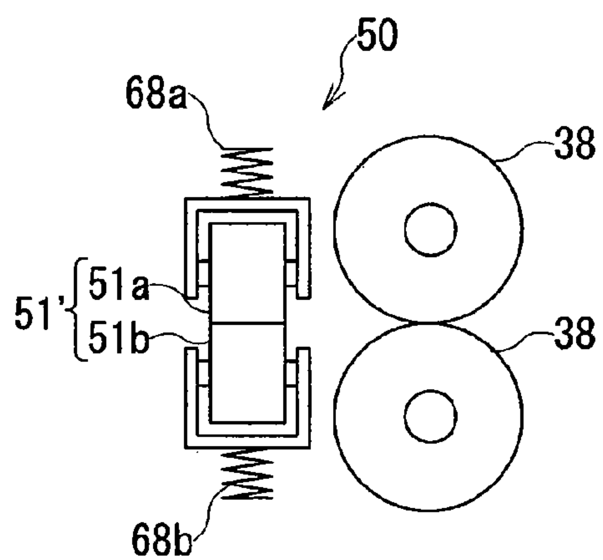
X-X' CROSS-SECTION
