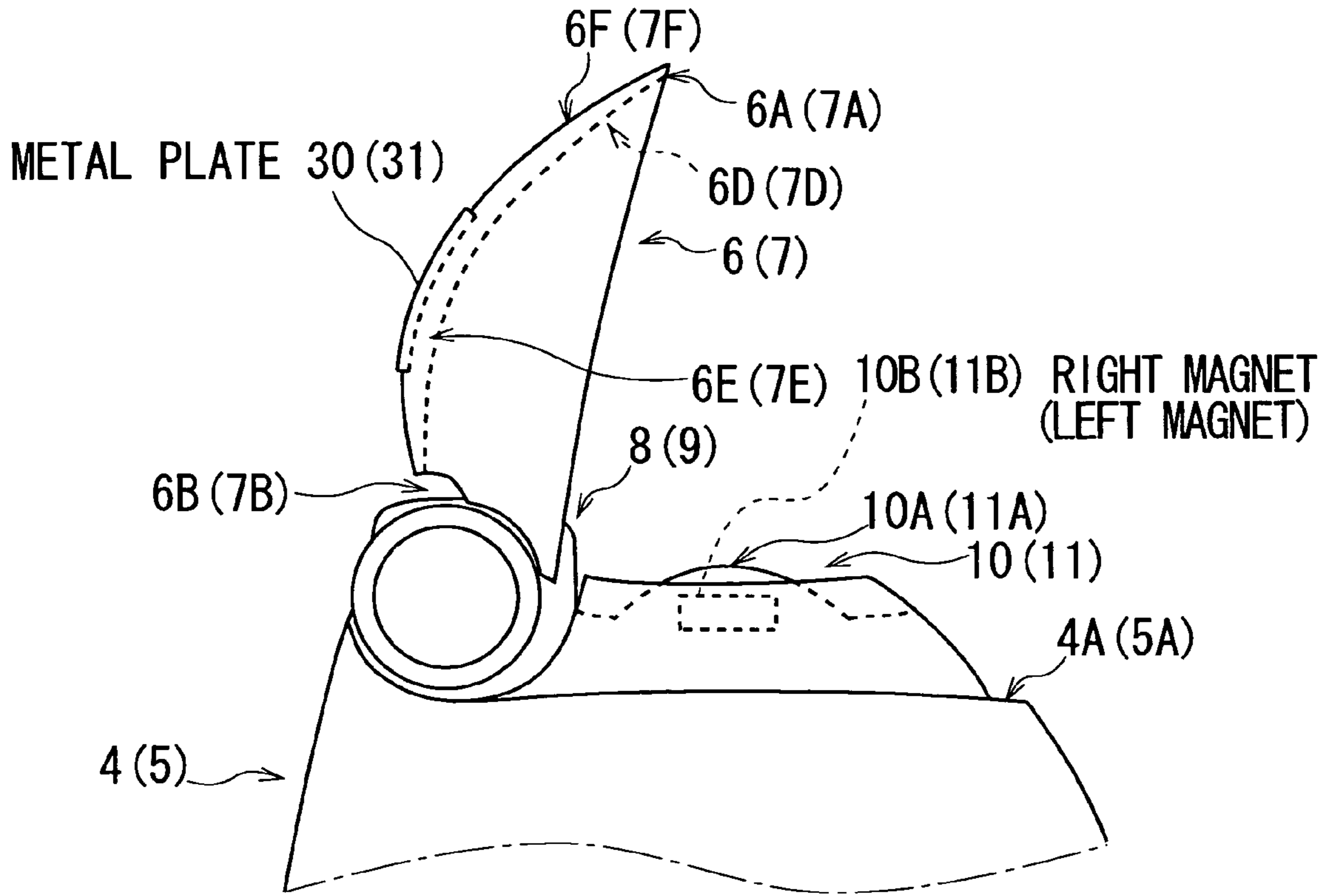
FIG.9A
