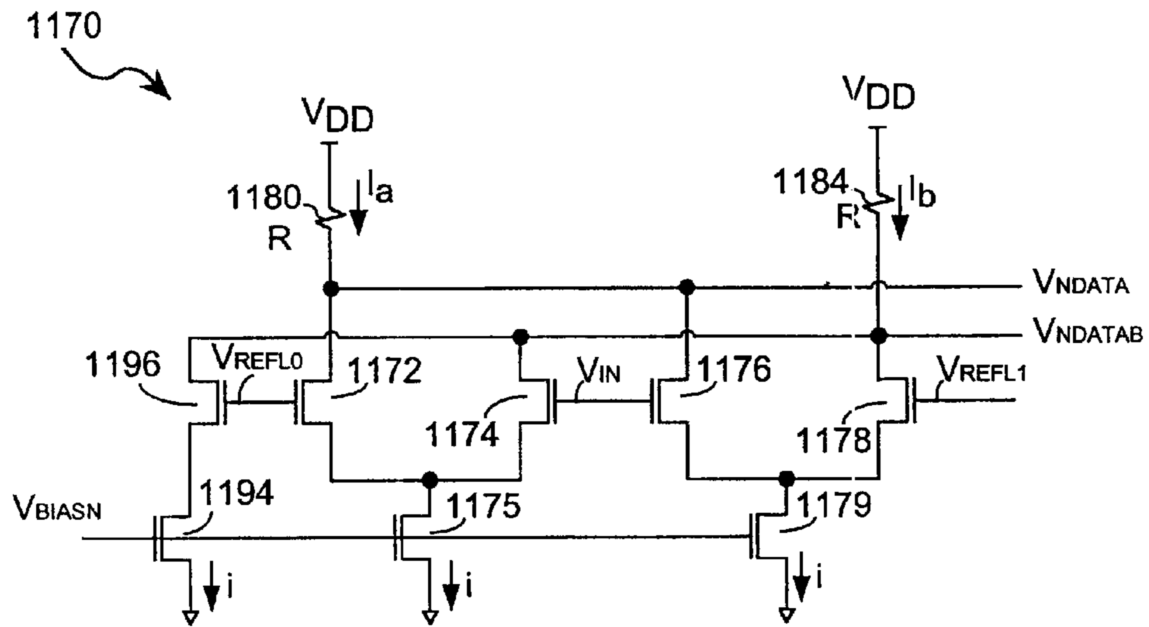
Multi-PAM Pre-Amplifier
