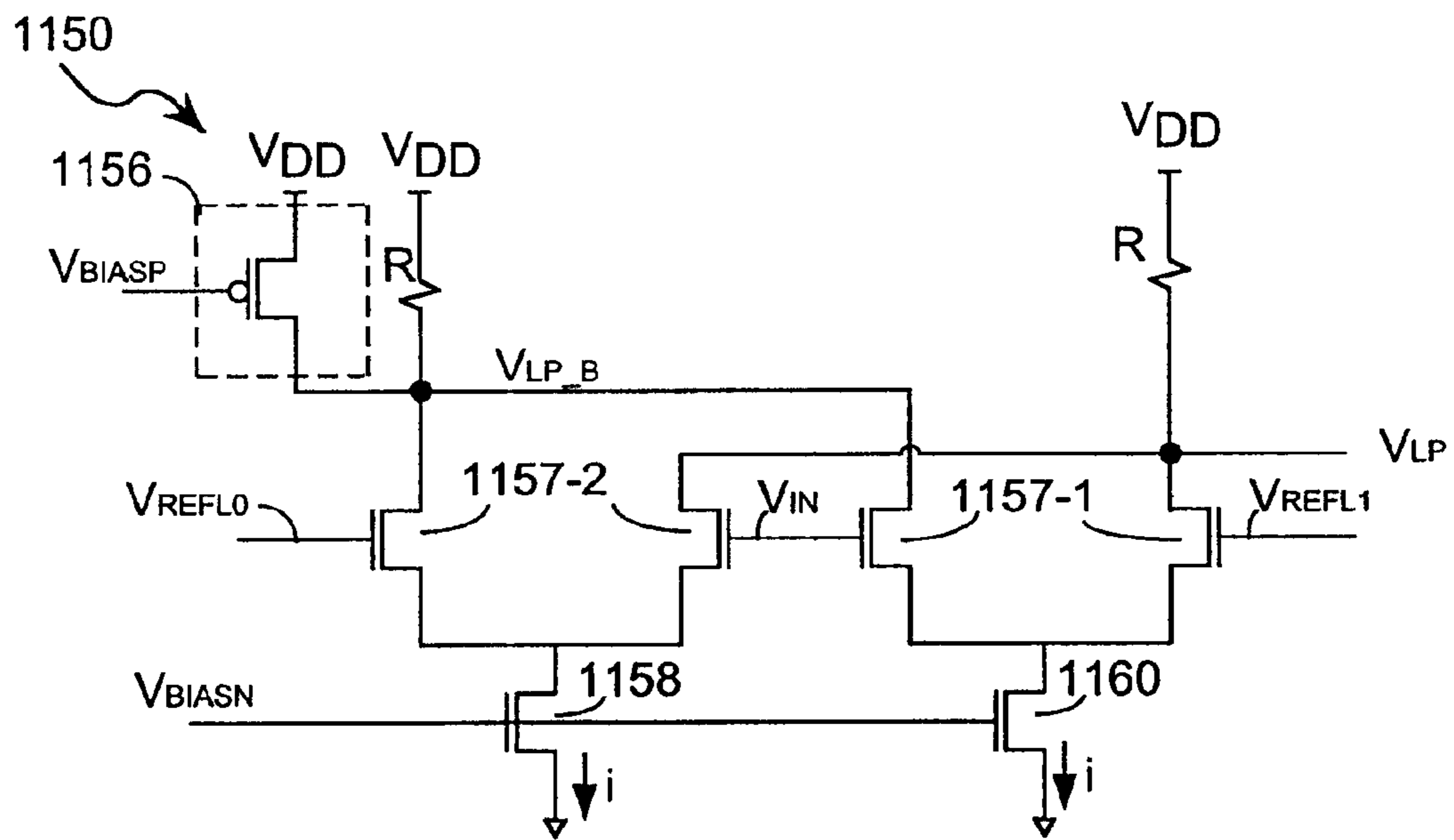
Multi-PAM Pre-Amplifier
