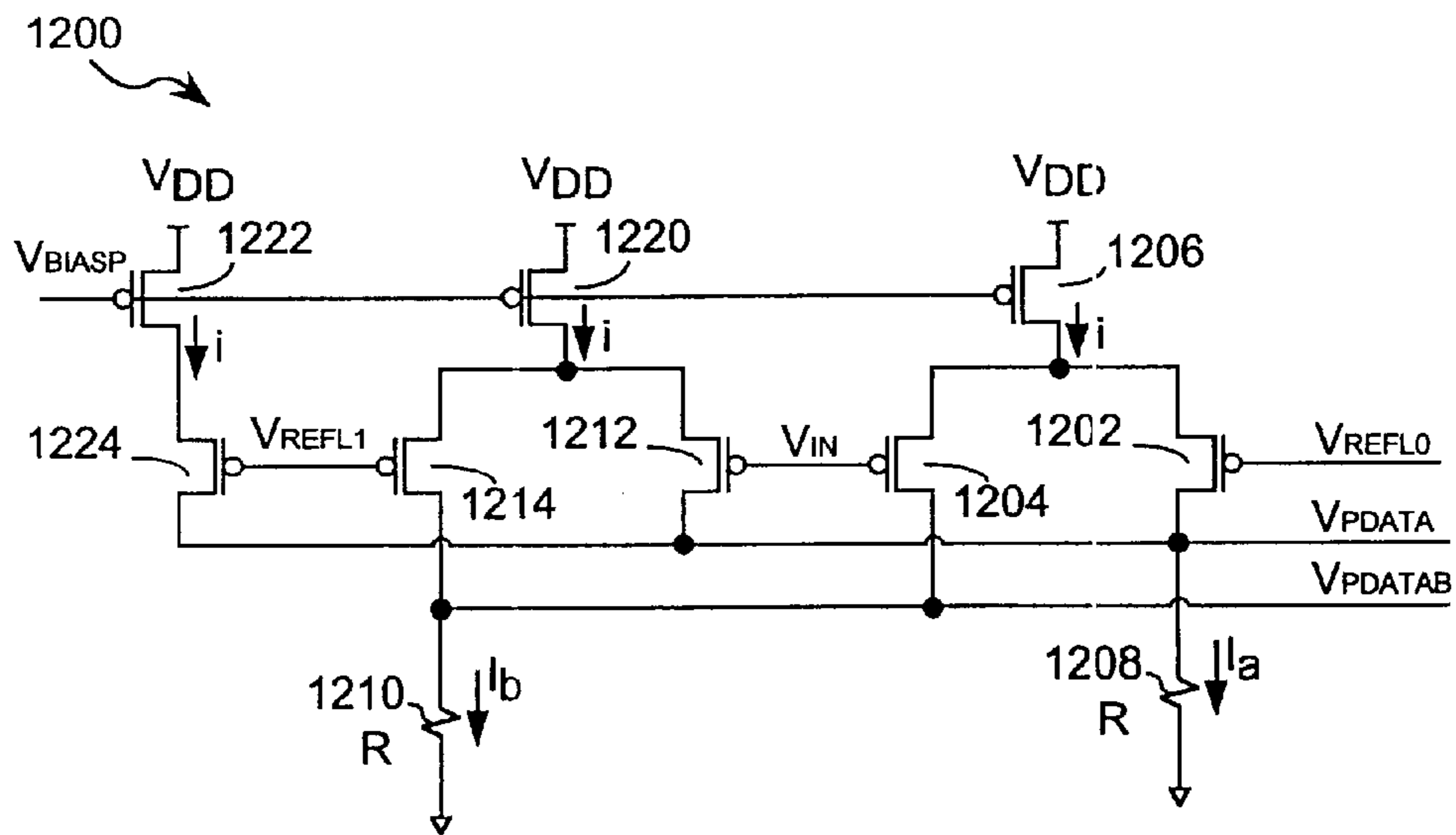
Multi-PAM Pre-Amplifier
