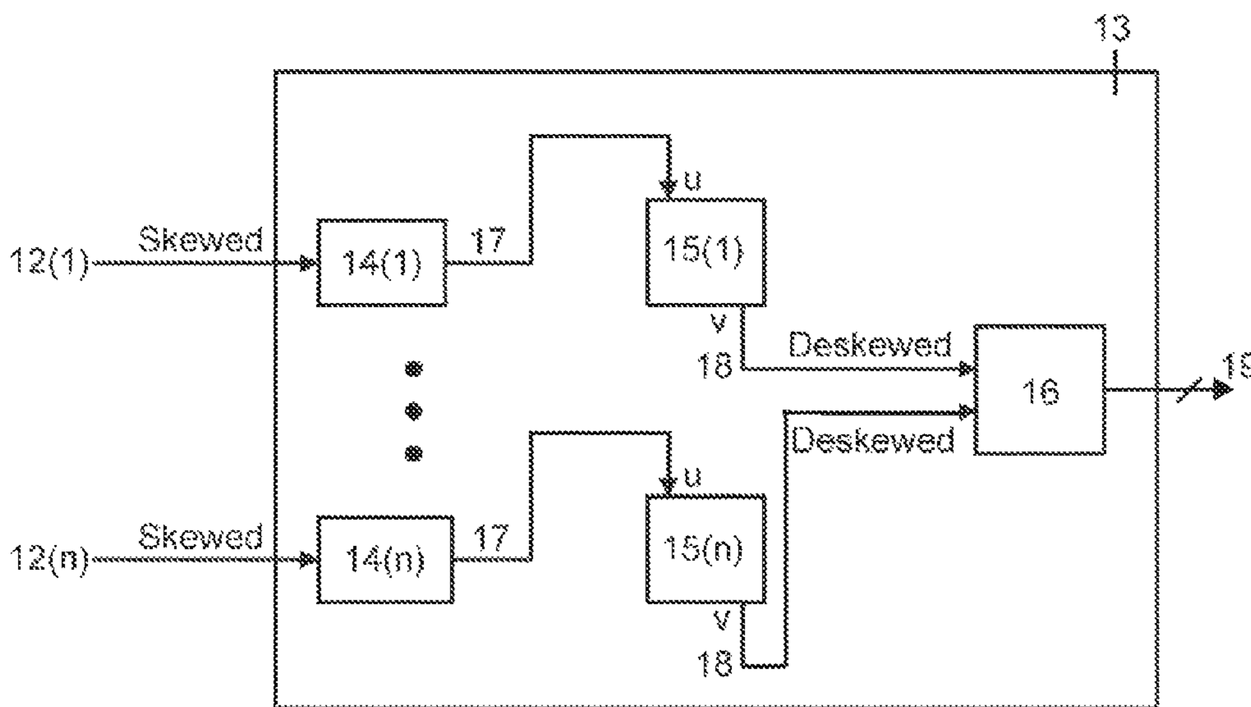
De-skewed Multiple Lane Distribution (MLD) System (Present Invention)
