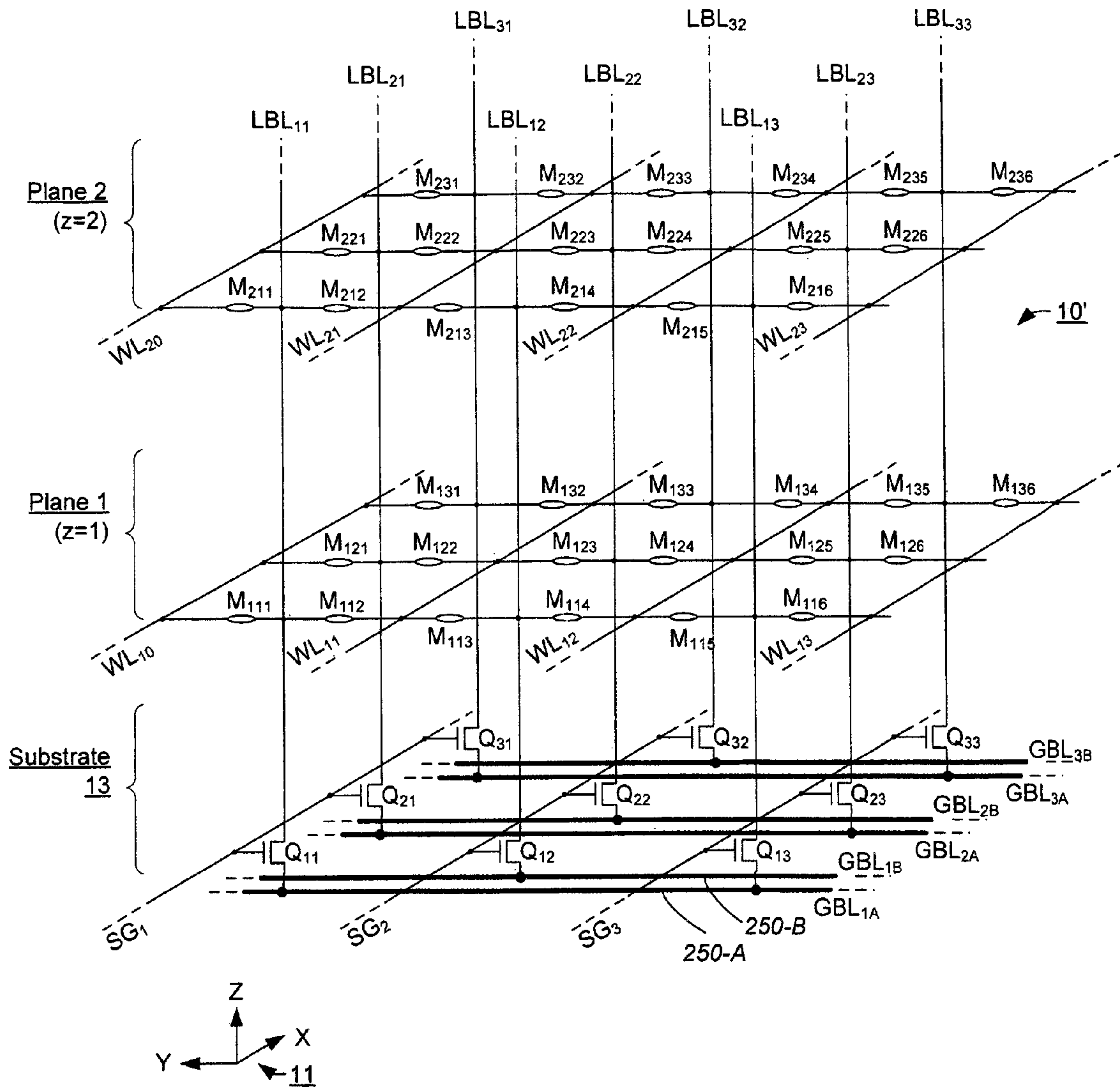
Double-Global-Bit-line Structure
