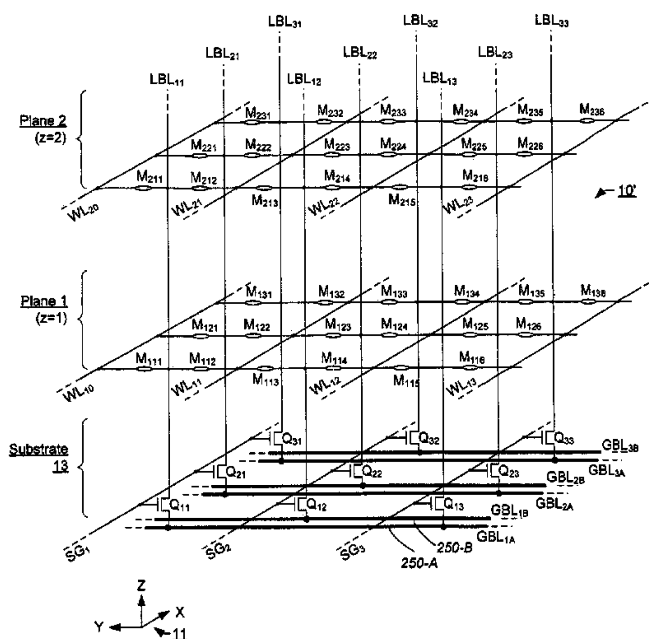
Double-Global-Bit-Line Structure
