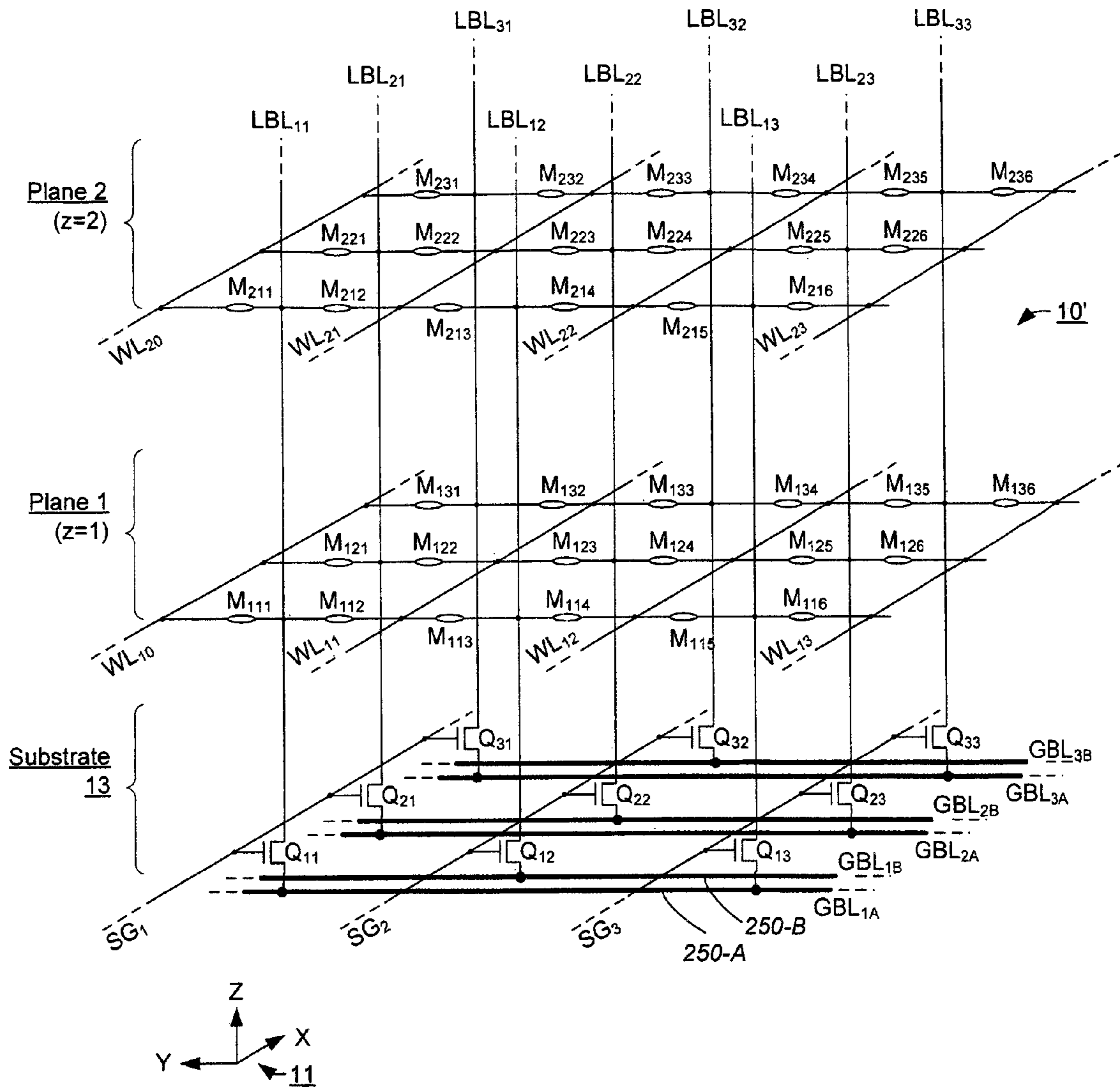
Double-Global-Bit-line Structure
