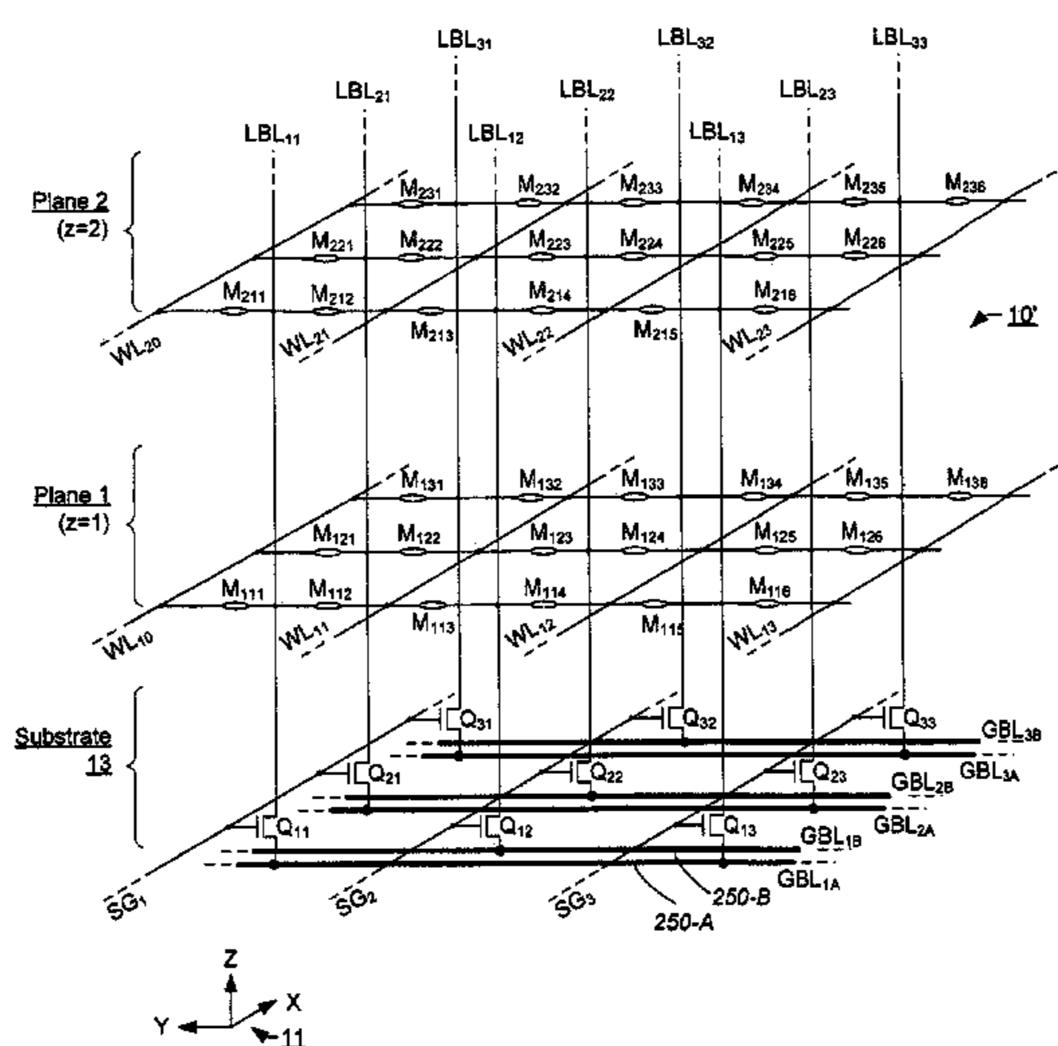
Double-Global-Bit-Line Structure
