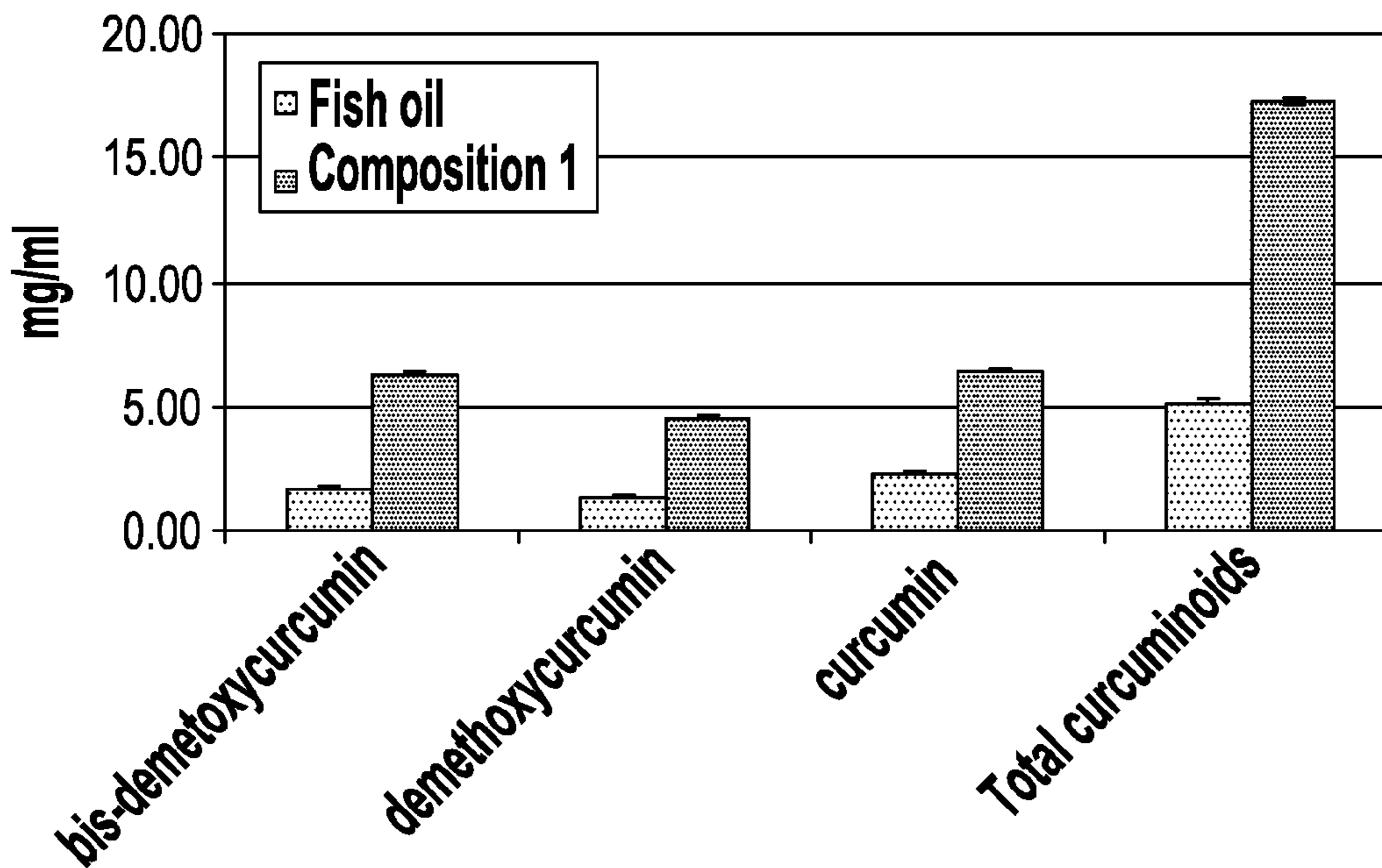
Curcuminoids solubility
