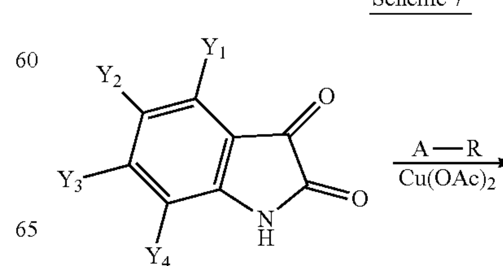
Scheme 7 a
