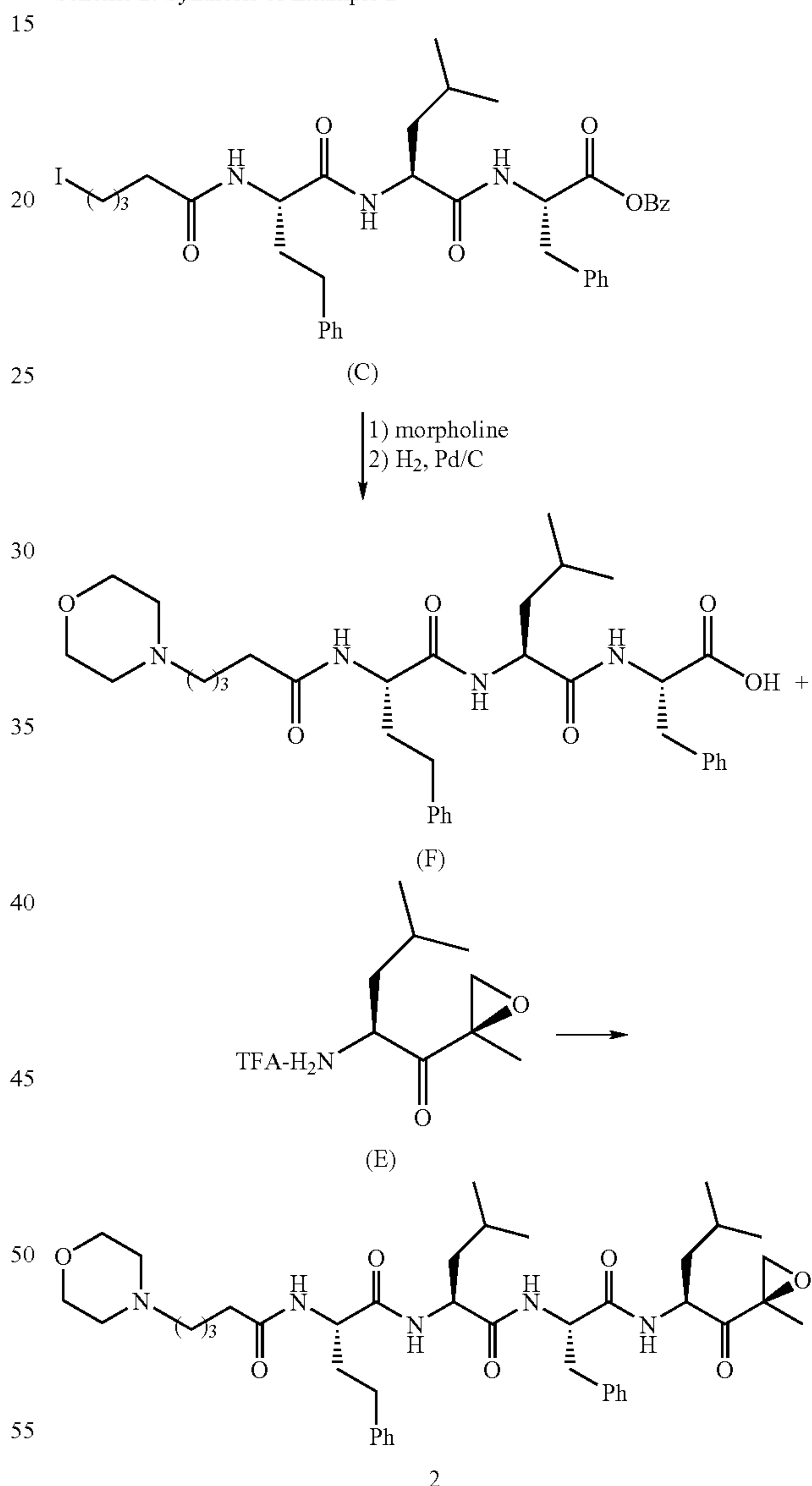
Scheme 2: Synthesis of Example 2
