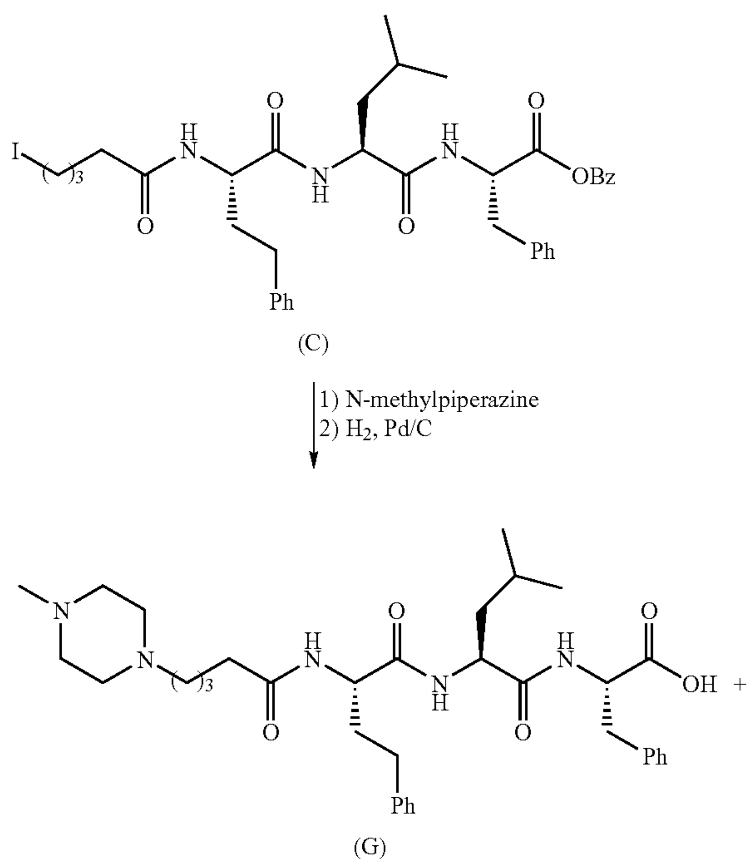
Scheme 3: Synthesis of Example 3
