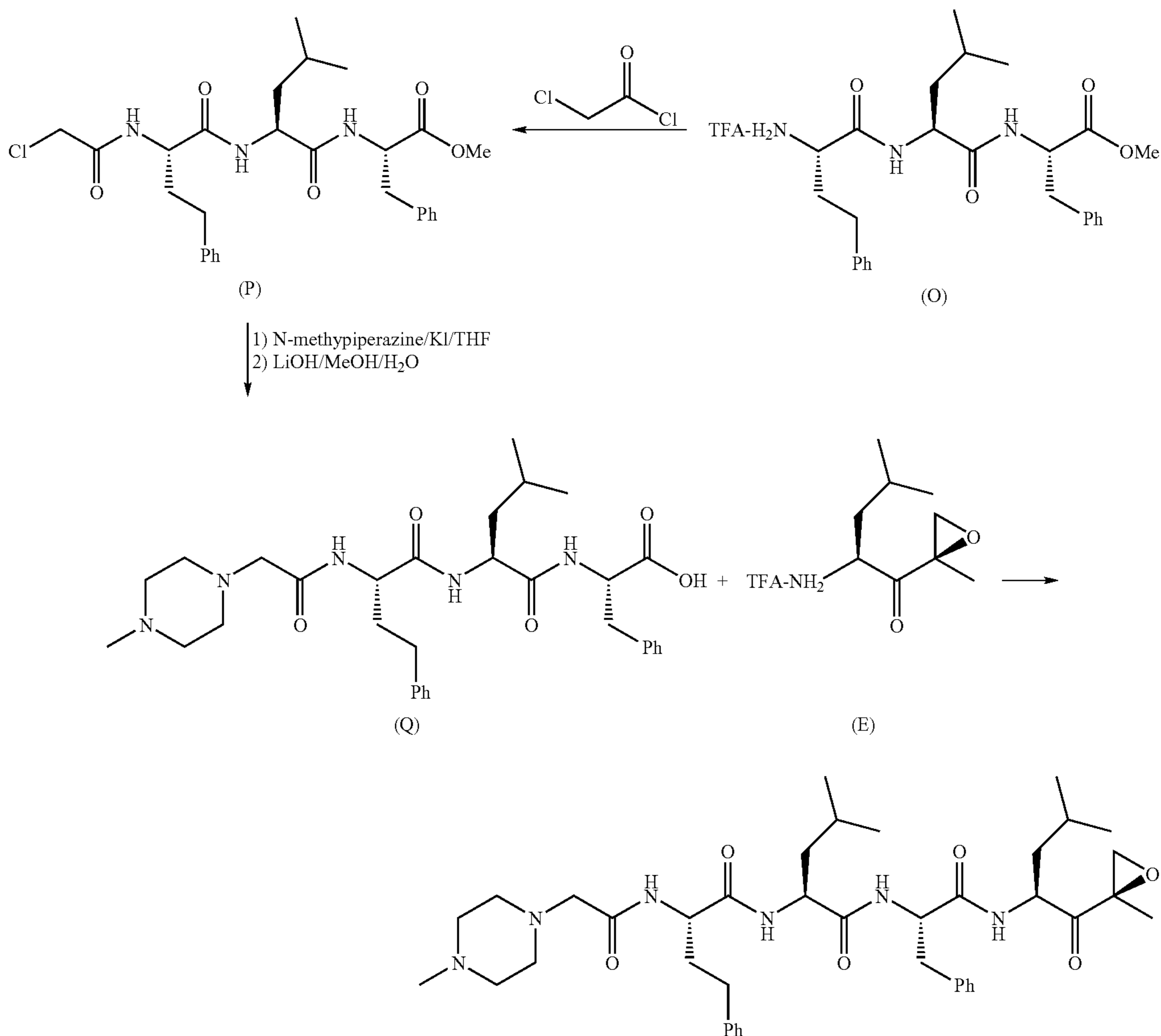
Scheme 8: Synthesis of Example 9
