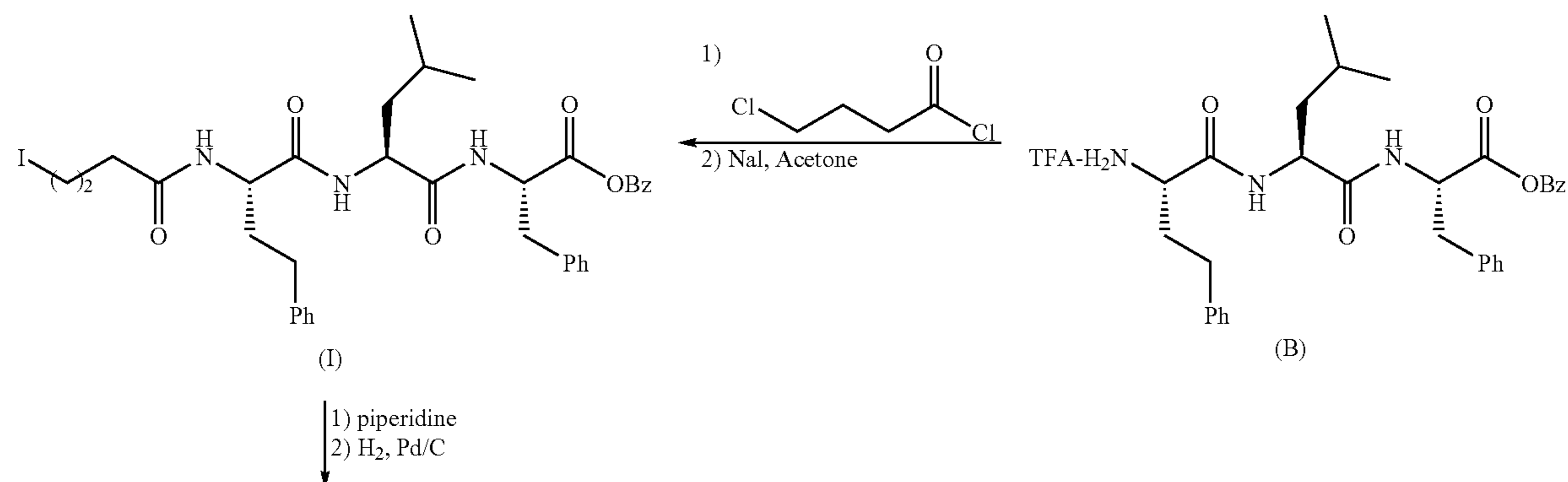
Scheme 4: Synthesis of Example 5
