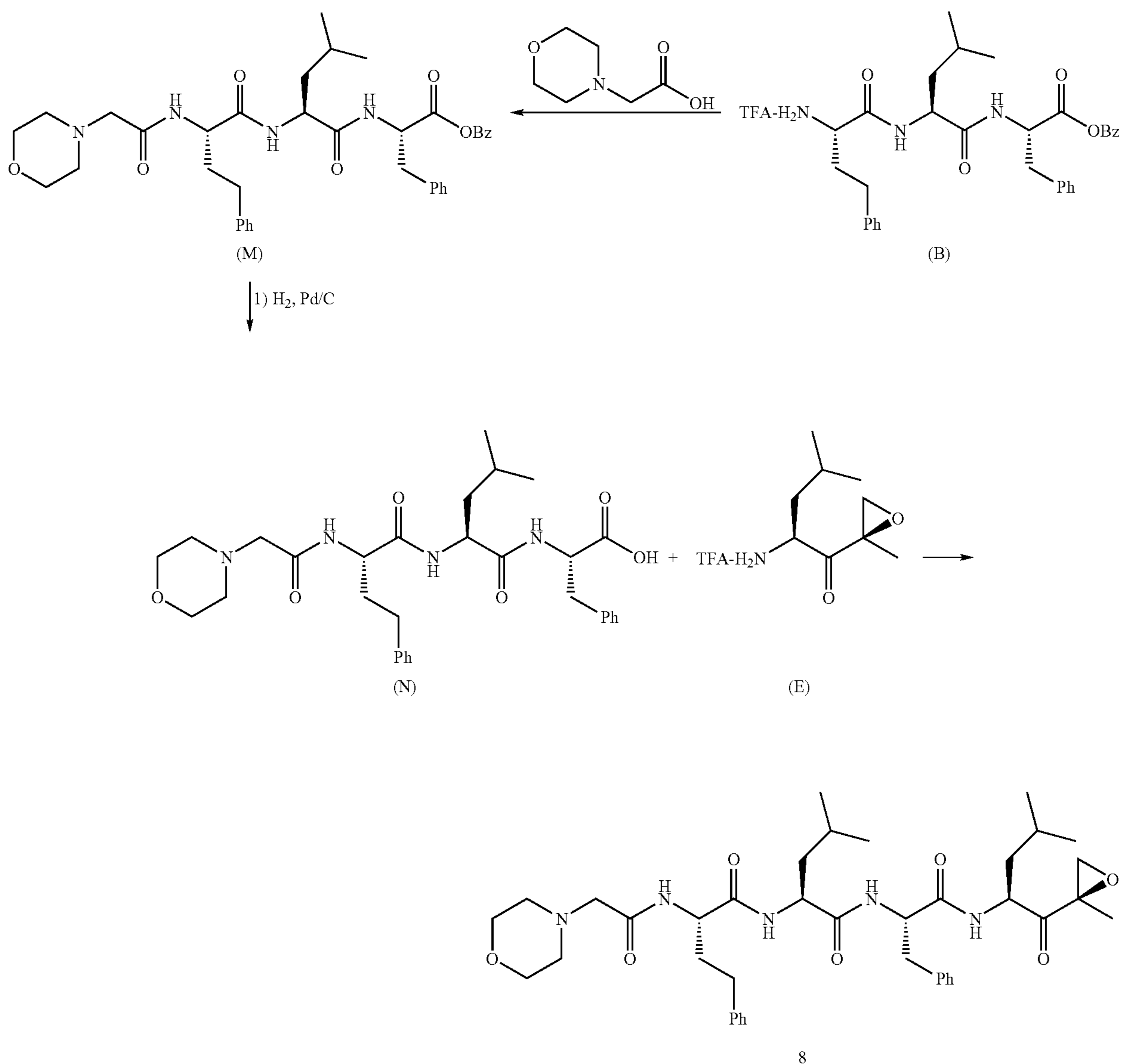
Scheme 7: Synthesis of Example 8
