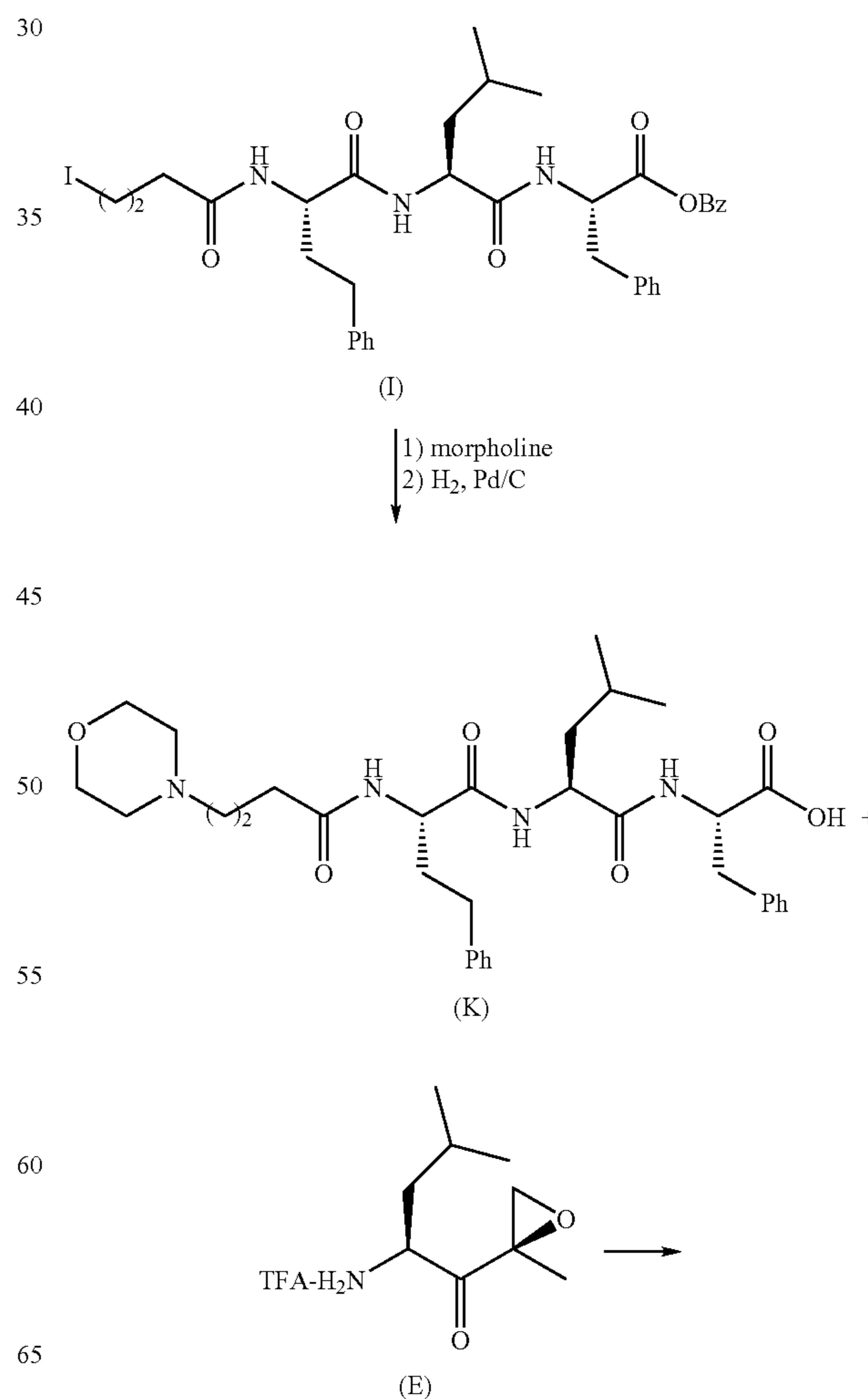
Scheme 5: Synthesis of Example 6
