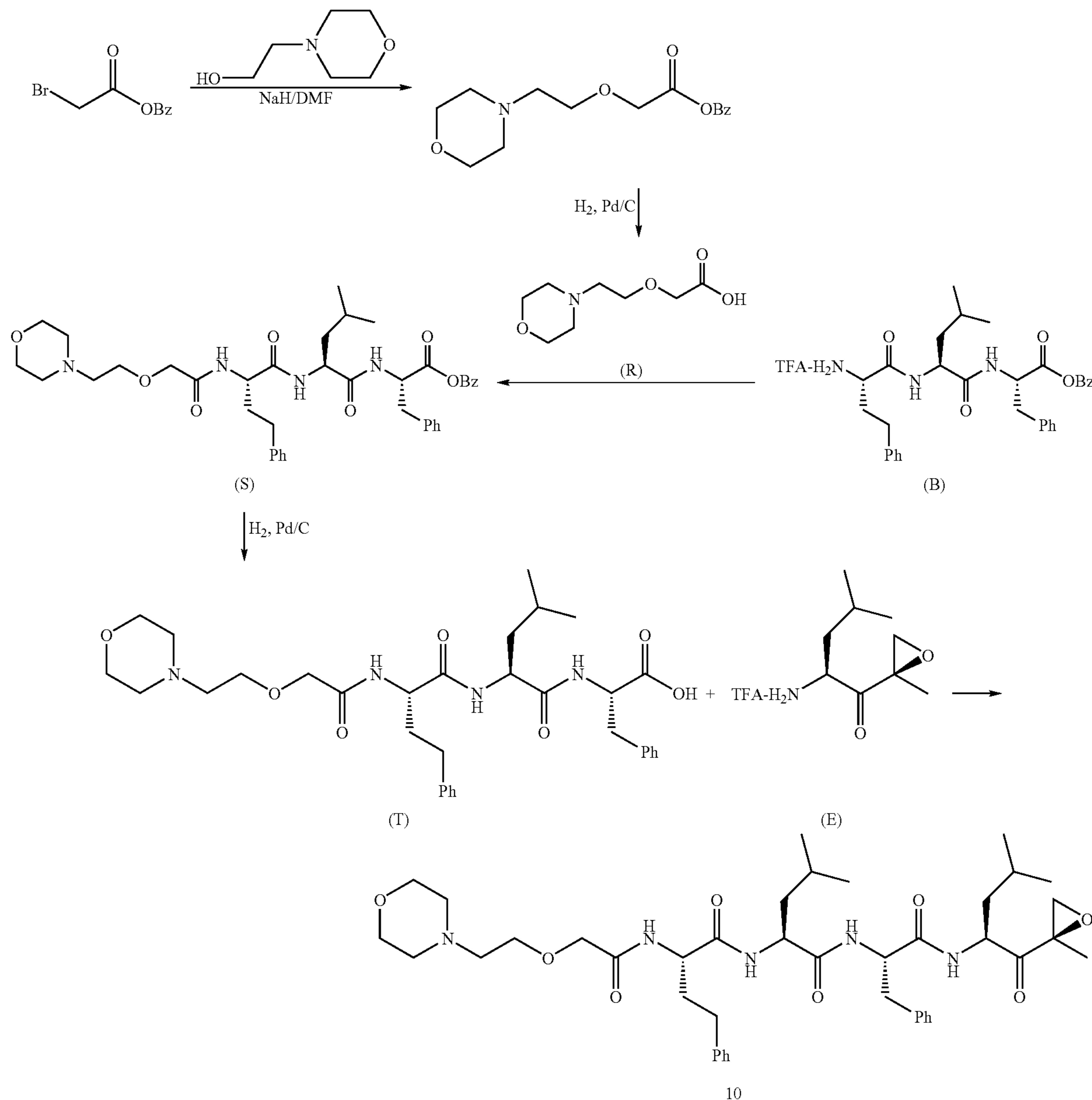
Scheme 9: Synthesis of Example 10
