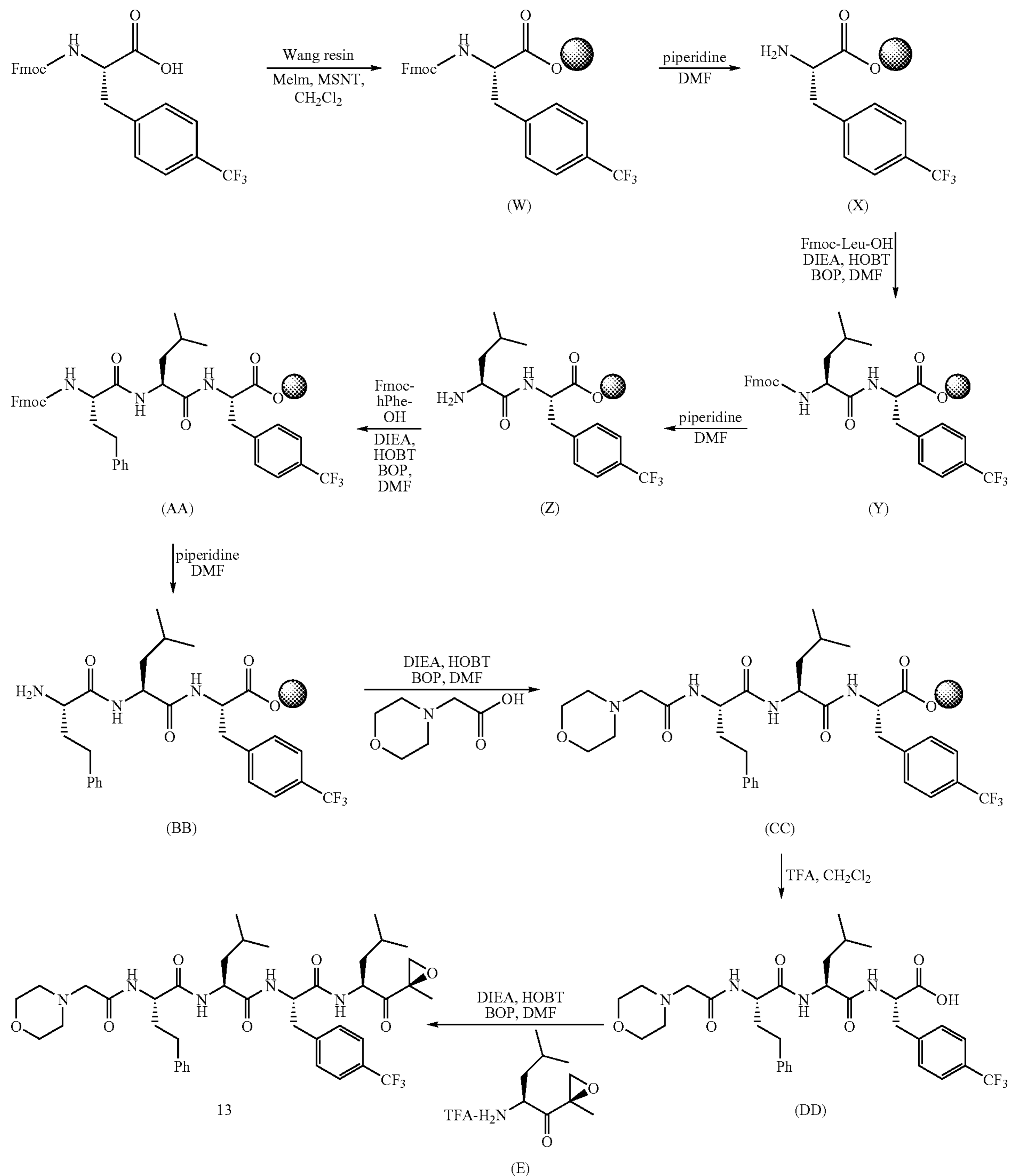
Scheme 10: Synthesis of Example 13
