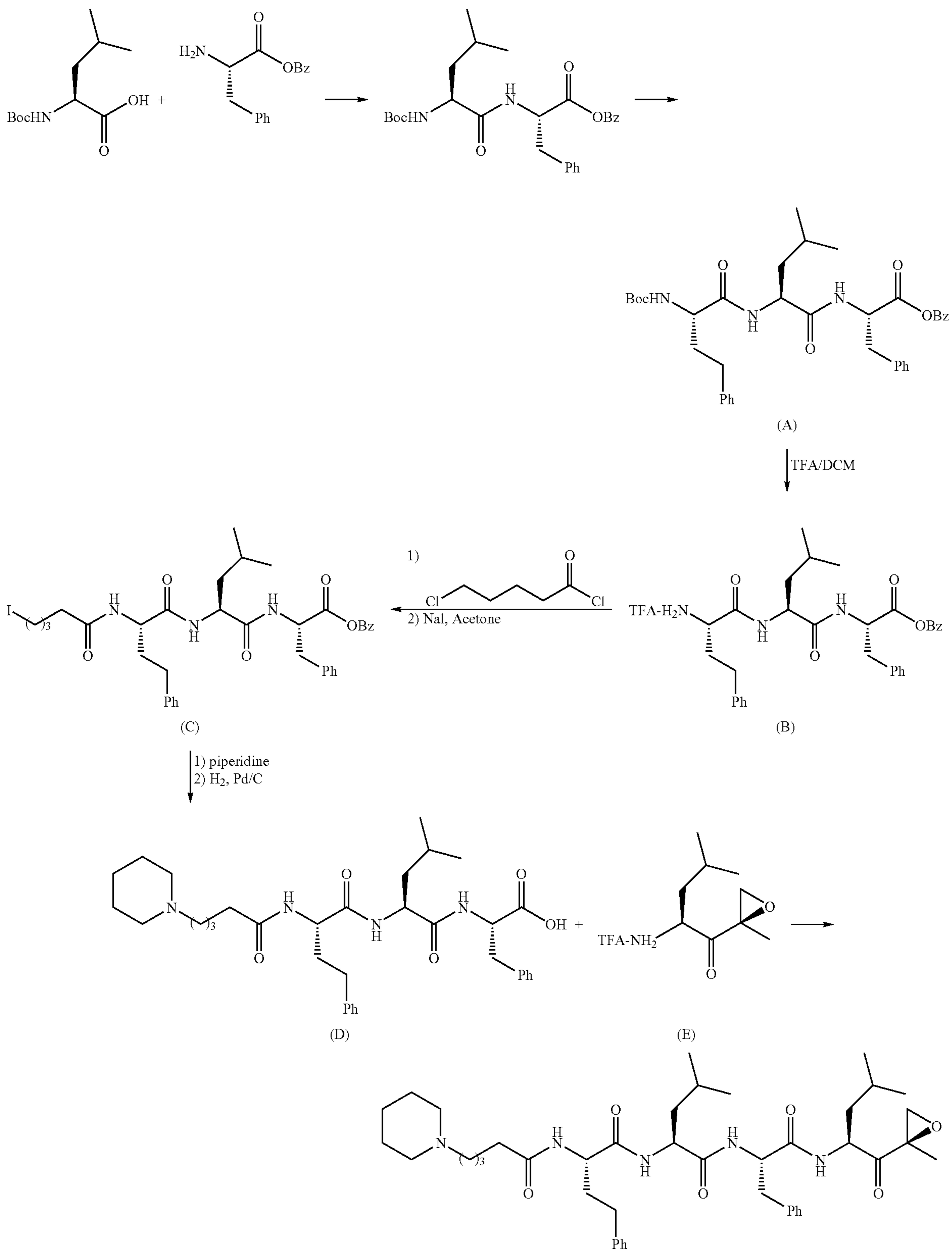
Scheme 1: Synthesis of Example 1
