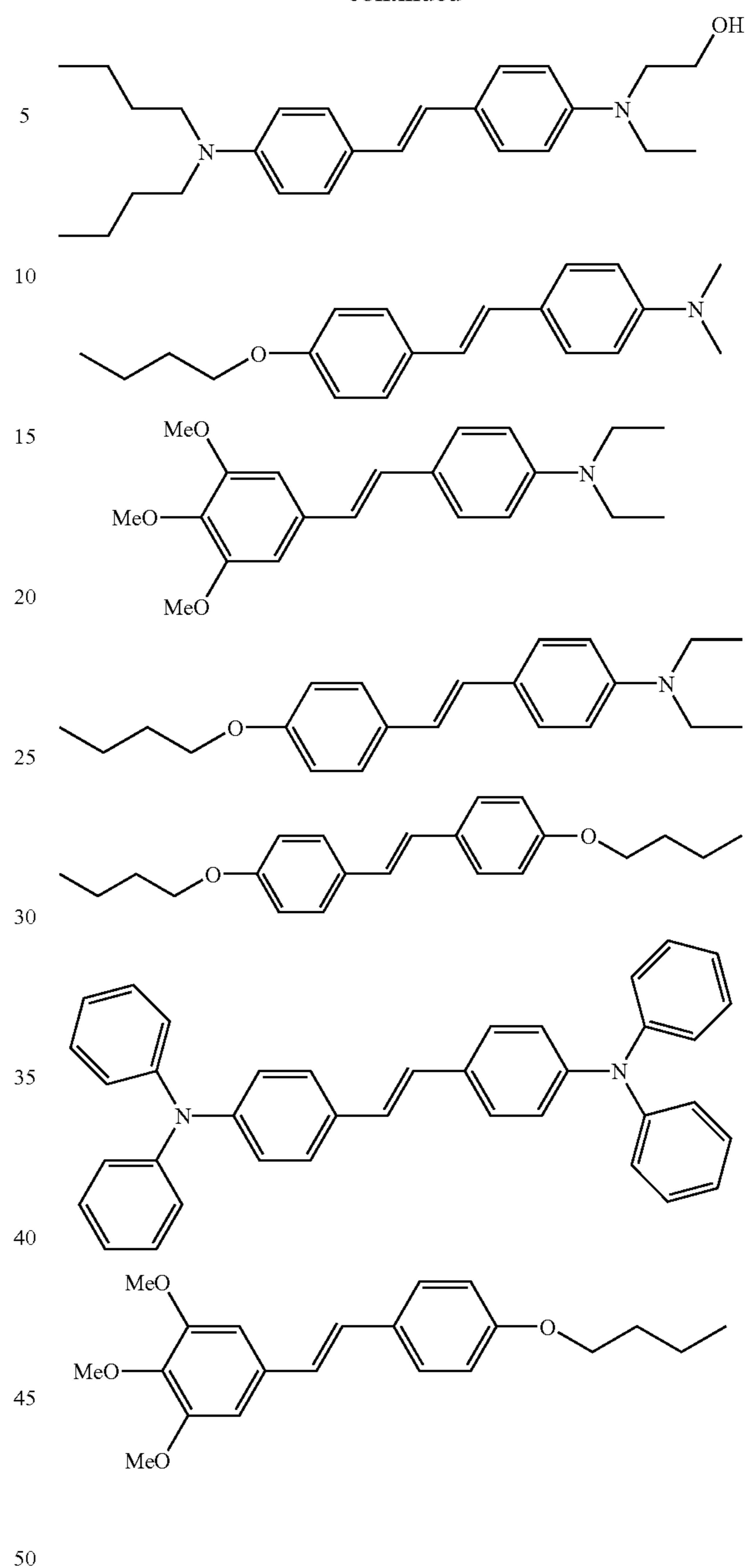
EXAMPLES OF STILBENE CHROMOPHORES
