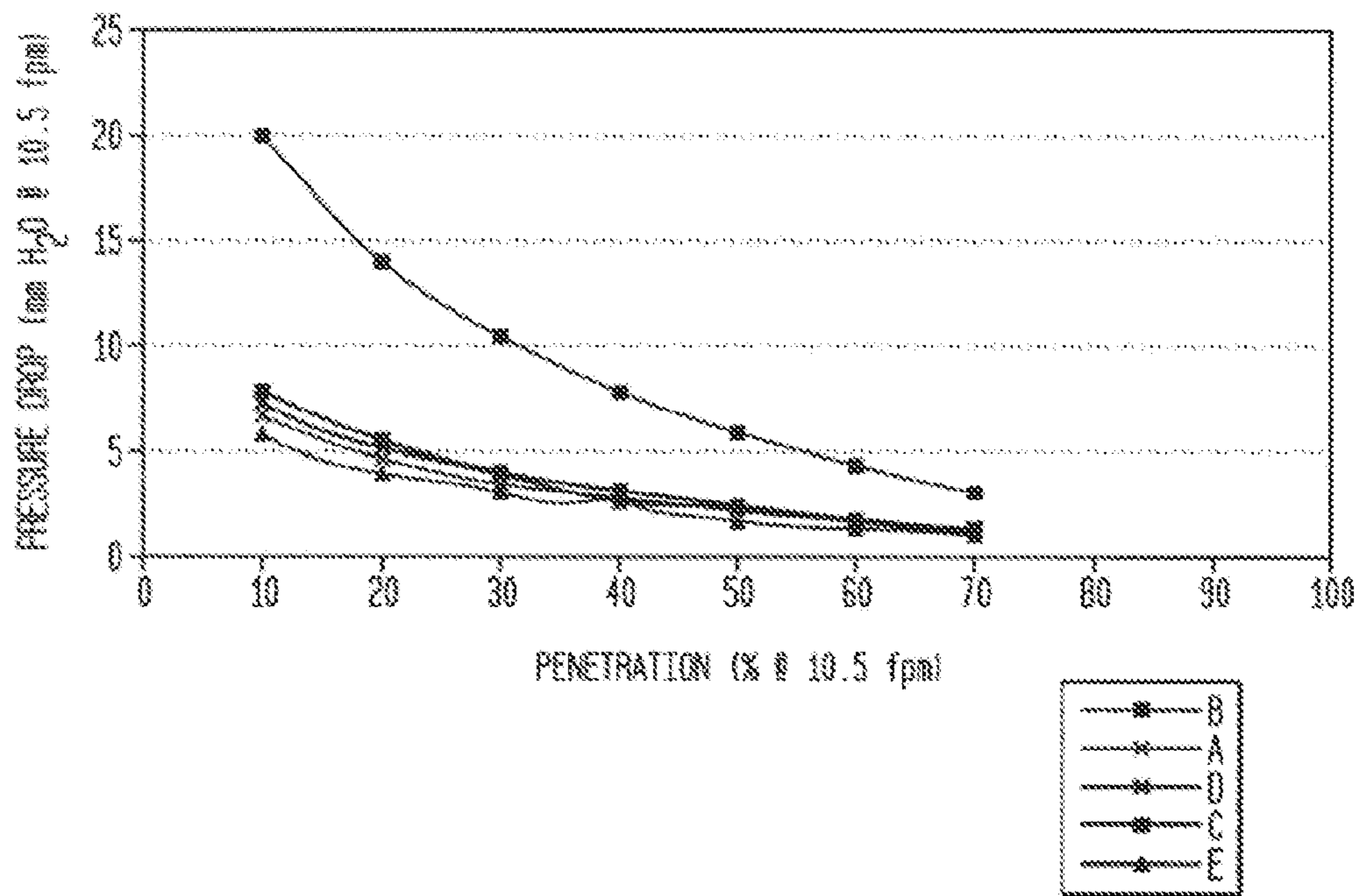
DISCHARGED DOP PENETRATION VERSUS PRESSURE DROP
