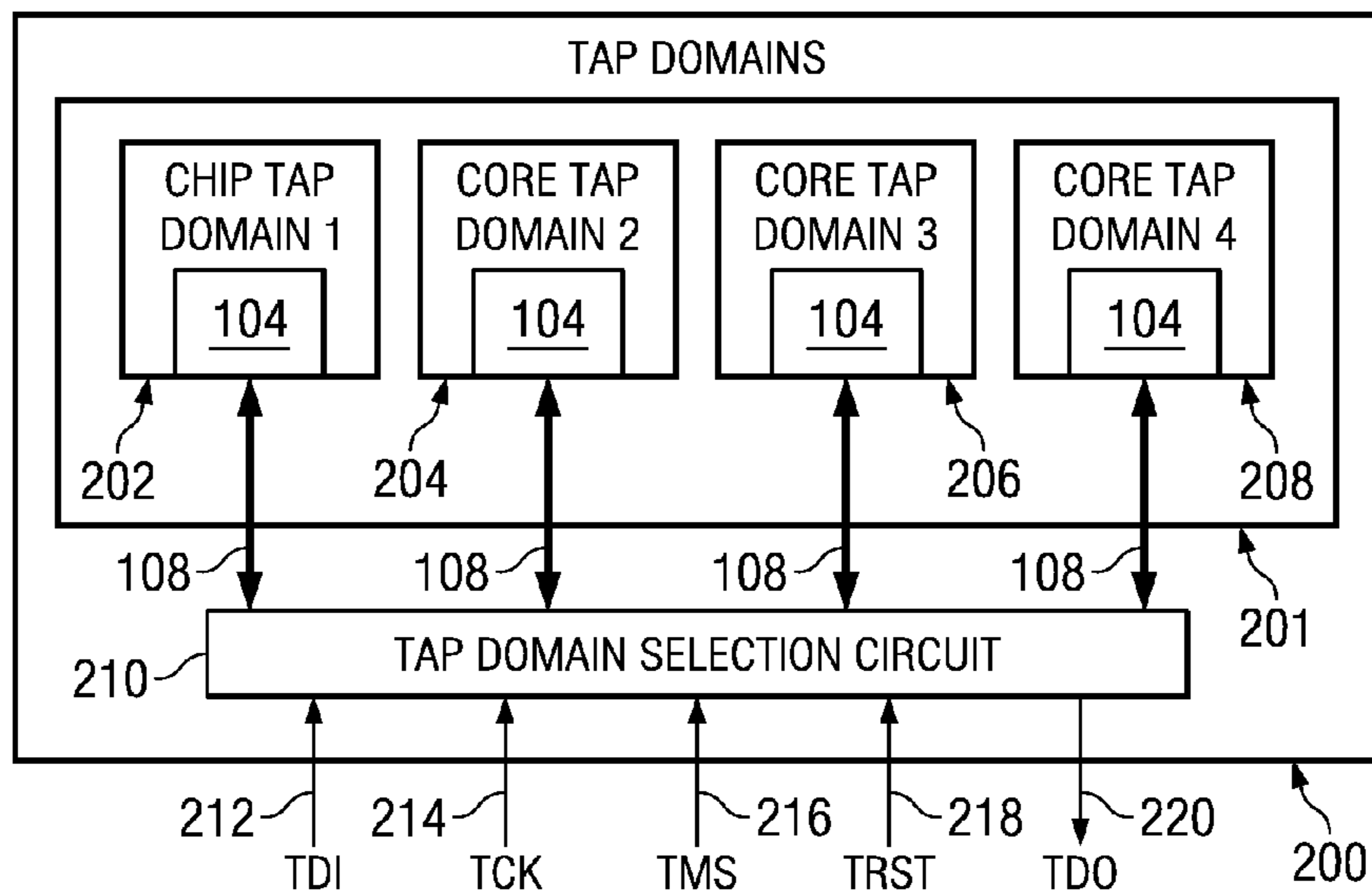
FIG. 2 (PRIOR ART)
