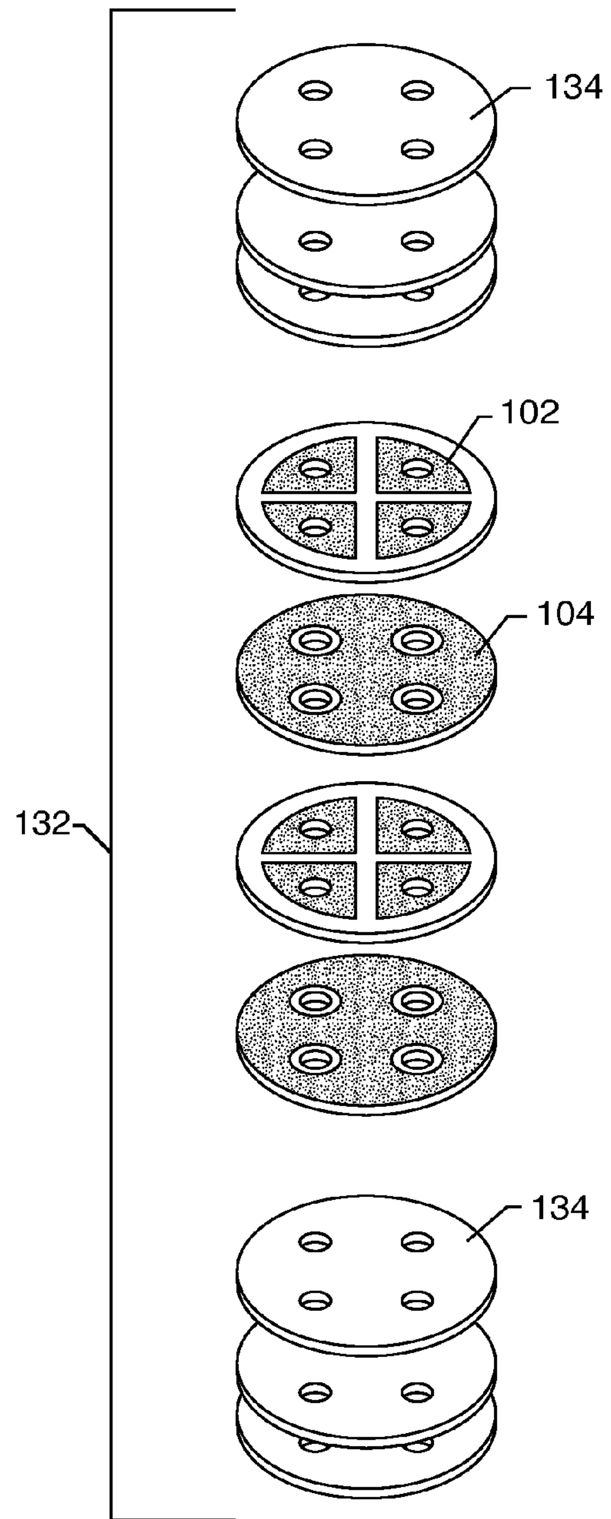
FIG. 9 PRIOR ART
