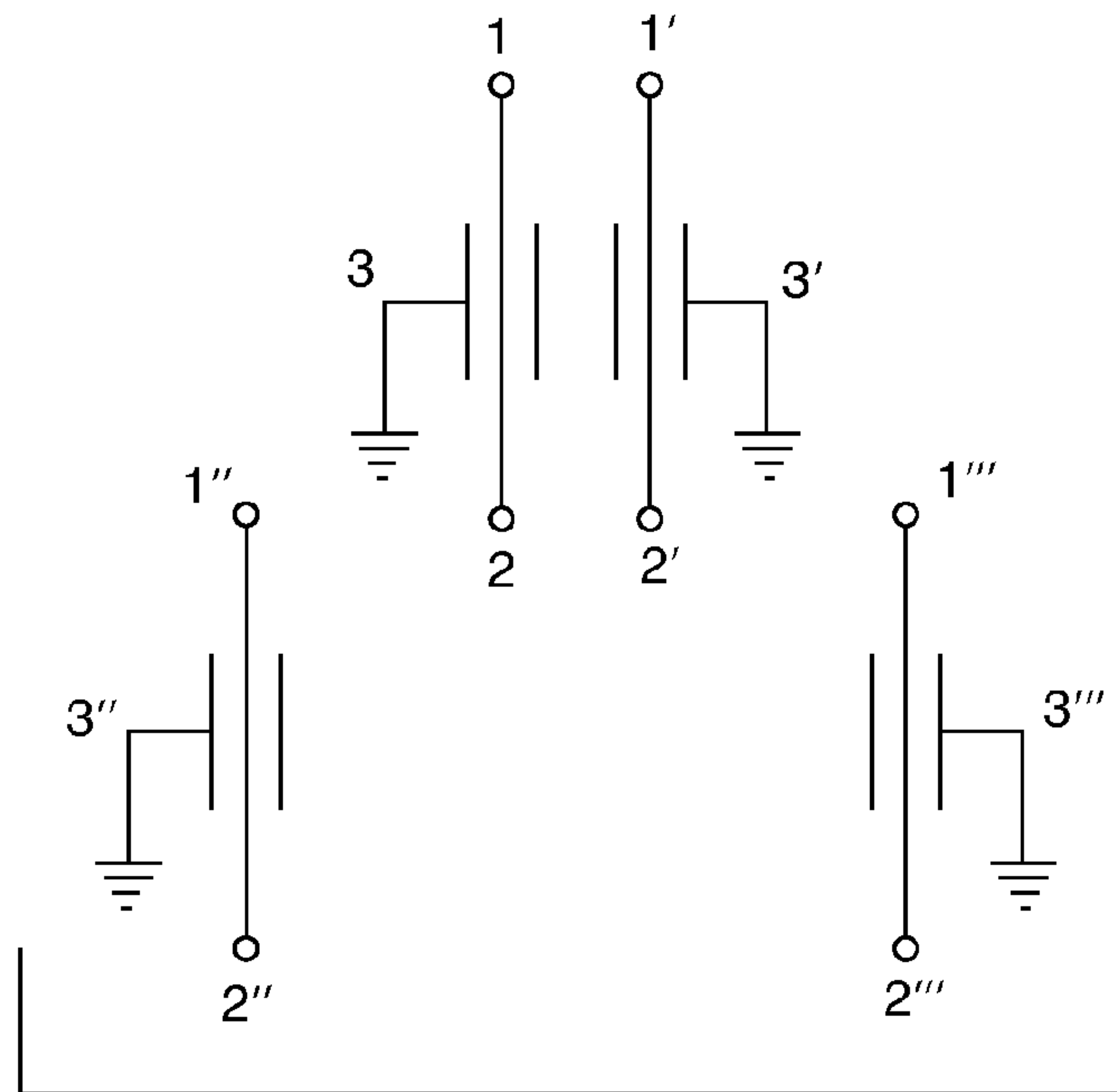
FIG. 7 PRIOR ART
