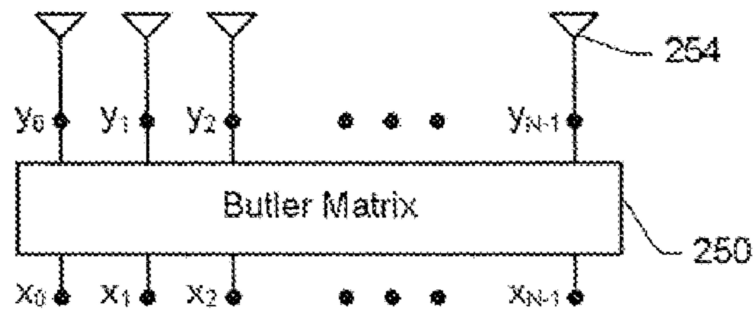
Fig. 4 (Prior Art)
