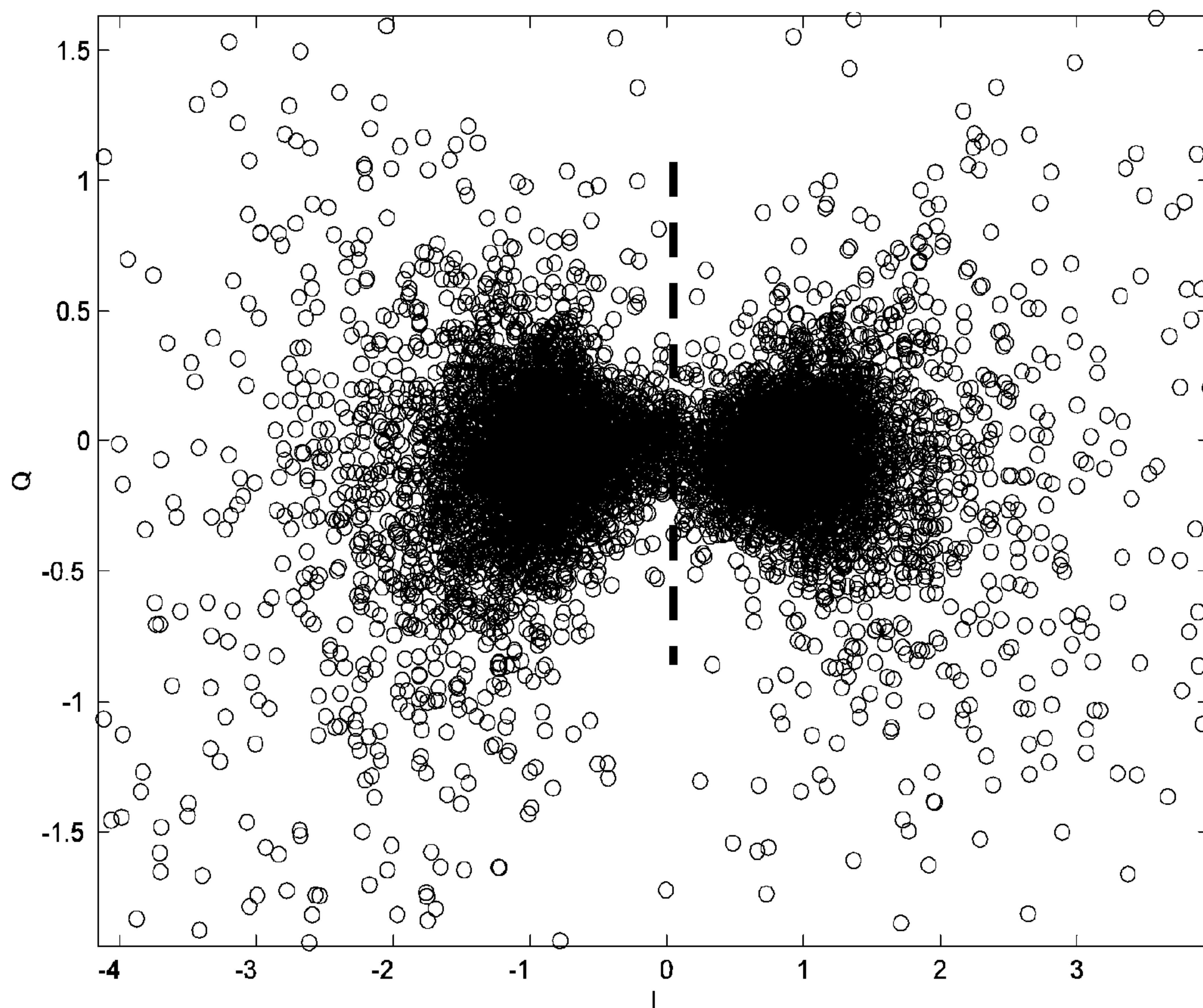
Differential BPSK Demodulation: 10 bits/frame, 500Hz carrier
