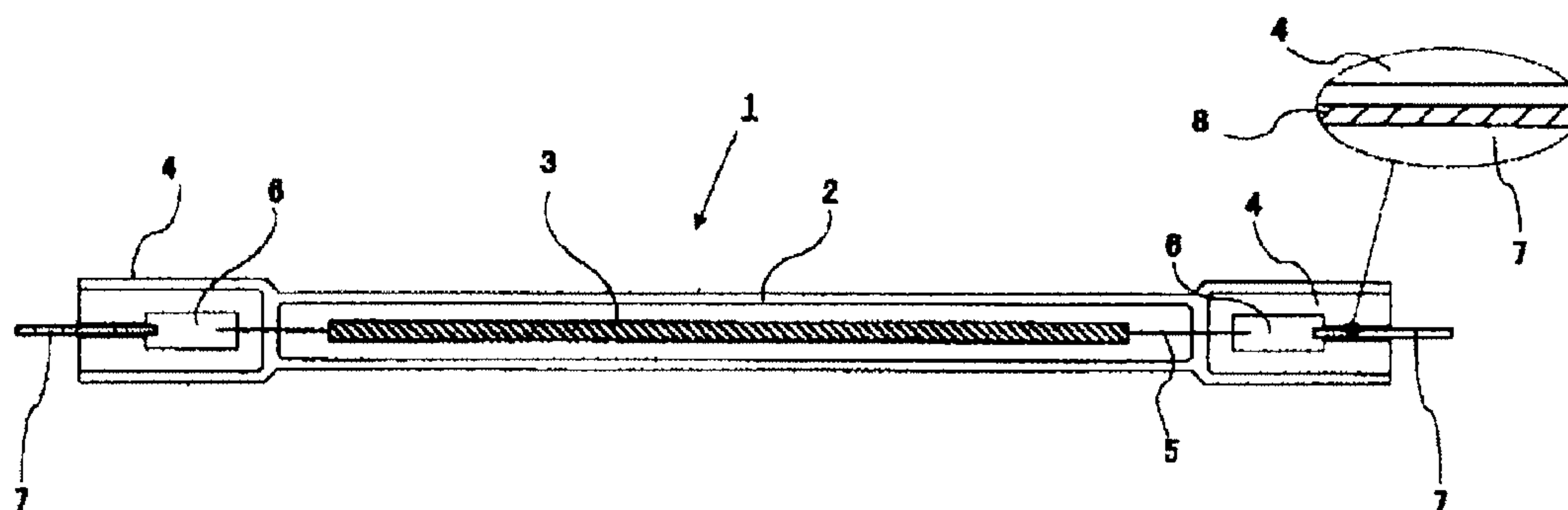
Fig. 5 (Prior Art)
