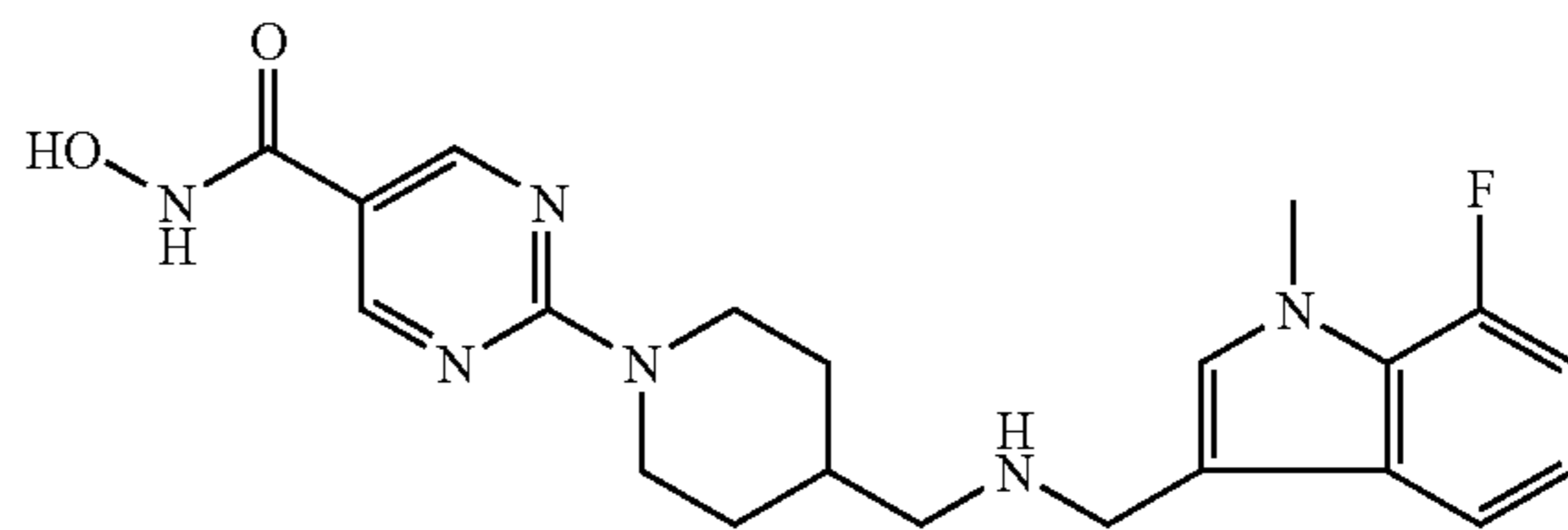
compound 30
