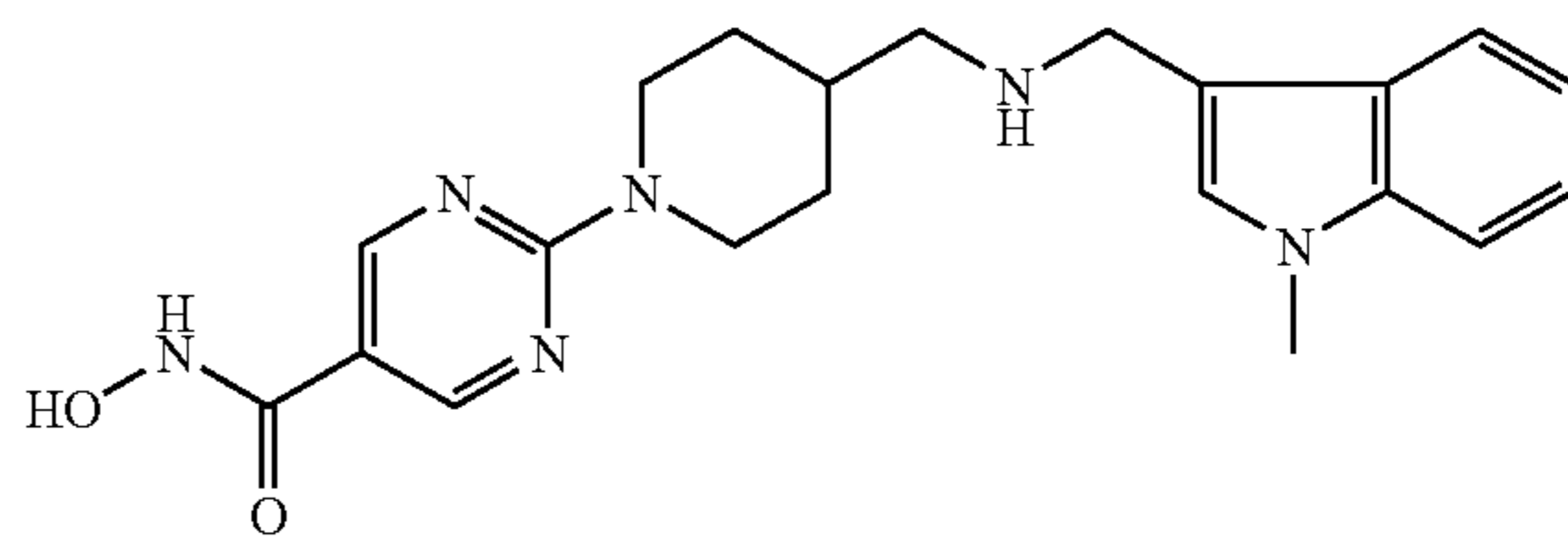
Compound 1a
