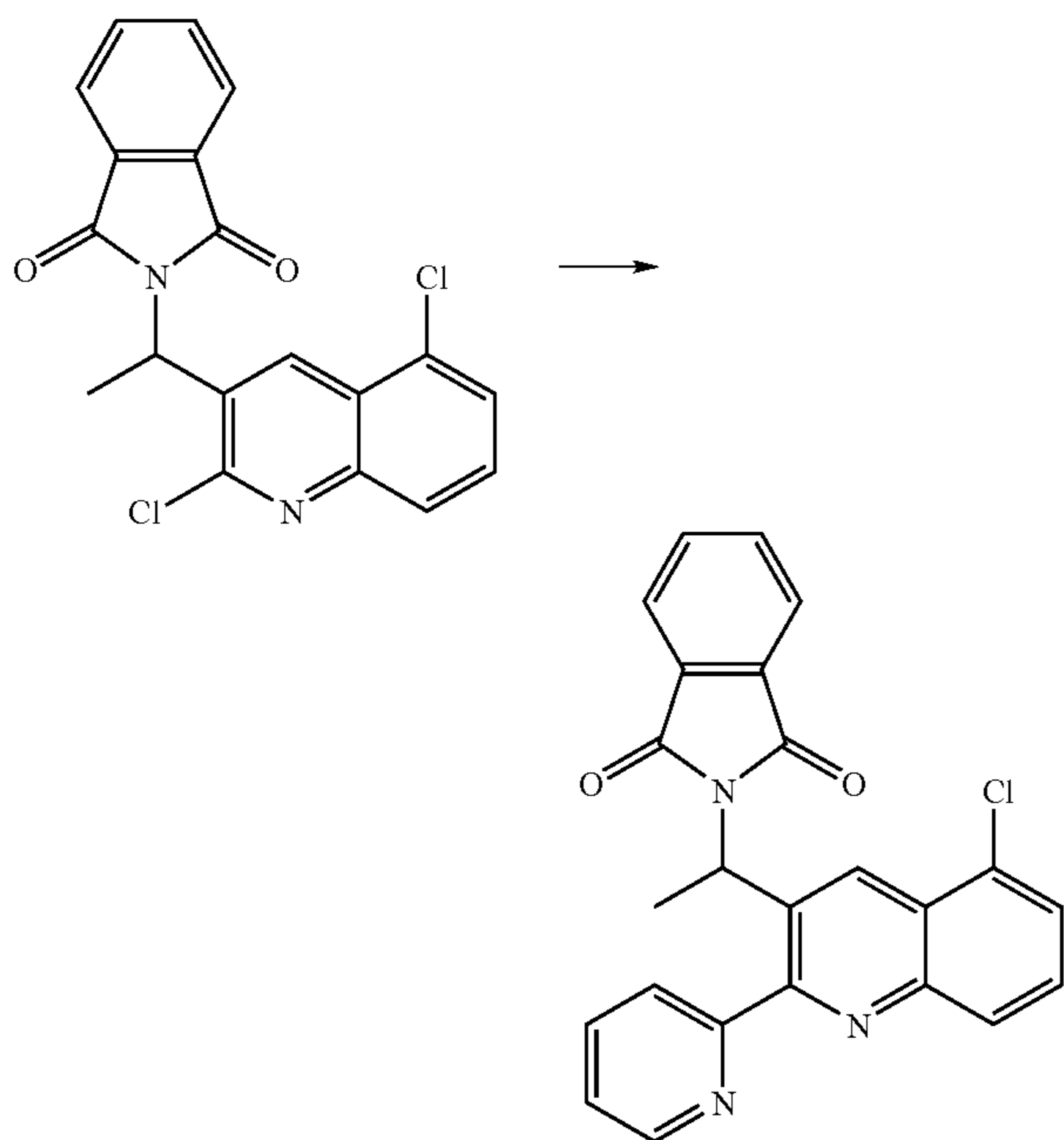
2-(1-(5-Chloro-2-(pyridin-2-yl)quinolin-3-yl)ethyl)isoindoline-1,3-dione
