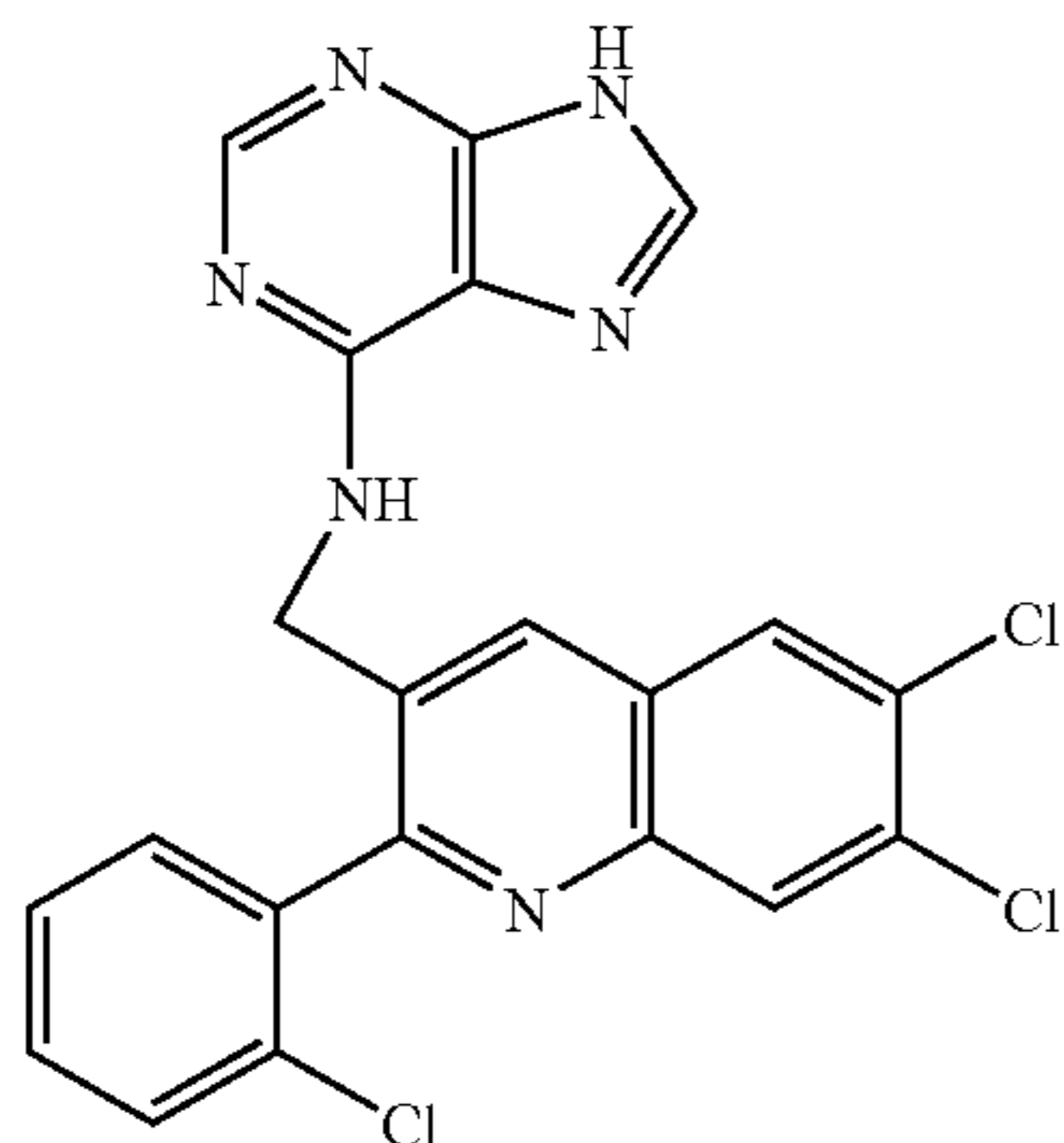
Example 71
