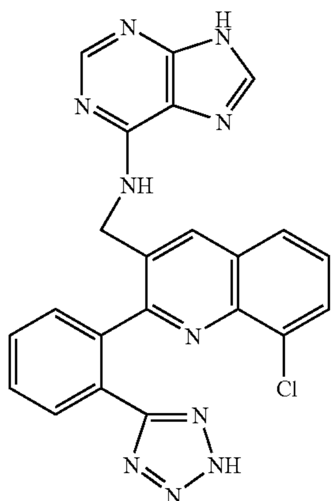
Example 70
