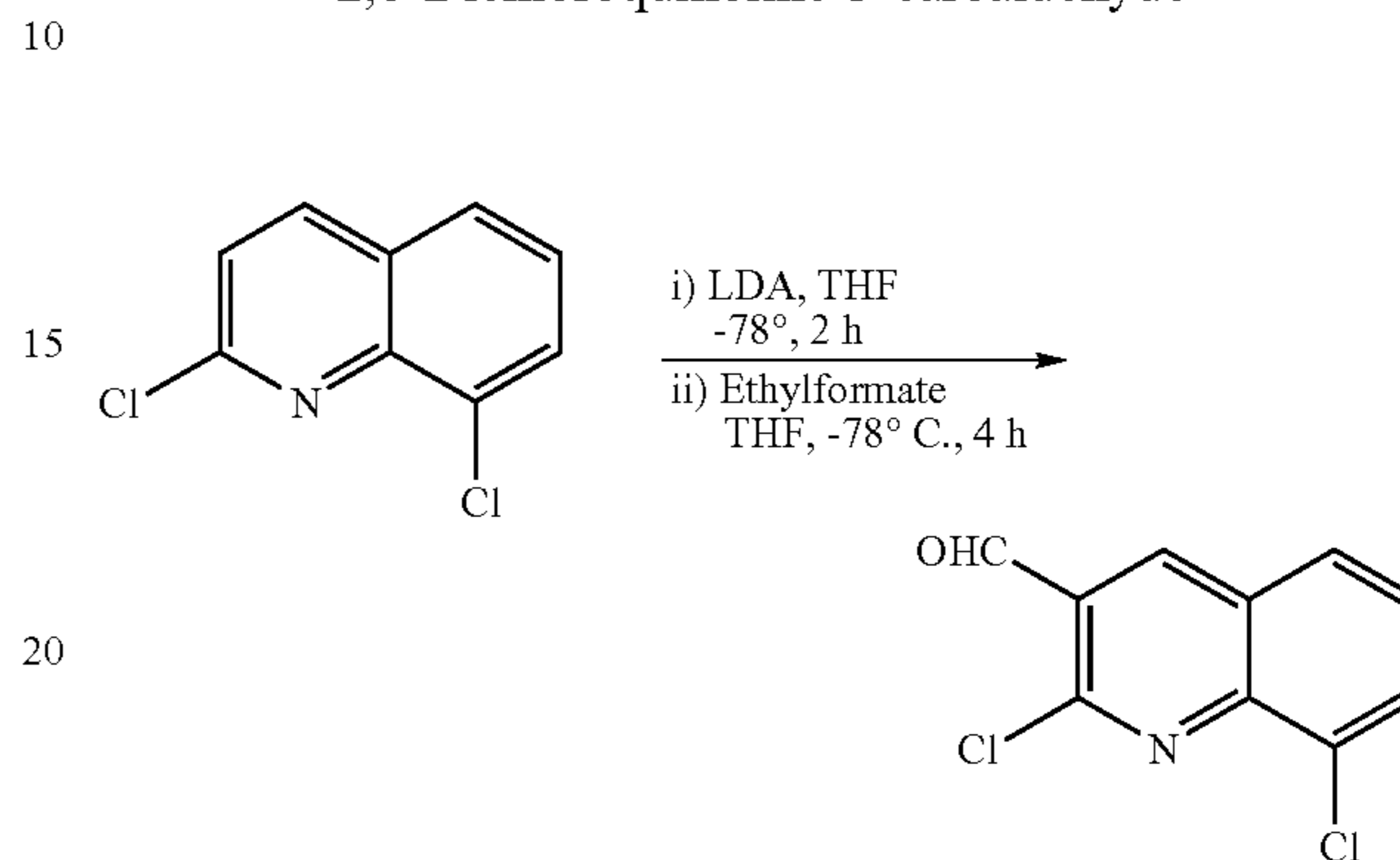
2,8-Dichloroquinoline-3-carbaldehyde
