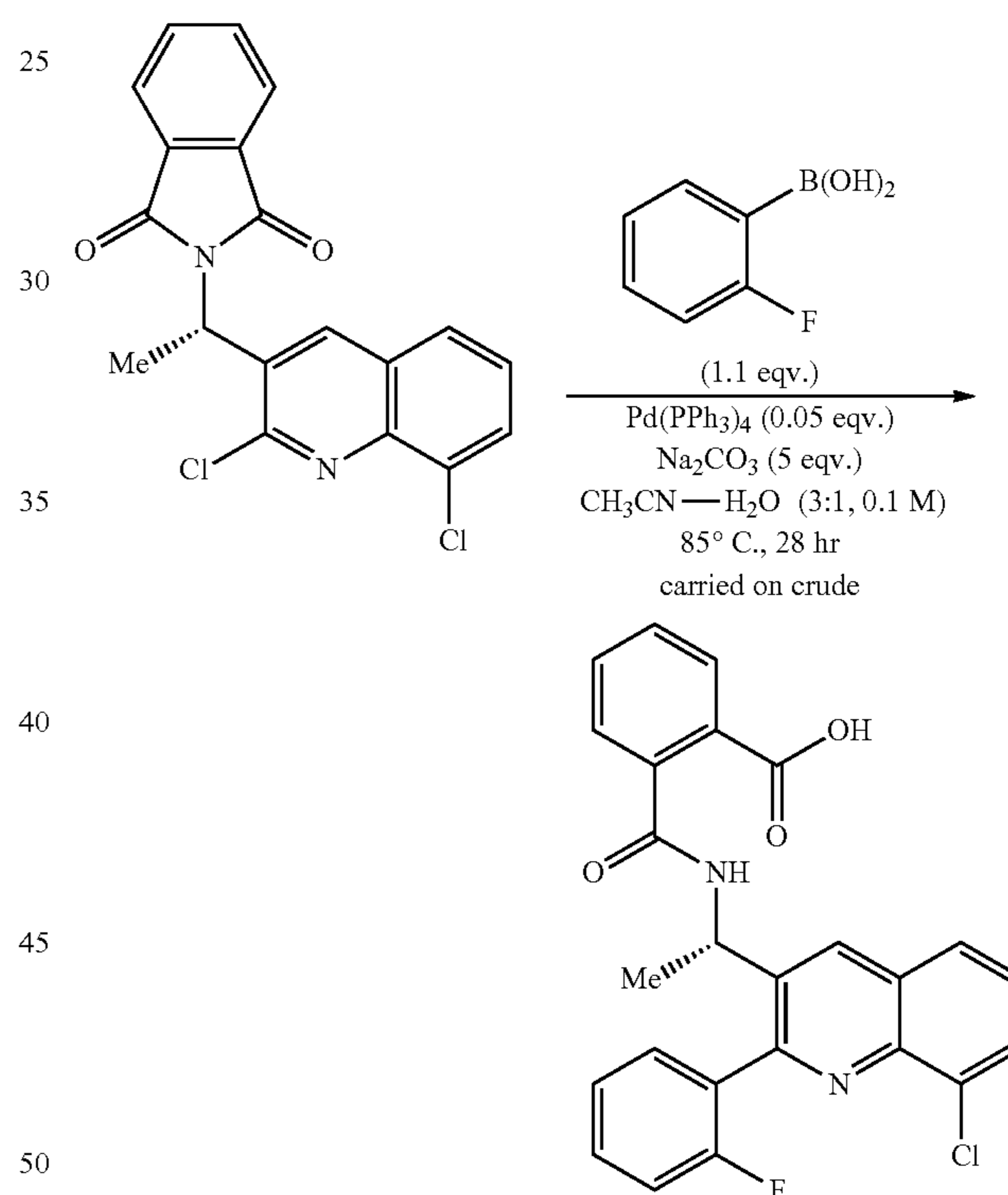
N-((2-(3-Fluorophenyl)-8-methoxyquinolin-3-yl)methyl)-9H-purin-6-amine
