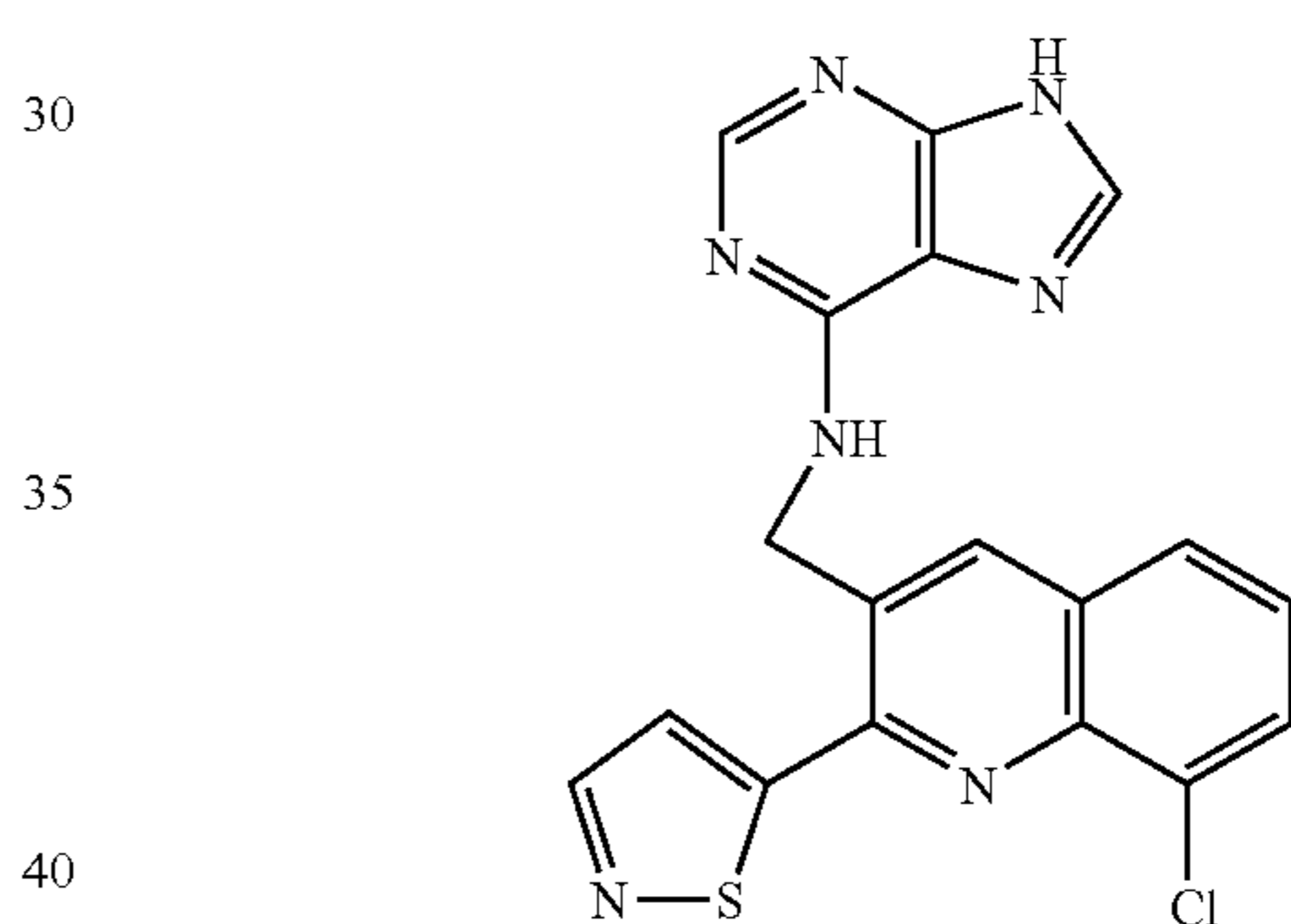
Example 74
