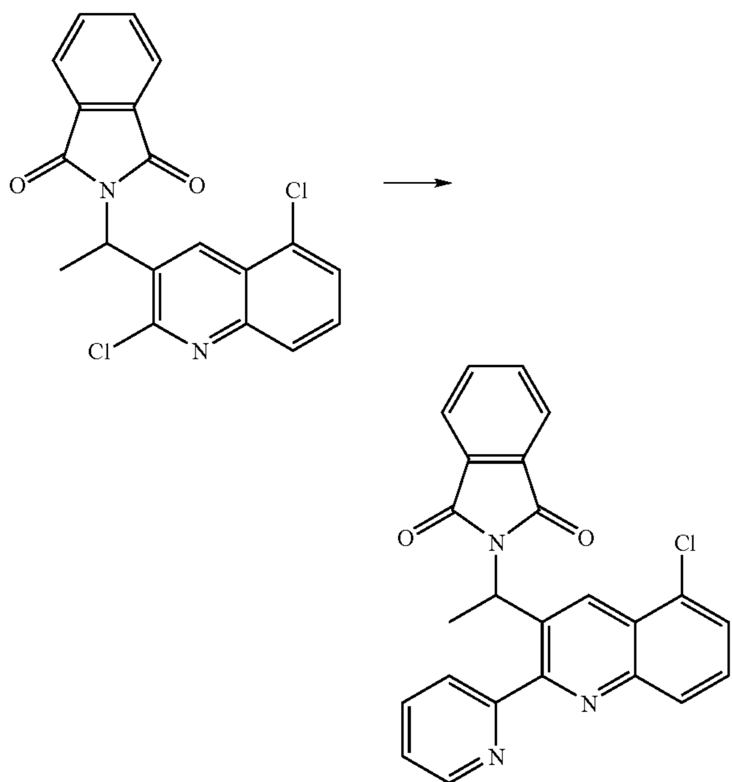
2-(1-(5-Chloro-2-(pyridin-2-yl)quinolin-3-yl)ethyl)isoindoline-1,3-dione
