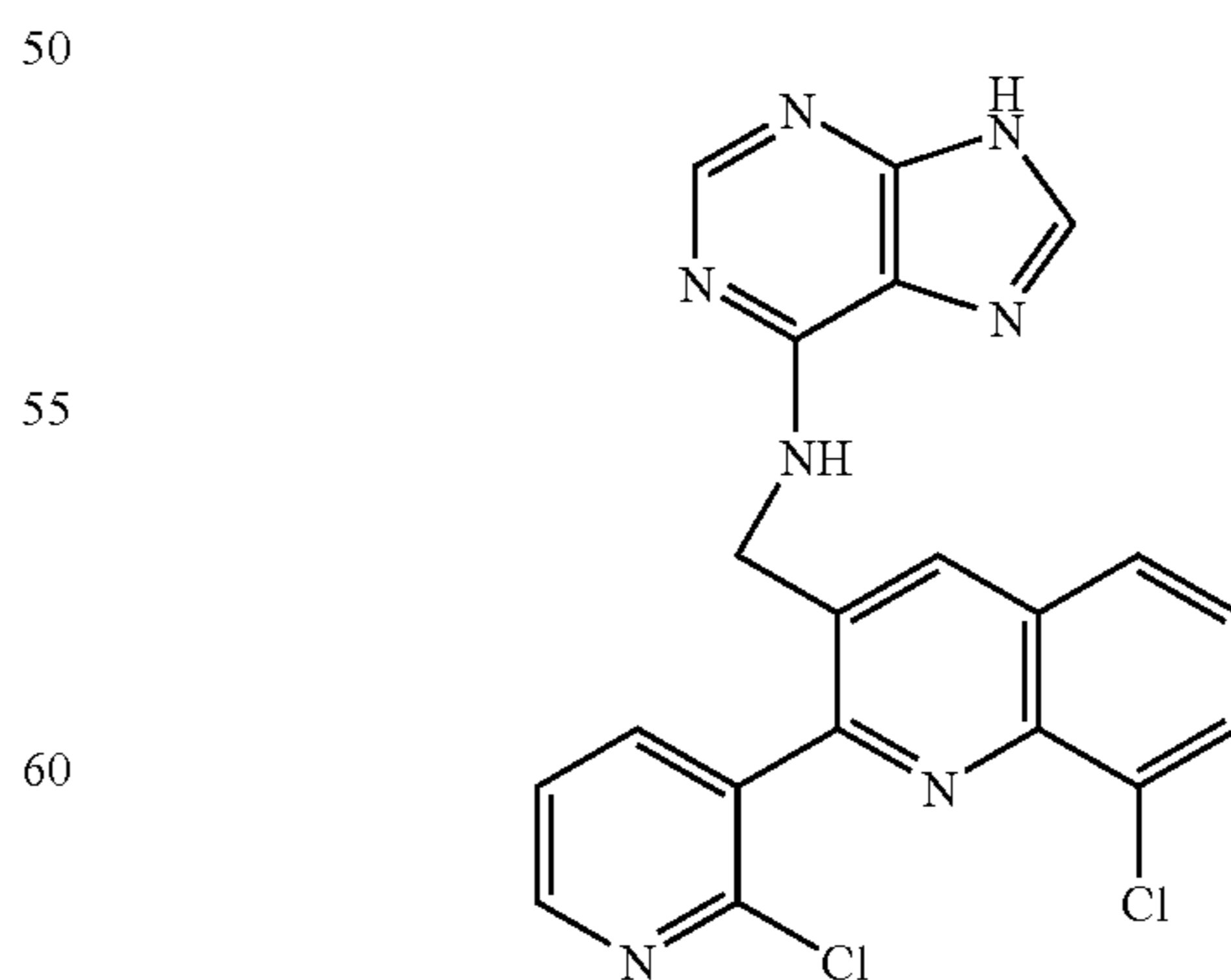
Example 75
