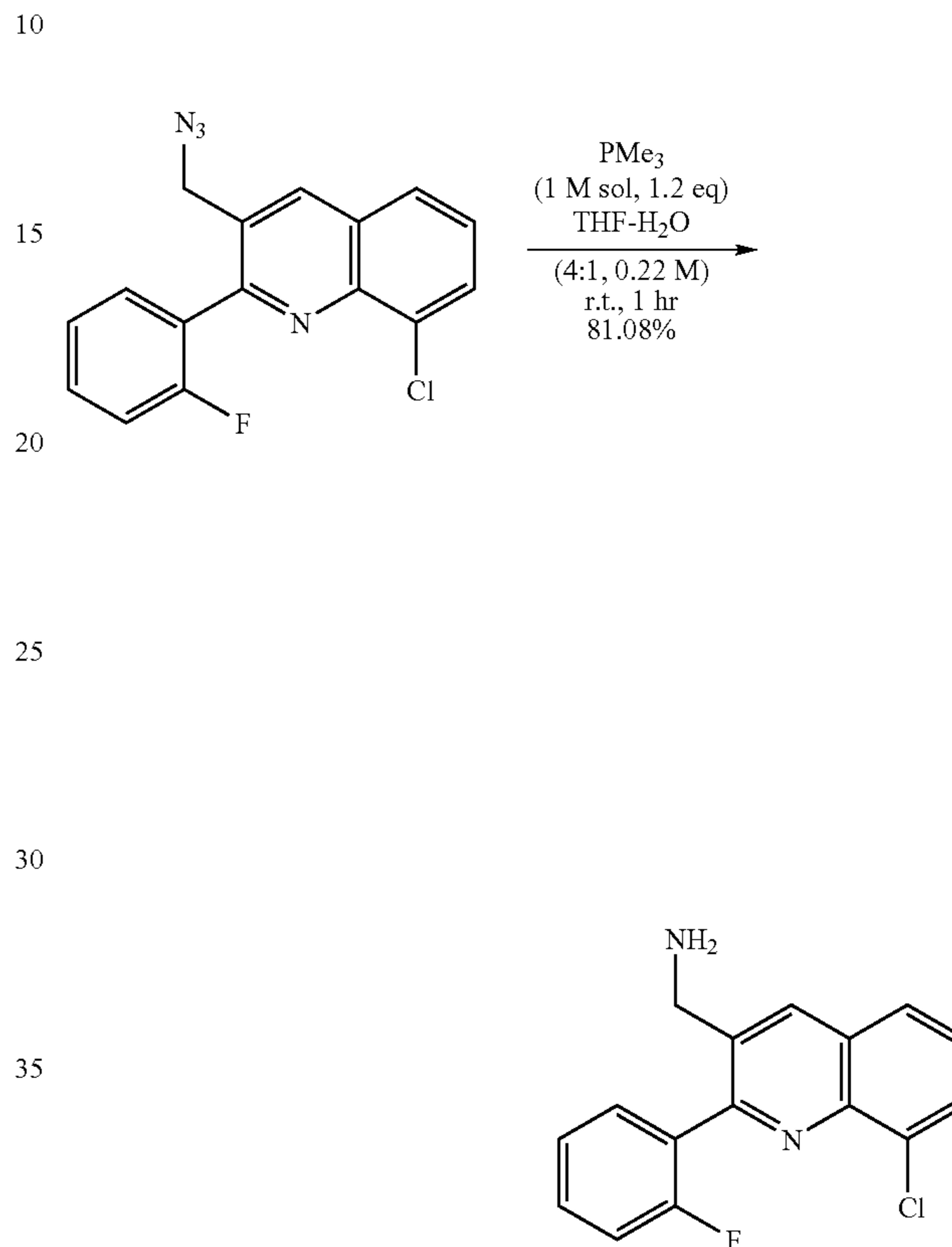
(8-Chloro-2-(2-fluorophenyl)quinolin-3-yl)methanamine
