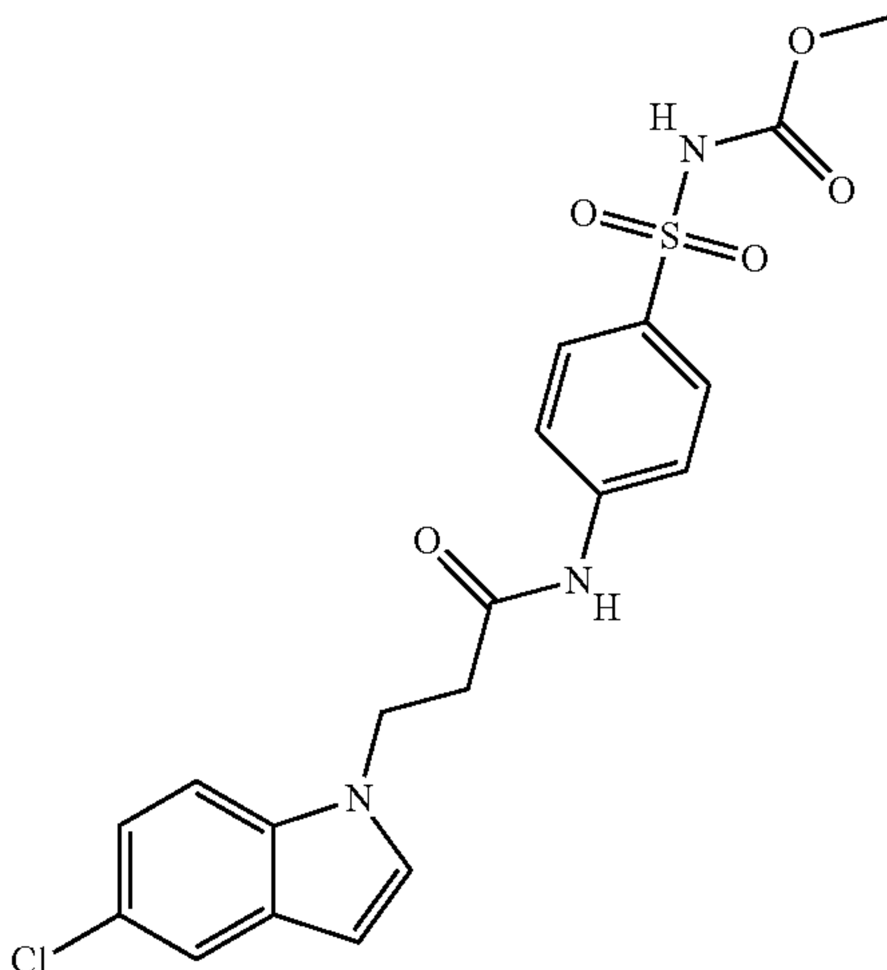
120 -continued
