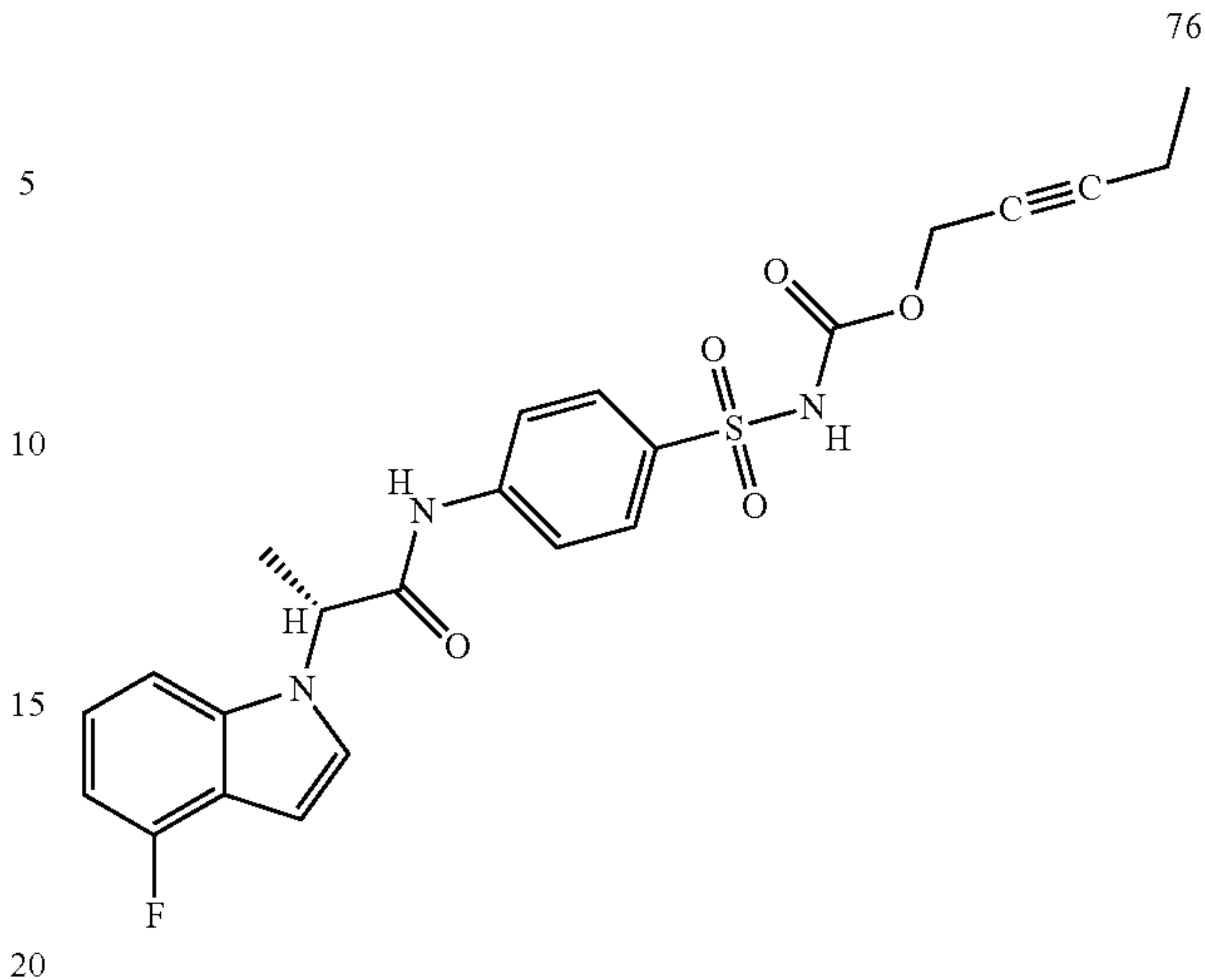
128 -continued
