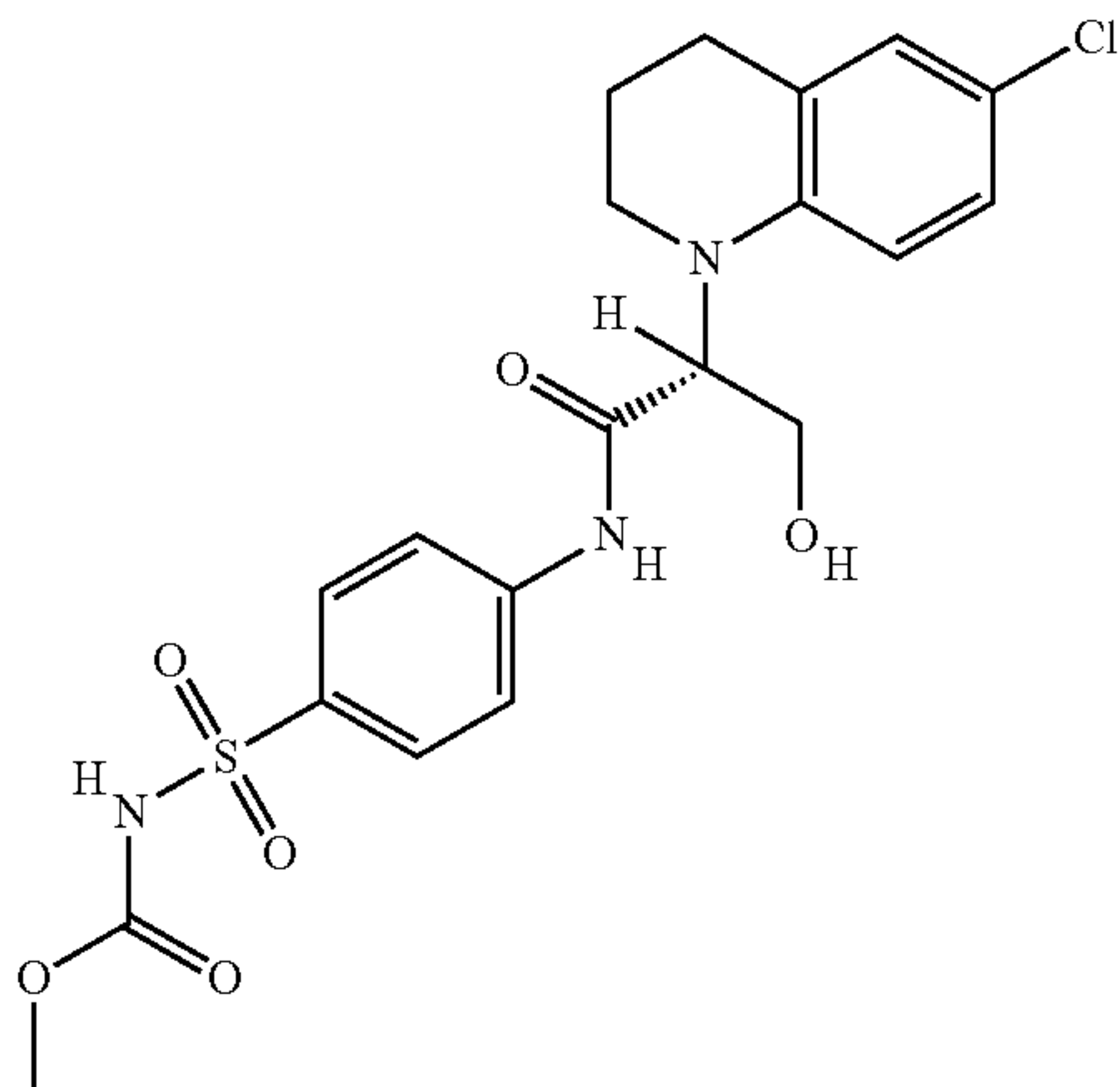
127 -continued
