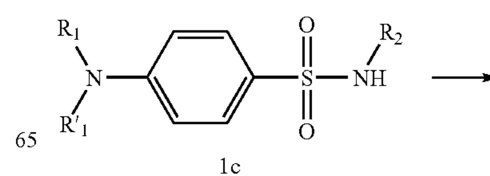
Scheme 13:
