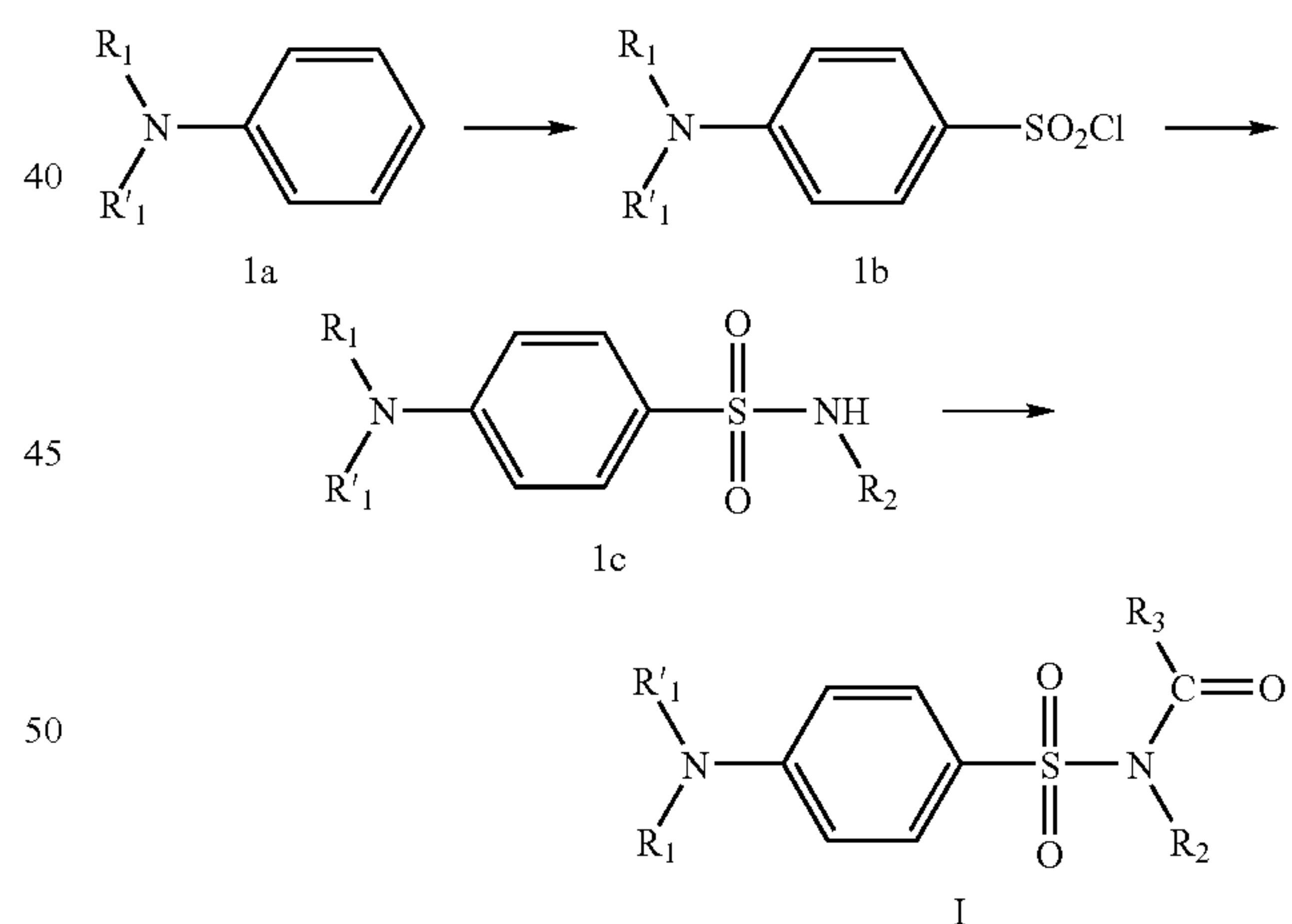
Scheme 1:
