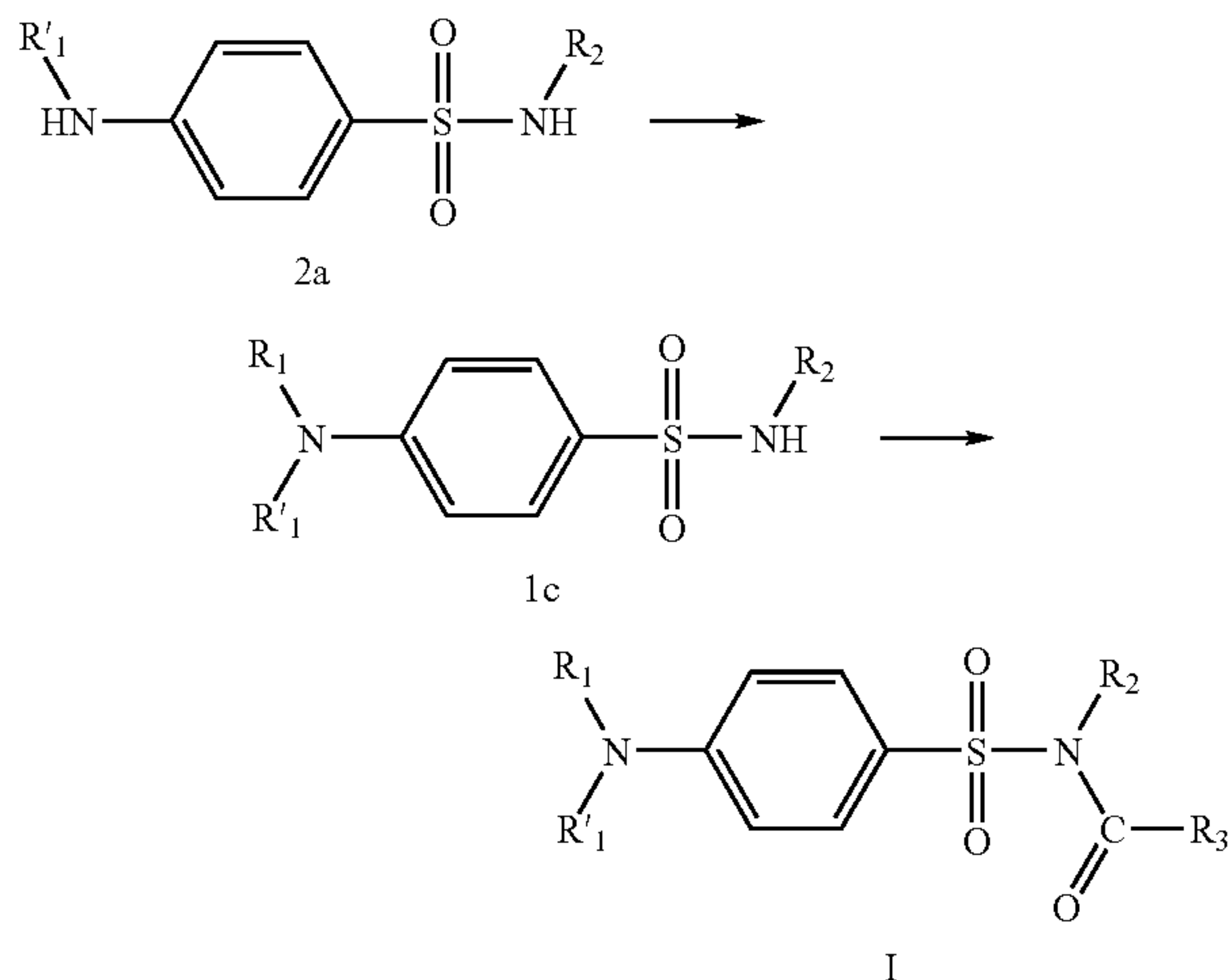
Scheme 2:
