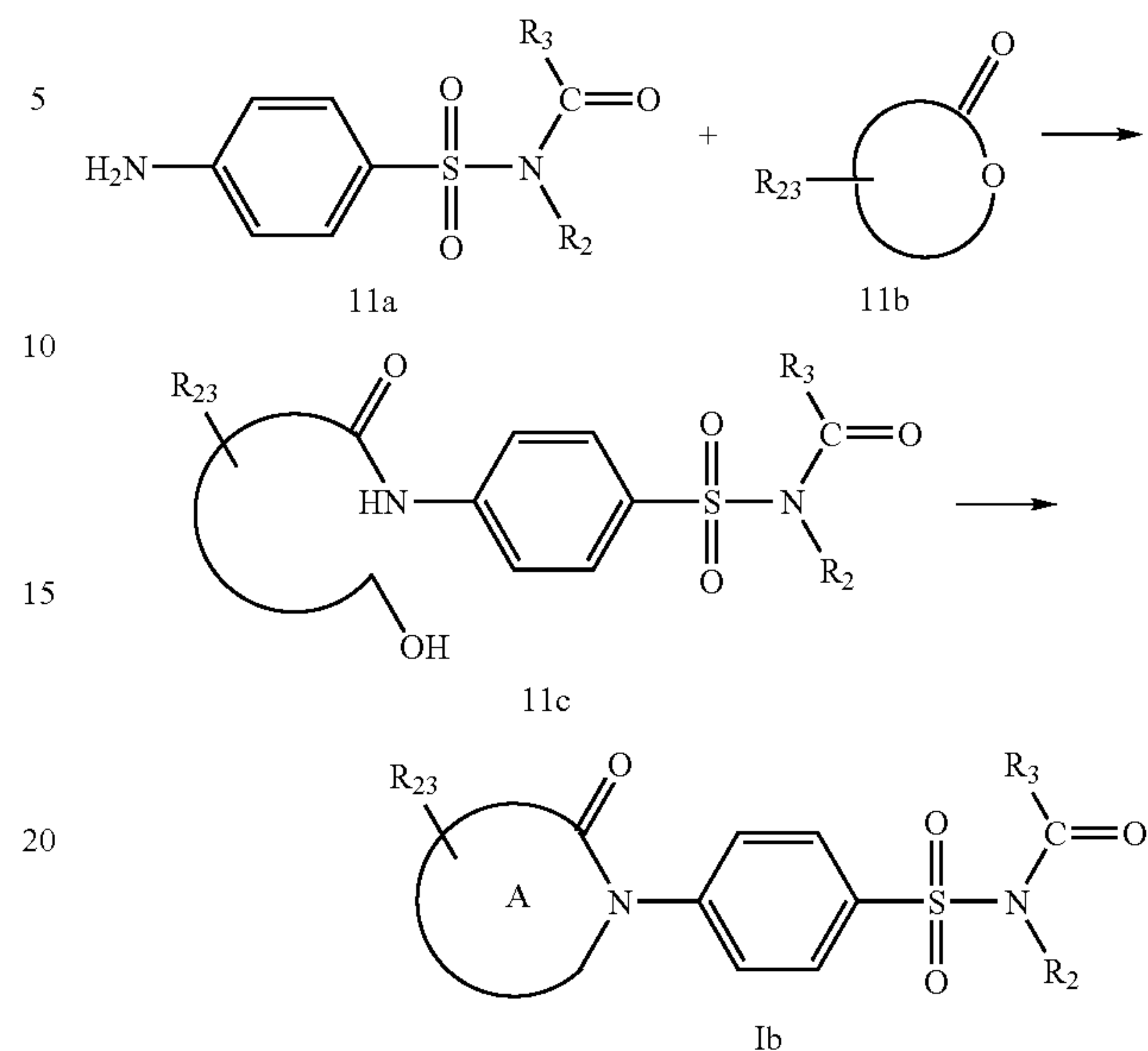
Scheme 11:
