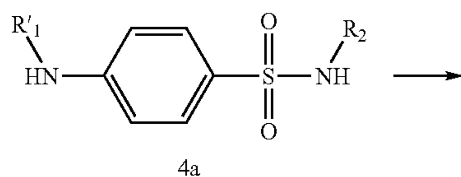
Scheme 4:
