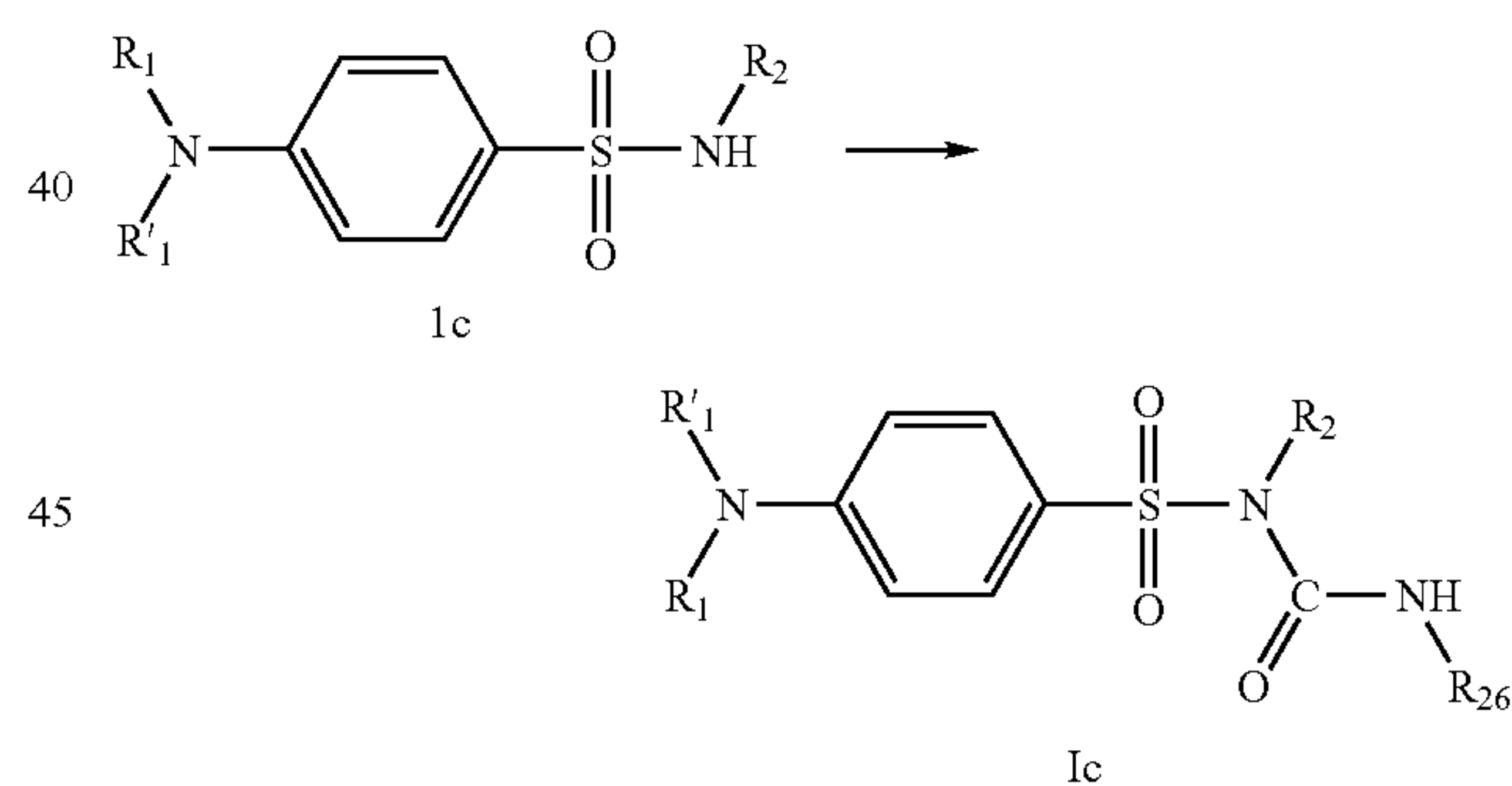
Scheme 12:
