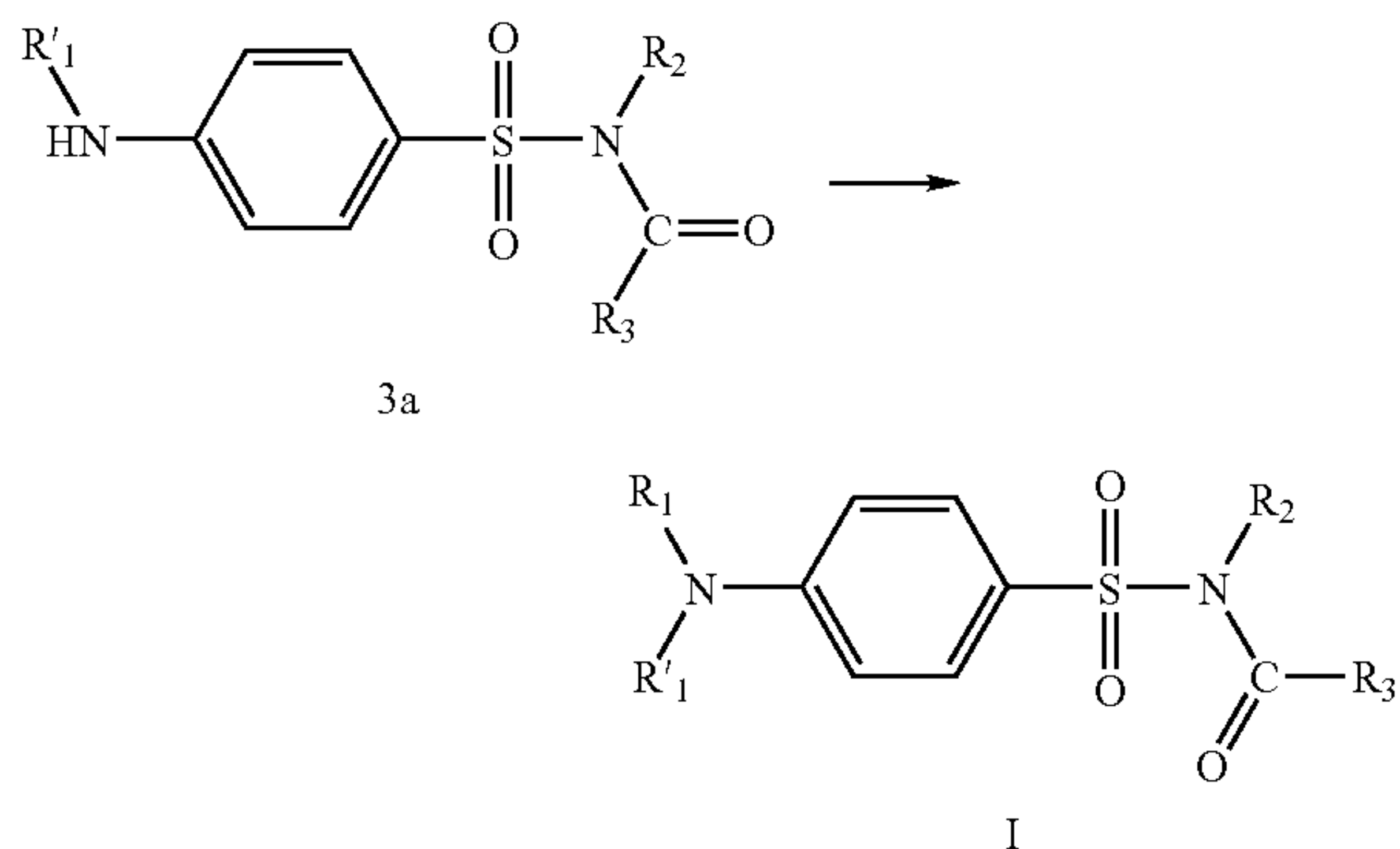
Scheme 3:
