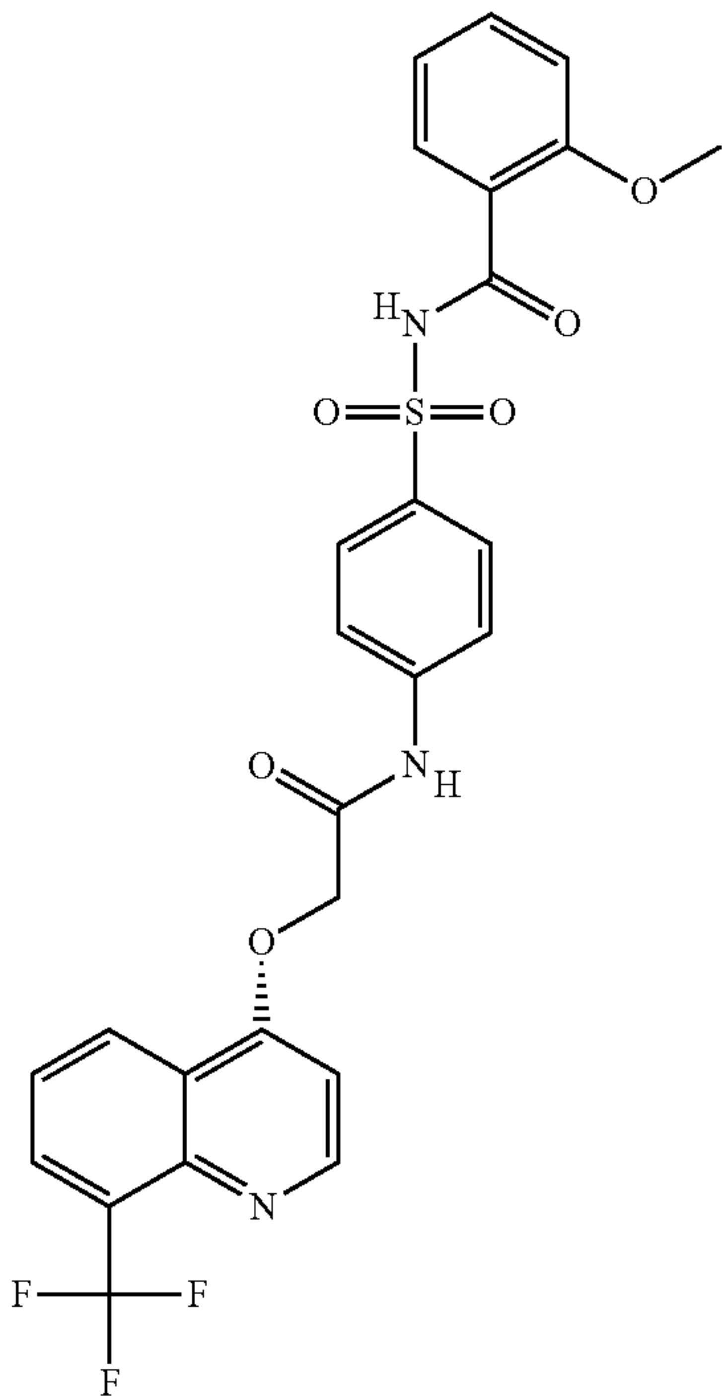
119 -continued
