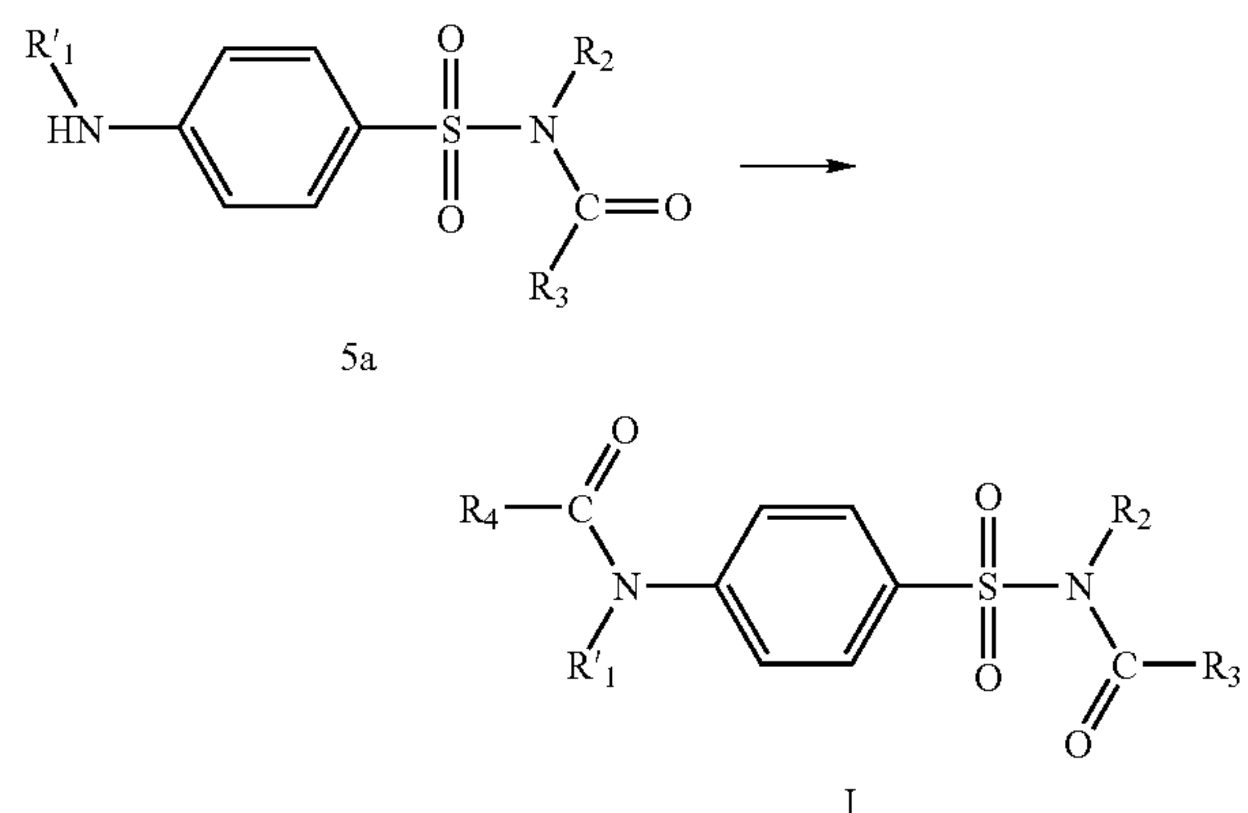
Scheme 5:
