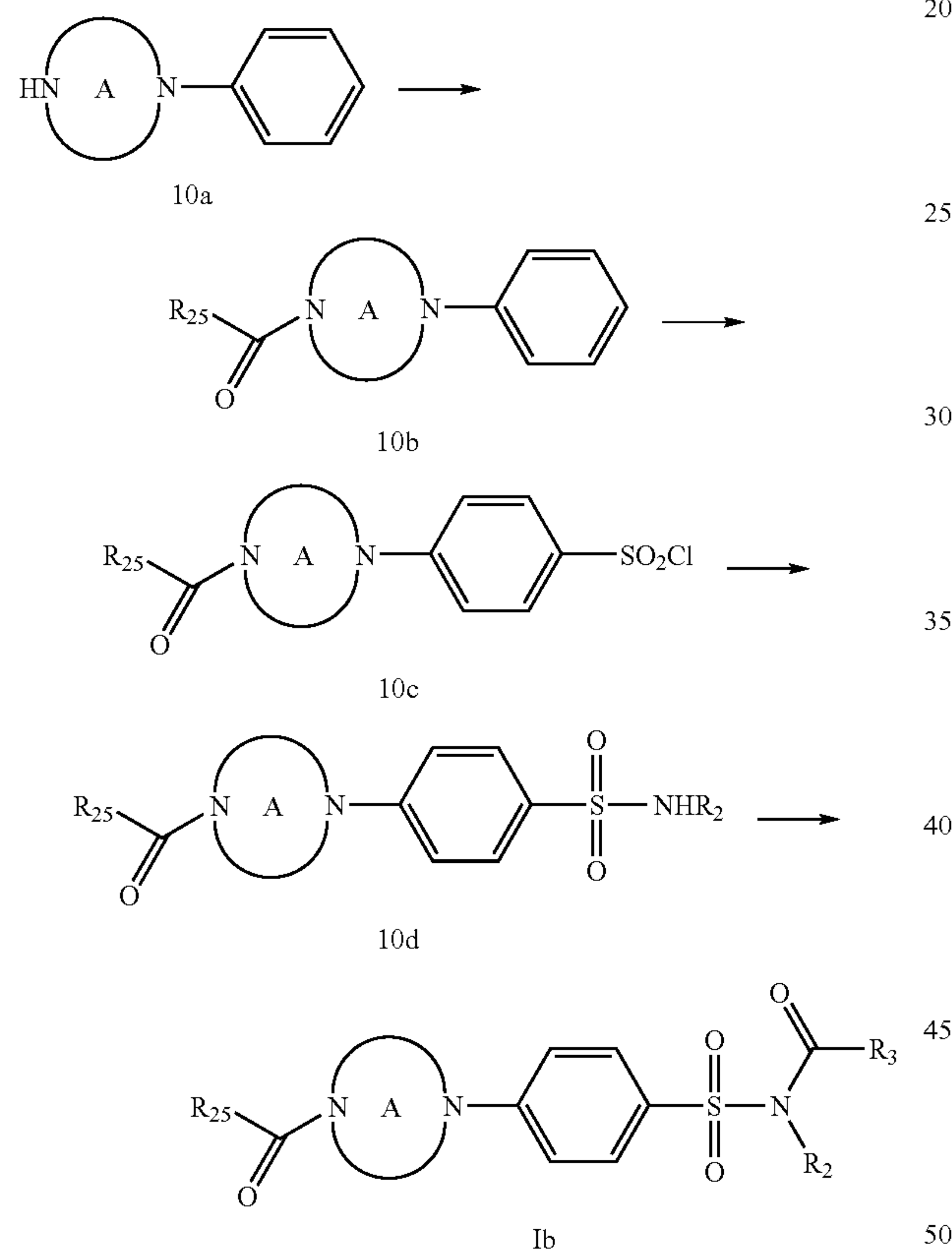
Scheme 10:
