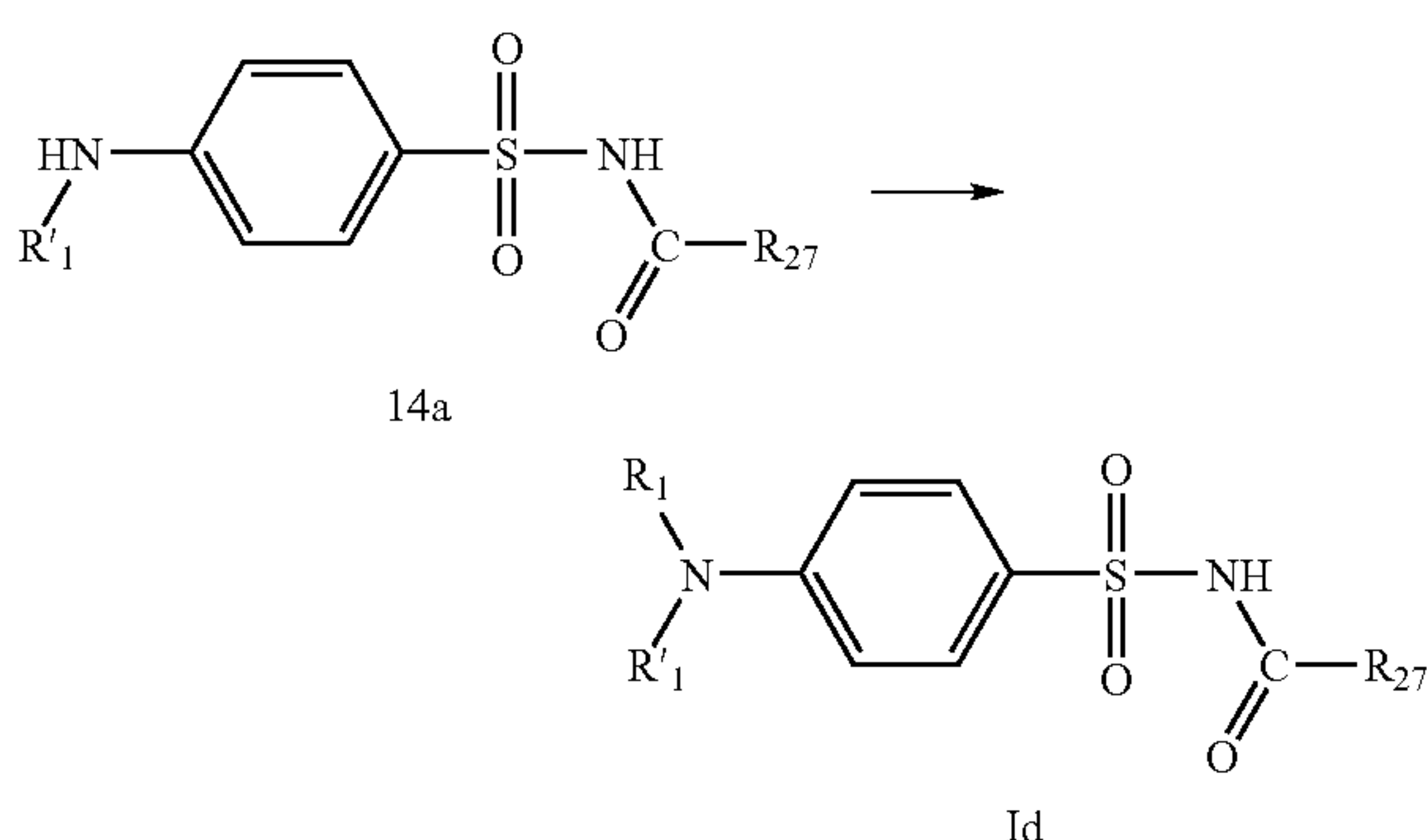
Scheme 14:
