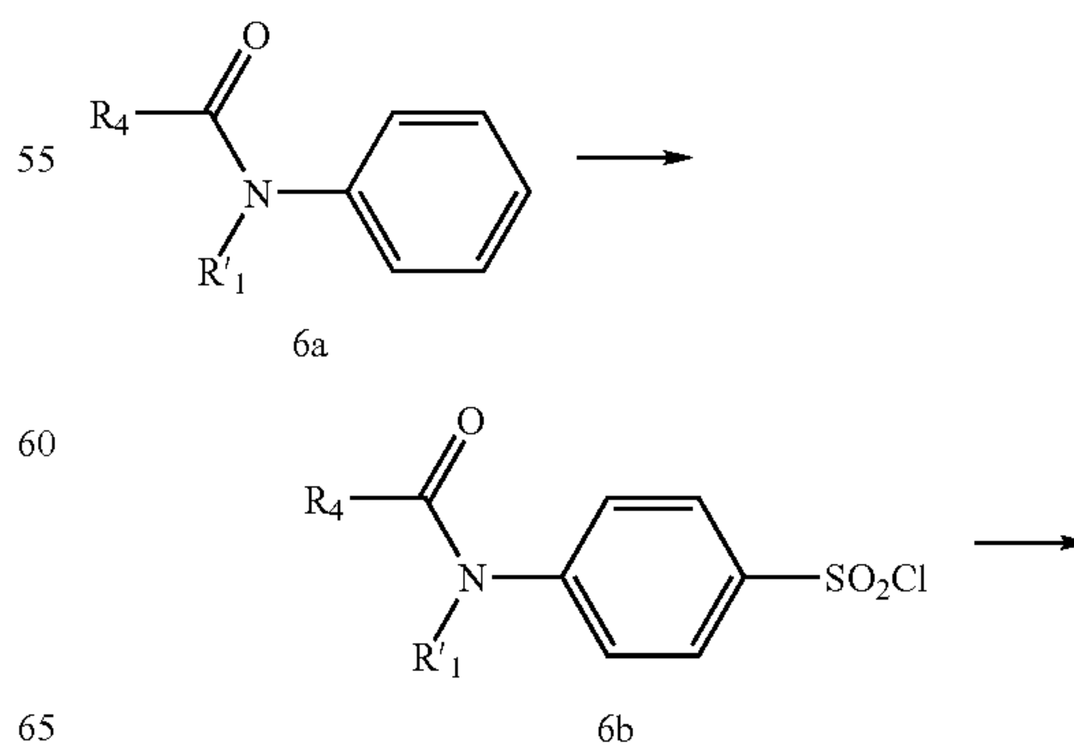
Scheme 6:
