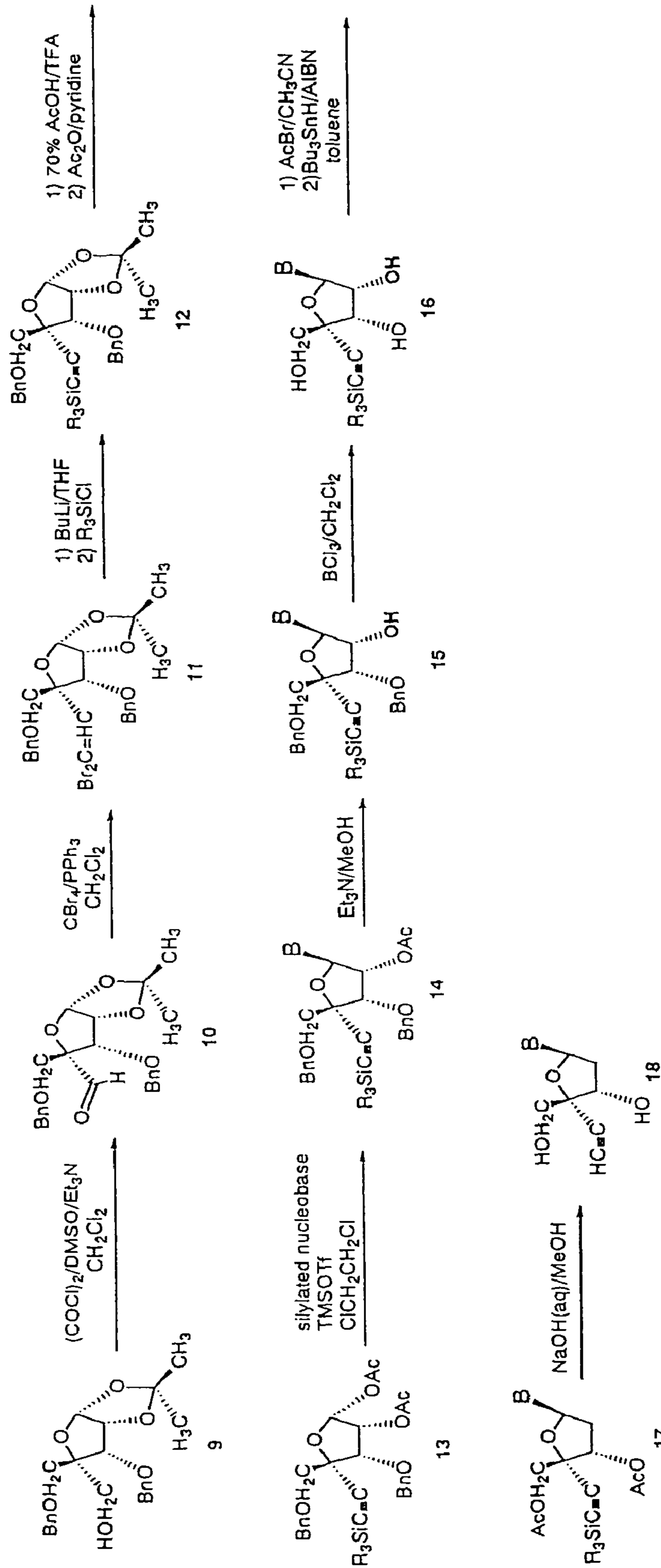
Scheme 2. Synthesis of 4'-ethynyl-2'-deoxynucleosides from sugar precursor
