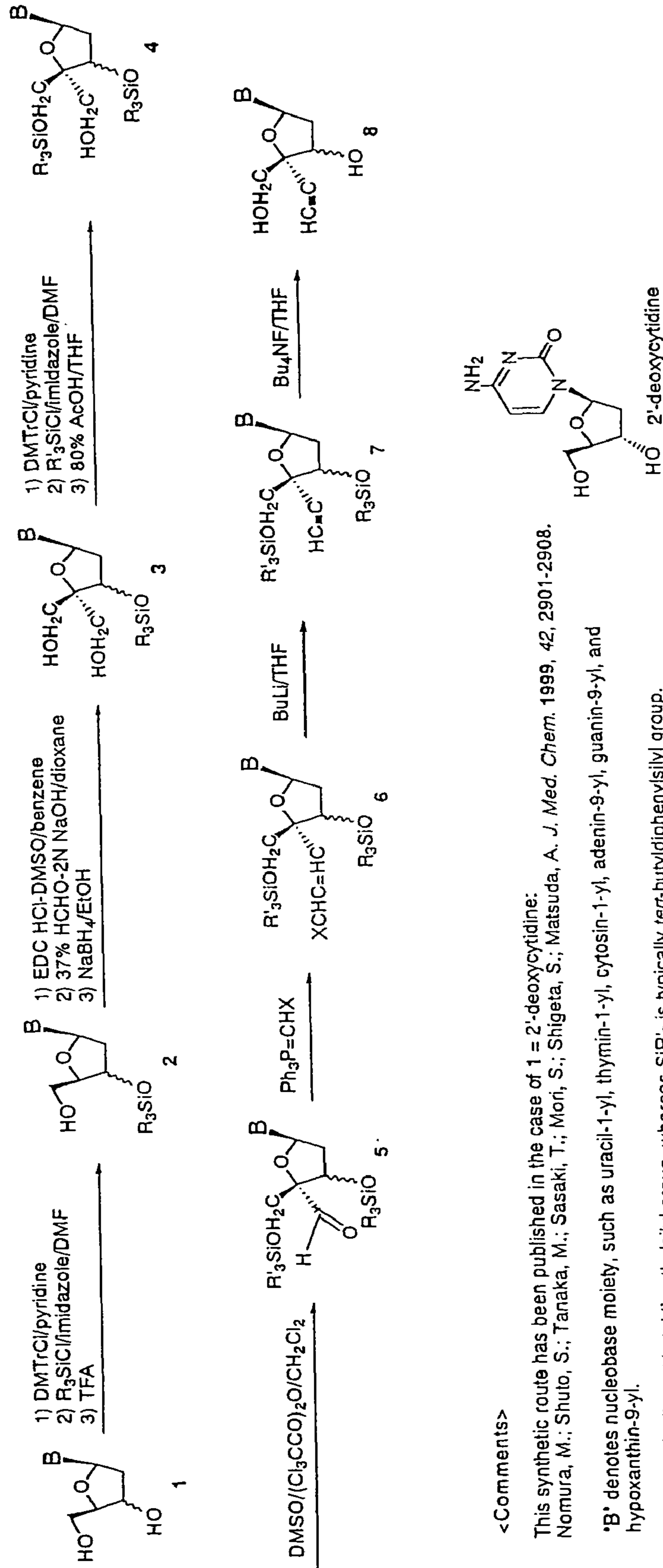
Scheme 1. Synthesis of 4'-ethynyl-2'-deoxynucleosides from 2'-deoxynucleosides
