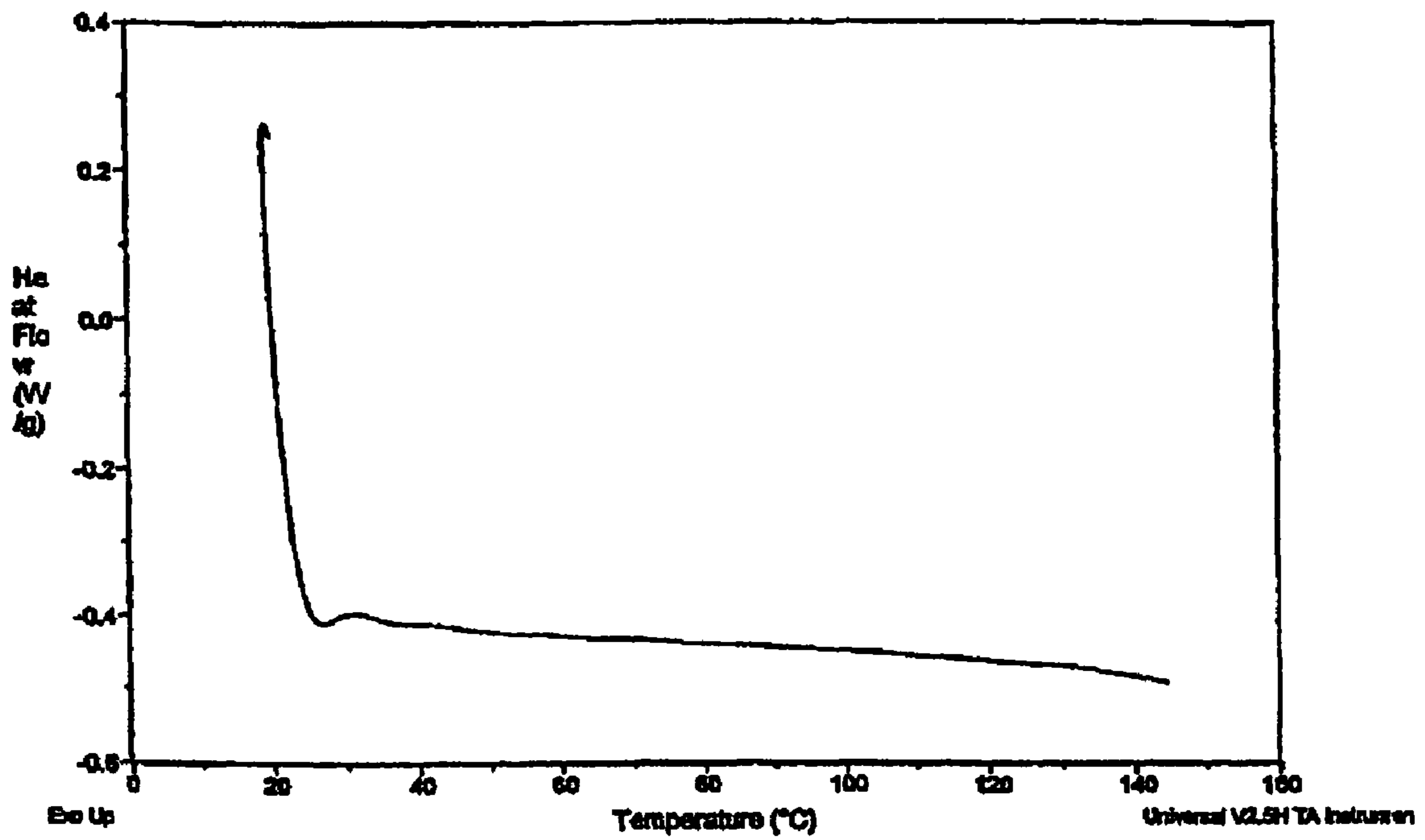
Fig. 1. DSC Thermograms of the starch described.
