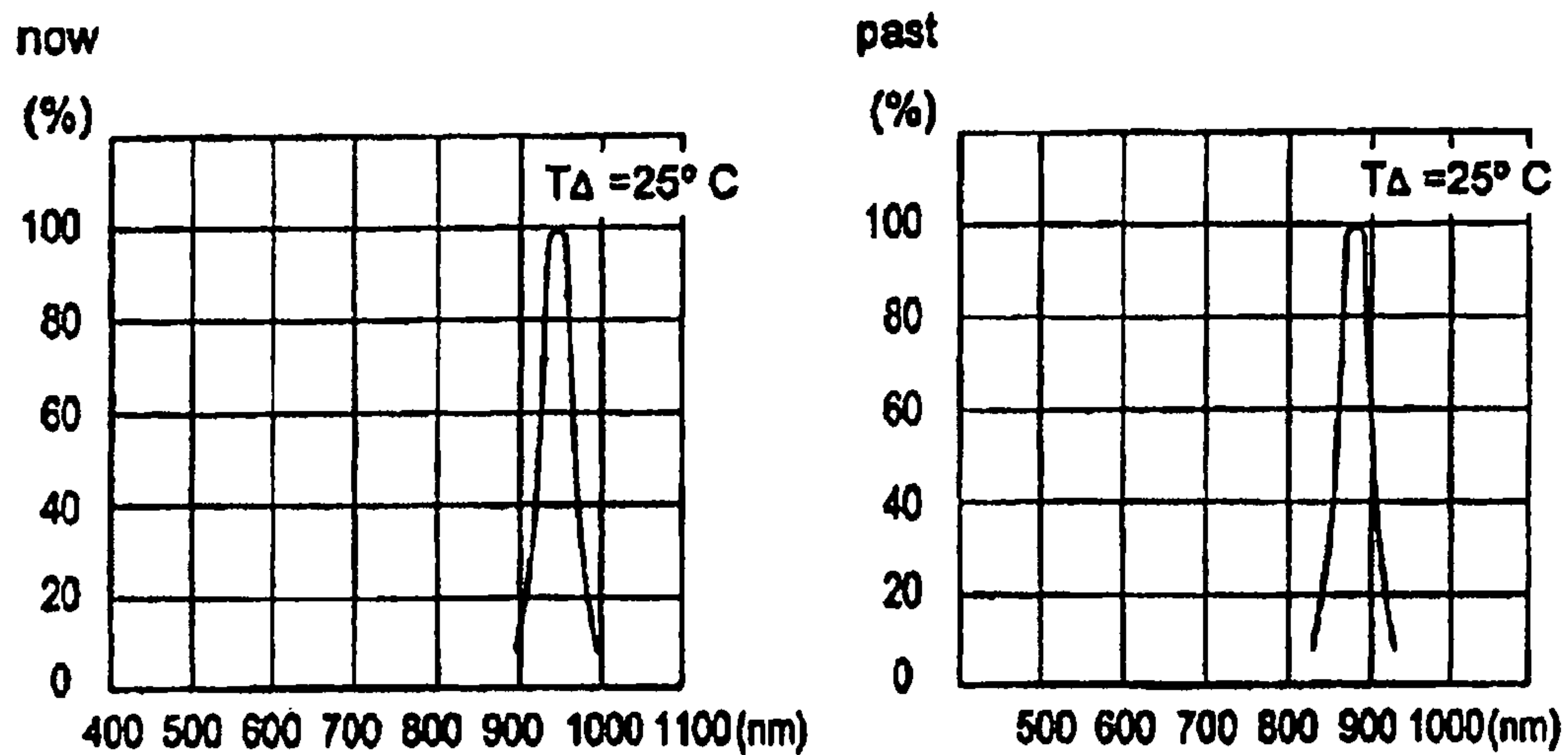
The spectral curve of the LED
