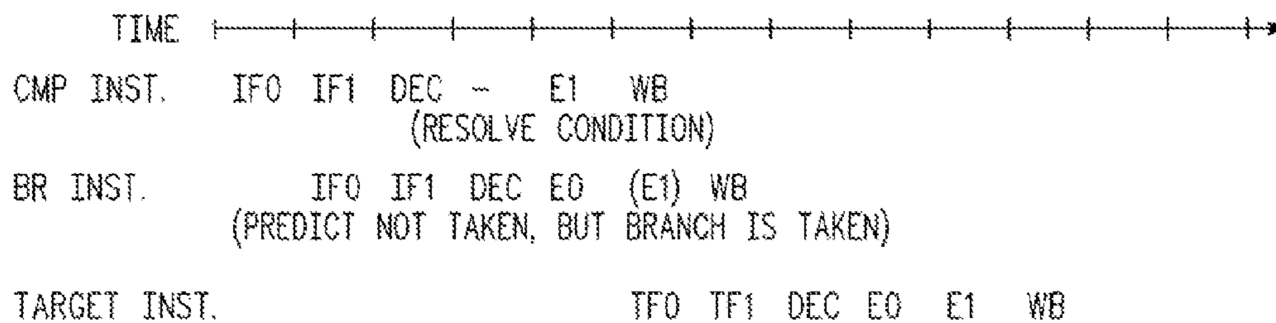
BASIC PIPELINE FLOW, BRANCH INSTRUCTIONS, PREDICT NOT TAKEN, INCORRECT PREDICTION, ECC MODE
