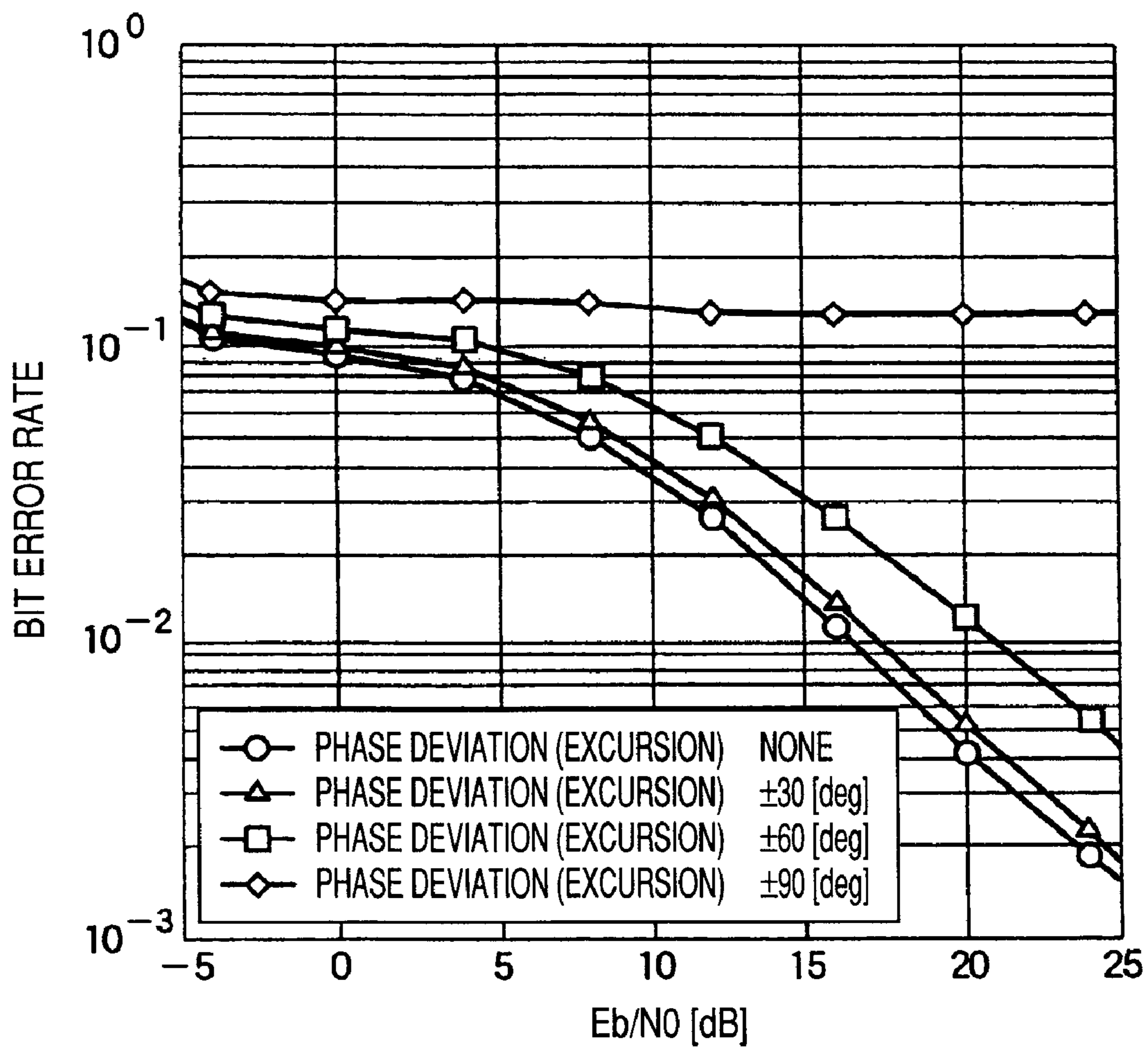
RECEPTION CHARACTERISTIC FOR E_b/N_0
