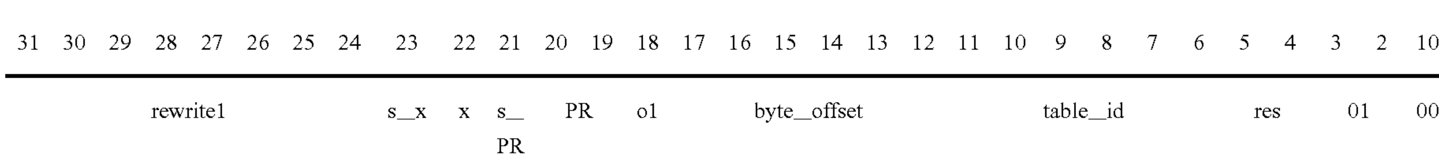
Regular Termination res = 2'b10, 2'b11 Instruction Format
