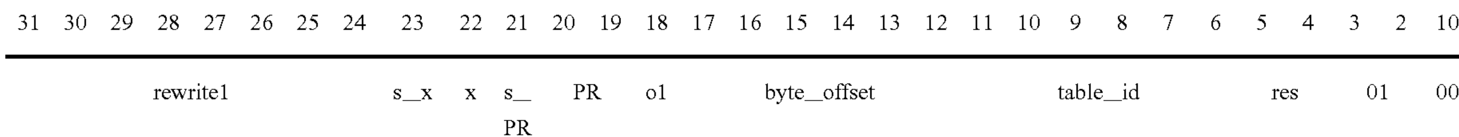
Regular Termination res = 2'b10, 2'b11 Instruction Format
