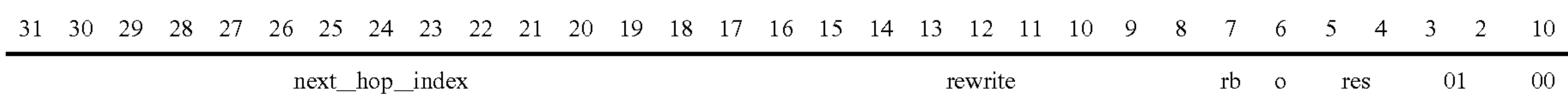
Regular Termination res = 2'b01 Instruction Format
