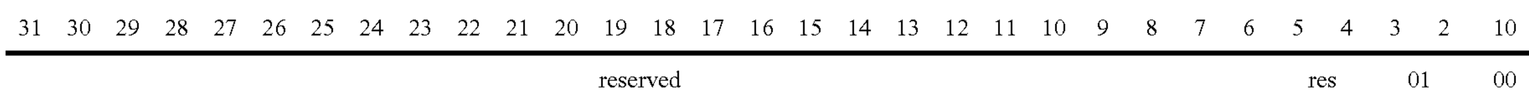
Regular Termination res = 2'b00 Instruction Format
