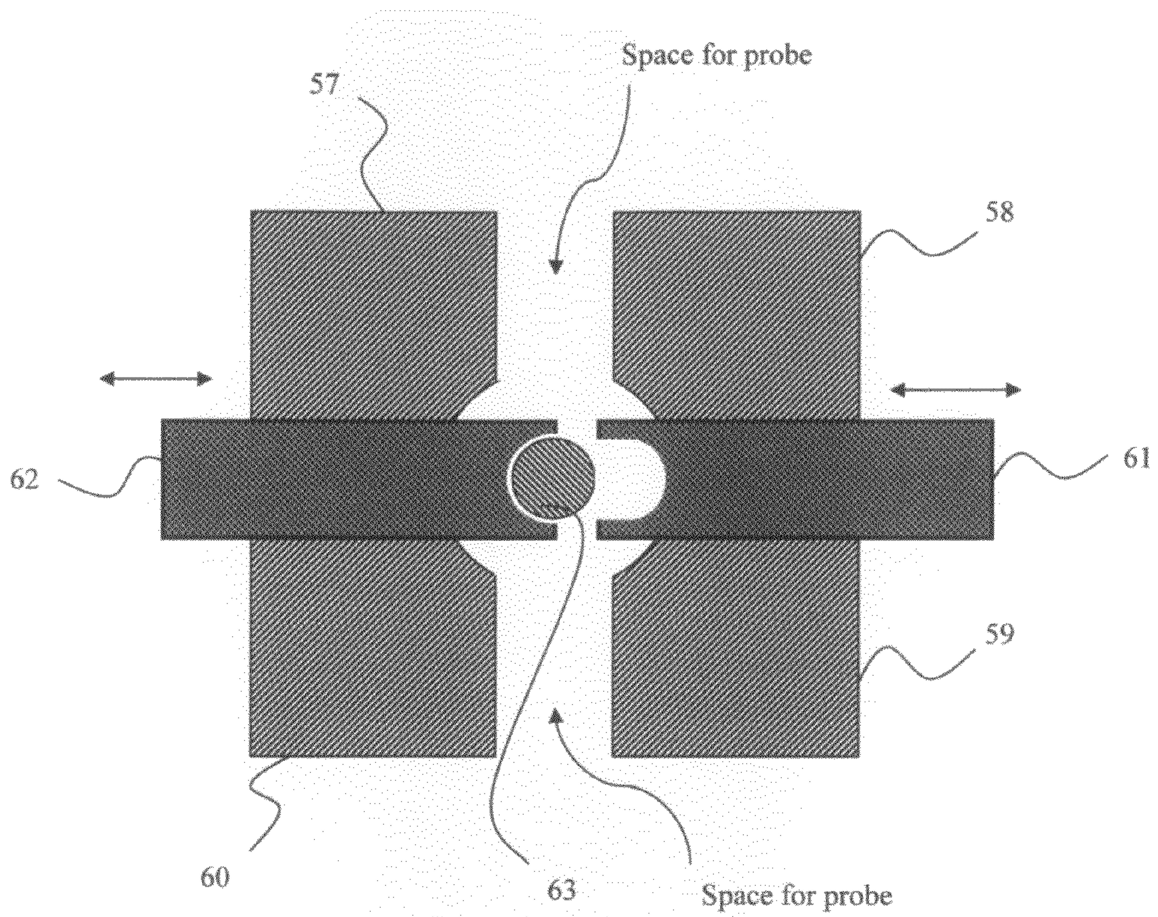
Figure 12: Concept of double slabline with two probes
