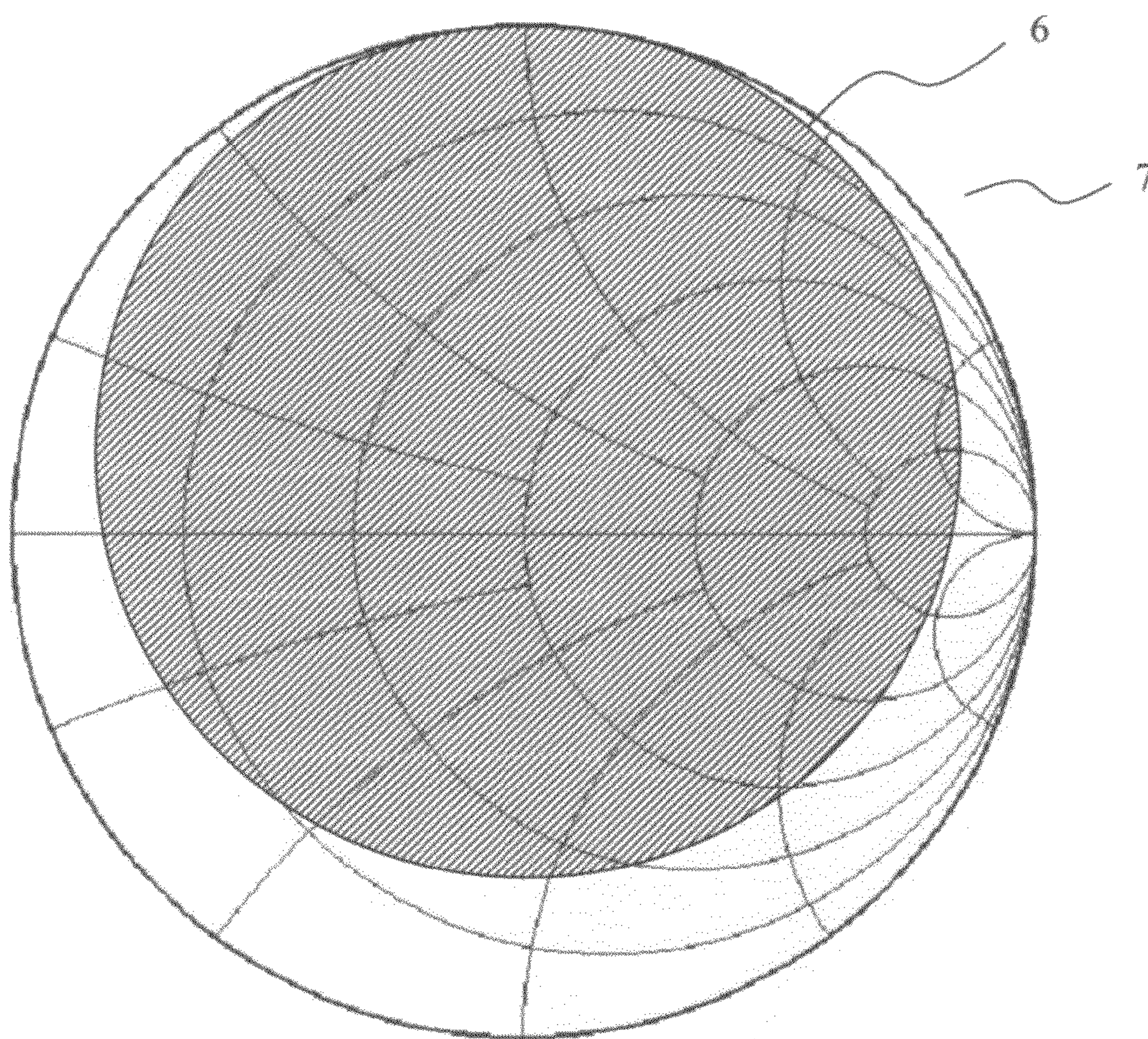
Figure 2: Prior art, tuning range of slide screw tuner
