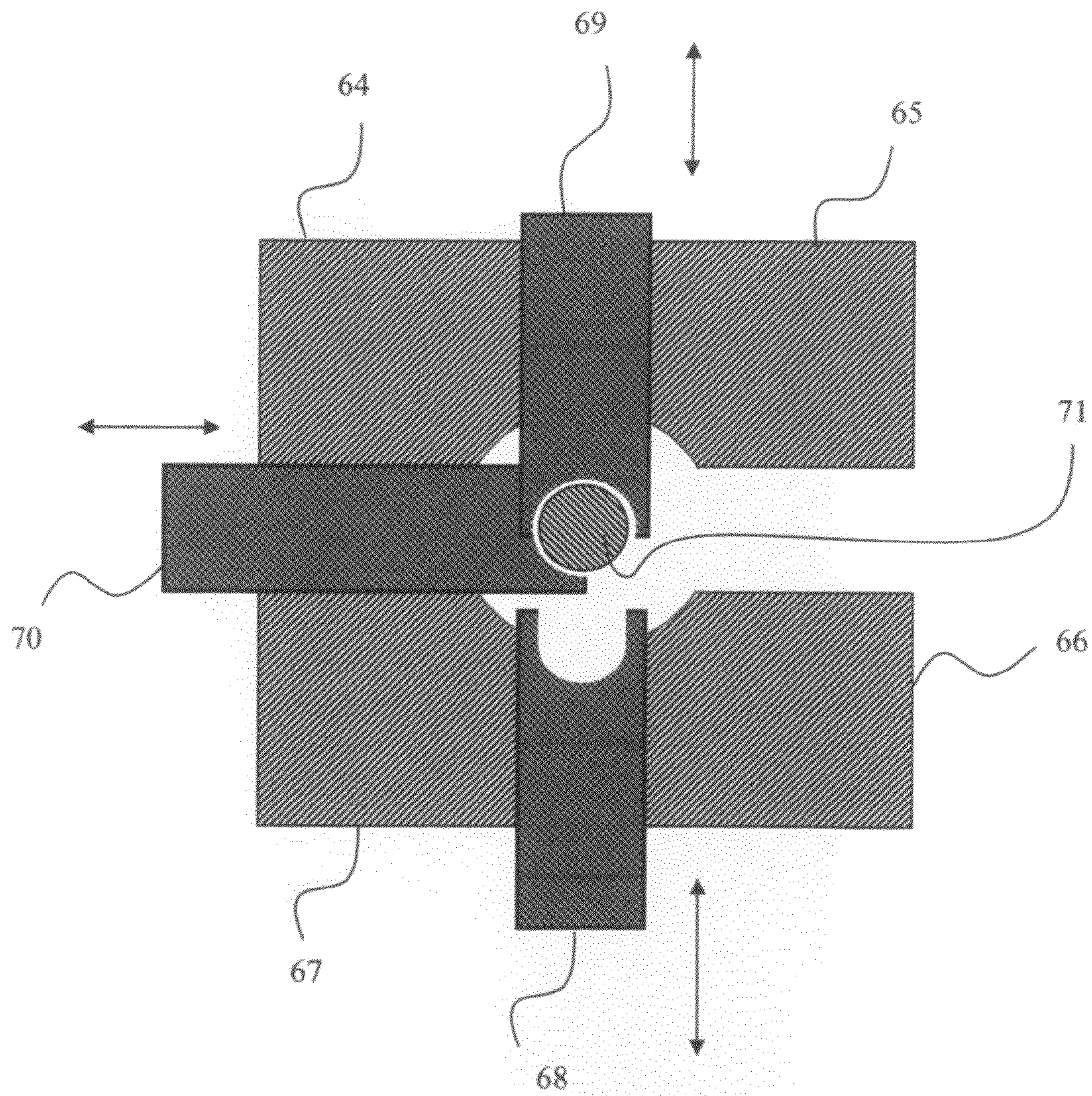
Figure 13: Concept of double slabline with three probes
