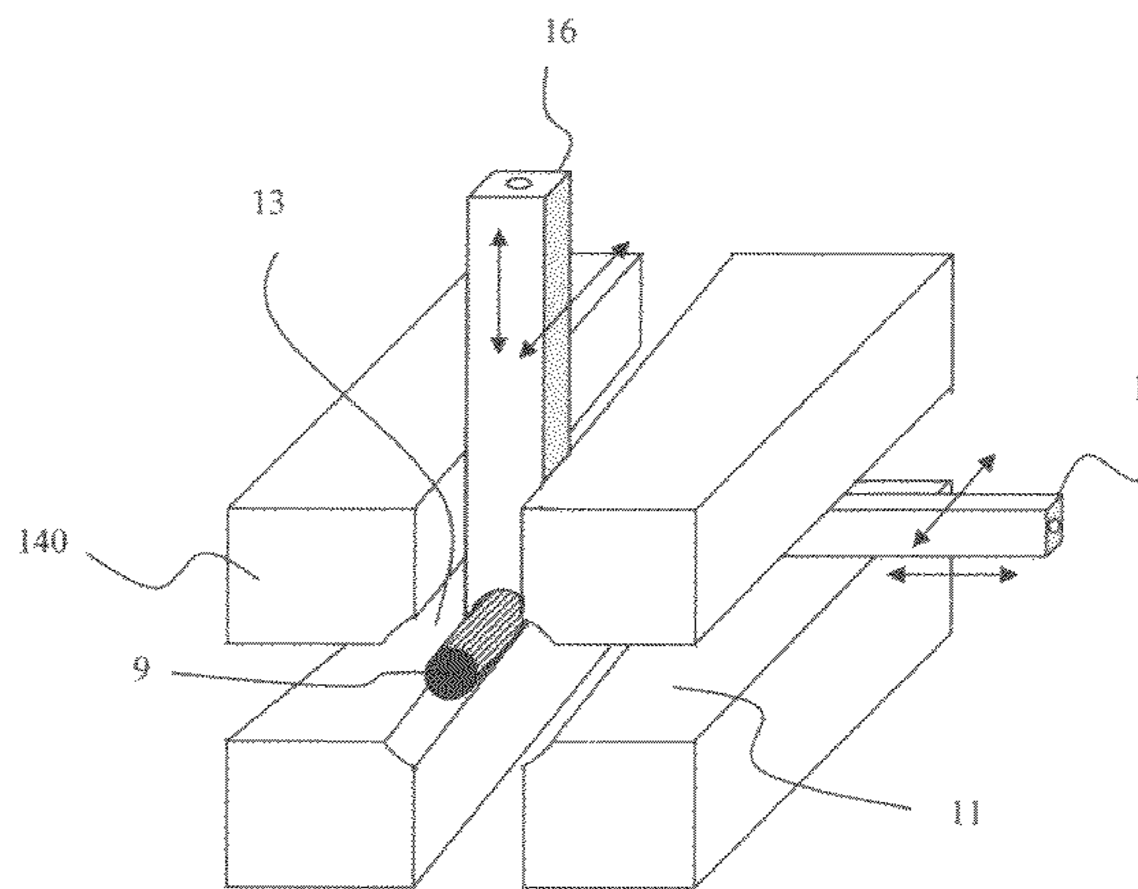
Perspective view of double slabline with probes
